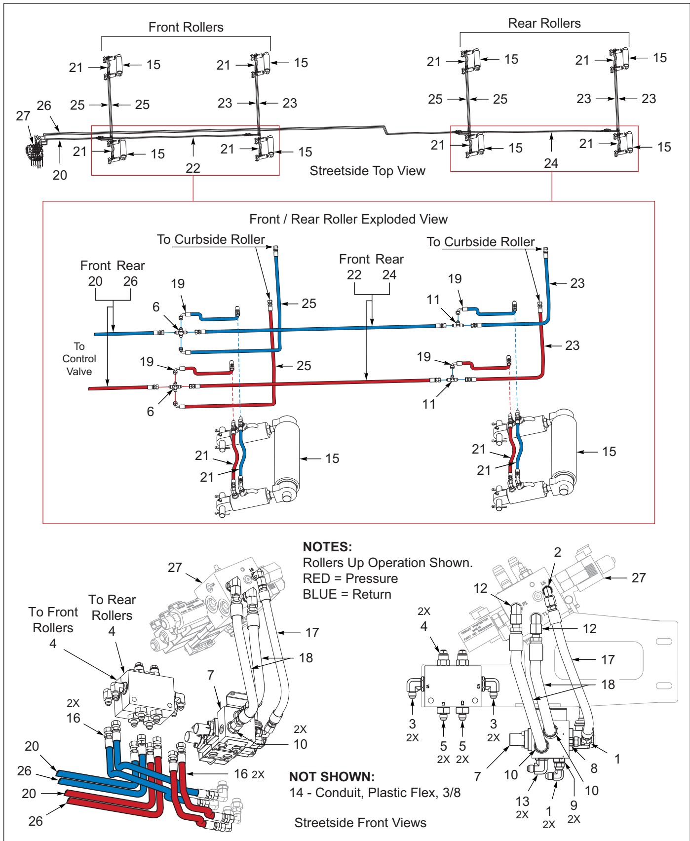
Figure 11-6: Rollers, Deck, 8-Pop-Ups, 48 / 50 / 53 Foot (Options)
