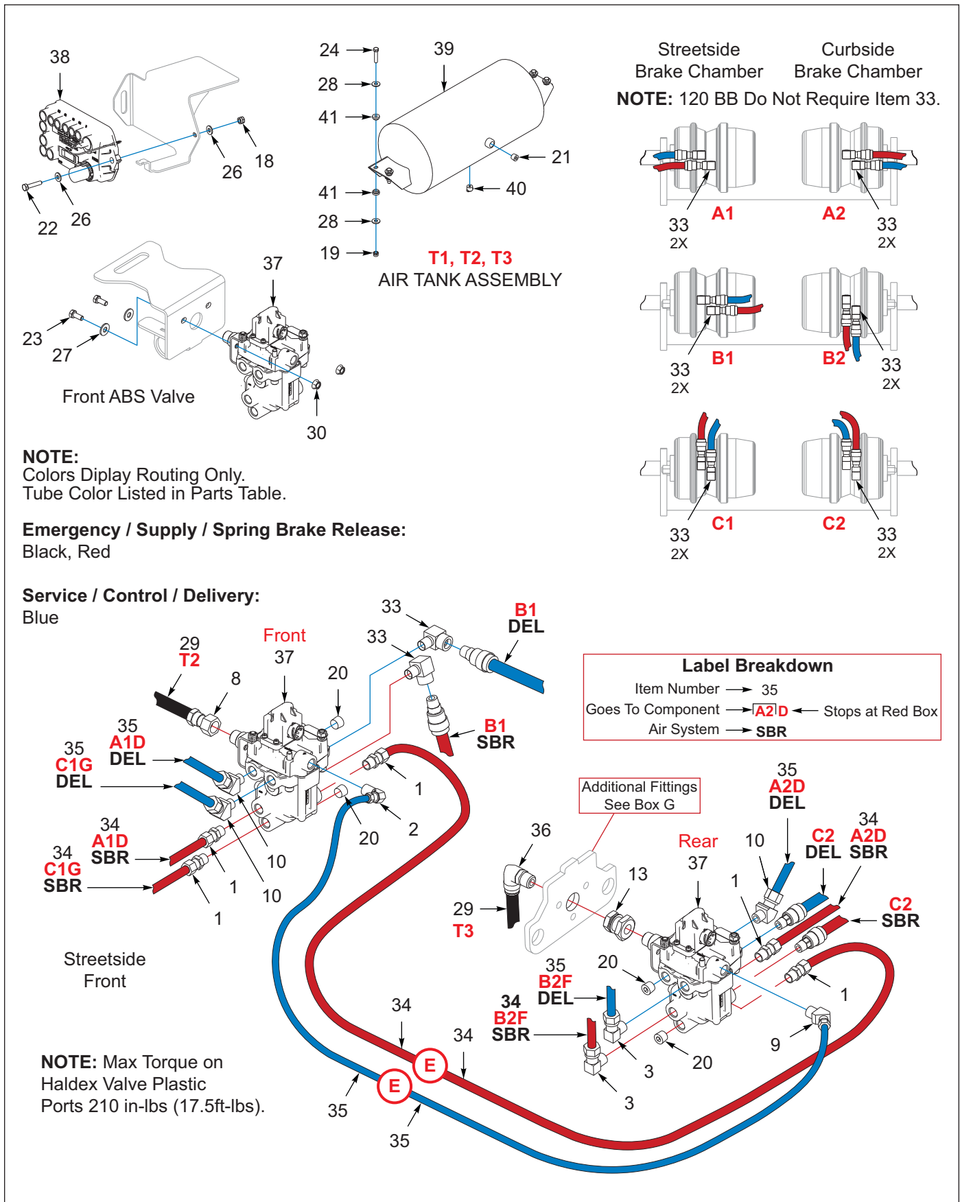
Figure 8-14: ABS, 3 Axle, Disc, Haldex, 120 (Option) (After 12/01/2025) (2 of 2)
