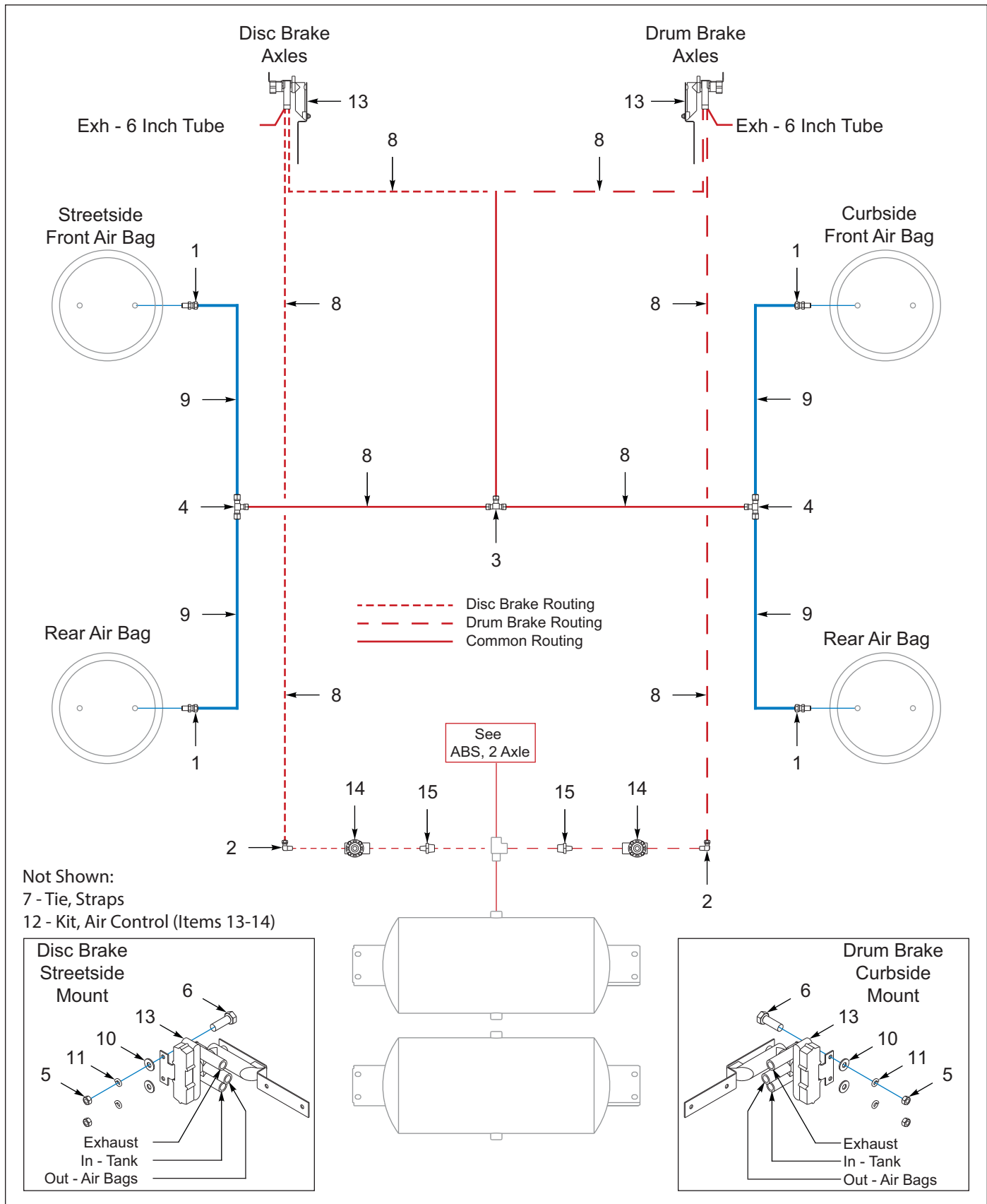
Figure 8-40: Suspension, Air Ride, 2 Ax, 1/4 in (Before 06/14/2023)
