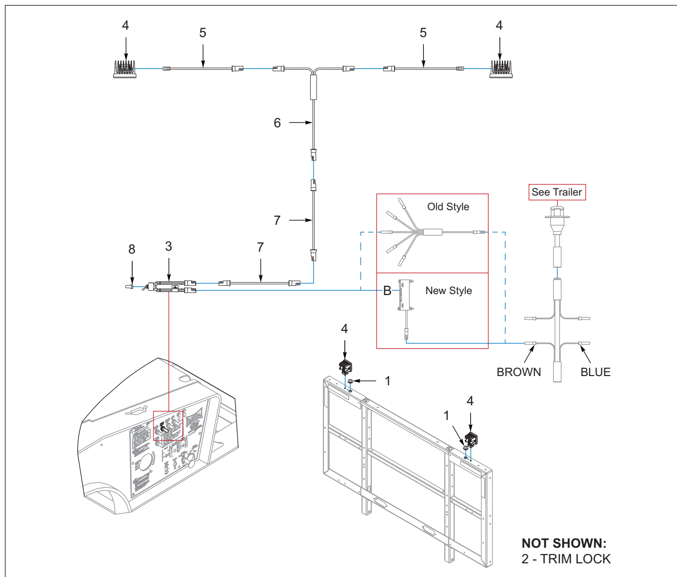
Figure 9-28: Lights, Work, Bulkhead (Options)
