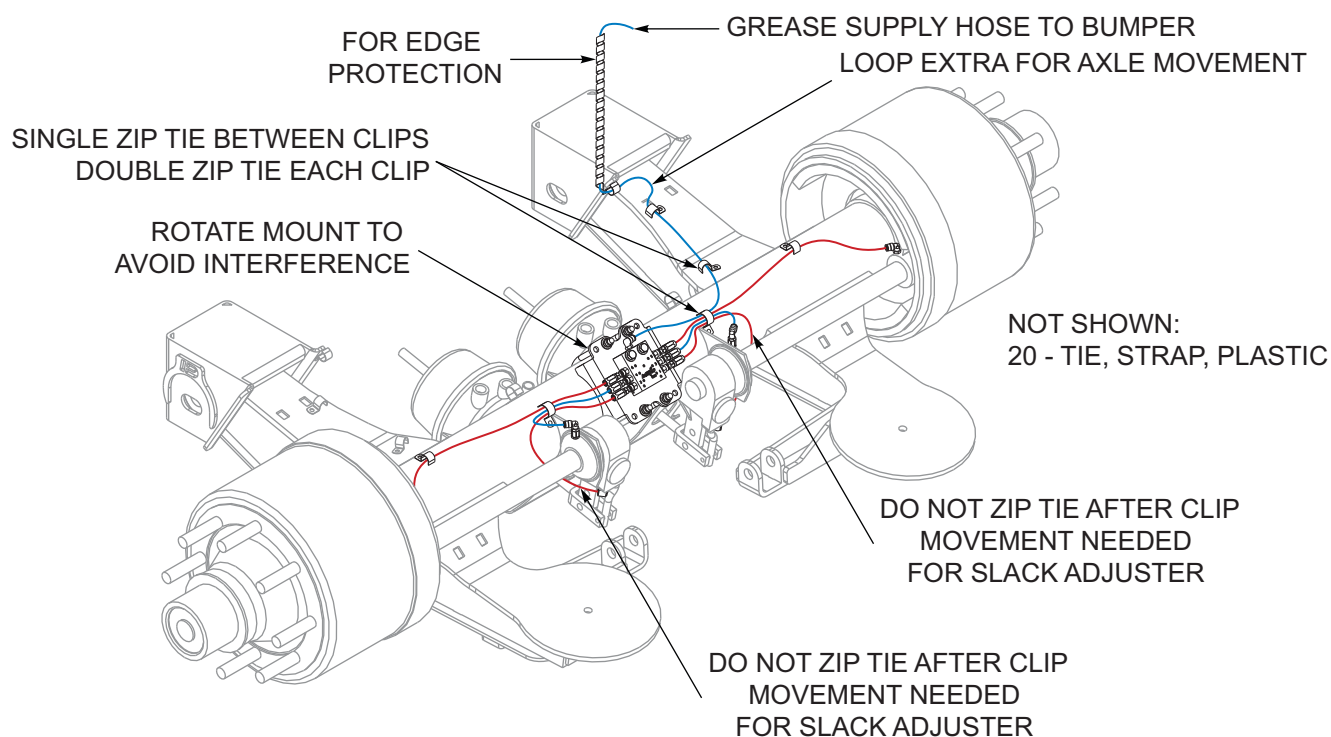
Figure 10-8: Axle, Drum Brakes (After 08/31/2020 To 09/01/2024) (3 of 3)
