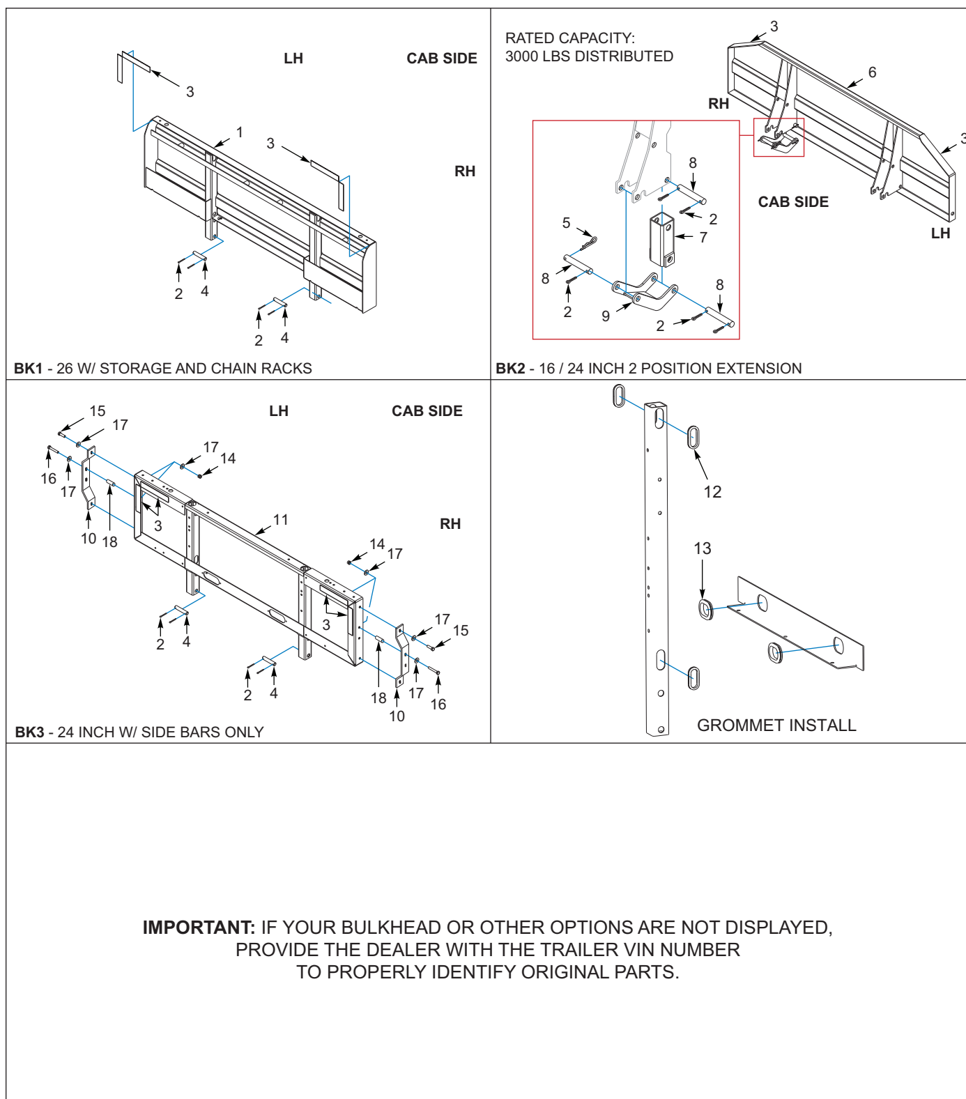
Figure 4-1: Bulkhead Components, 24, 25 & 26 x 102
