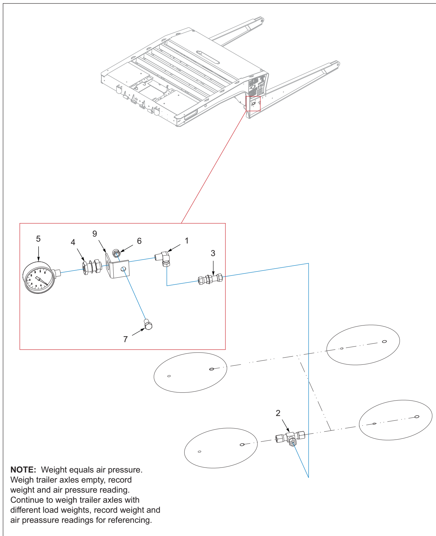
Figure 8-35: Scale, Air Pressure Gauge (Option)
