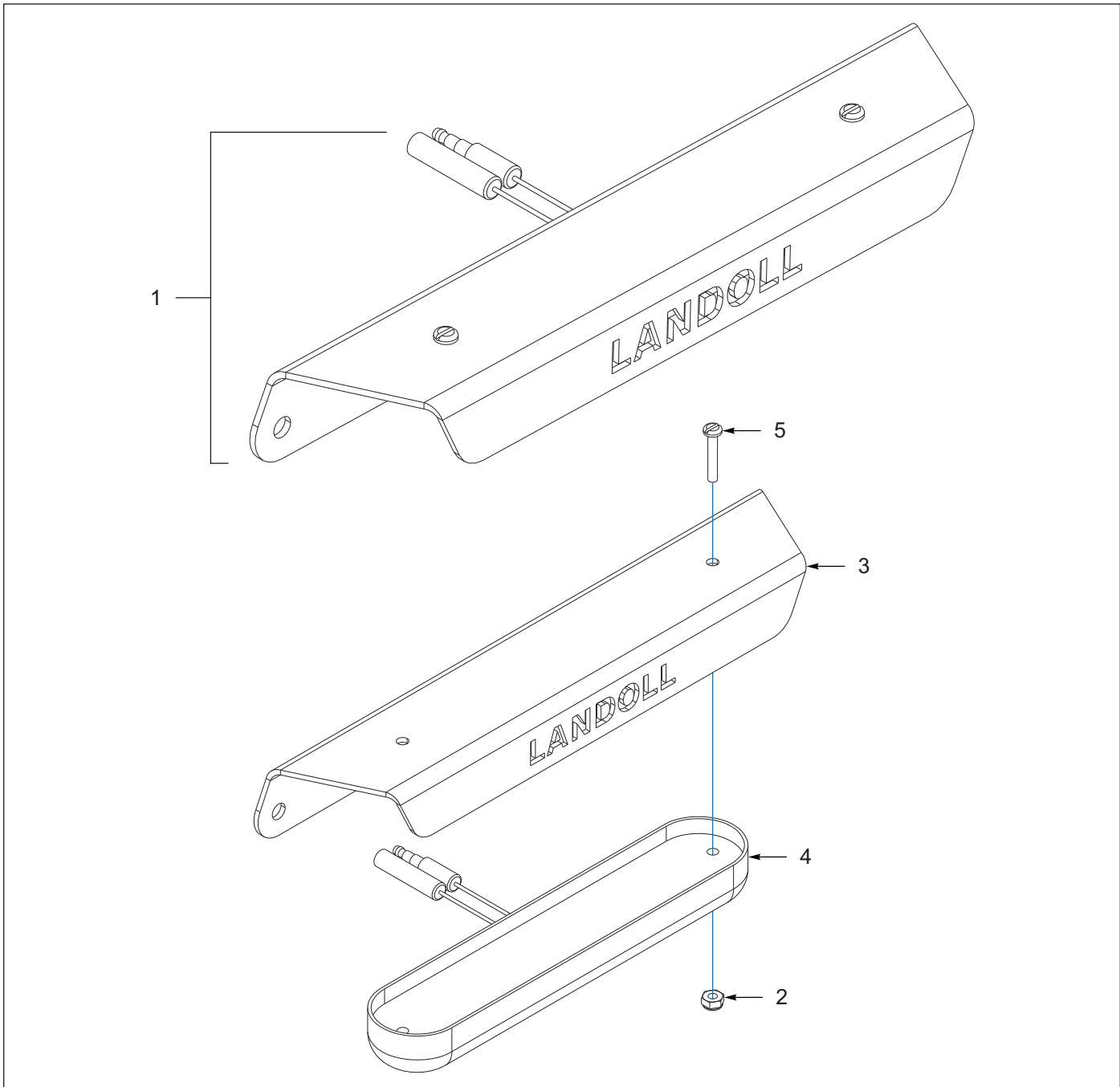
Figure 9-18: Light Assembly, Control Panel
