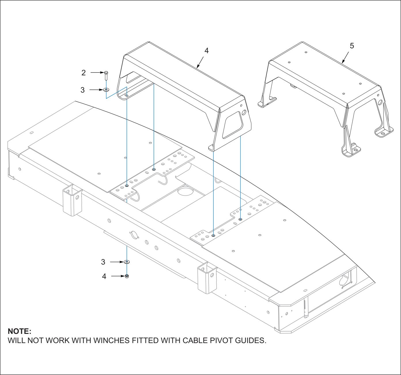
Figure 7-26: Guard, Winch, WO/ Cable Pivot Guide
