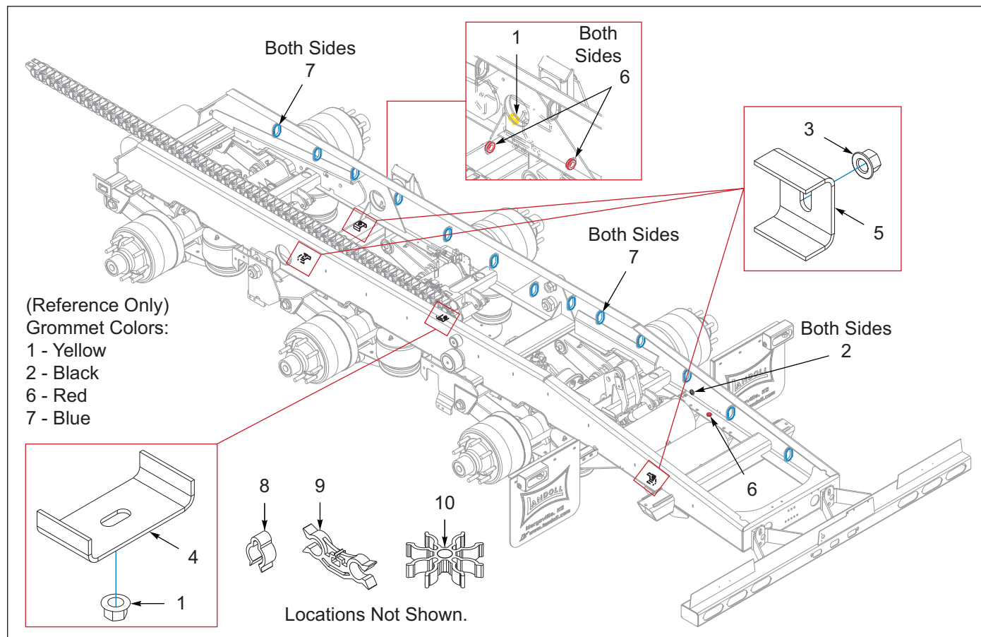
Figure 2-19: Hose Clamps, Clips, Grommets, 2 Axle (03/10/2023 To 12/01/2025)
