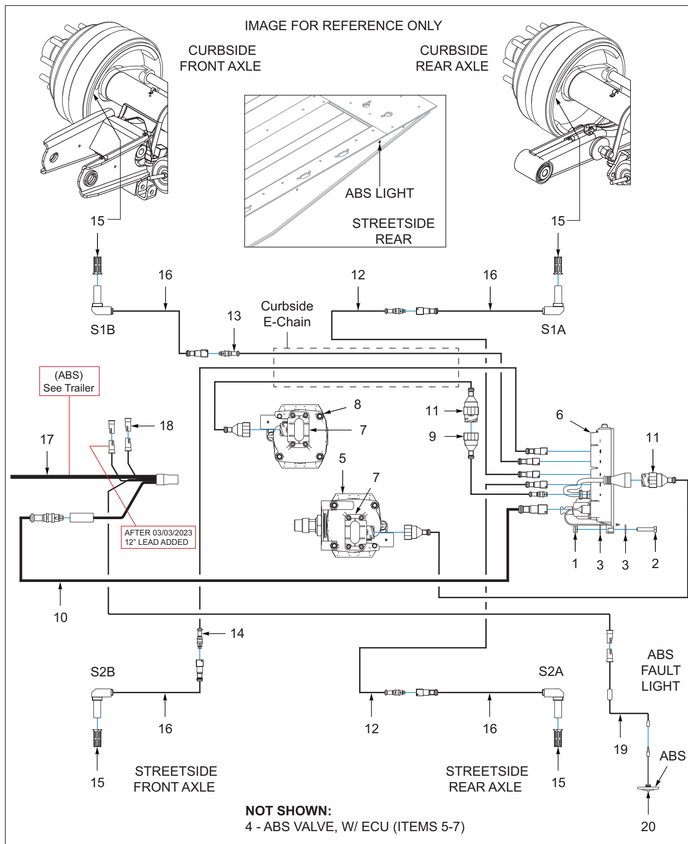
Figure 9-11: ABS, Haldex, 2 Axle, Spread (Option) (1 of 2)
