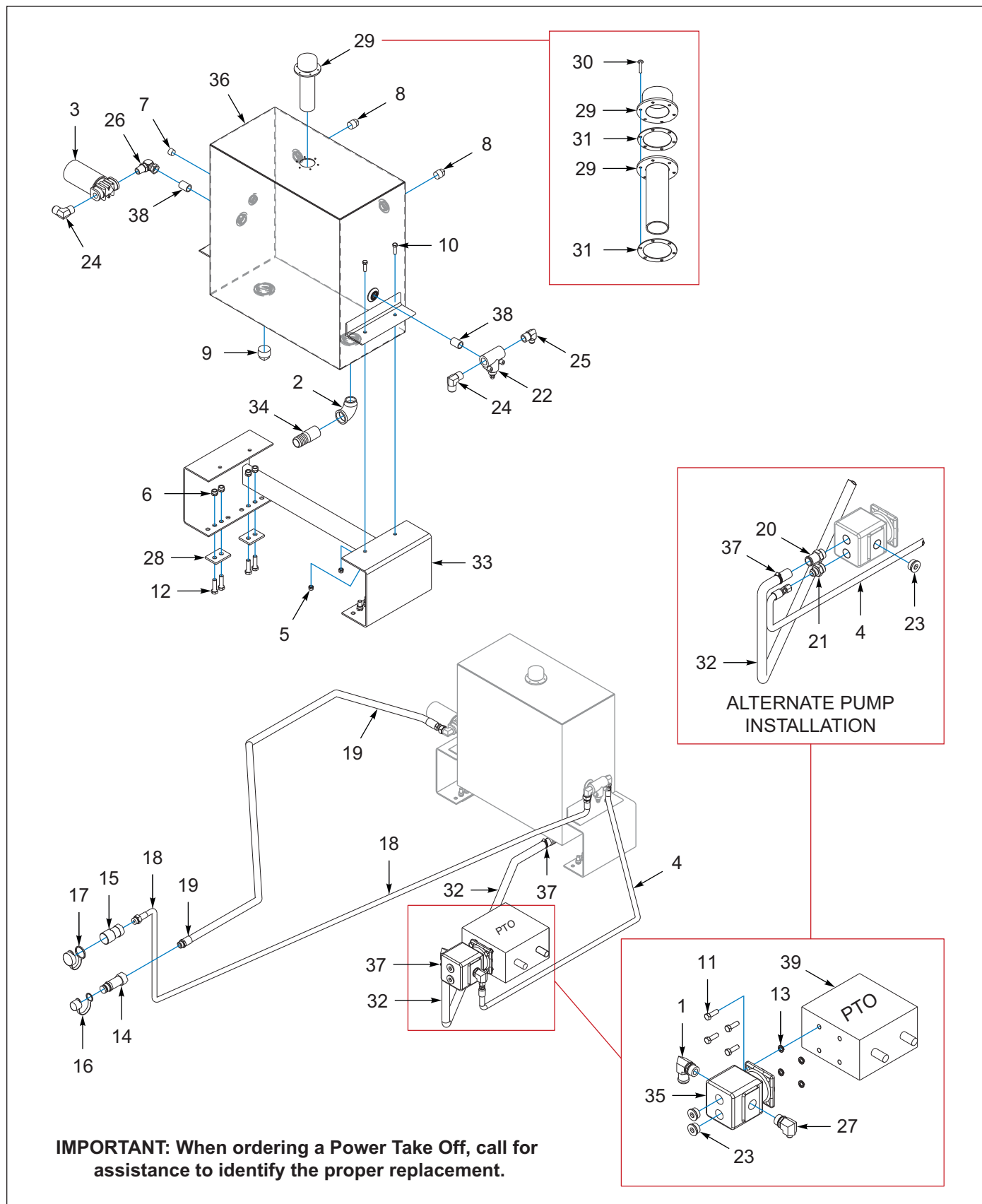
Figure 6-9: Wet Kit, Truck Hydraulic (Before 03/01/2019)
