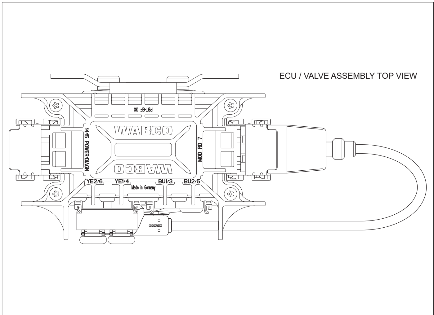
Figure 9-8: ABS, Wabco, Aqua (2 of 2)
