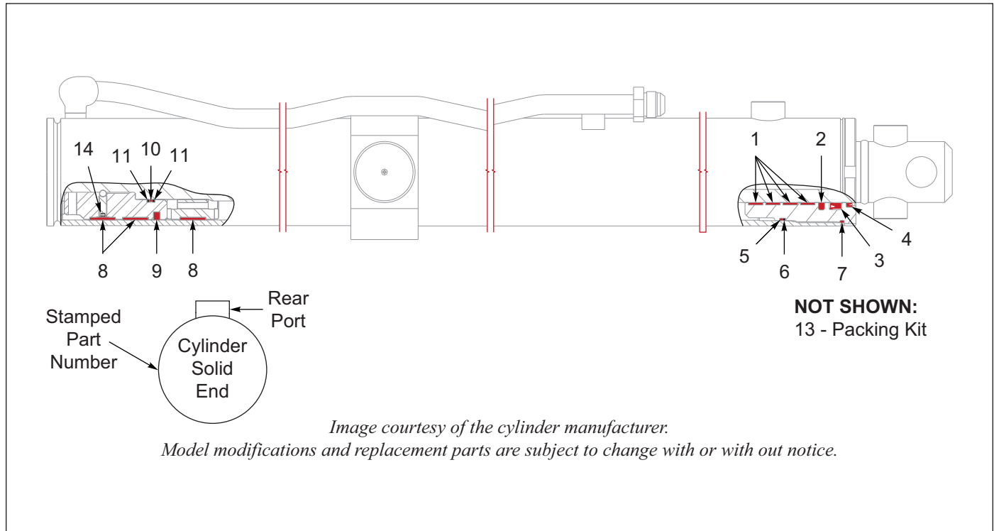
Figure 11-17: Cylinder Components, 4 x 100, 126, 138, Hi-Flow, Ported Rod, Dantal
