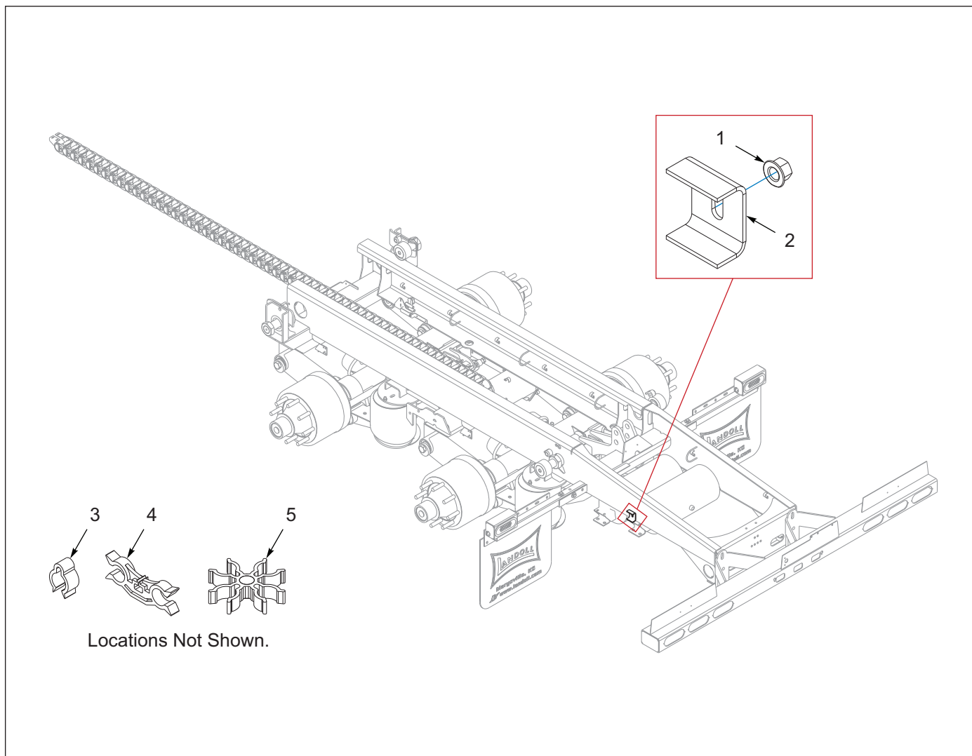
Figure 2-15: Hose Clamps, Clips, No Grommets, 2 Axle (Before 09/01/2024)
