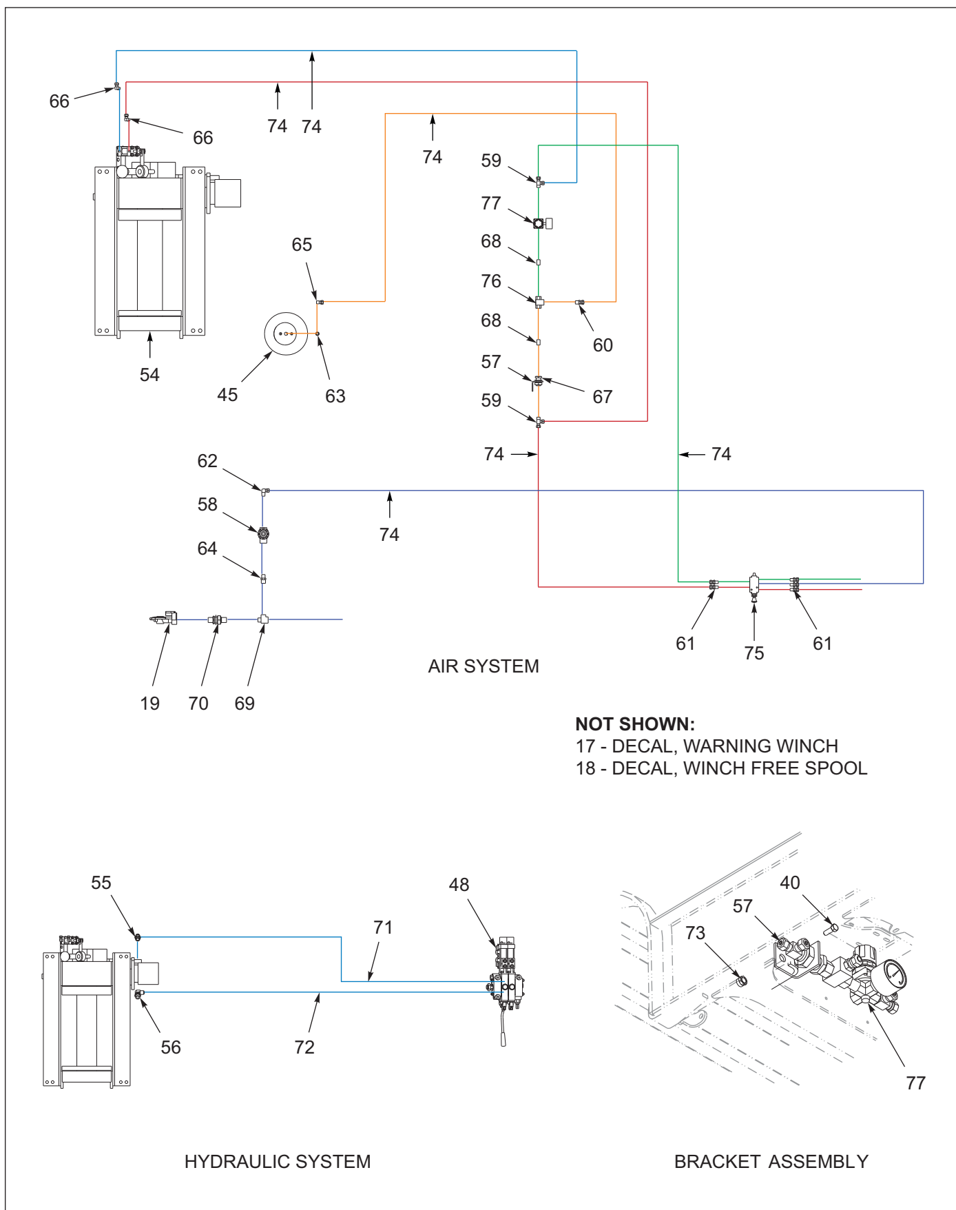
Figure 7-5: Winch Install, Braden 20K, 1-Speed, Air Tension (3 of 3)
