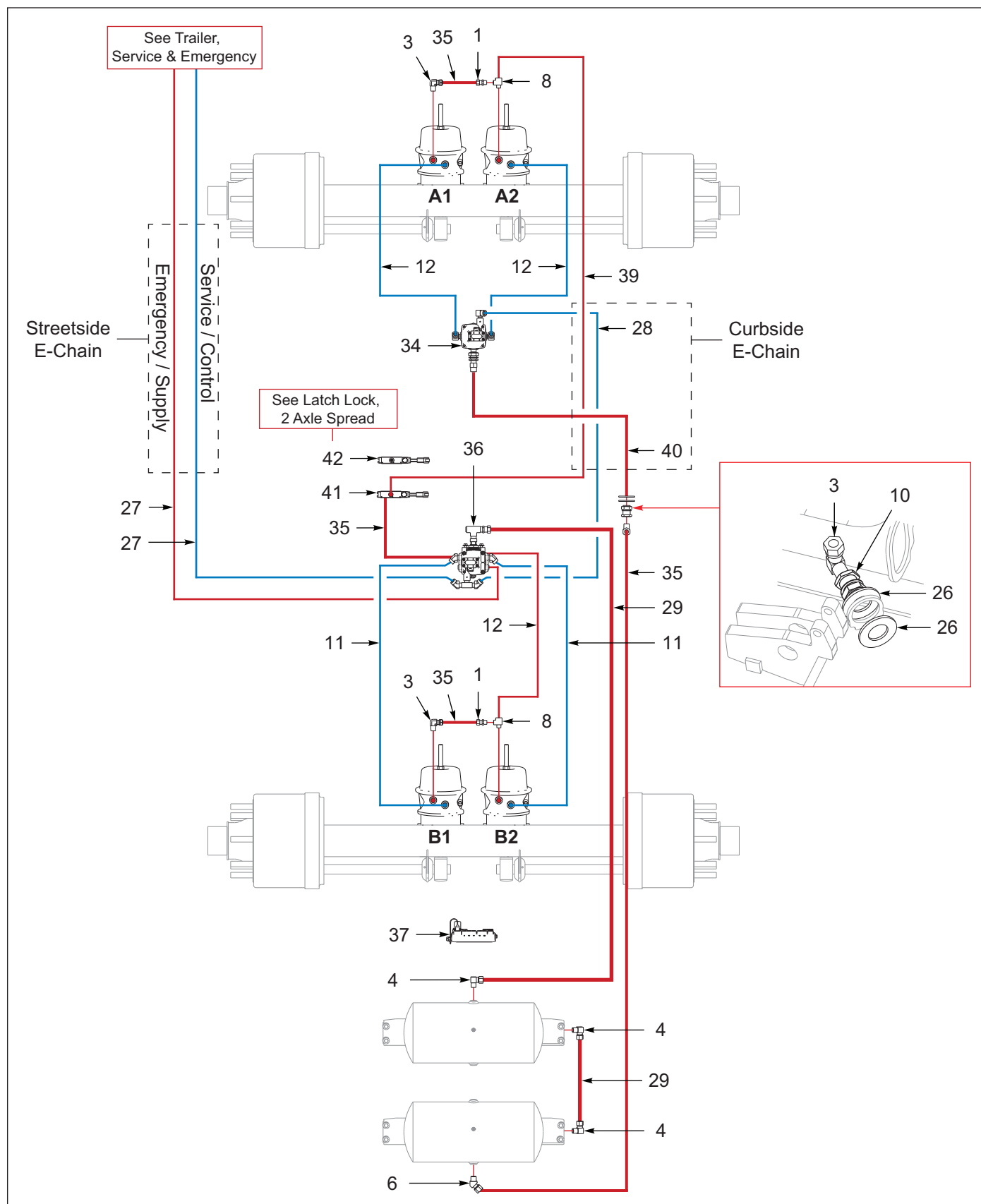
Figure 8-9: ABS, 2 Axle Spread, Haldex (Option) (1 of 2)
