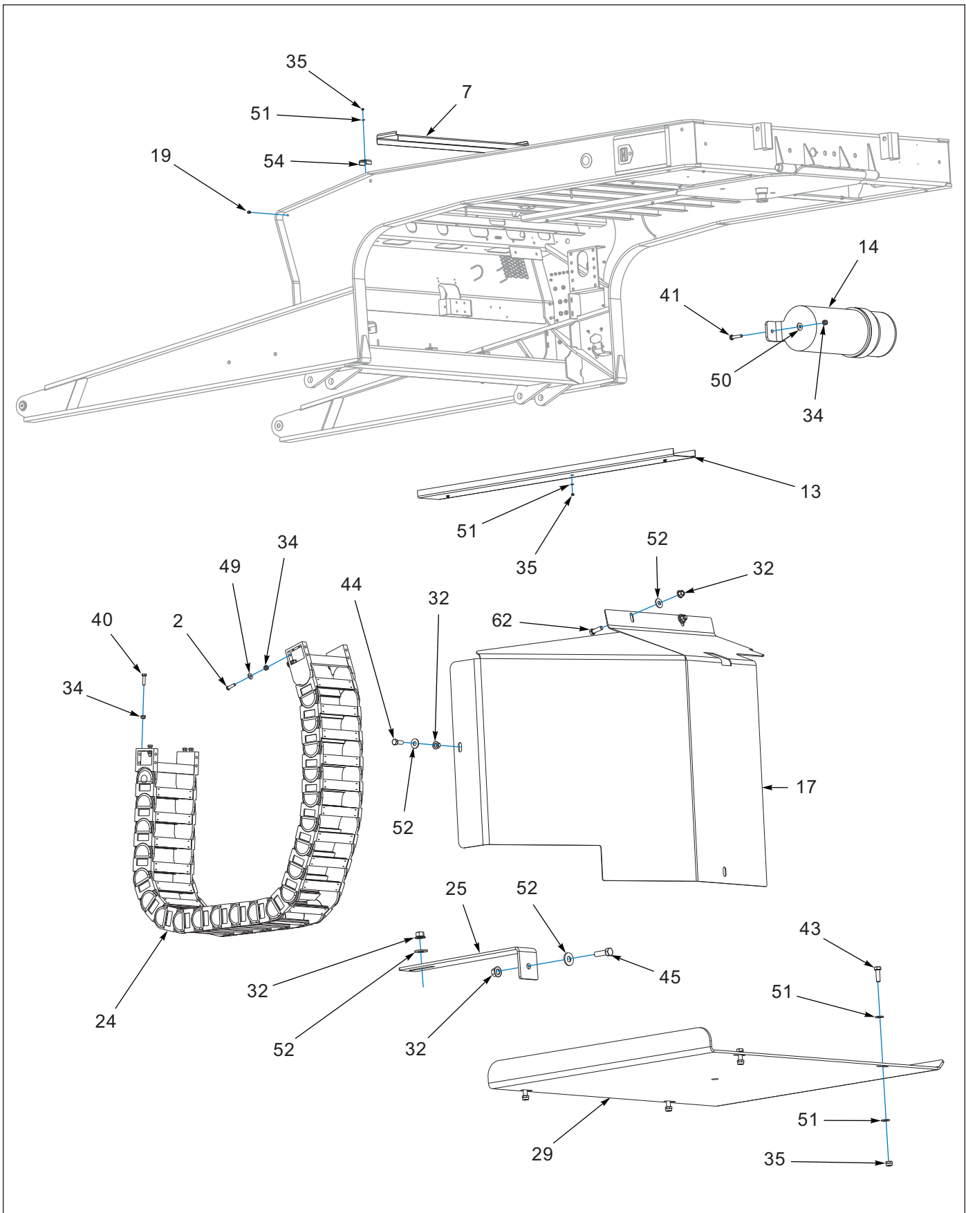
Figure 2-3: Frame Components, Upper Deck (3 of 3)
