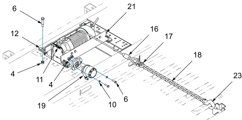
WINCH ASSEMBLY
