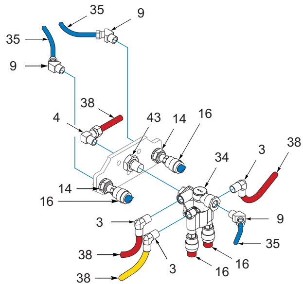
4 PORT VALVE REAR STREETSIDE VIEW
