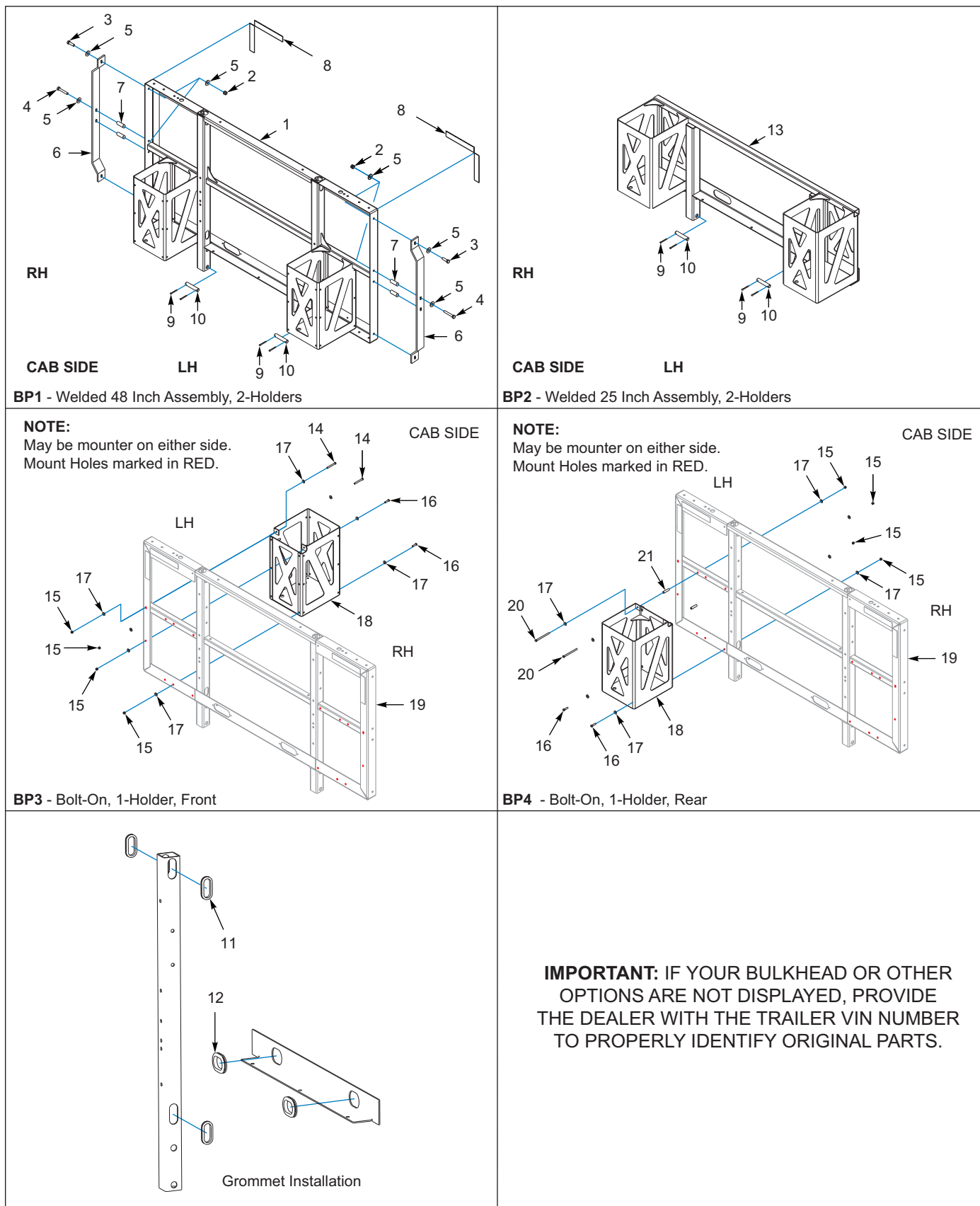
Figure 4-3: Bulkhead Components, Propane Holders
