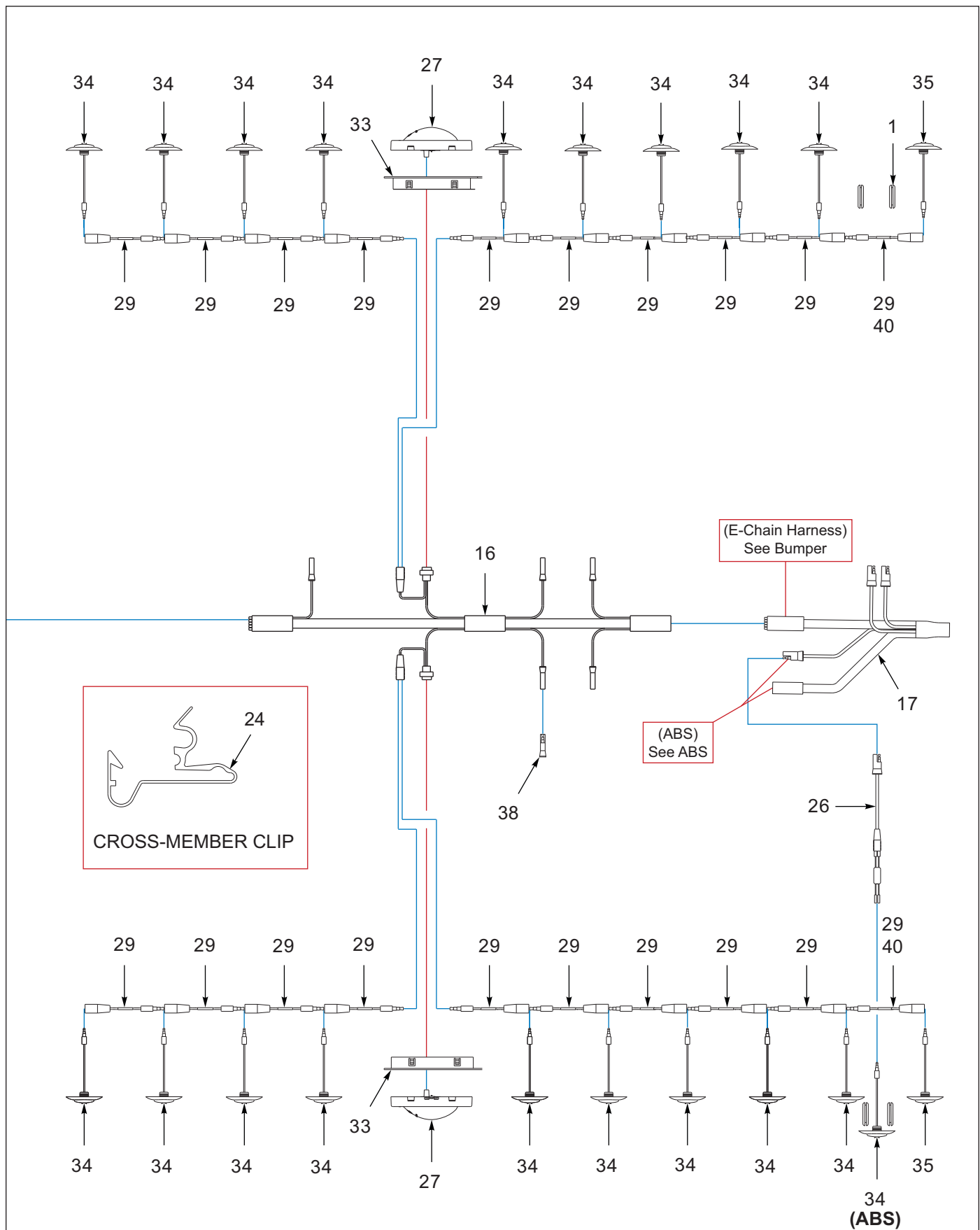
Figure 9-3: Trailer (2 of 2) (After 6/13/2023)
