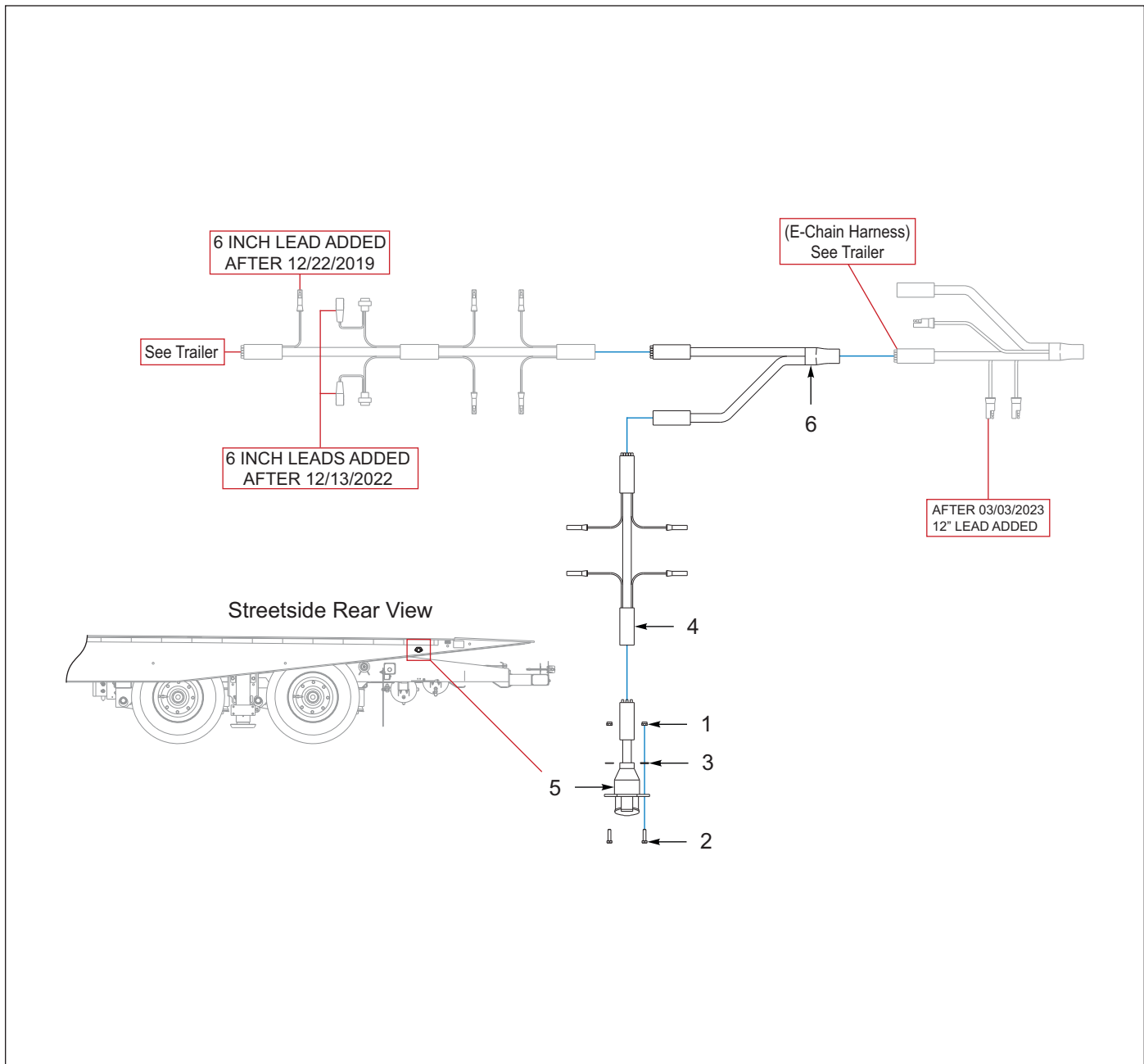
Figure 9-34: Outlet, Electrical, 7-Way, Rear (Option)
