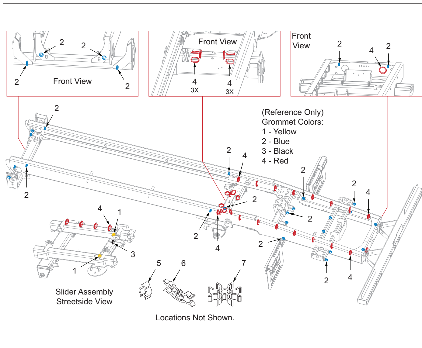
Figure 2-17: Hose Clamps, Clips, Grommets, 2 Axle Slider (Option)
