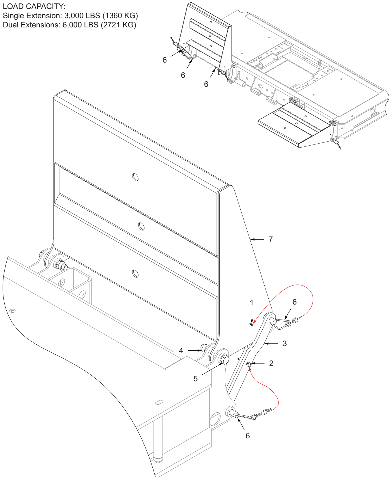
Figure 2-13: Extension, Front Flip, Upper Deck (Options)
