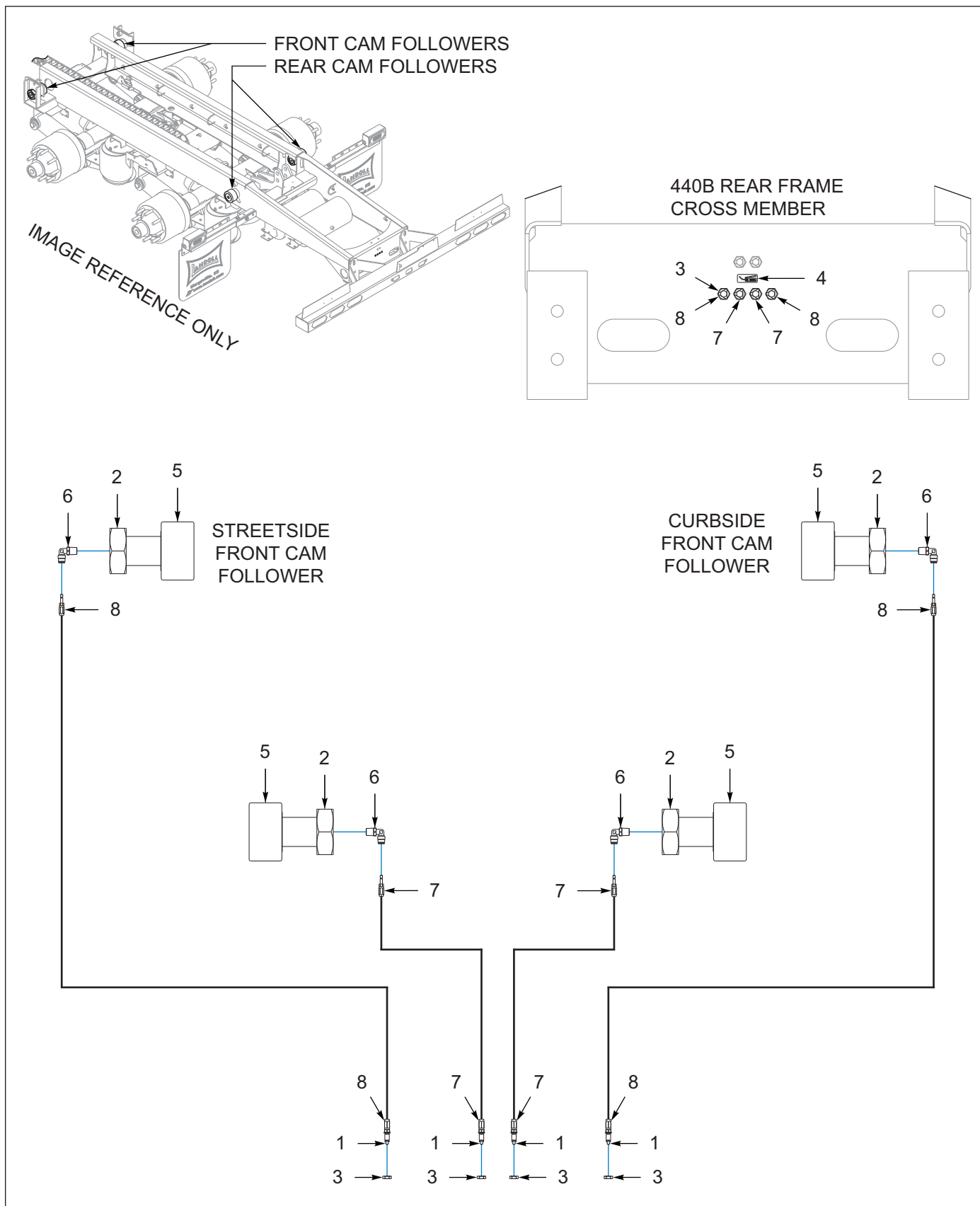
Figure 10-3: 2 Axle, Cam Followers (After 08/31/2020 To 09/01/2024)
