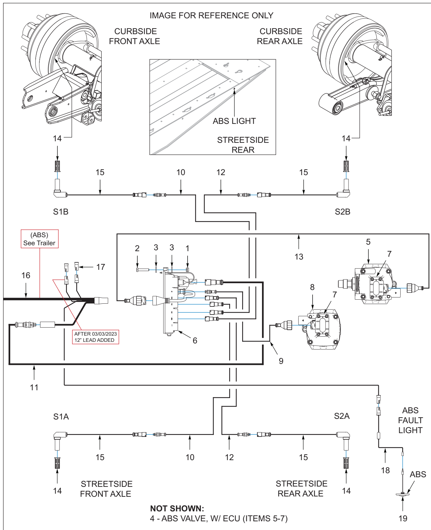
Figure 9-9: ABS, Haldex, 2 Axle (1 of 2)
