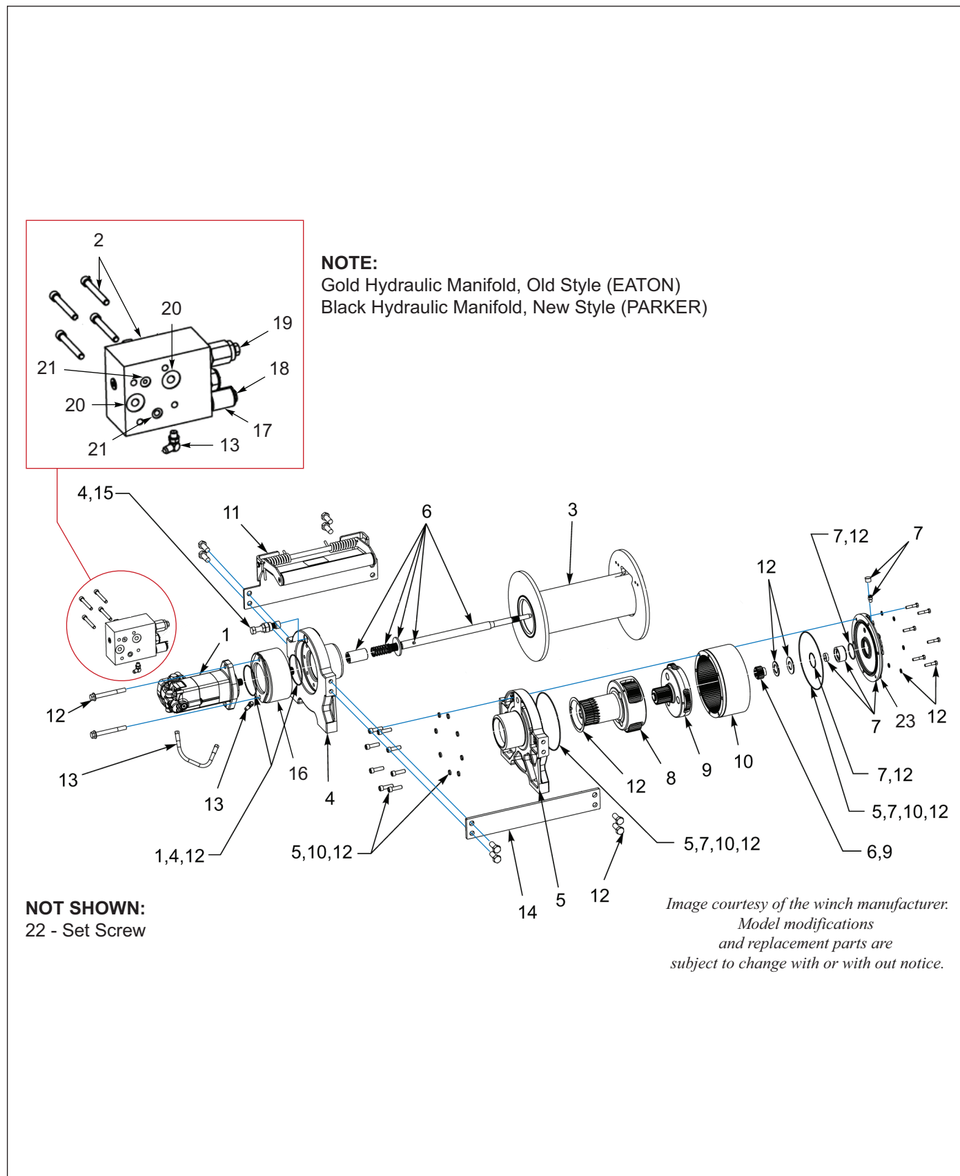
Figure 7-21: Winch Components, Warn 20K, 2-Speed
