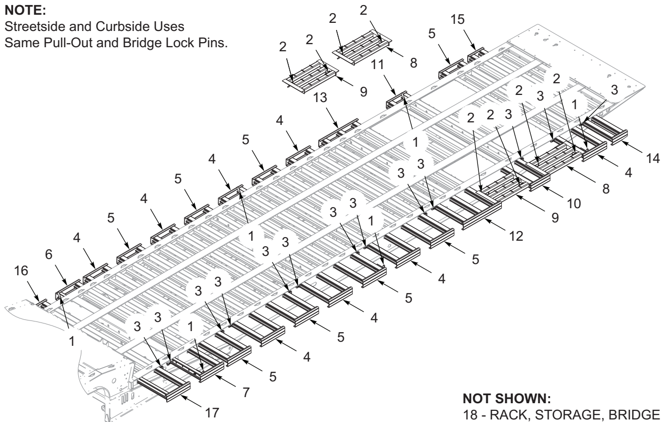
Figure 5-5: Pull-Out / Bridge, 2 Axle, 50 Foot, CA
