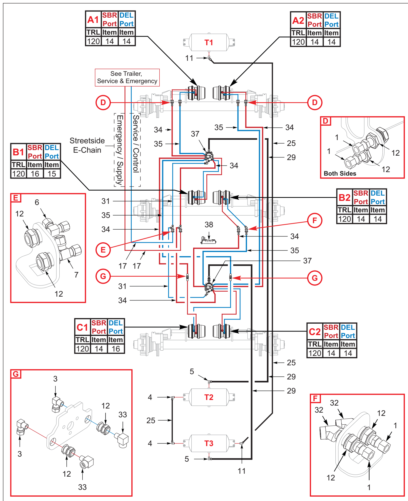
Figure 8-13: ABS, 3 Axle, Disc, Haldex, 120 (Option) (After 12/01/2025) (1 of 2)
