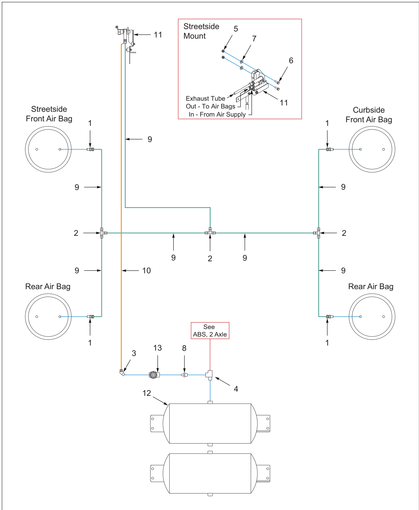
Figure 8-42: Suspension, Air Ride, 2 Ax, 3/8 in (After 09/01/2024)
