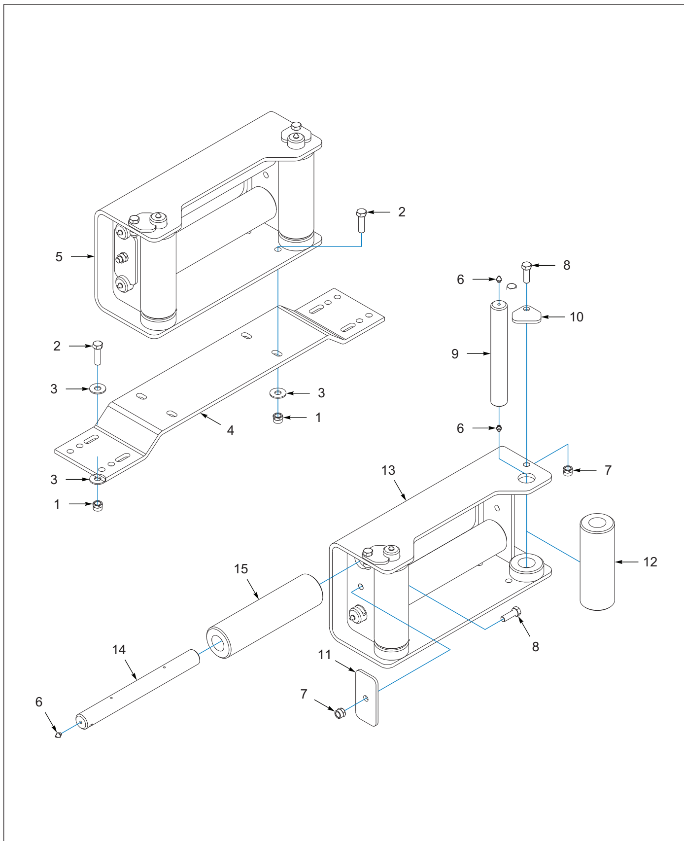
Figure 7-24: Cable Guide, 4-Roller, Warn 20K / 30K
