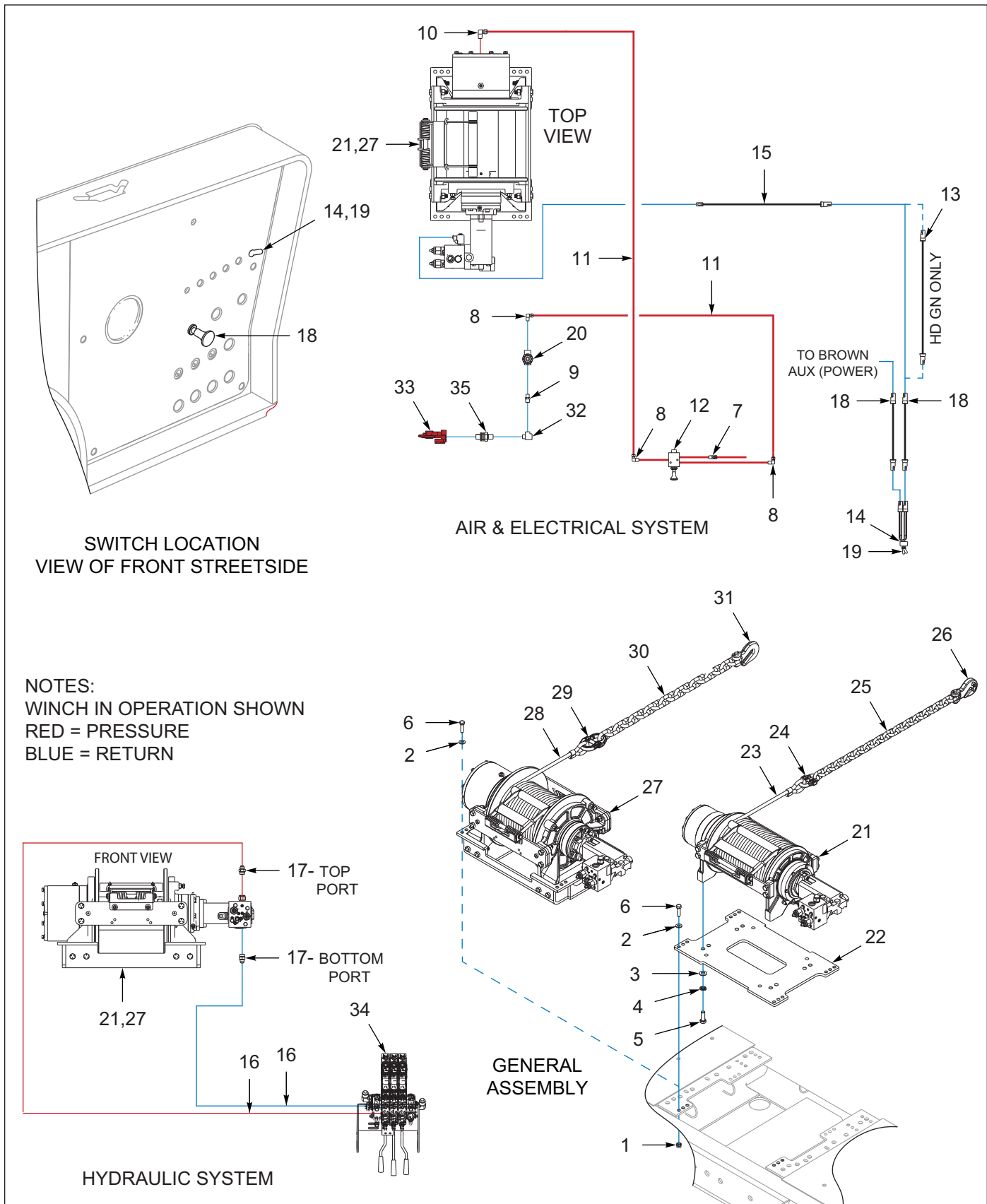
Figure 7-7: Winch Install, Ramsey 20K / 30K, 2-Speed
