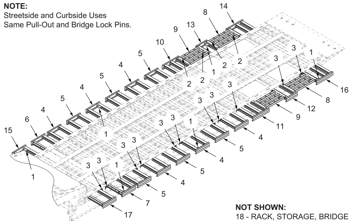
Figure 5-3: Pull-Out / Bridge, 2 Axle, 45 Foot
