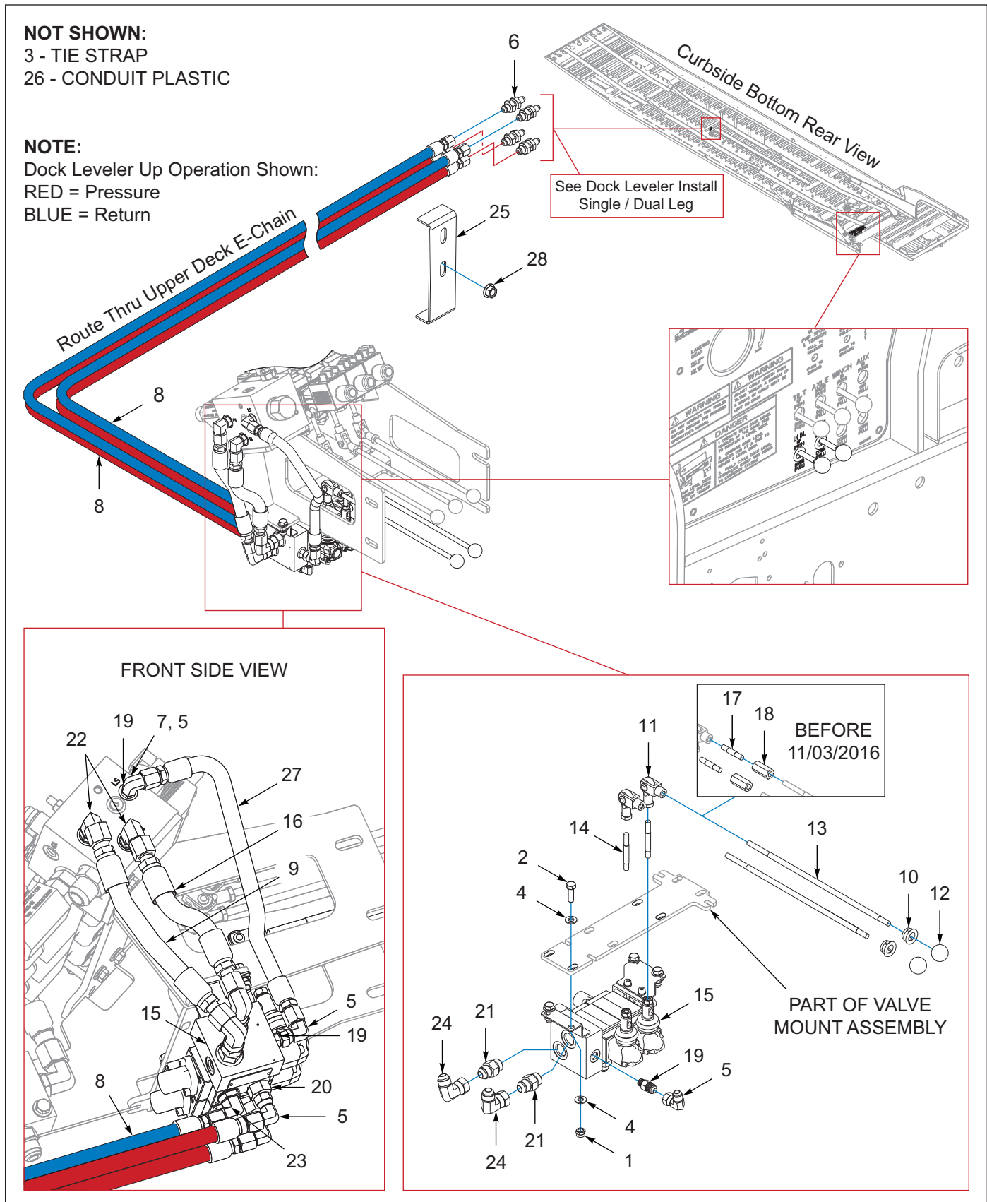
Figure 11-2: Dock Leveler Install, Control Valve & Hoses (Option)
