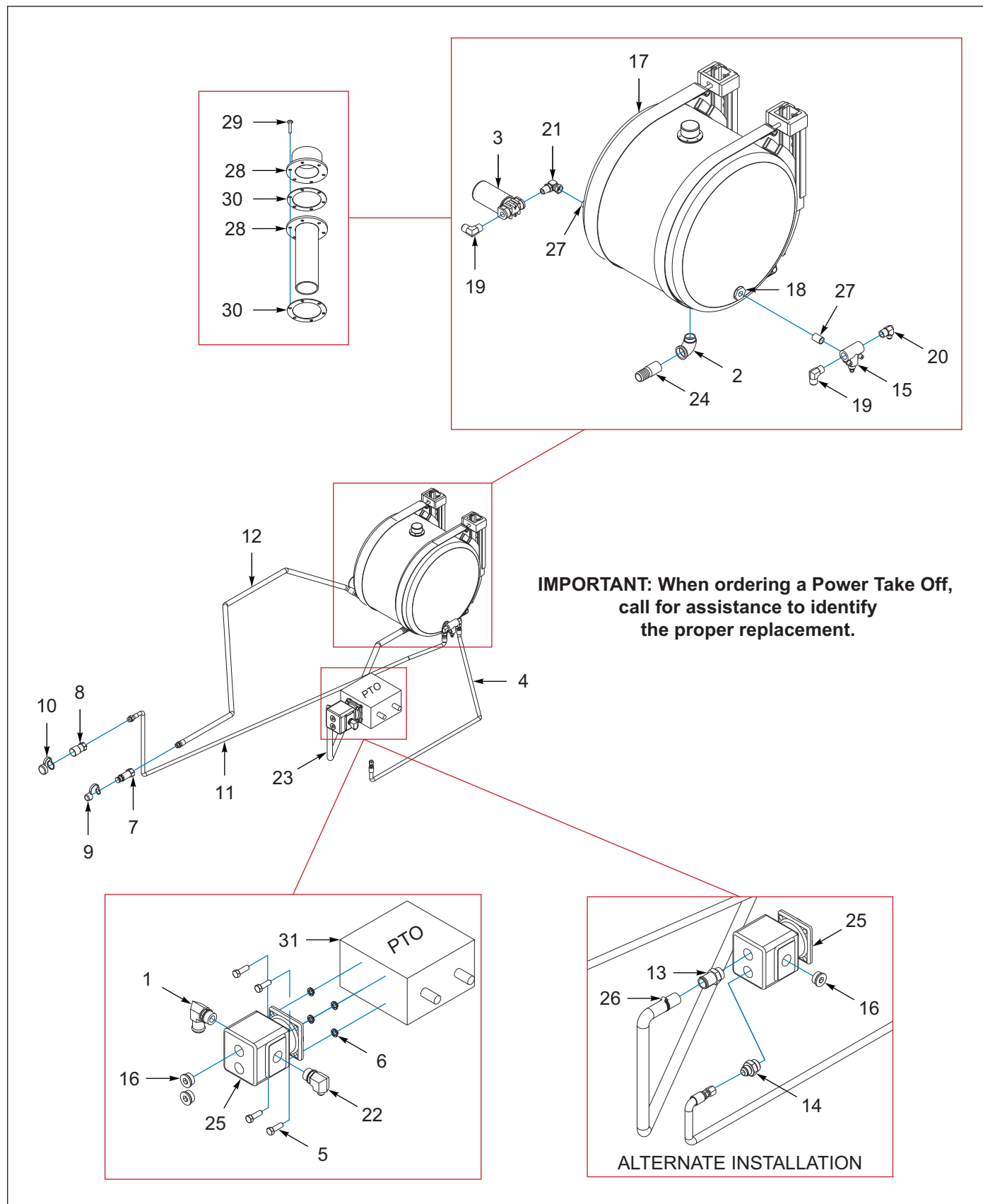
Figure 6-10: Wet Kit, Truck Hydraulic (After 03/01/2019)
