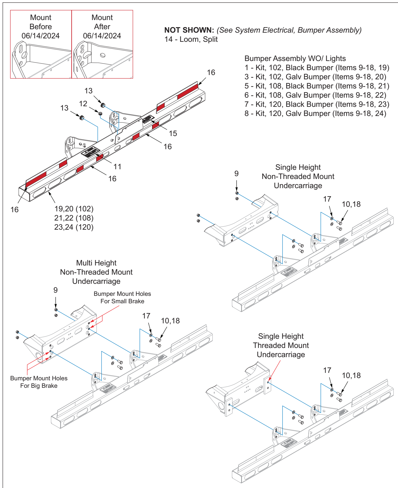
Figure 2-5: Bumper, Rear (1 of 2)
