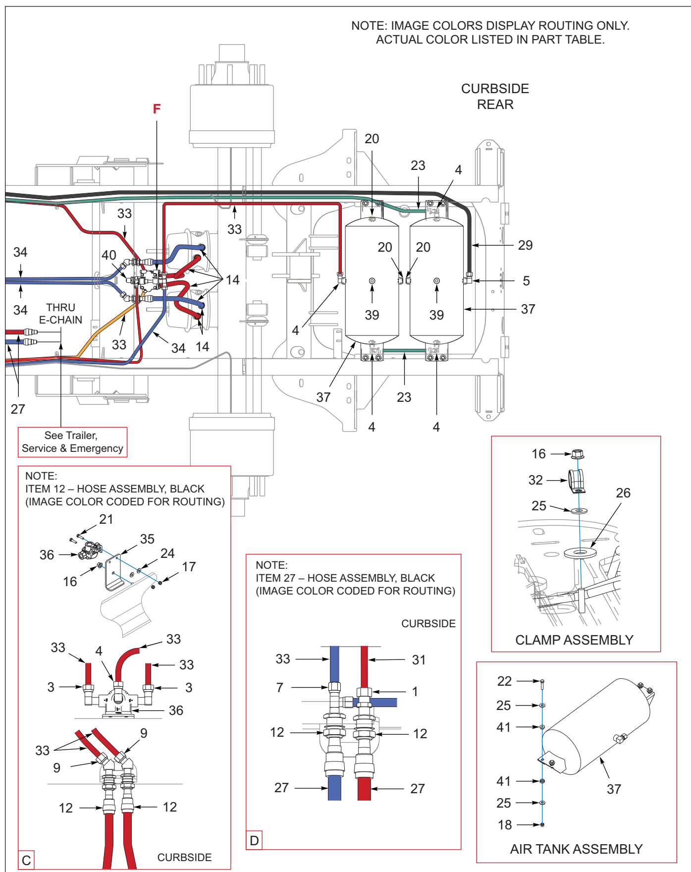
Figure 8-23: ABS, 3 Axle, Drum, Wabco (10/06/2023 To 12/01/2025) (2 of 3)
