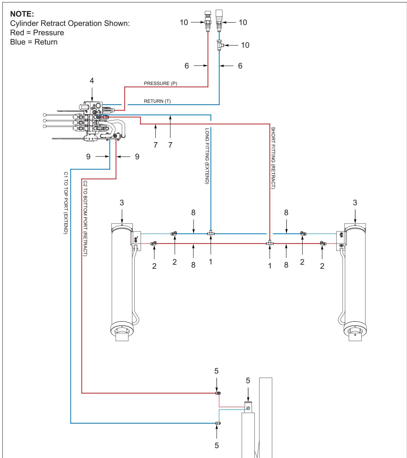
Figure 11-1: Trailer, Hitch Tilt / Travel Axle
