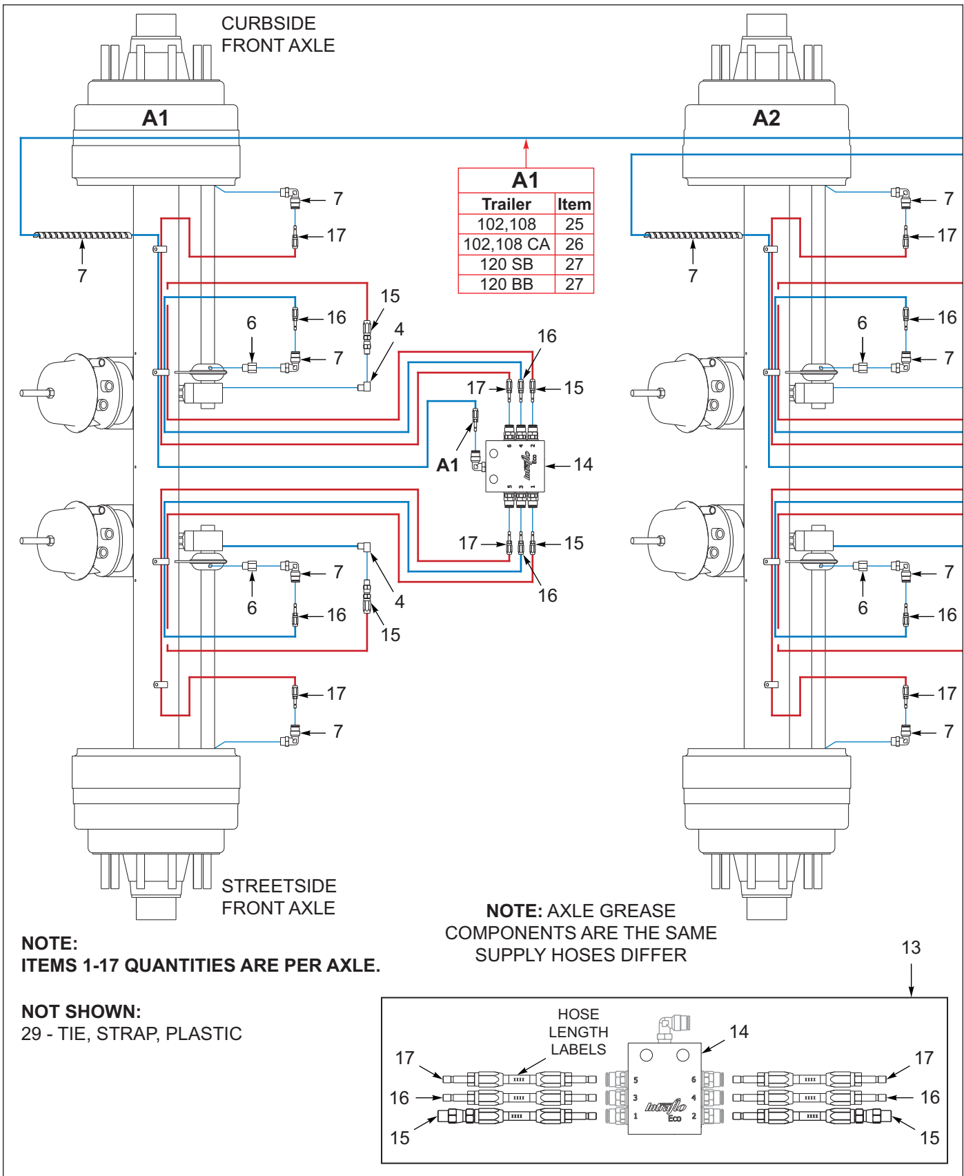
Figure 10-23: 3 Axle, Drum Brakes (After 12/01/2025) (1 of 3)
