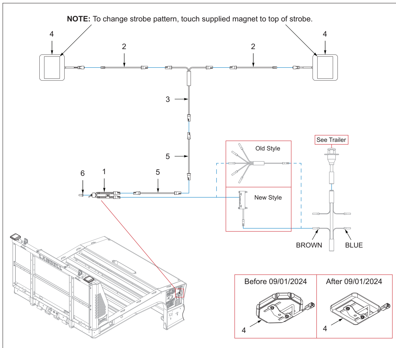
Figure 9-22: Lights, Strobe, Bulkhead, 360 Degree Amber (Option)
