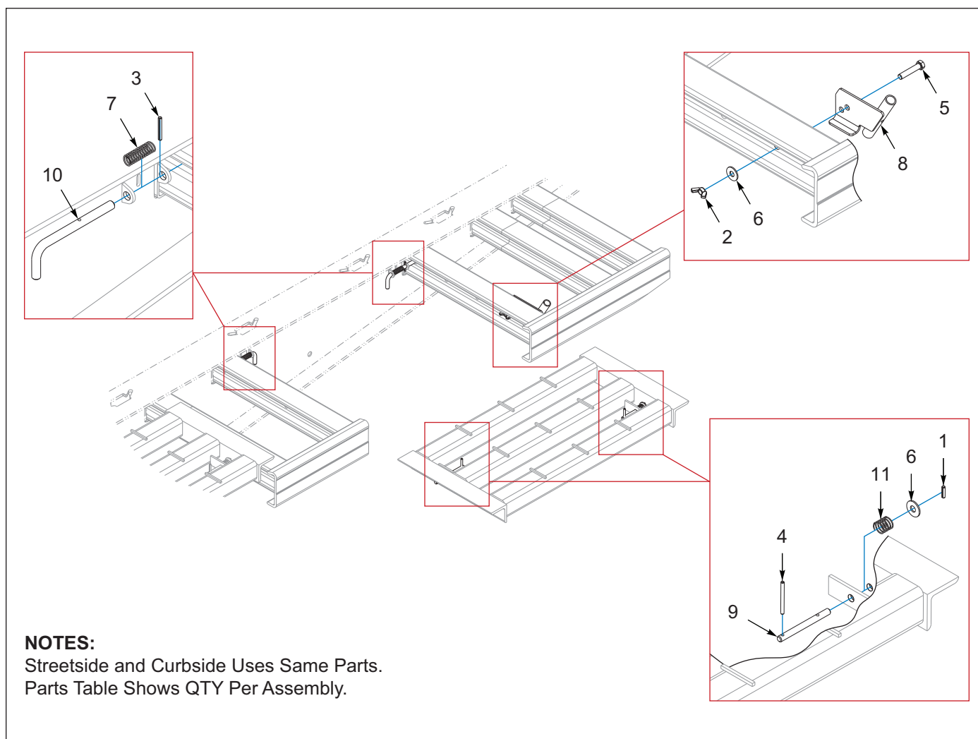
Figure 5-1: Lock Pins & Flag Holder, Pull-Out / Bridge
