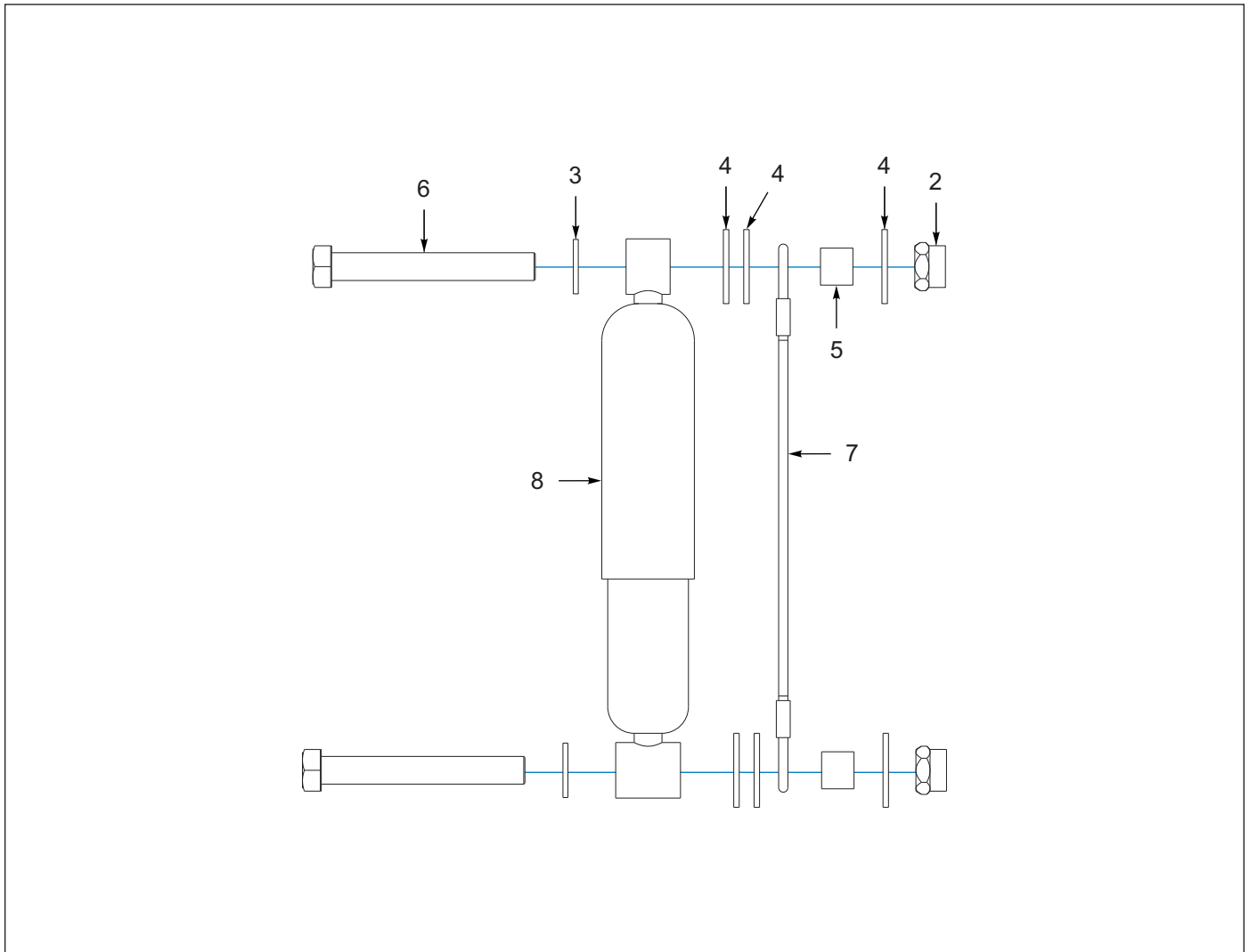
Figure 3-18: Shock Strap, Limit, LSS-25K-5.5 (Option)
