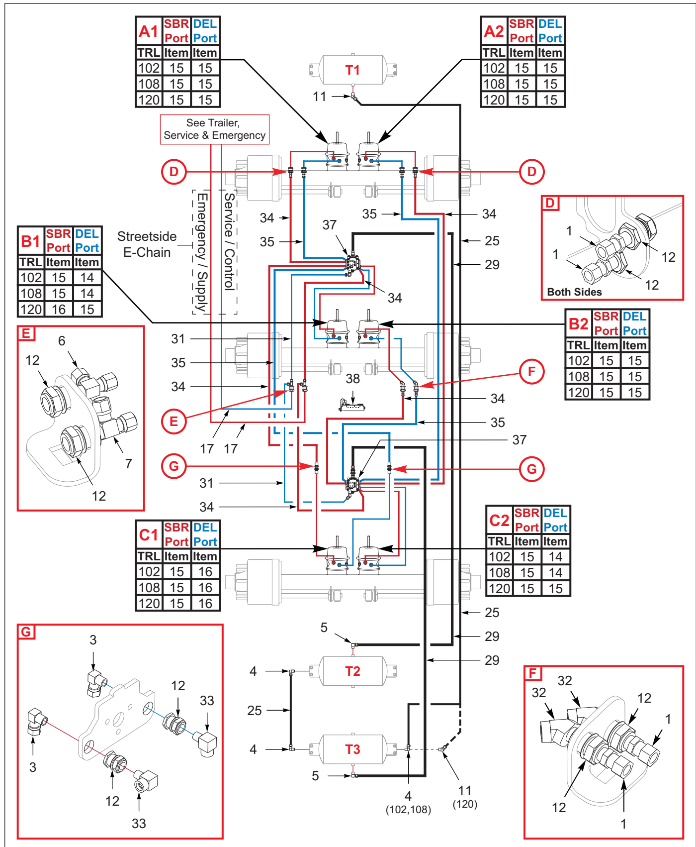
Figure 8-25: ABS, 3 Axle, Drum, Haldex (After 12/01/2025) (1 of 2)
