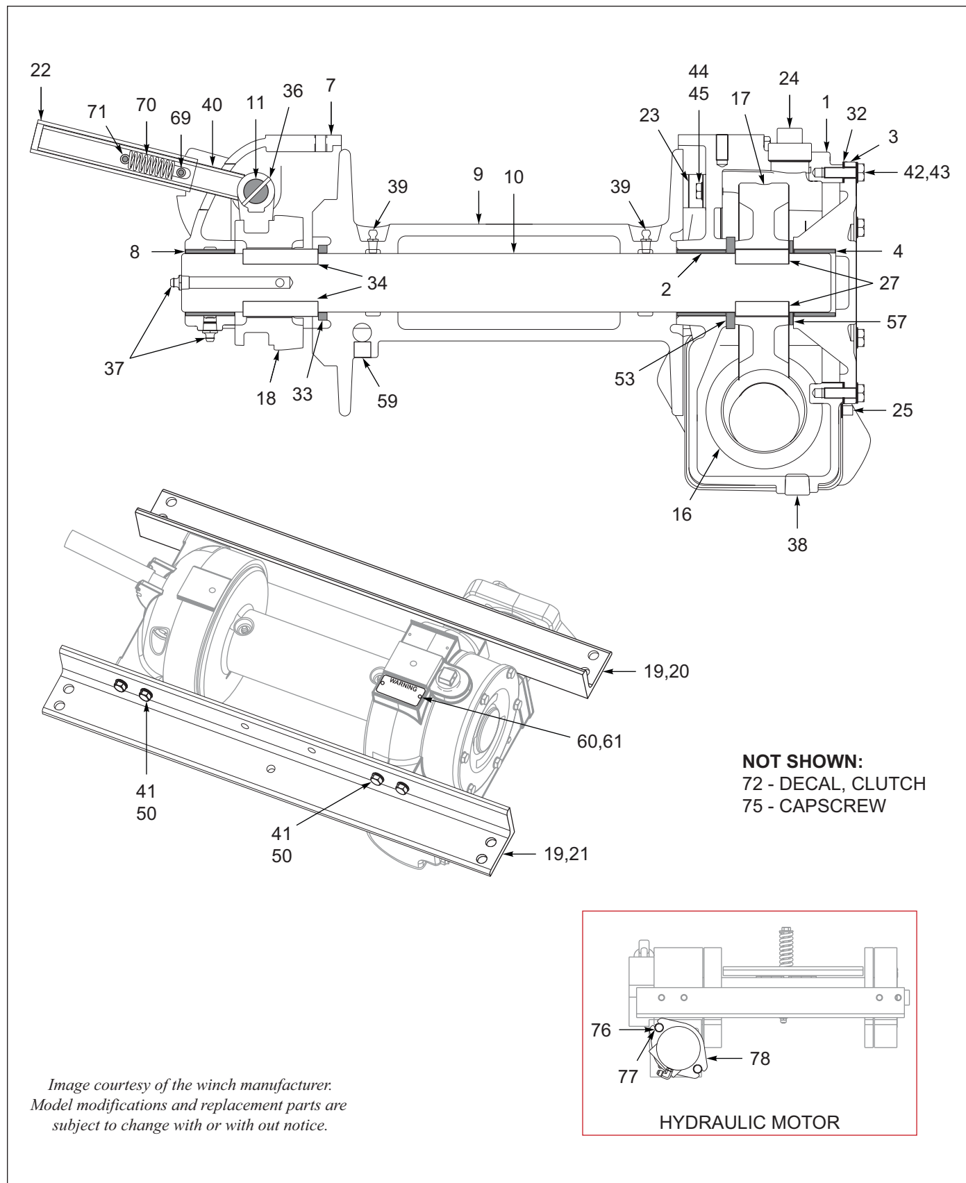
Figure 7-11: Winch Components, Braden 12K, 1-Speed (1 of 2)
