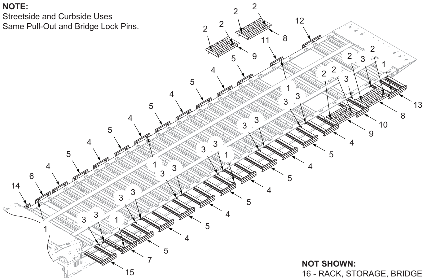
Figure 5-6: Pull-Out / Bridge, 2 Axle, 53 Foot
