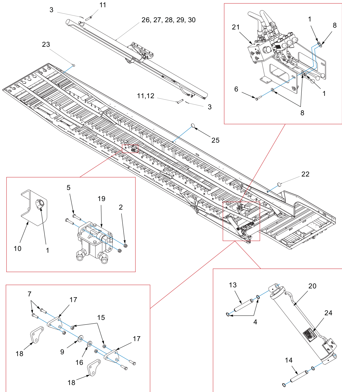
Figure 2-4: Frame Components, Hydraulic & Air
