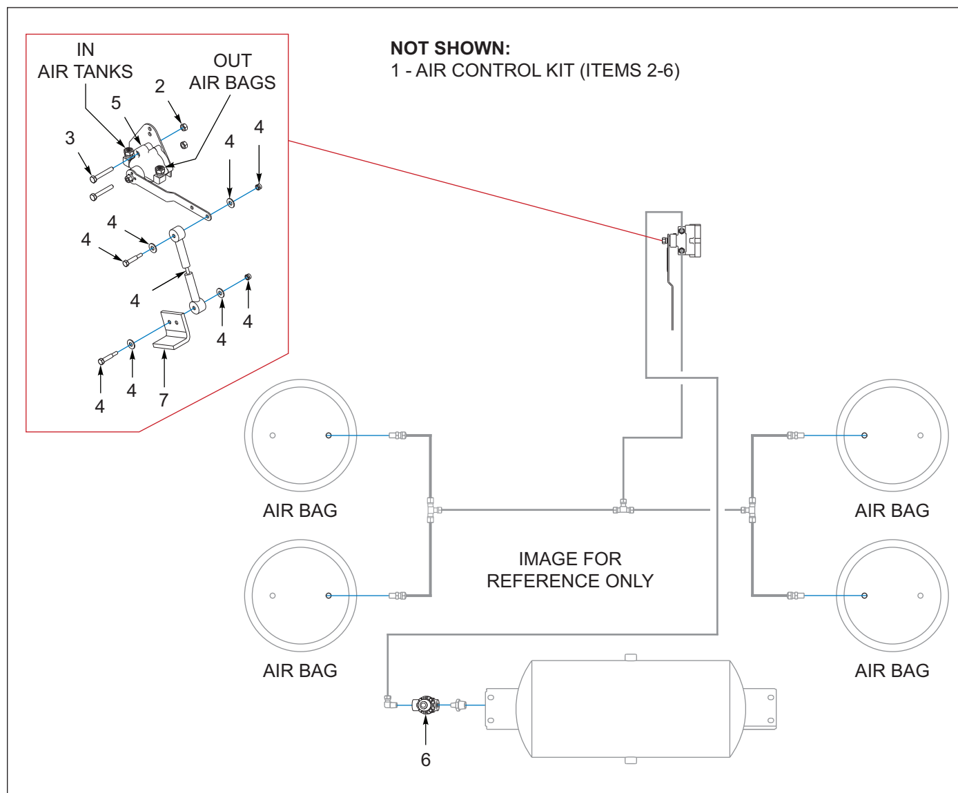
Figure 8-53: Suspension, Air Ride Control Kit, 1/4 in, Aqua (Option)
