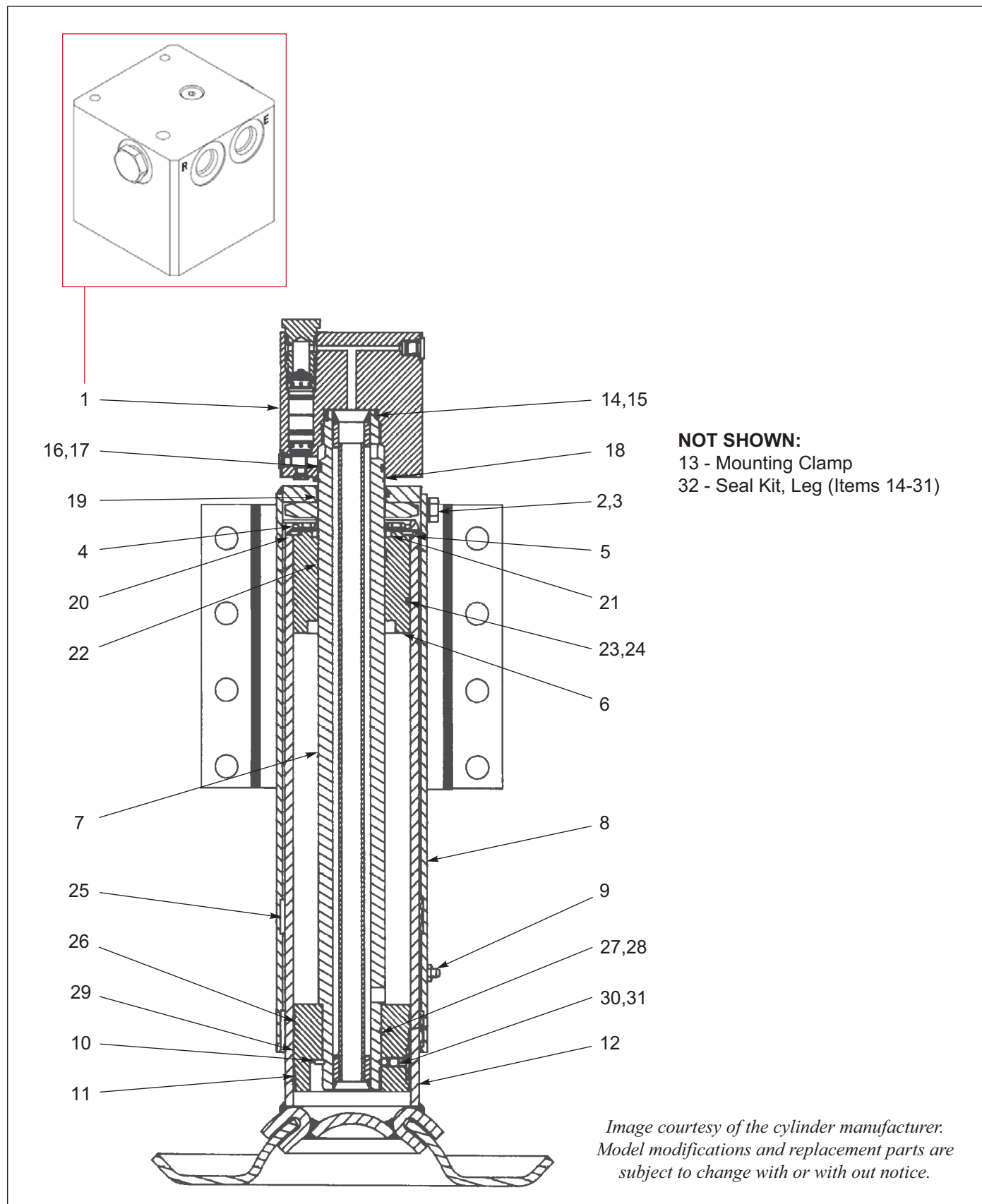
Figure 11-13: Cylinder Components, 4 x 15 (Option)
