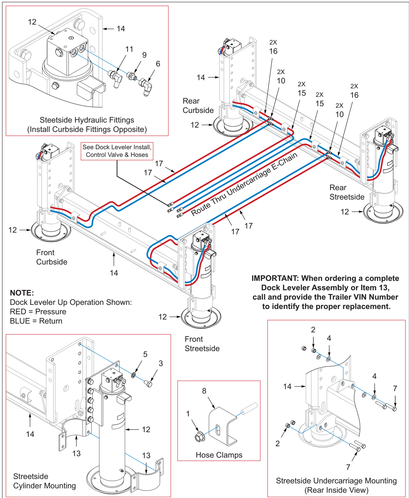
Figure 11-4: Dock Leveler Install, Dual Leg Assembly, 124K (Option)
