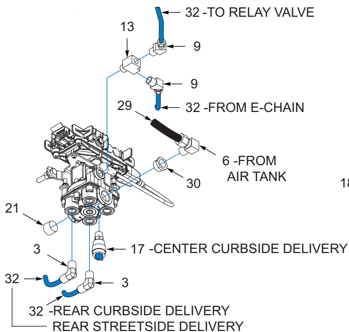
ECU VALVE FRONT CURBSIDE VIEW
