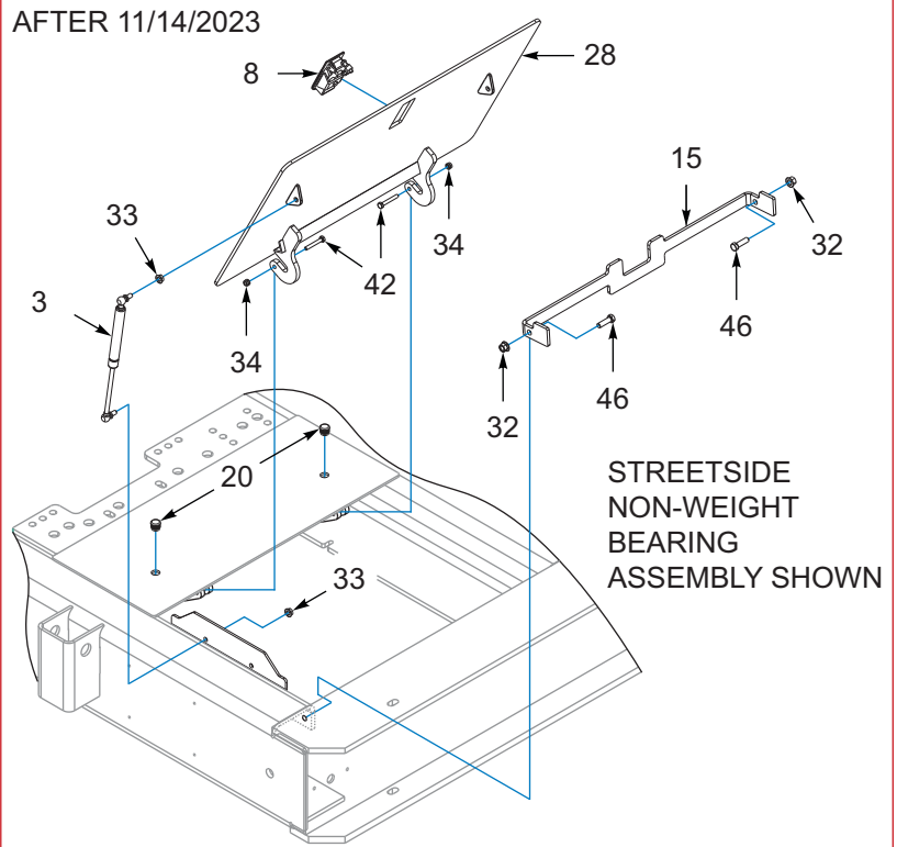
Figure 2-2: Frame Components, Upper Deck (2 of 3)
