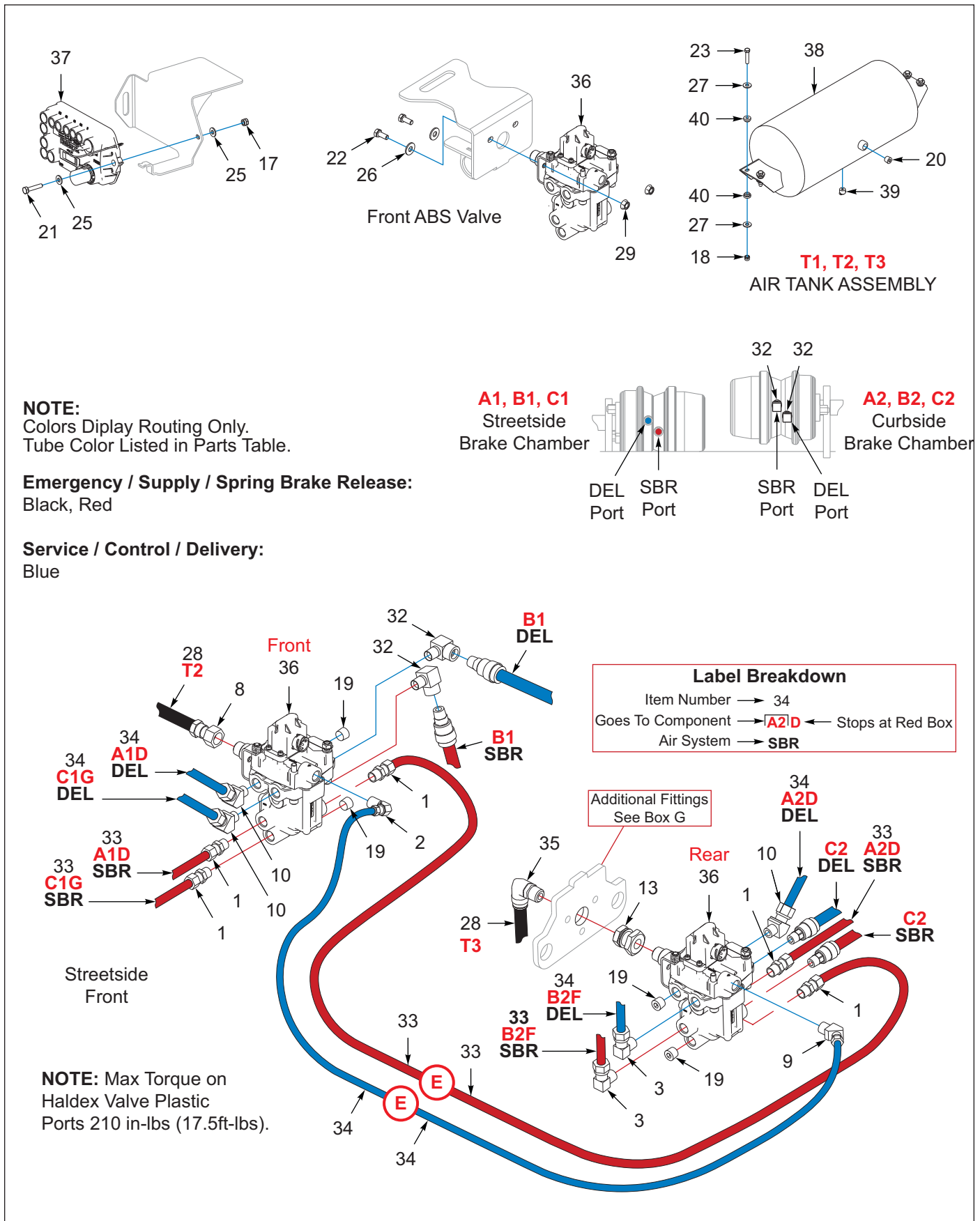
Figure 8-12: ABS, 3 Axle, Disc, Haldex, 102 / 108 (Option) (After 12/01/2025) (2 of 2)
