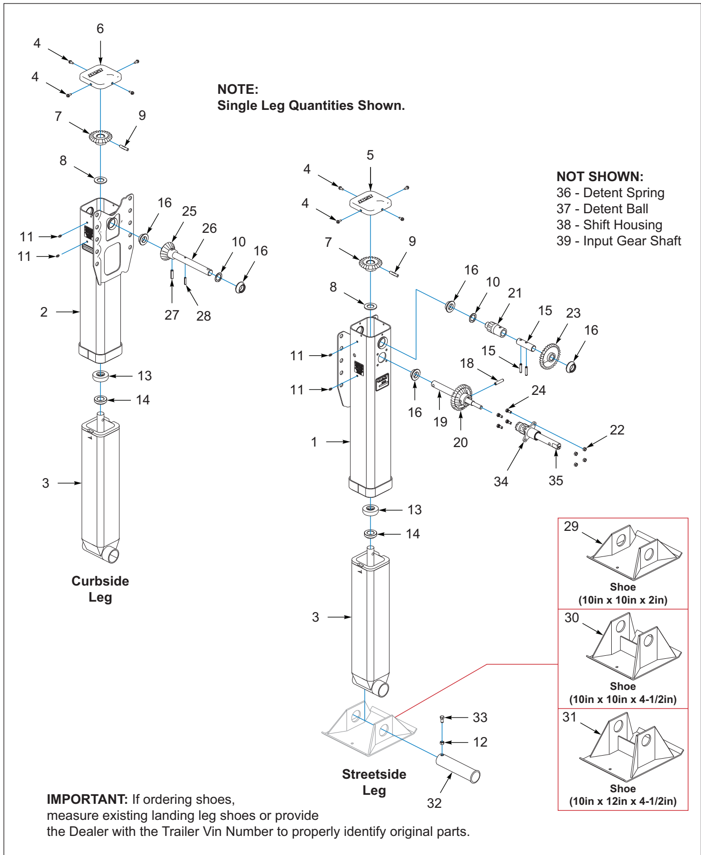
Figure 2-24: Landing Leg Components, Gear, 2-Speed
