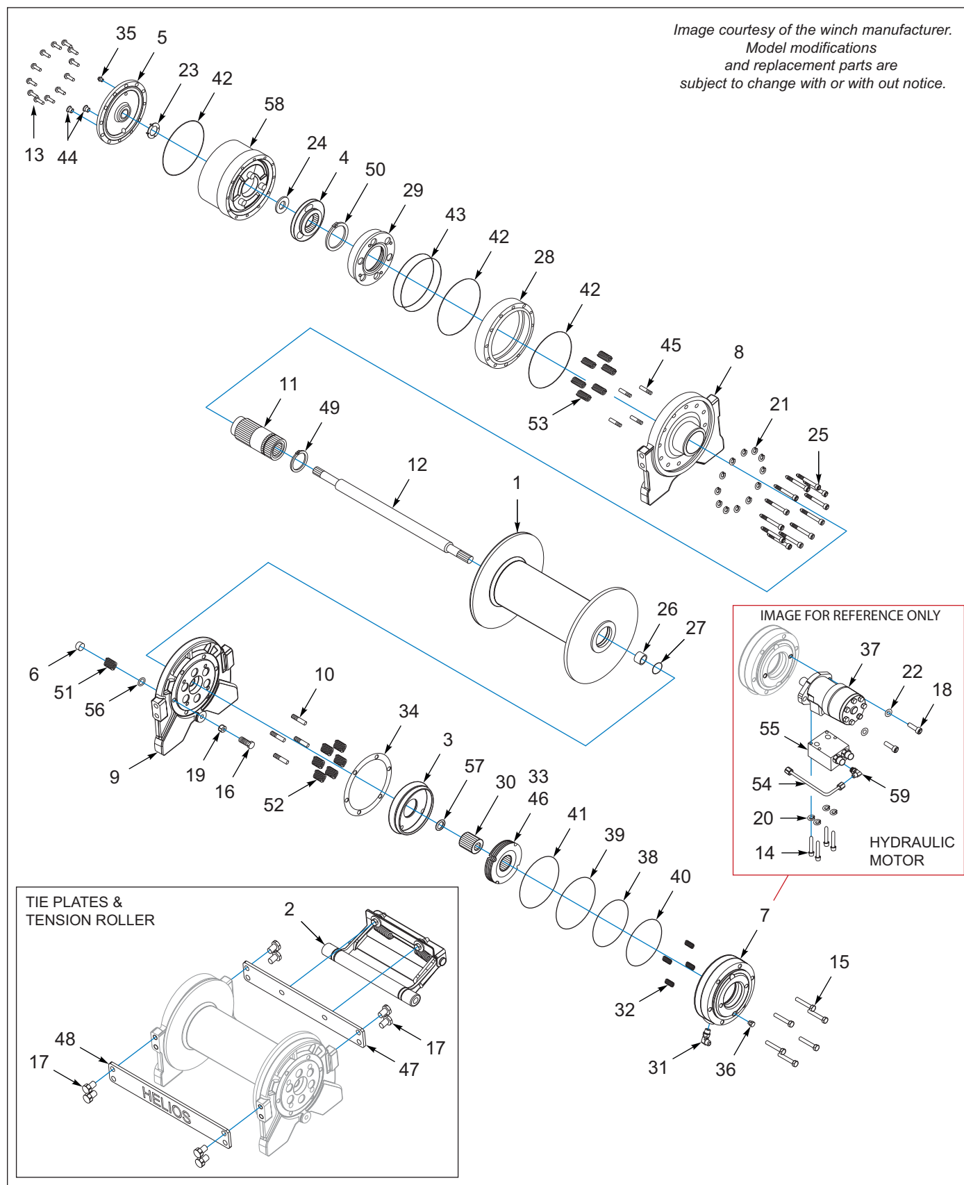
Figure 7-19: Winch Components, Ramsey 20K, 2-Speed
