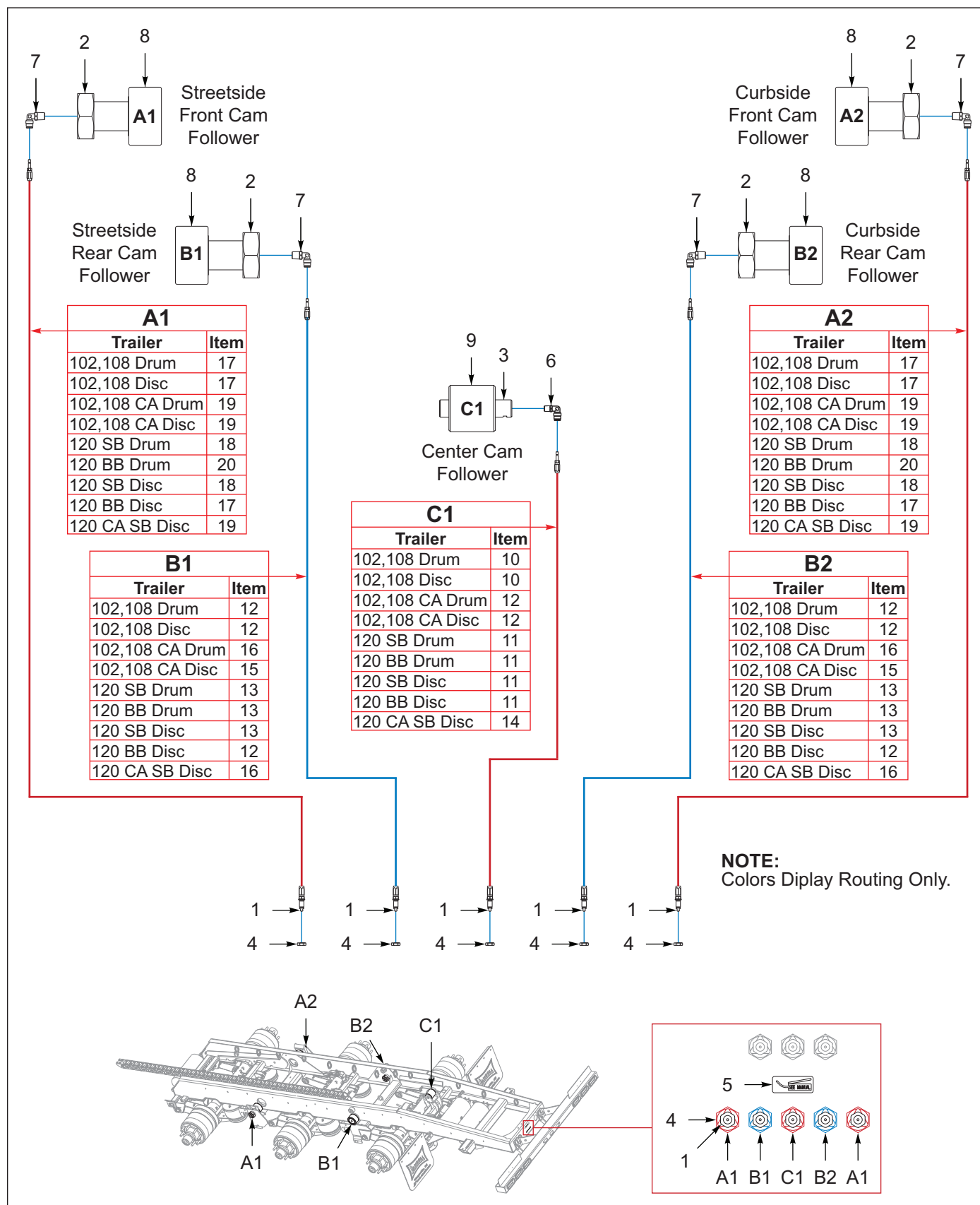
Figure 10-22: 3 Axle, Cam Followers, Roller (After 12/01/2025)
