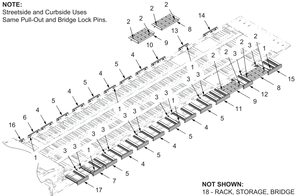
Figure 5-4: Pull-Out / Bridge, 2 Axle, 48 Foot
