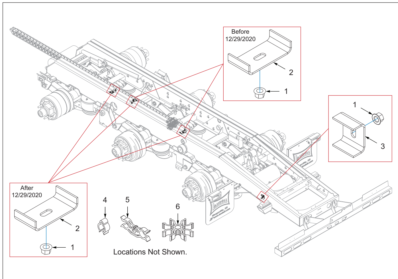
Figure 2-18: Hose Clamps, Clips, No Grommets, 3 Axle (Before 03/10/2023)
