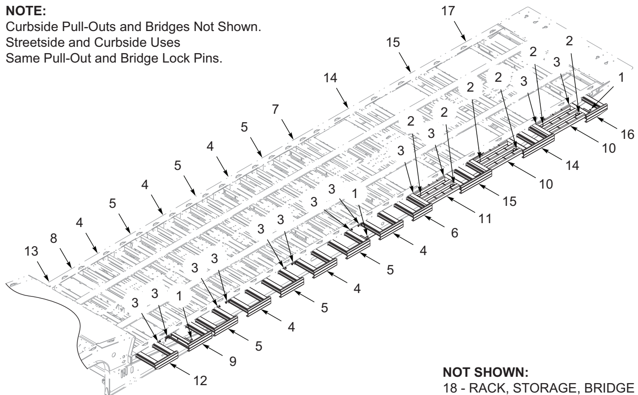
Figure 5-8: Pull-Out / Bridge, 3 Axle, 50 Foot
