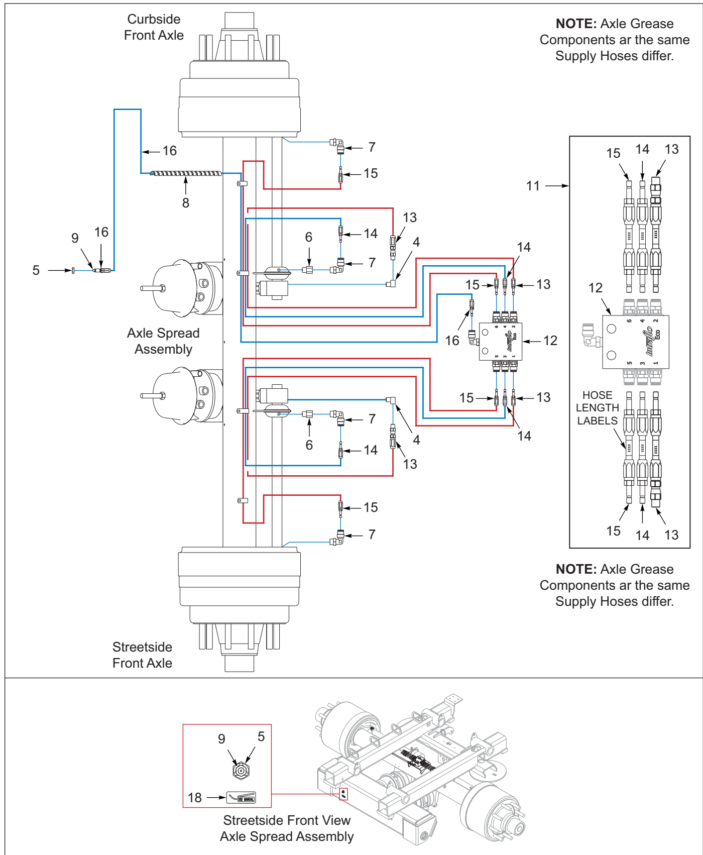
Figure 10-12: 2 Axle Spread, Drum Brakes (Option) (1 of 3)
