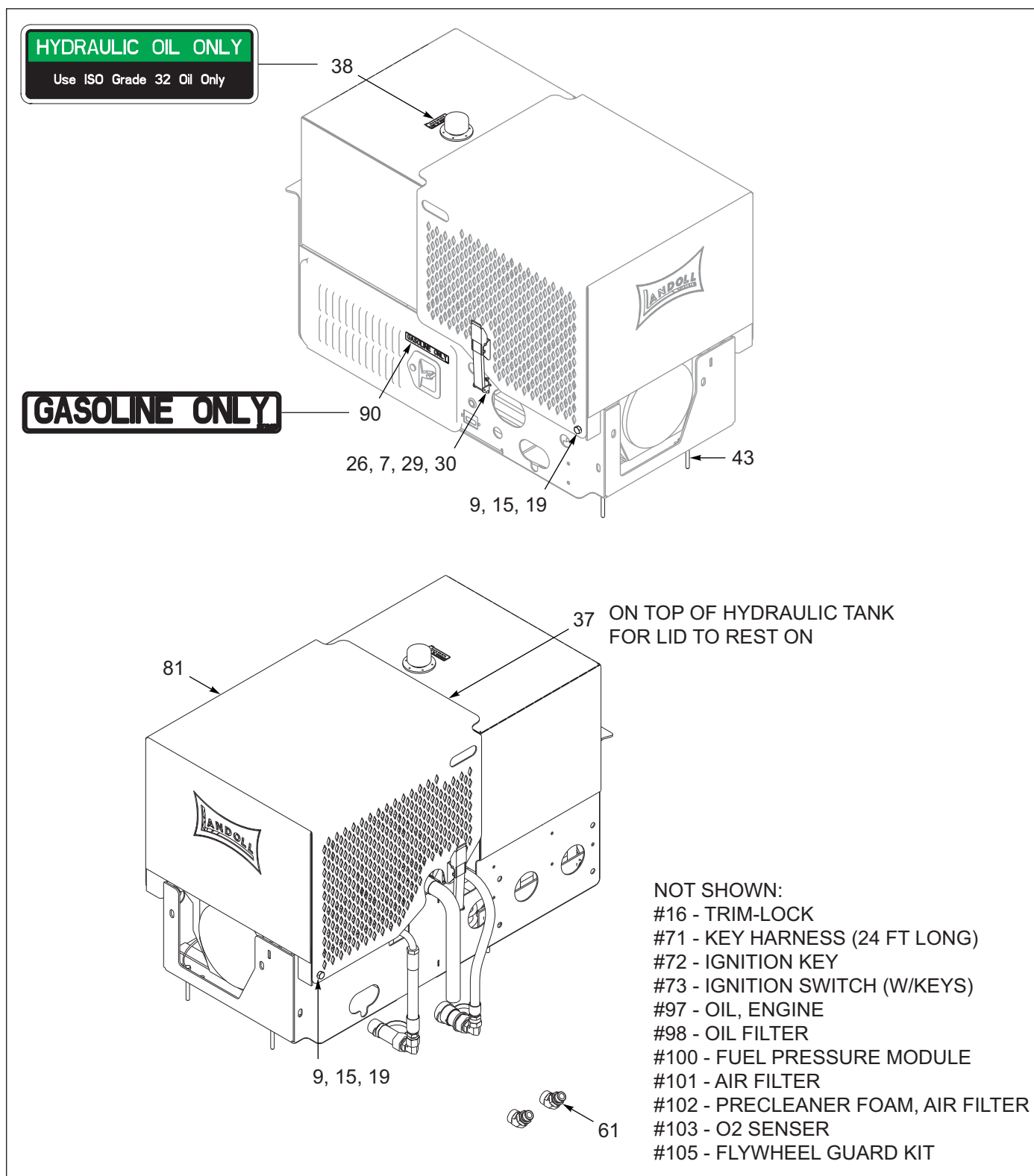
Figure 6-1: Engine, 25HP, Upper Deck Assembly (1 of 5)
