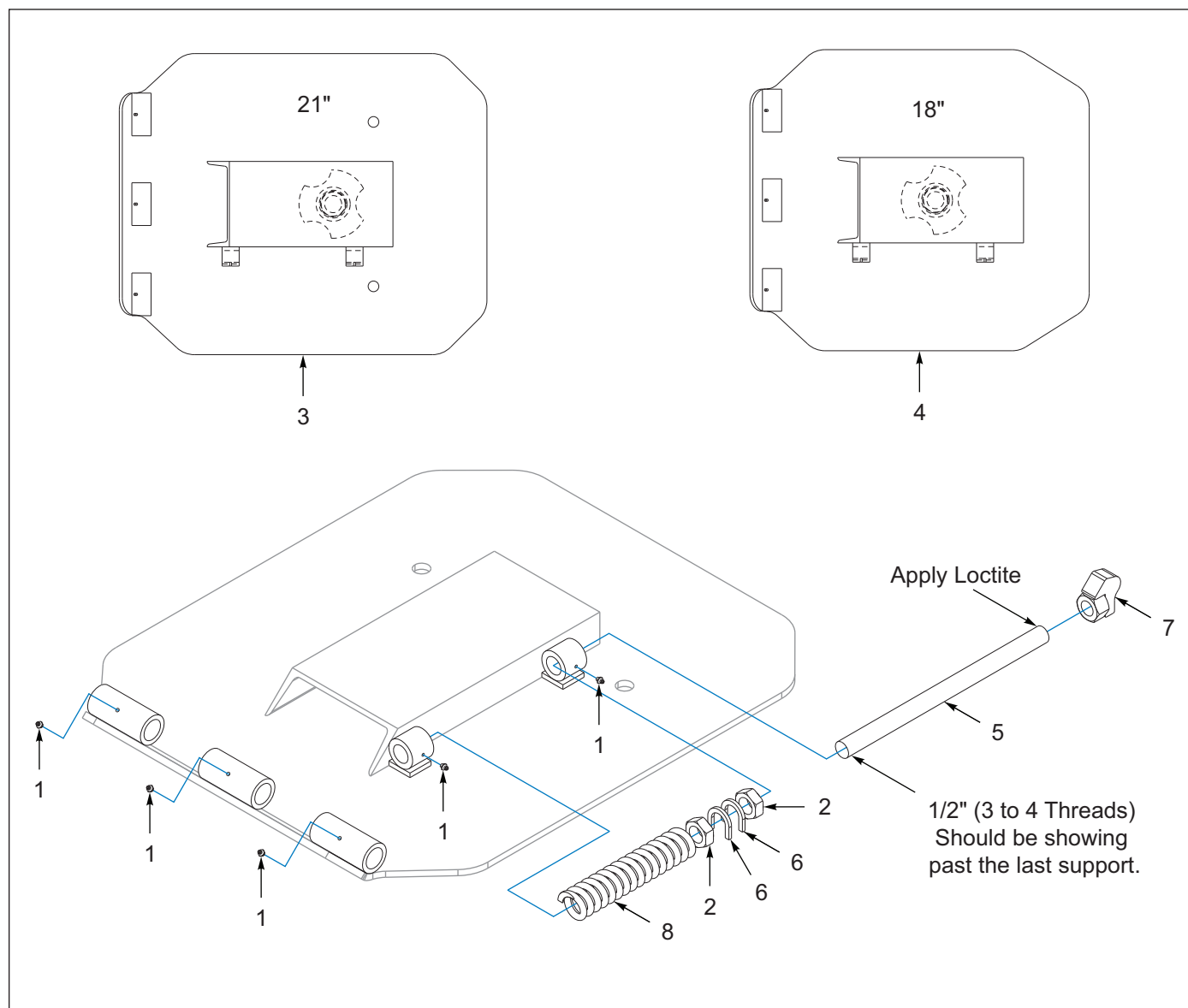
Figure 2-14: Hitch Plate Assembly
