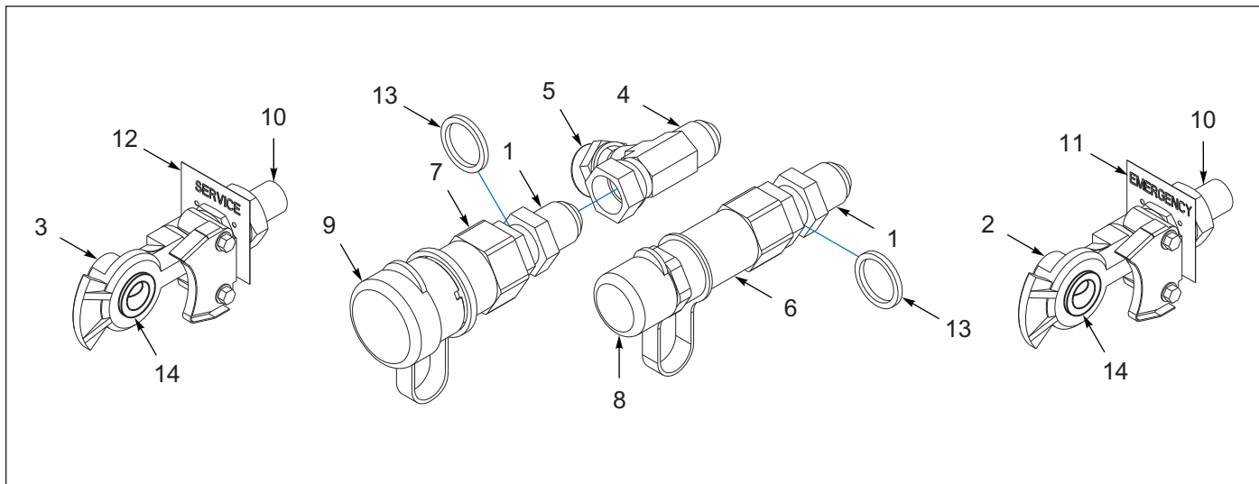
Figure 11-8: Coupler, Front Sub-Assembly, Hydraulic & Air
