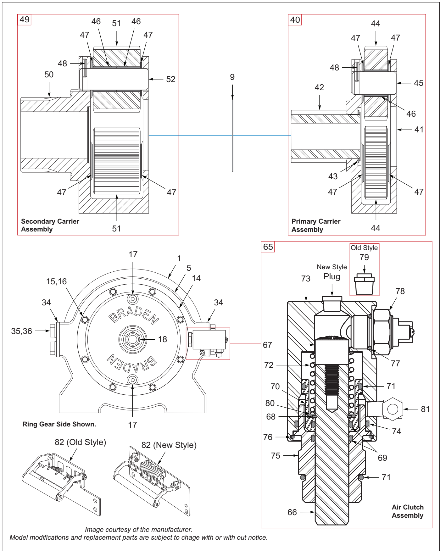
Figure 7-16: Winch Components, Braden 20K, 2-Speed (2 of 2)
