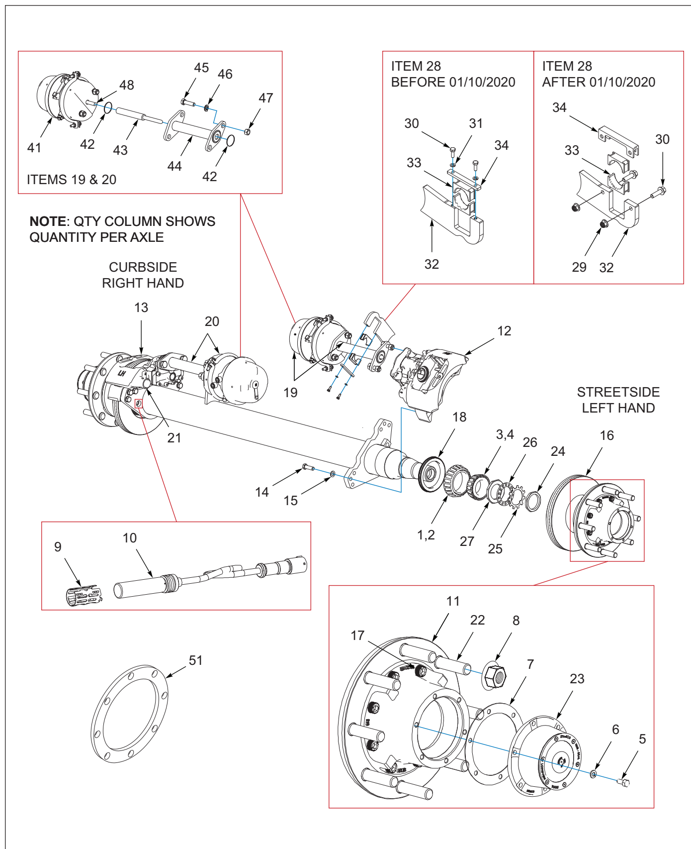
Figure 3-3: Axle 12.25 Disc Brake &amp; Hub Components (Option) (1 of 2)
