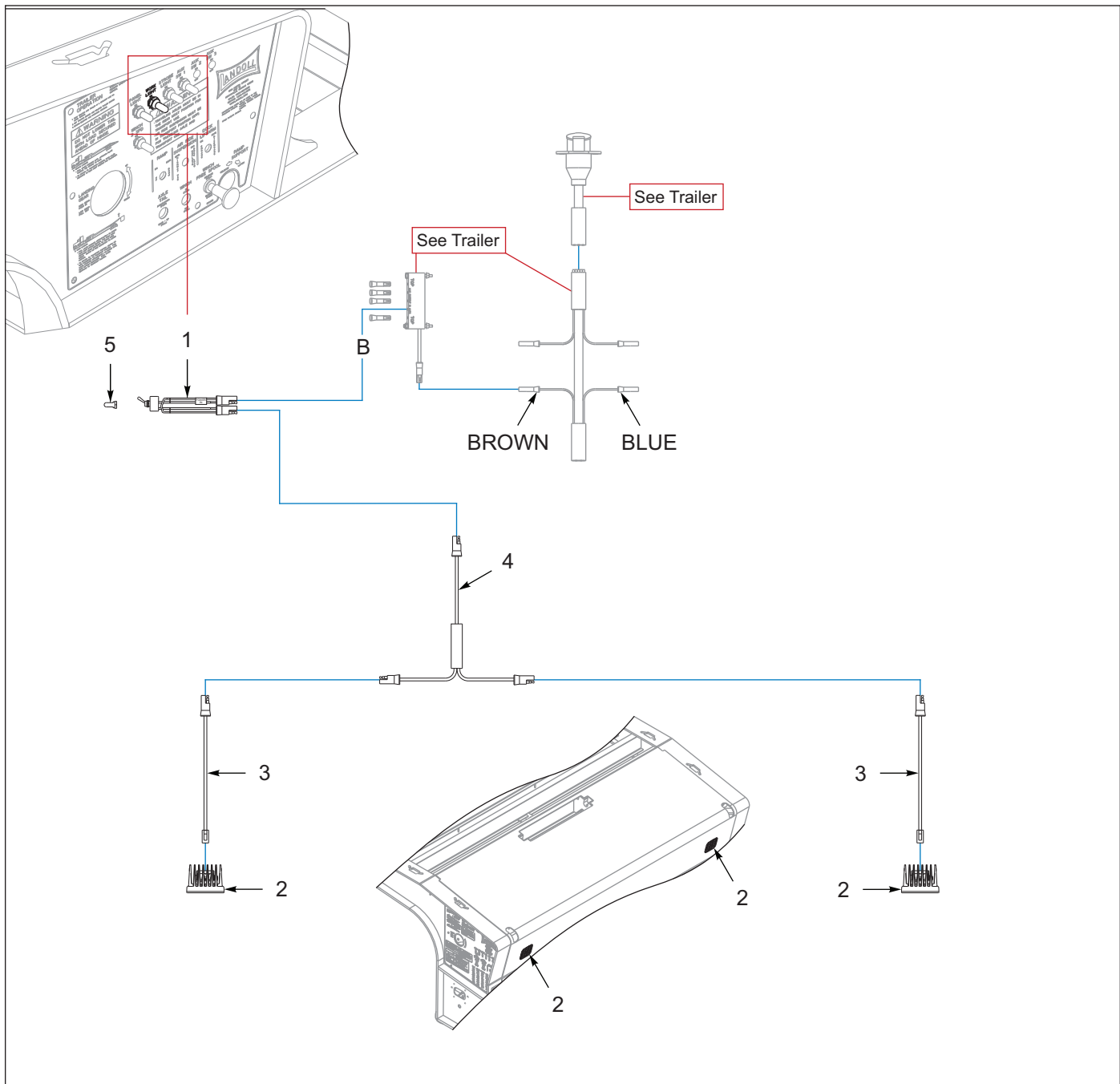
Figure 9-29: Lights, Work, Upper Deck, Slope (Option)
