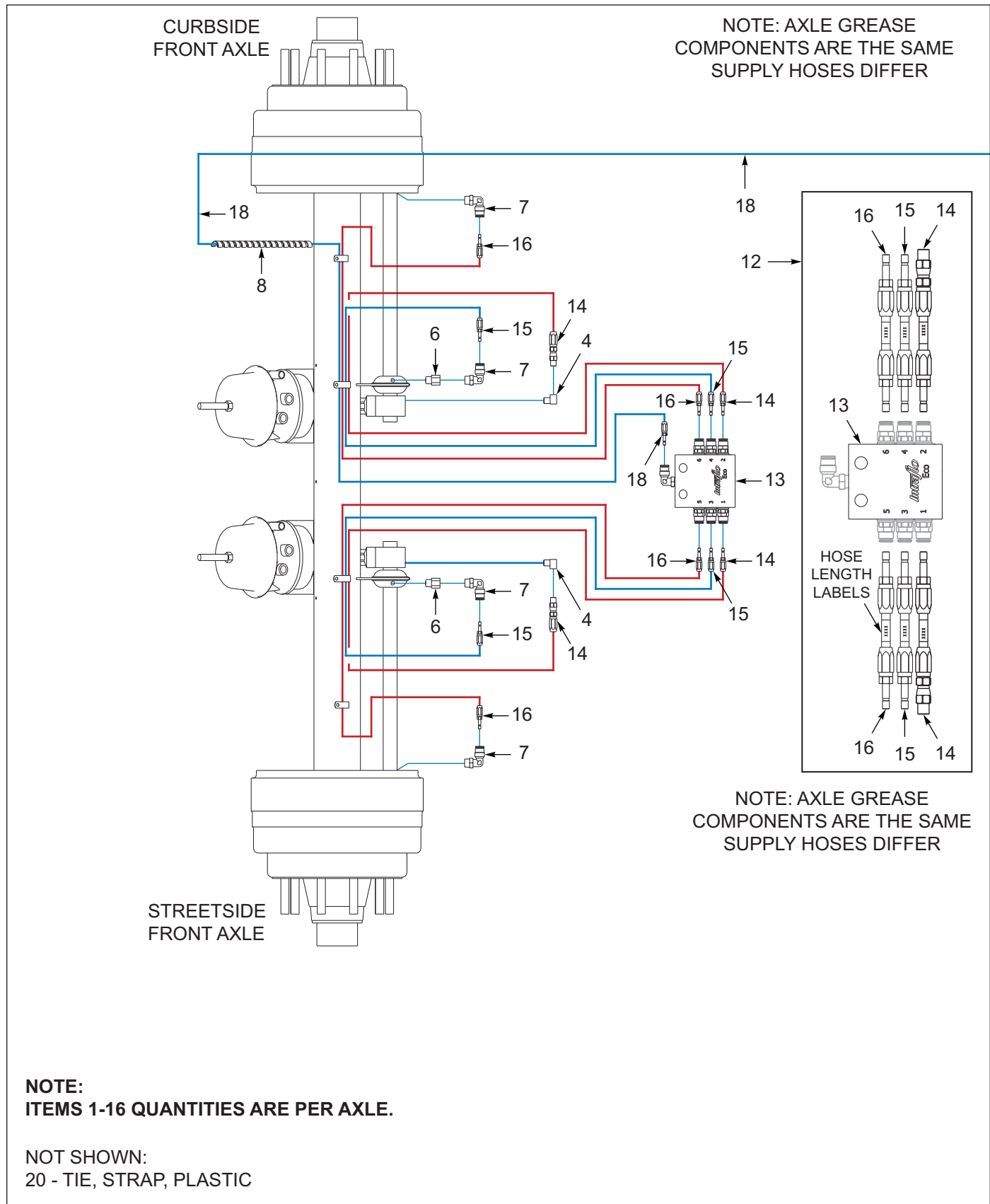
Figure 10-6: Axle, Drum Brakes (After 08/31/2020 To 09/01/2024) (1 of 3)
