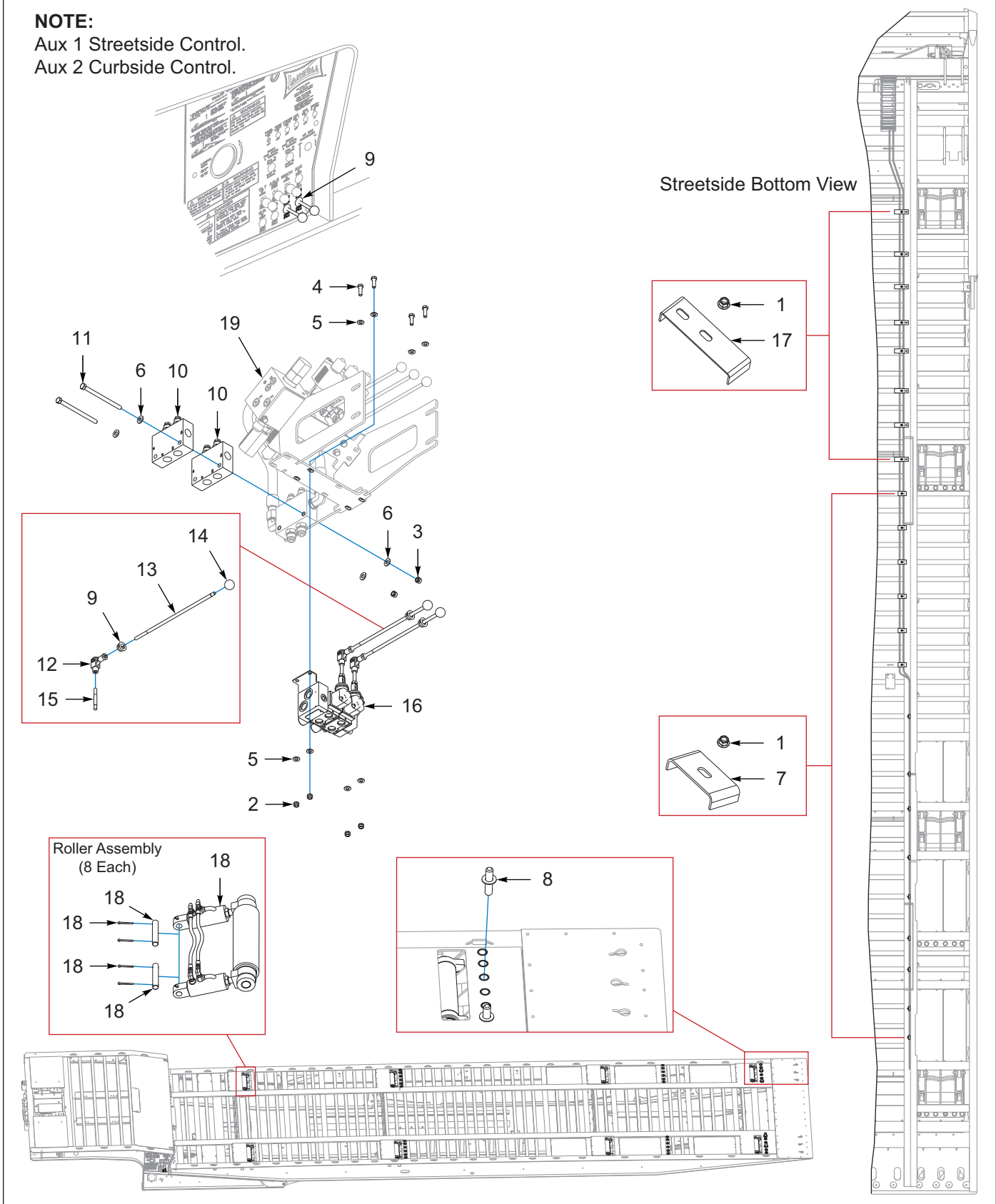
Figure 2-29: Rollers, Deck, 8-Pop-Ups (Options)
