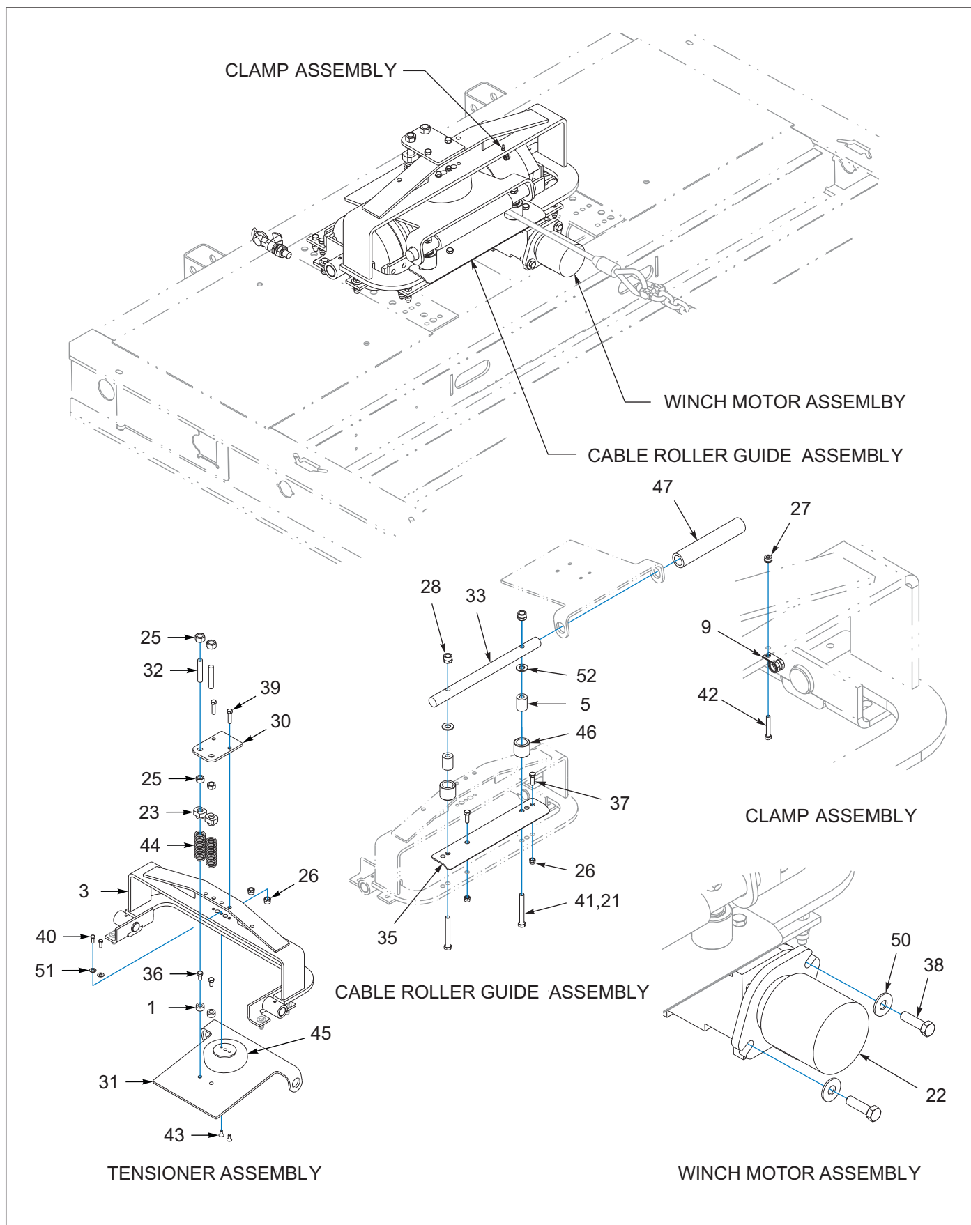
Figure 7-4: Winch Install, Braden 20K, 1-Speed, Air Tension (2 of 3)
