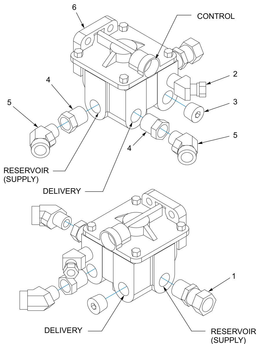
Figure 8-61: Valve Assembly, Air Booster
