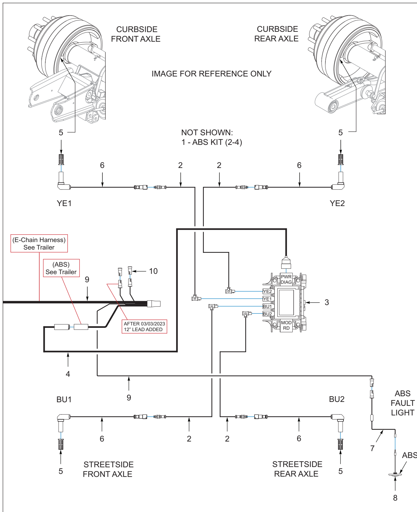
Figure 9-5: ABS, Wabco (1 of 2)
