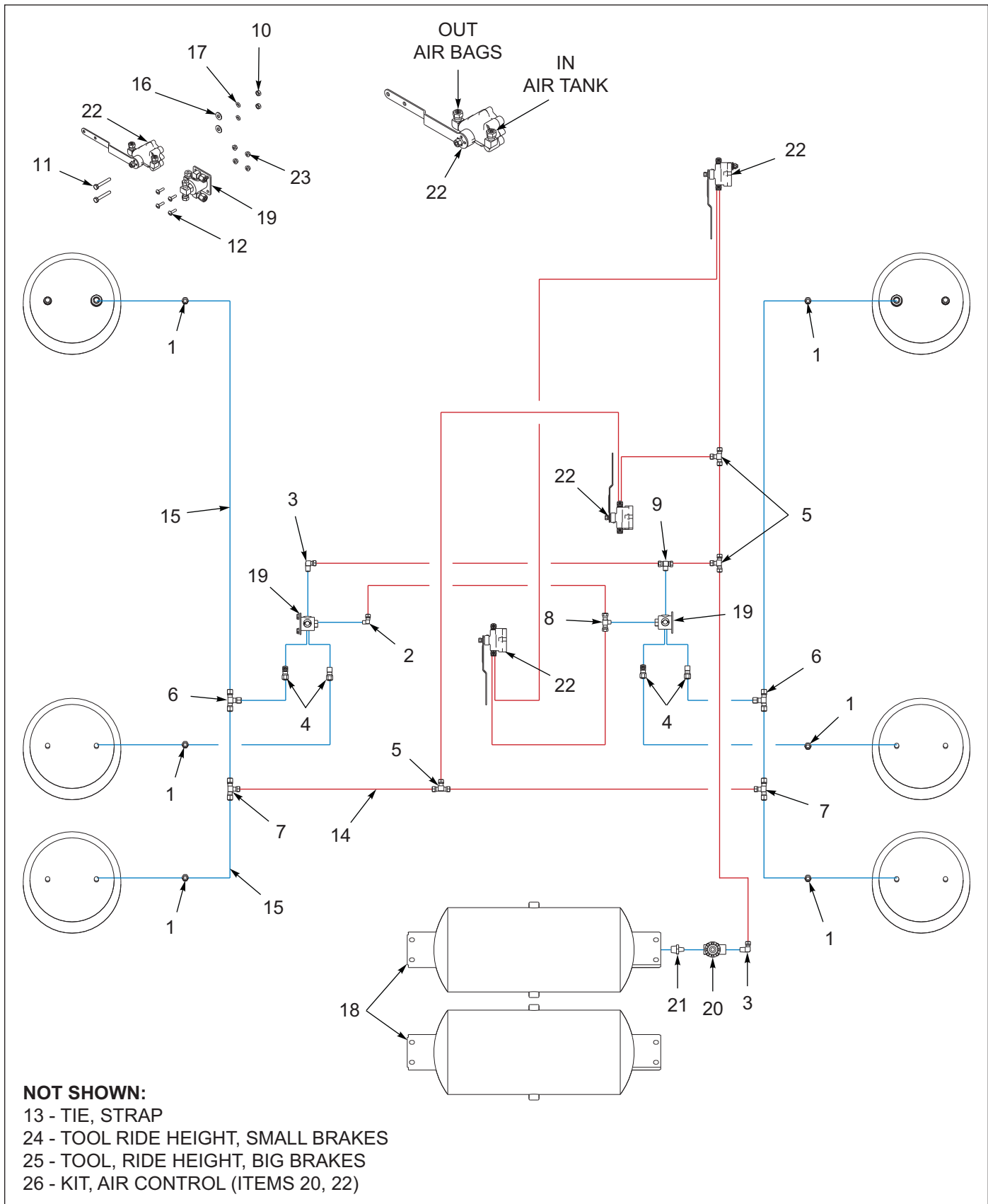
Figure 8-48: Suspension, Air Ride, 3 Ax, Aqua, 1/4 in (Option) (Before 03/10/2023)
