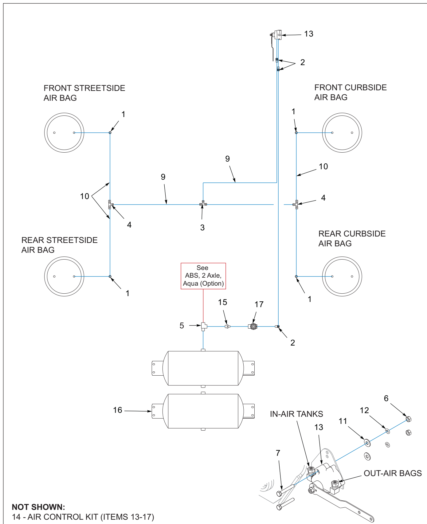
Figure 8-43: Suspension, Air Ride, 2 Ax, Aqua (Option)
