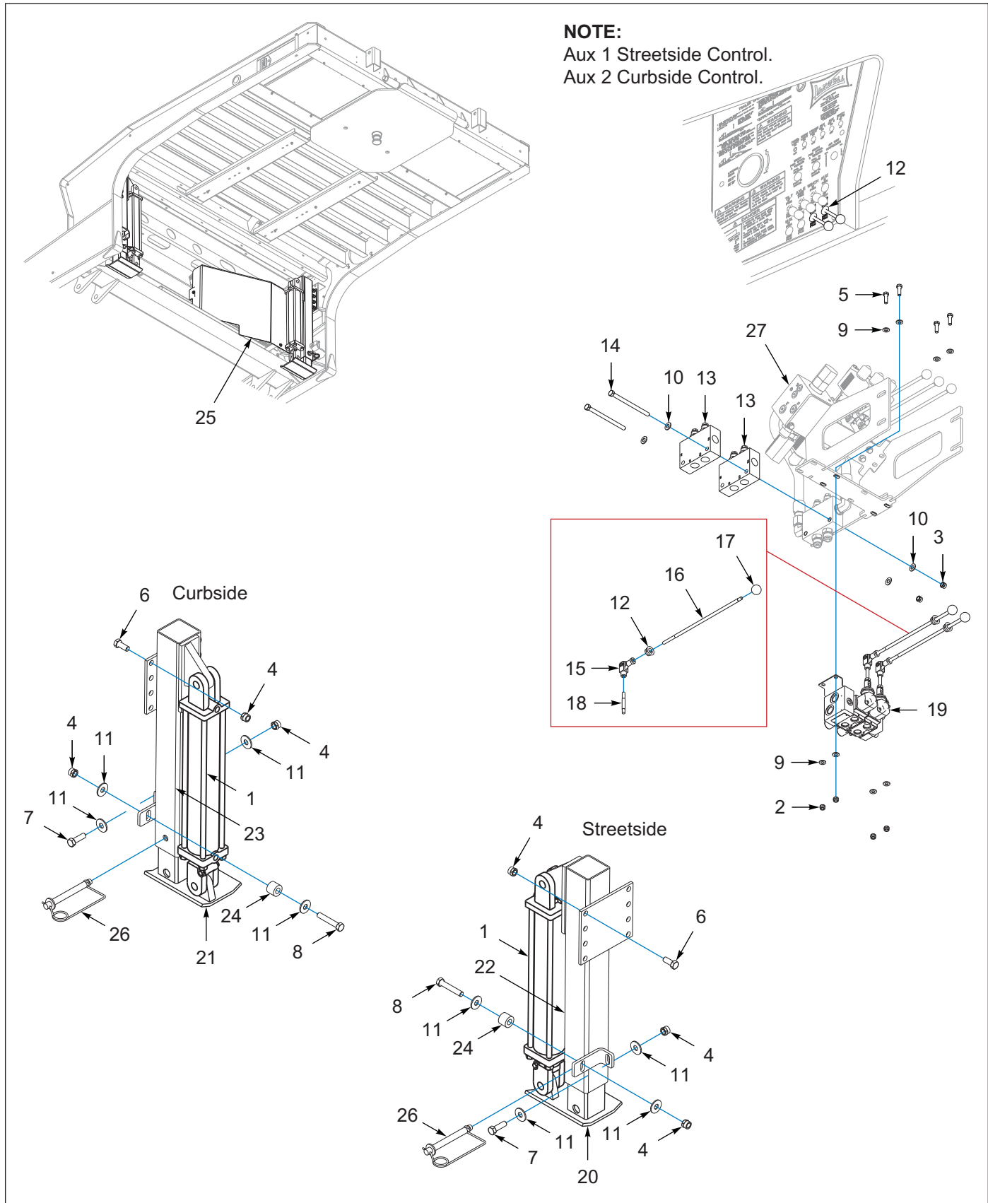
Figure 2-22: Landing Legs, Hydraulic (Option)
