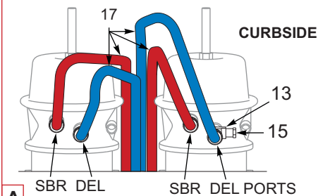
Figure 8-31: ABS, 3 Axle, Drum, Aqua (Option) (After 06/12/2023) (1 of 3)
