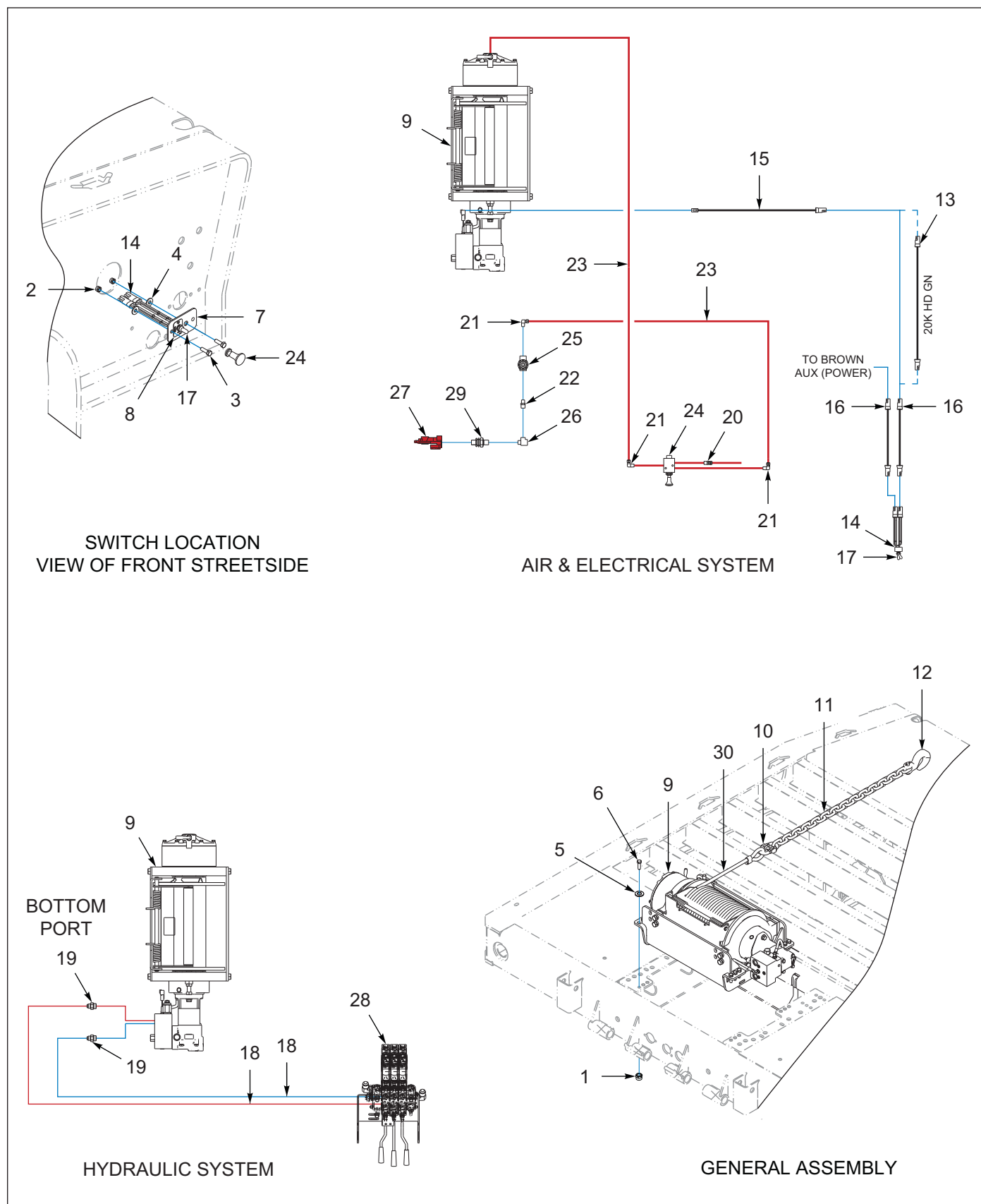
Figure 7-8: Winch Install, Warn 20K / 30K, 2-Speed
