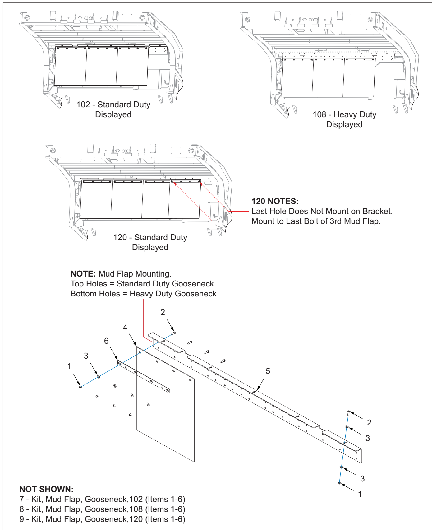
Figure 2-26: Mud Flaps, Gooseneck (Options)
