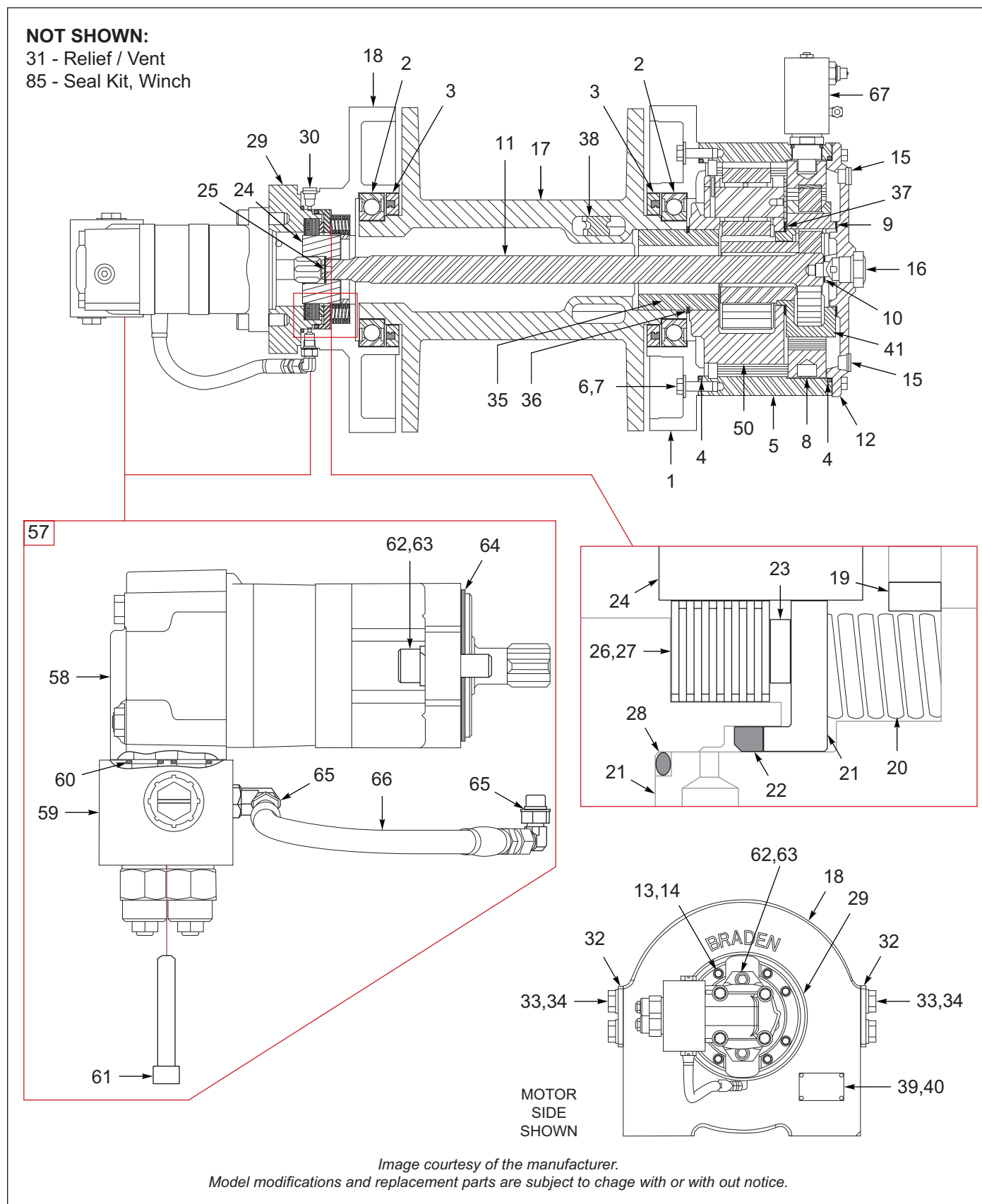
Figure 7-17: Winch Components, Braden 30K, 2-Speed (1 of 2)
