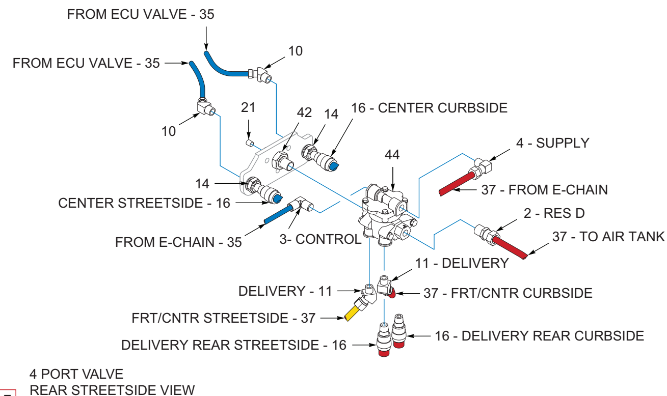
Figure 8-21: ABS, 3 Axle, Drum, Wabco (06/12/2023 To 10/06/2023) (3 of 3)
