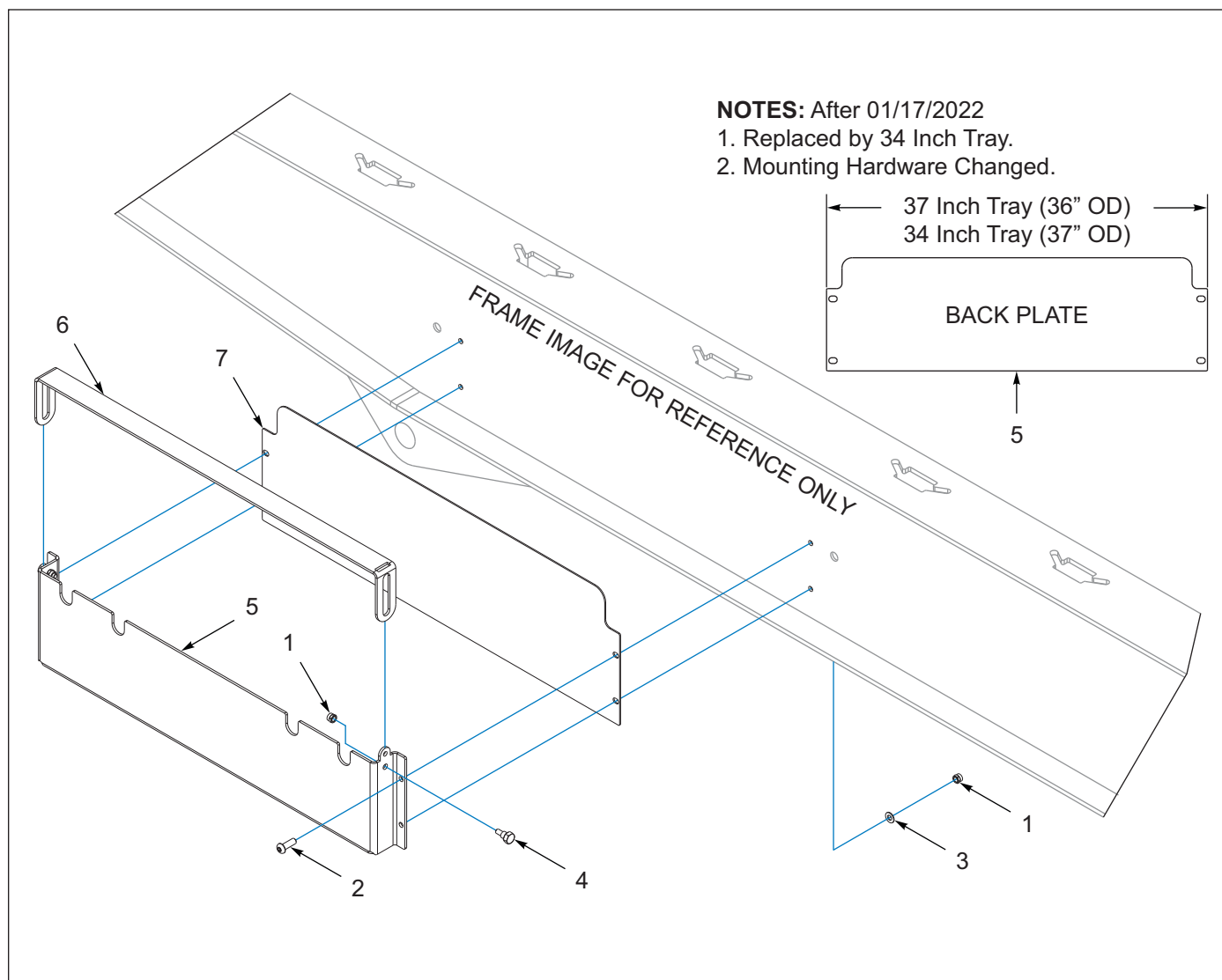
Figure 4-7: Chain Tray, Beam, Bolt-On (Before 01/17/2022)
