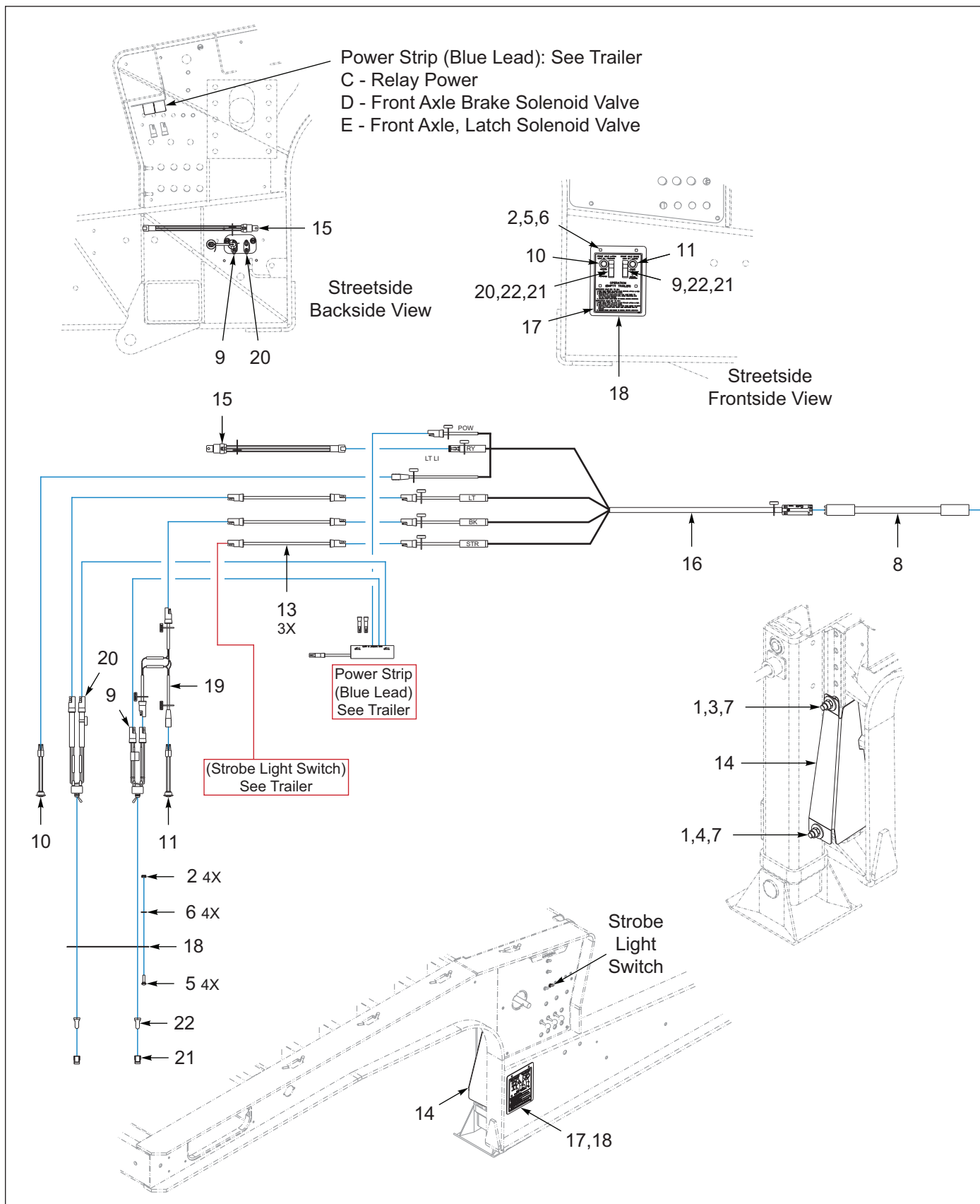
Figure 9-16: Latch Lock, 2 Axle Spread (Option) (1 of 2)
