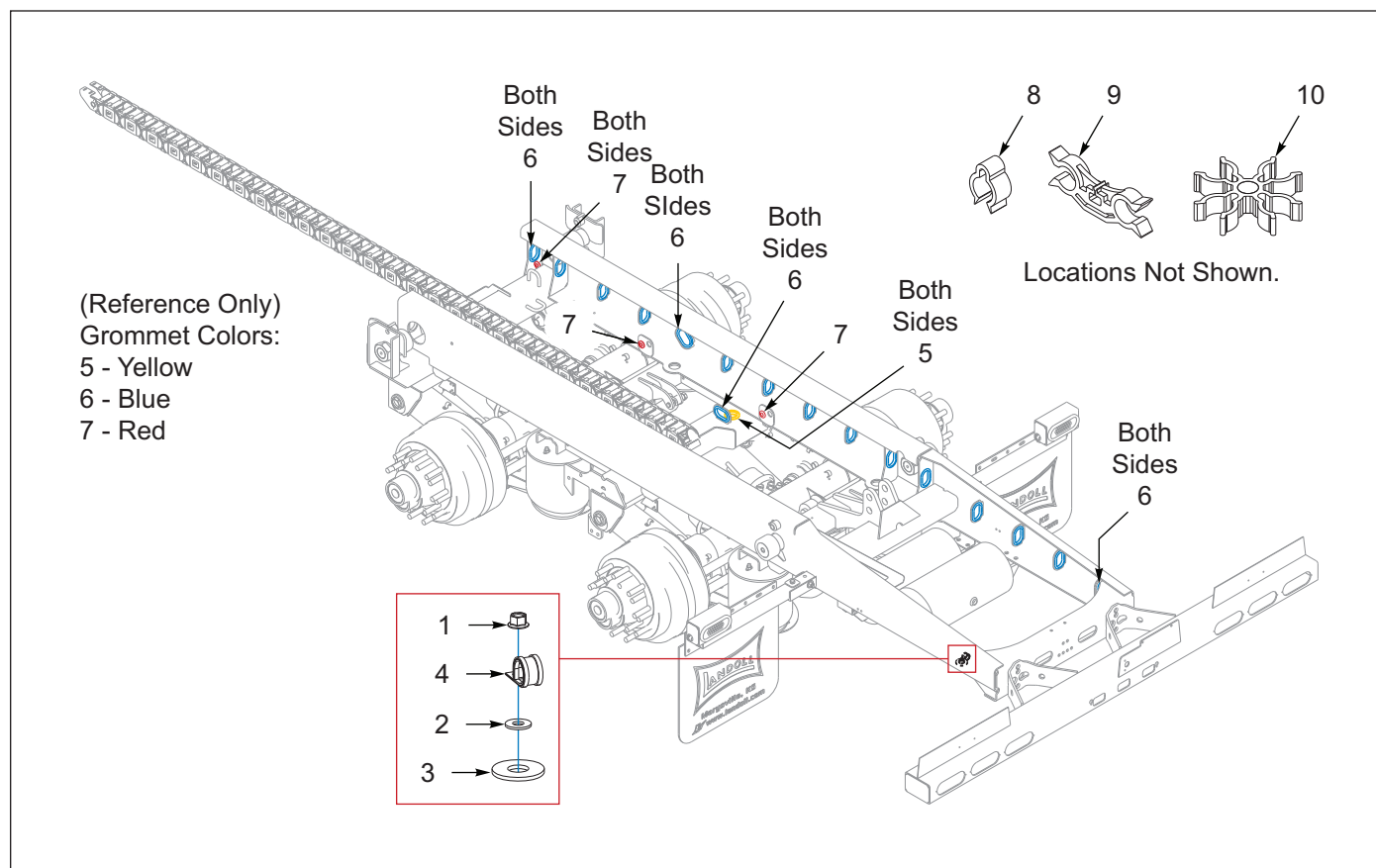
Figure 2-16: Hose Clamps, Clips, Grommets, 2 Axle (After 09/01/2024)
