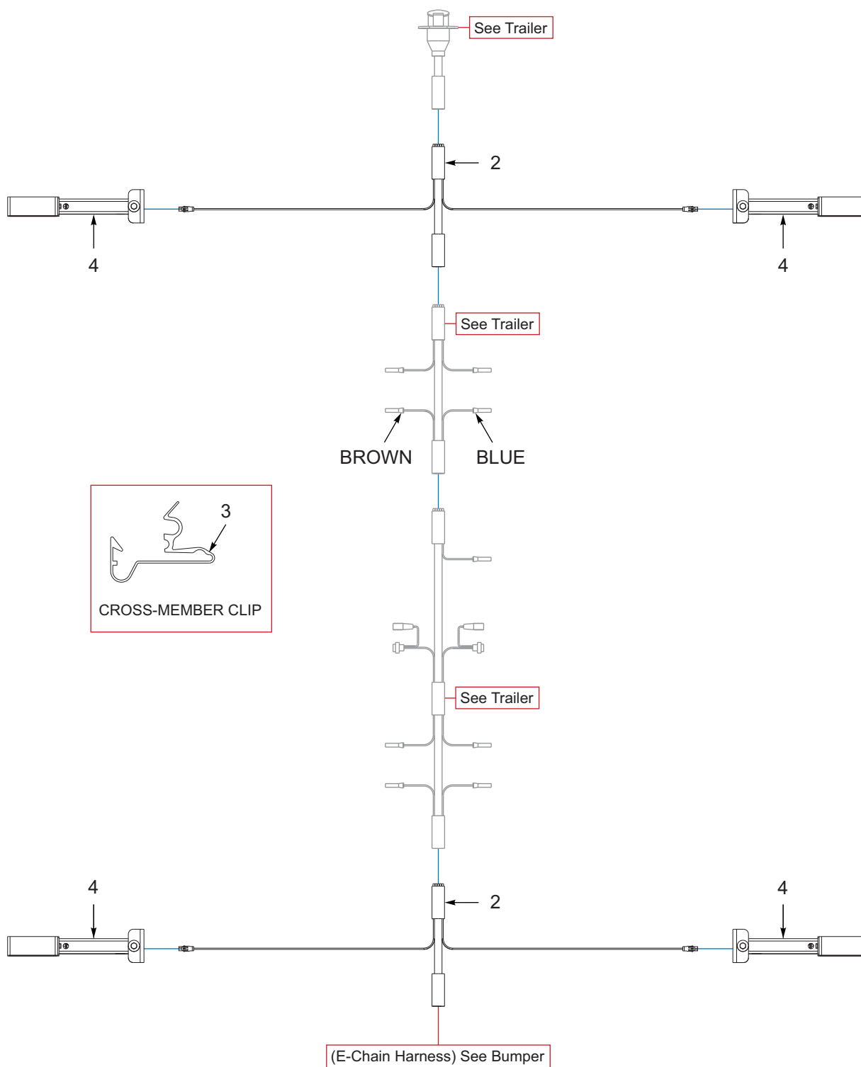
Figure 9-26: Lights, Swing Arm, Turn / Emergency, Amber (Options) (1 of 2)
