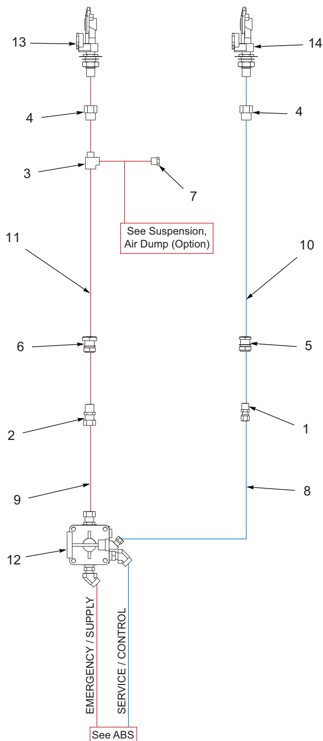
Figure 8-1: Trailer, Service & Emergency
