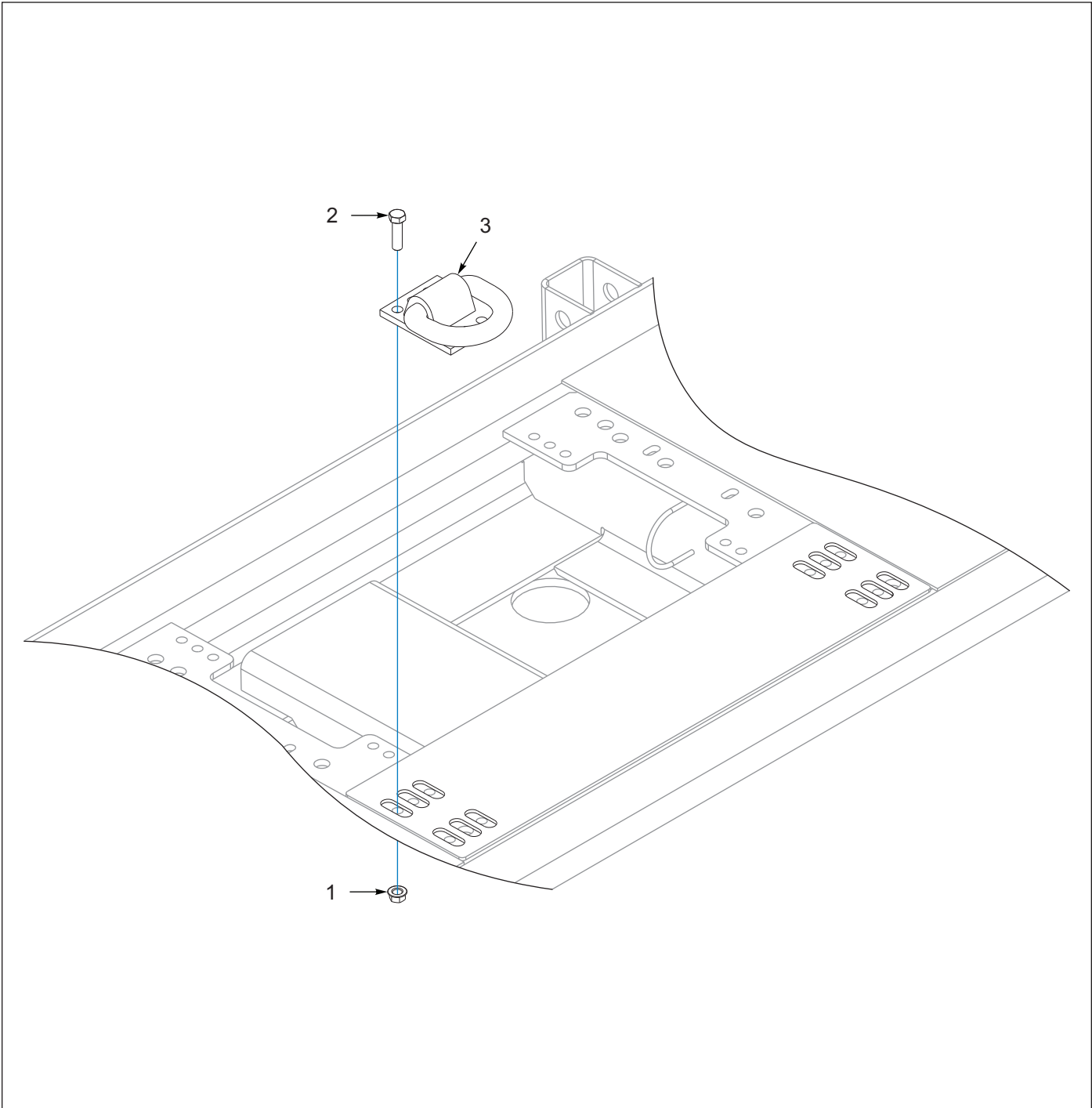
Figure 7-28: Tie Down, D-Ring, Bolt-On, Winch
