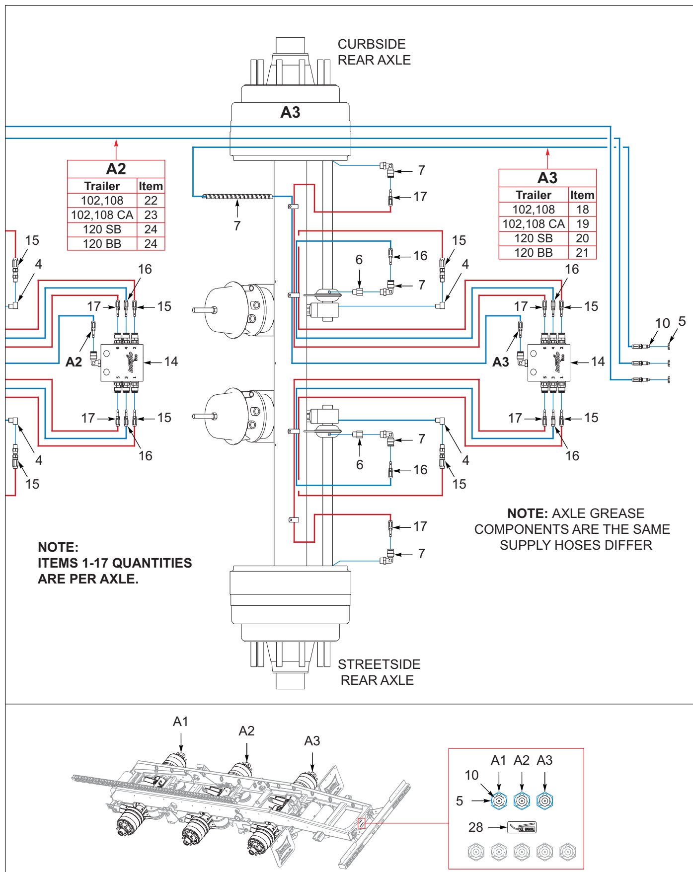
Figure 10-24: 3 Axle, Drum Brakes (After 12/01/2025) (2 of 3)
