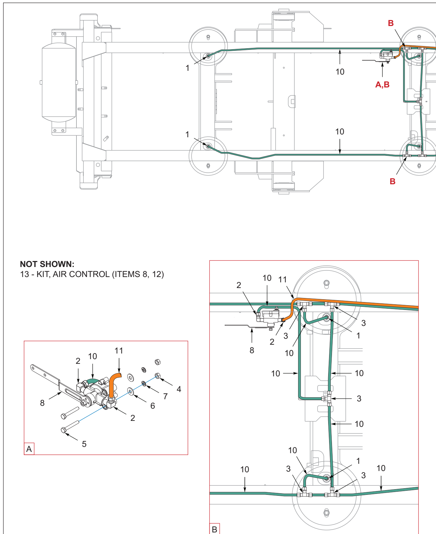
Figure 8-49: Suspension, Air Ride, 3 Ax, Aqua, 3/8 in (Option) (After 03/10/2023) (1 of 2)
