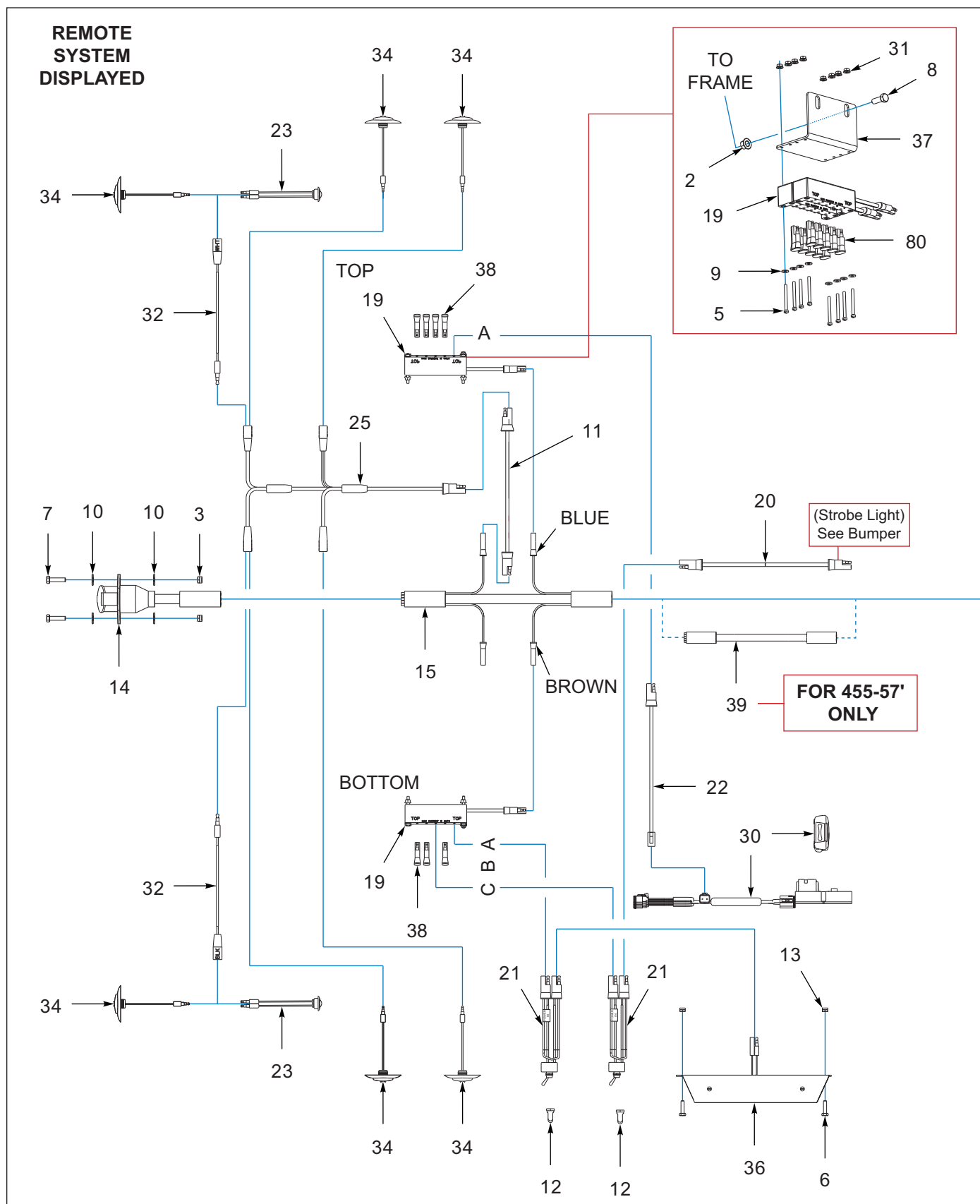
Figure 9-2: Trailer (1 of 2) (After 6/13/2023)
