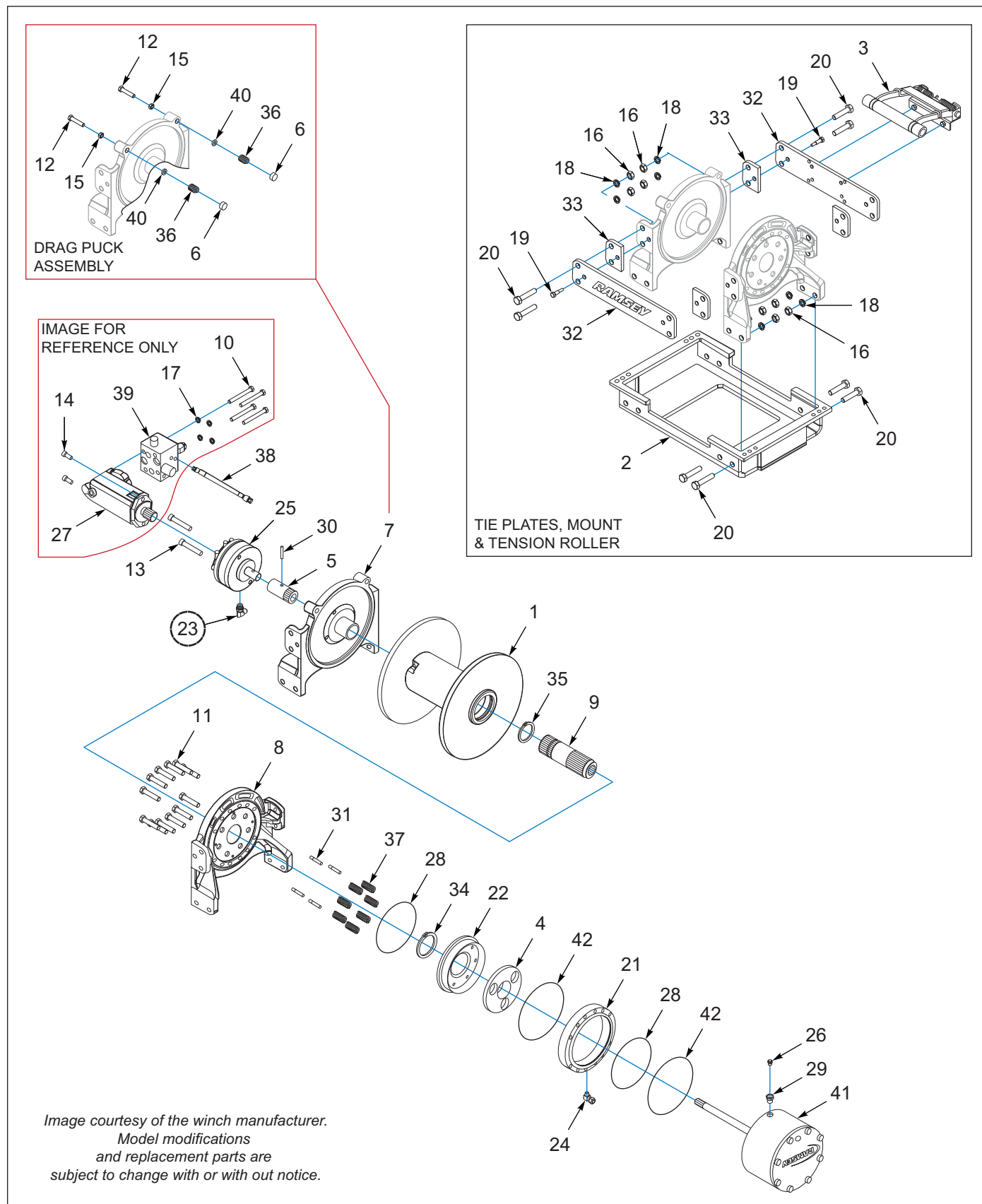
Figure 7-20: Winch Components, Ramsey 30K, 2-Speed
