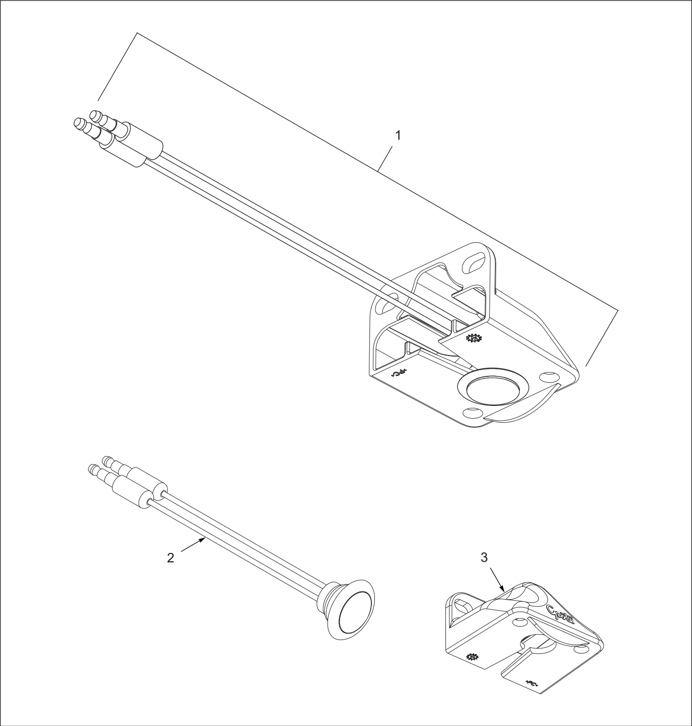
Figure 9-19: Light Assembly, License Plate
