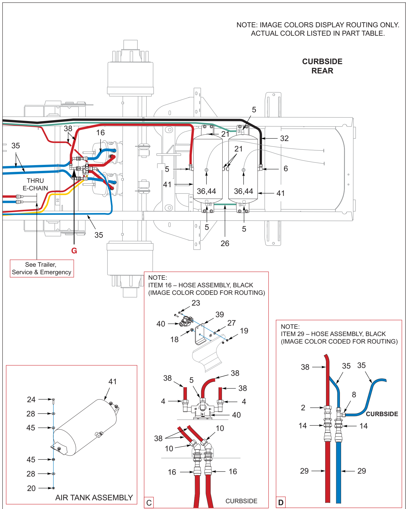
Figure 8-32: ABS, 3 Axle, Drum, Aqua (Option) (After 06/12/2023) (2 of 3)
