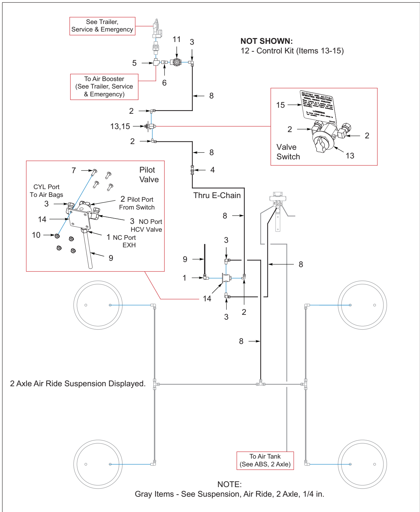
Figure 8-54: Suspension, Air Dump, 2 Axle, 1/4 in (Option) (BEFORE 06/14/2023)
