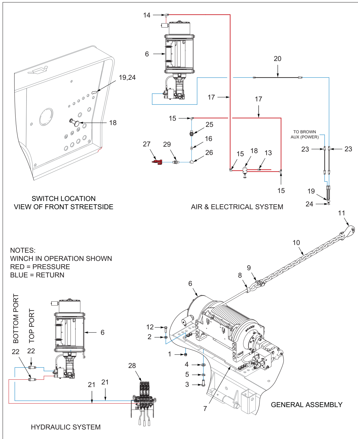
Figure 7-6: Winch Install, Braden 20K / 30K, 2-Speed
