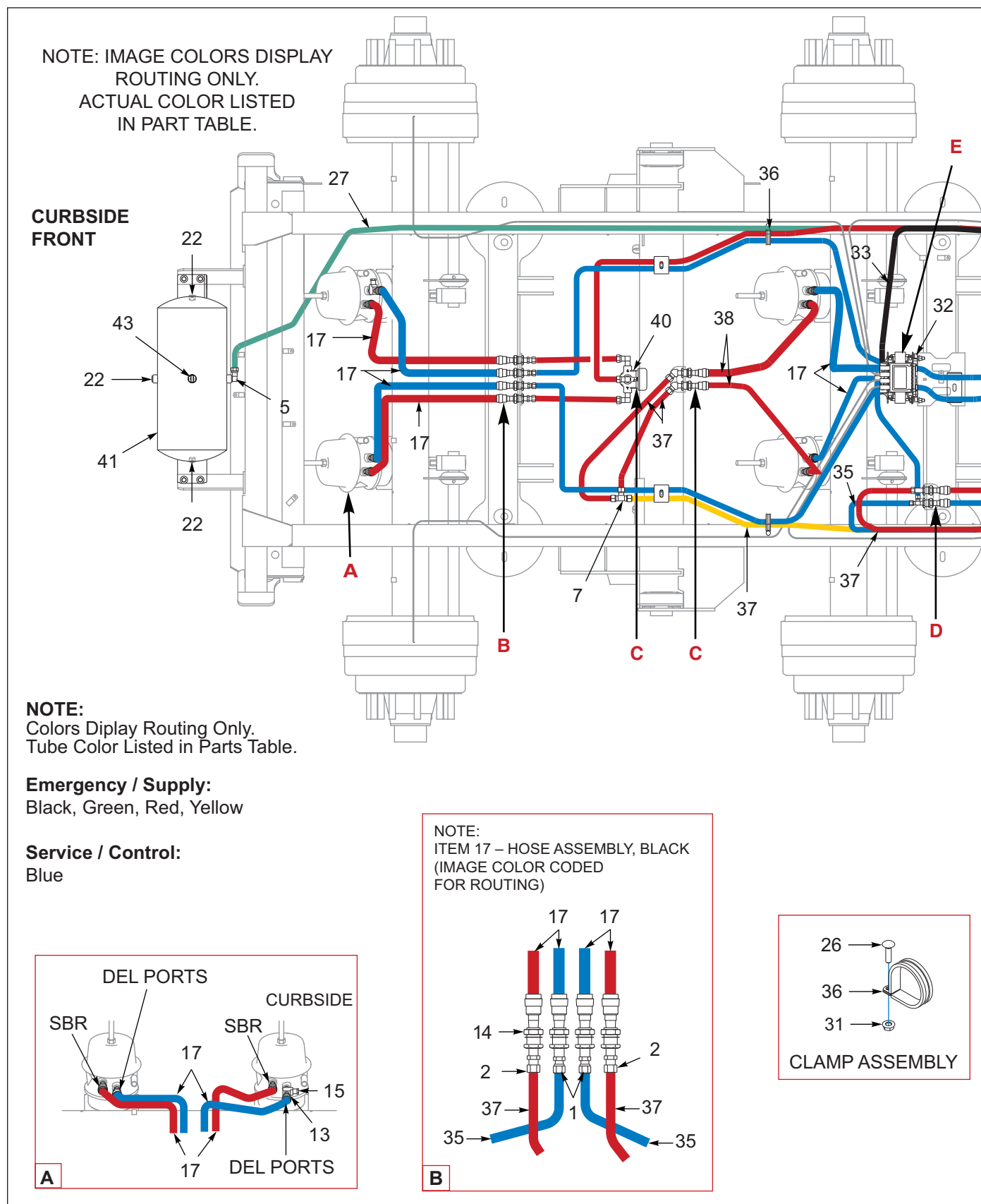
Figure 8-19: ABS, 3 Axle, Drum, Wabco (06/12/2023 To 10/06/2023) (1 of 3)
