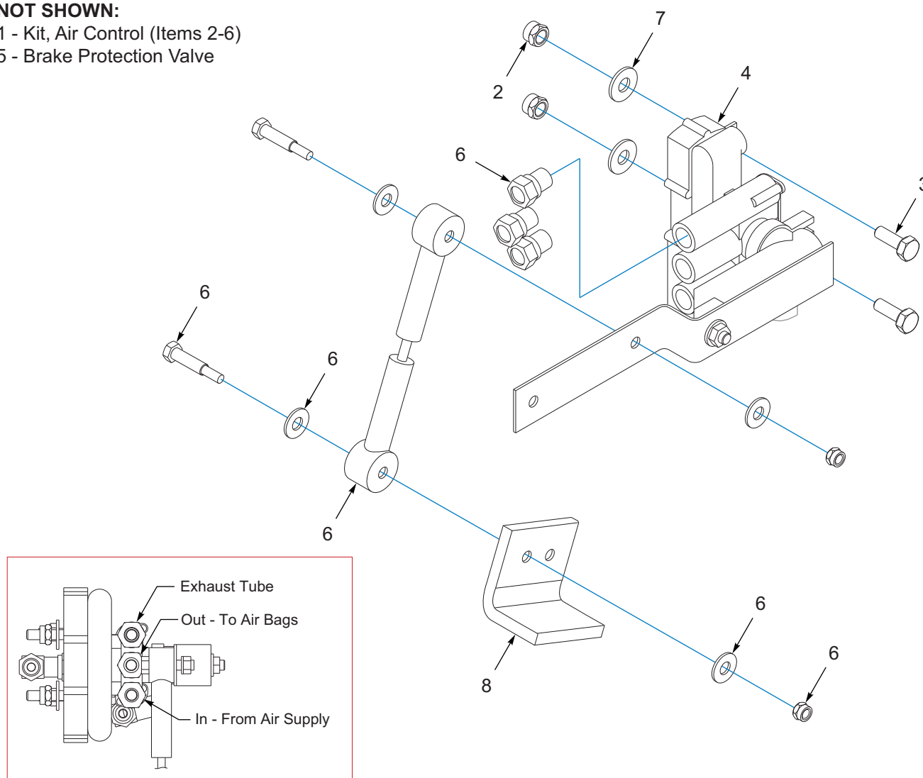
Figure 8-52: Suspension, Air Ride Control Kit, 3/8 in
