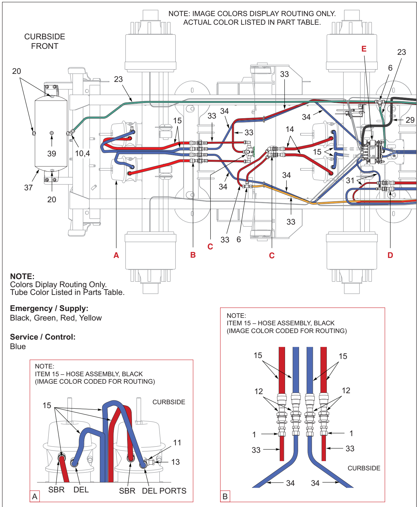
Figure 8-22: ABS, 3 Axle, Drum, Wabco (After 10/06/2023) (1 of 3)
