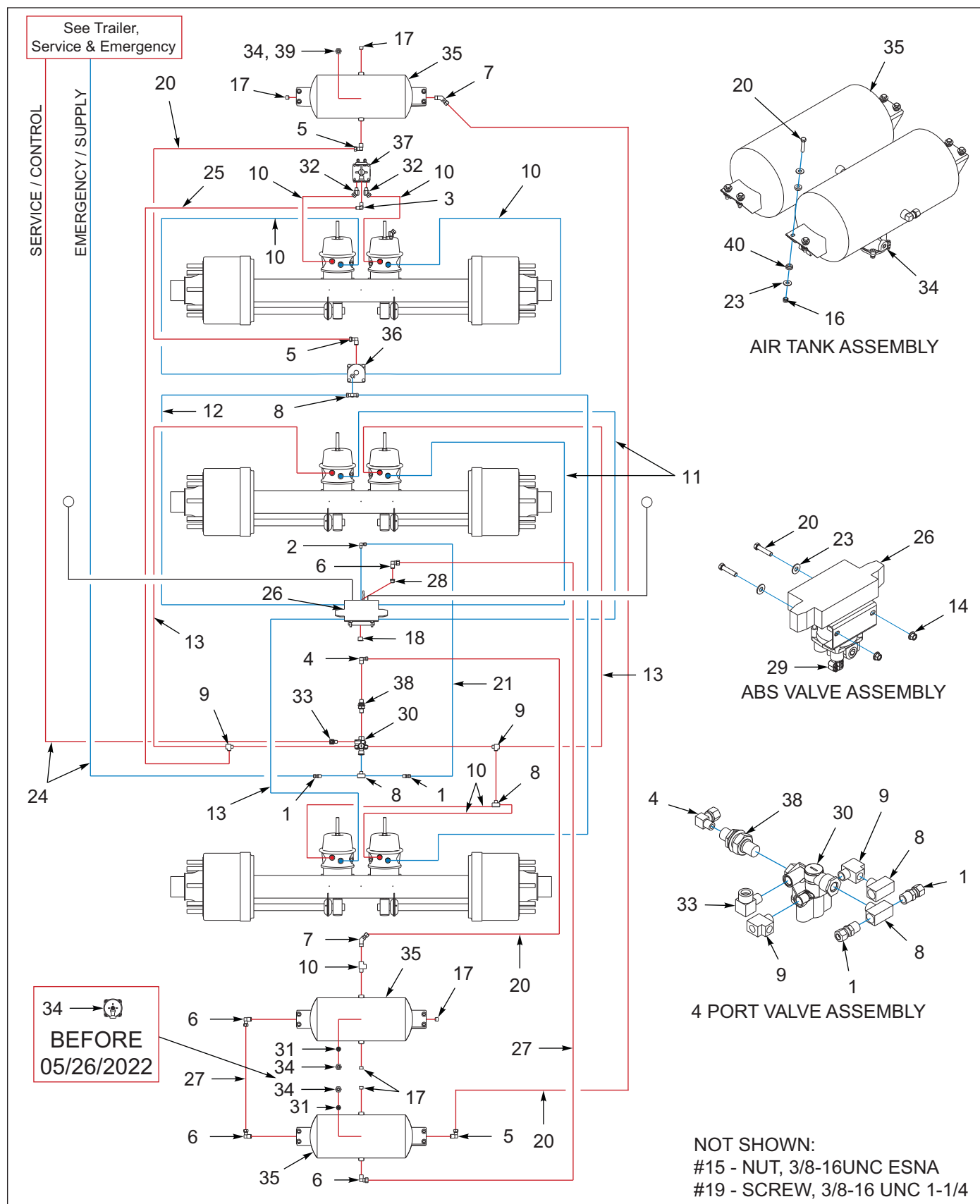
Figure 8-27: ABS, 3 Axle, Drum, Aqua (Option) (Before 03/10/2023)
