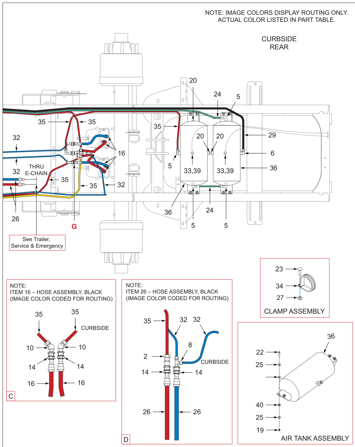
Figure 8-29: ABS, 3 Axle, Drum, Aqua (Option) (03/10/2023 To 06/12/2023) (2 of 3)
