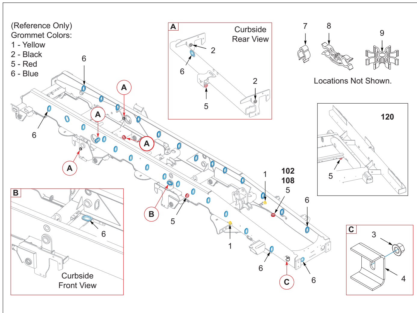
Figure 2-20: Hose Clamps, Clips, Grommets, 2 Axle (After 12/01/2025)
