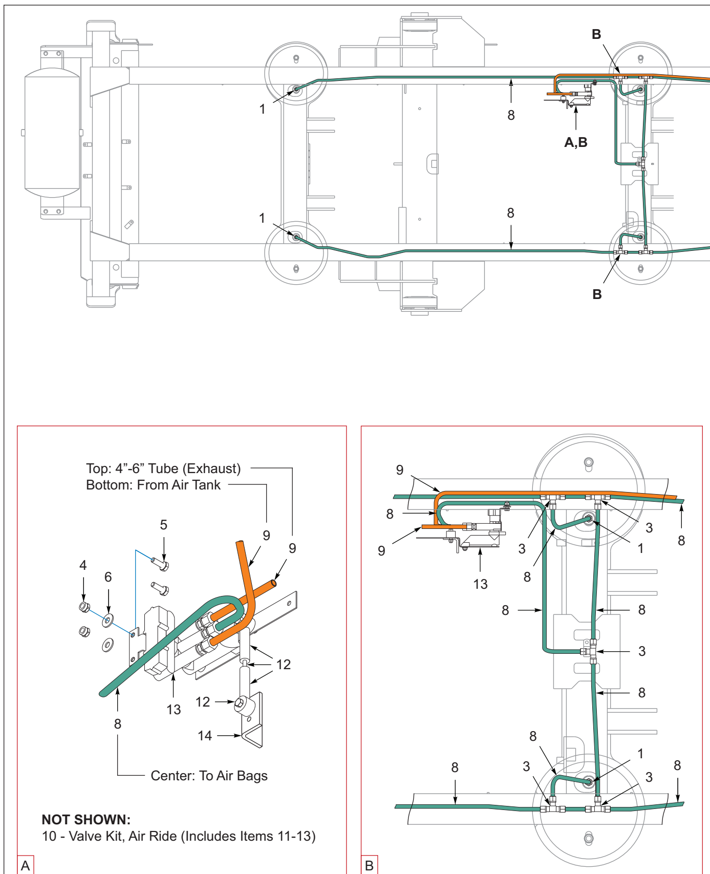
Figure 8-46: Suspension, Air Ride, 3 Ax, 3/8 in (After 03/10/2023) (1 of 2)
