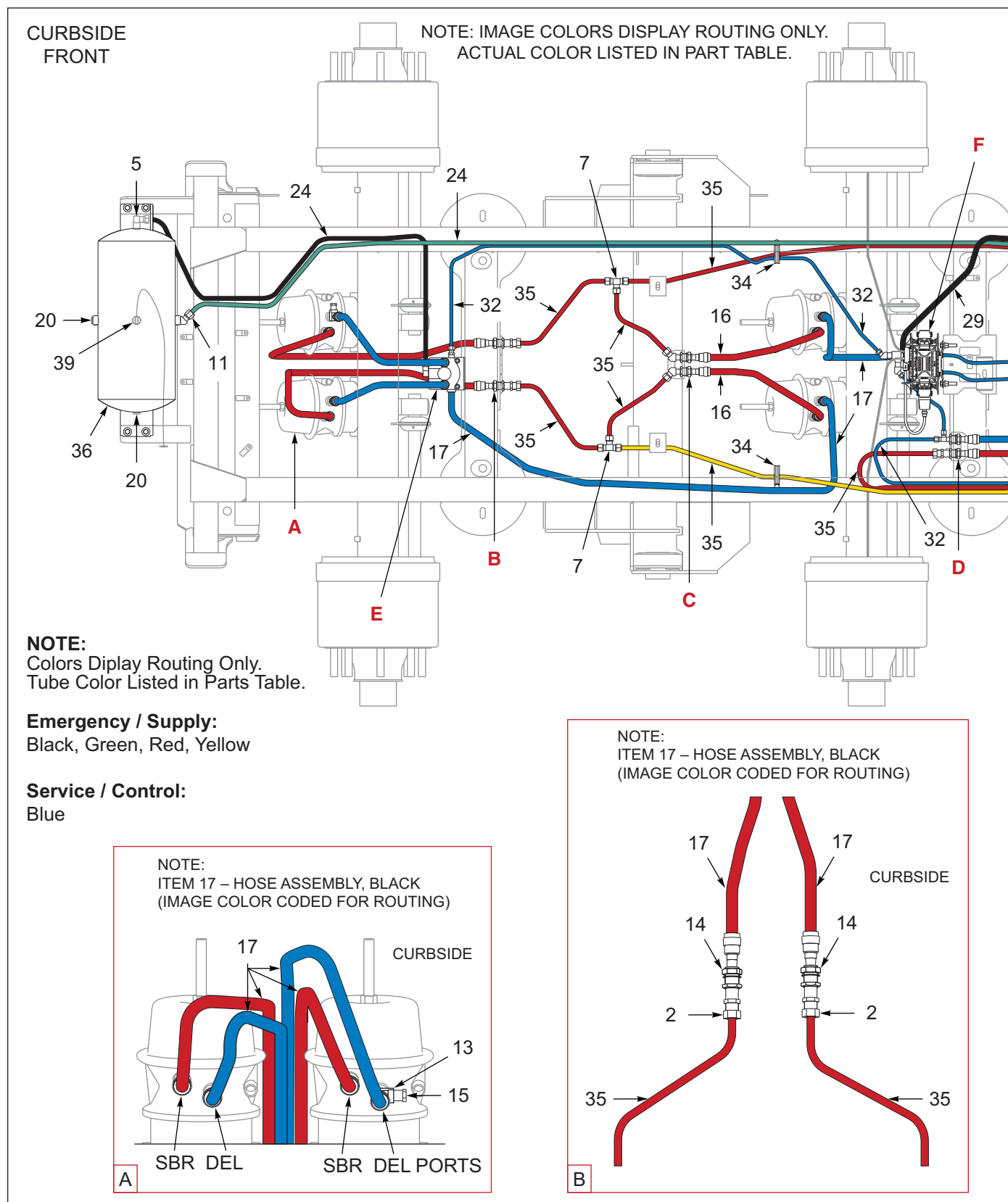
Figure 8-28: ABS, 3 Axle, Drum, Aqua (Option) (03/10/2023 To 06/12/2023) (1 of 3)
