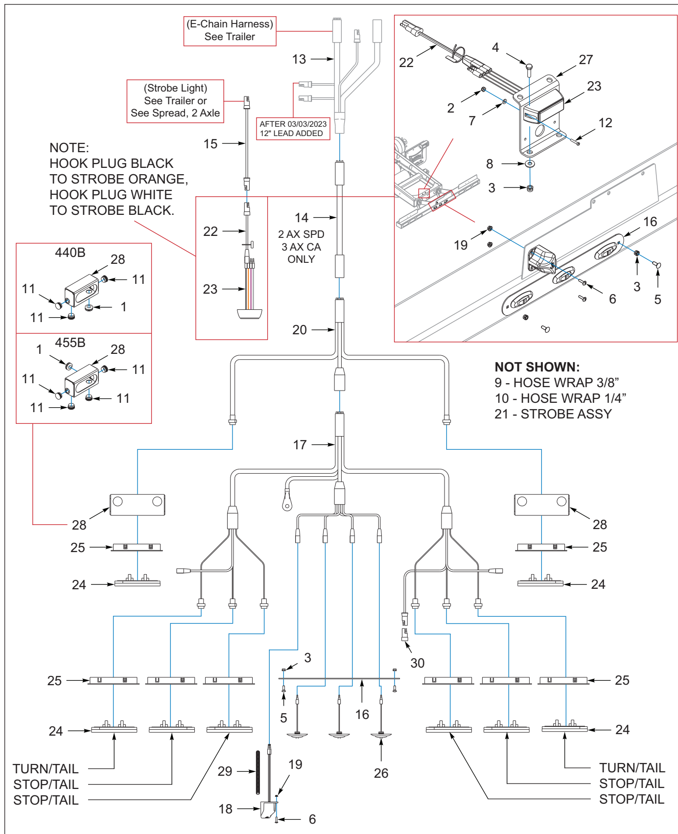
Figure 9-4: Bumper Assembly
