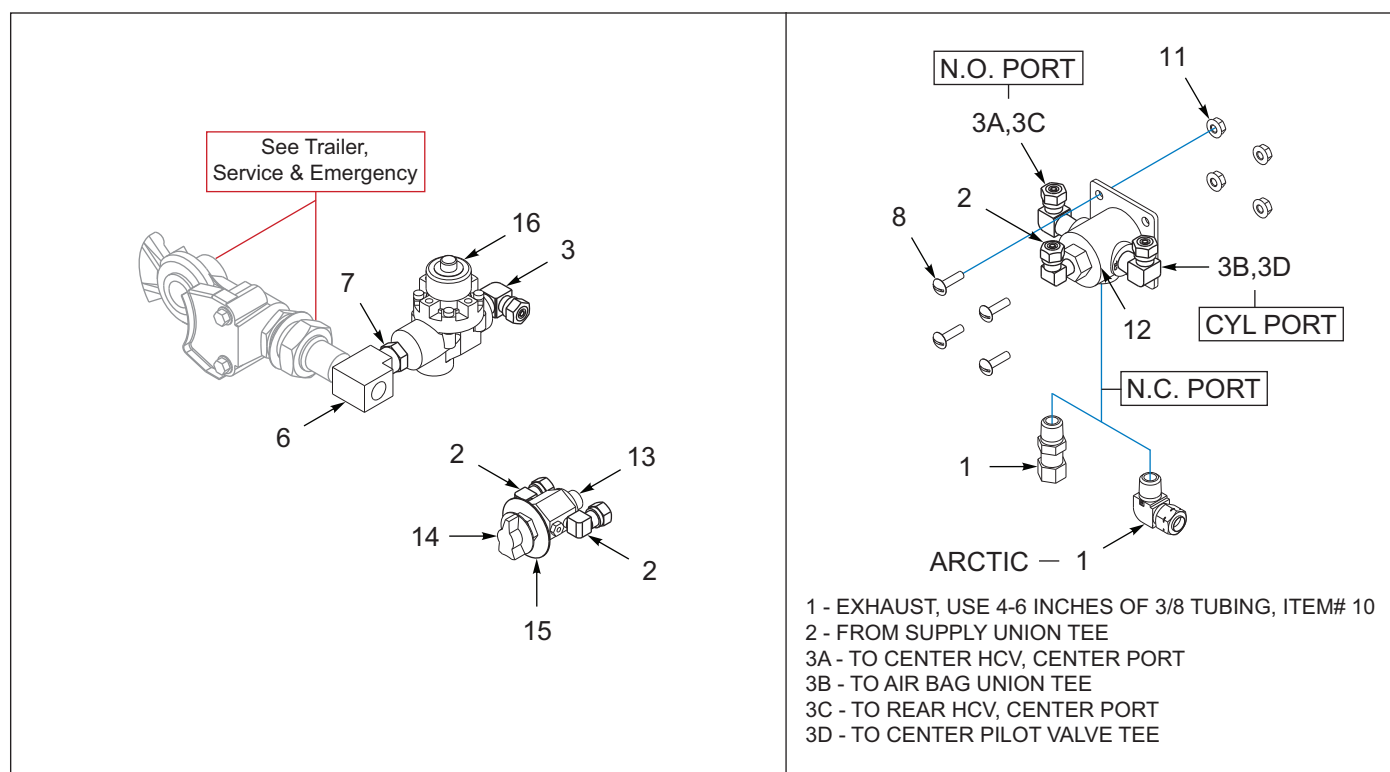
Figure 8-57: Suspension, Air Dump, 3 Axle, Double Pilot (Option) (2 of 2)
