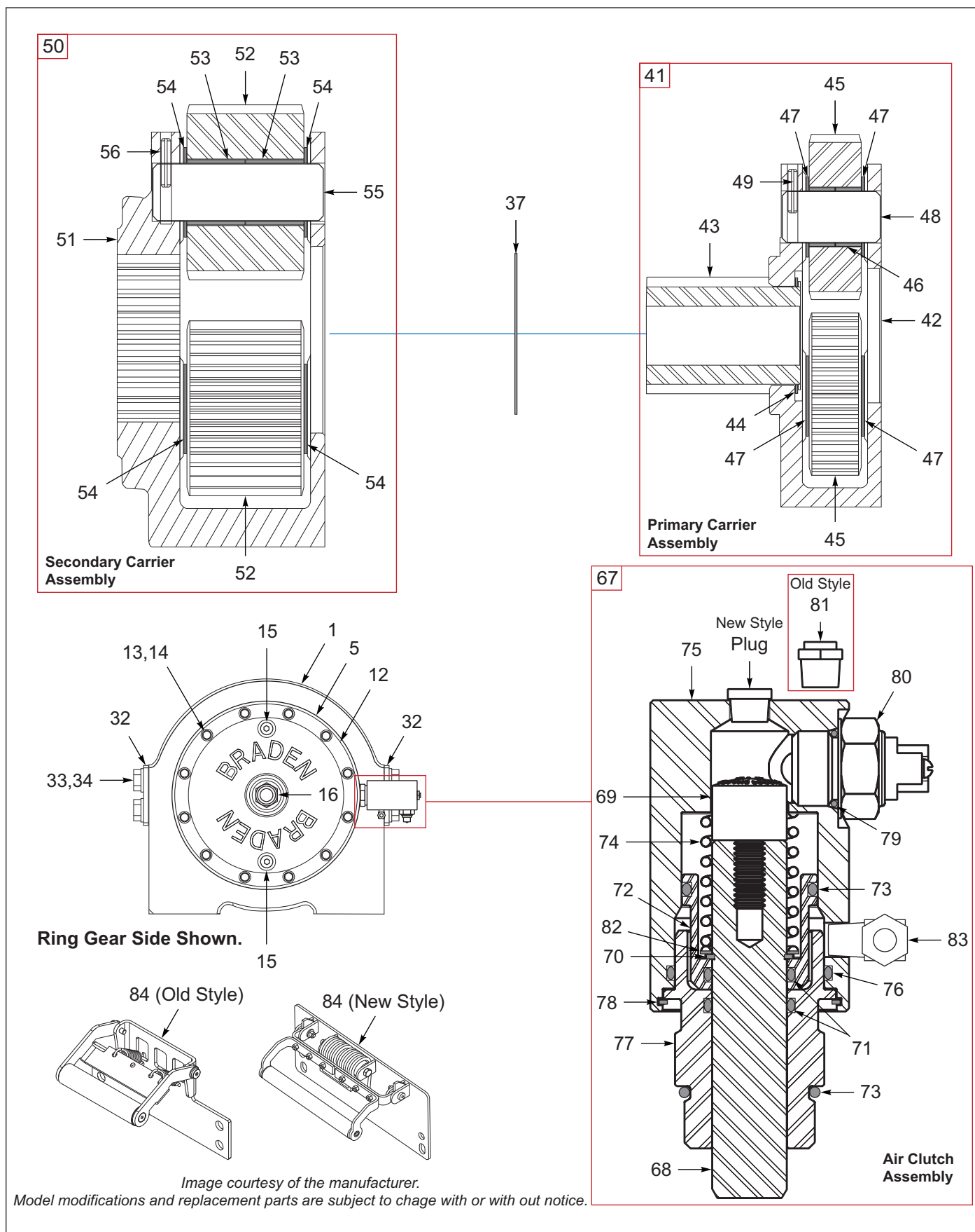
Figure 7-18: Winch Components, Braden 30K, 2-Speed (2 of 2)
