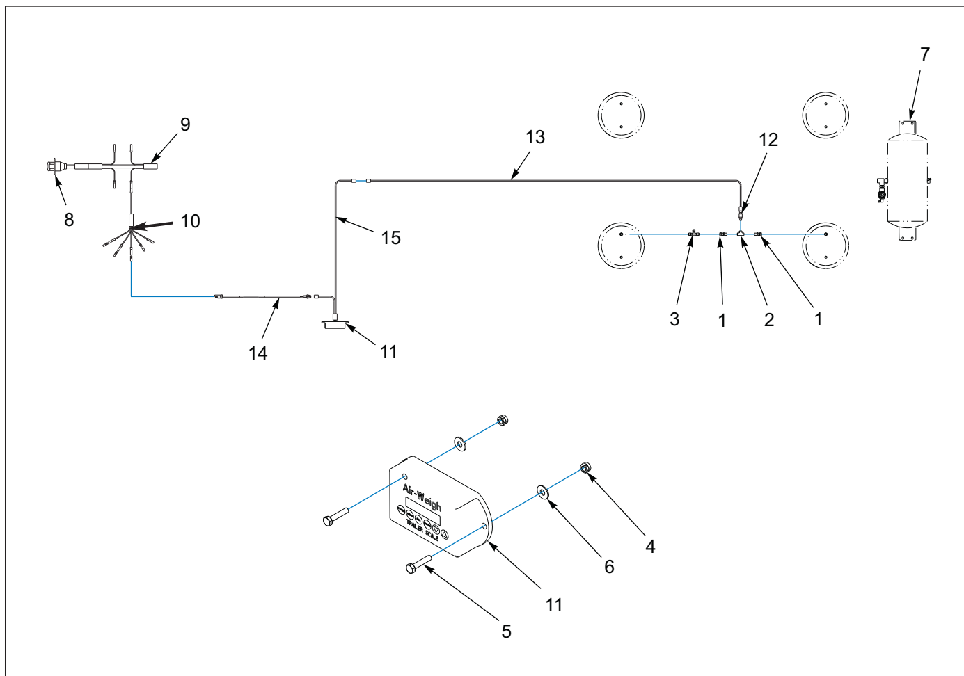
Figure 8-36: Scale, Loadmaxx (Option) (Before 03/31/2020)
