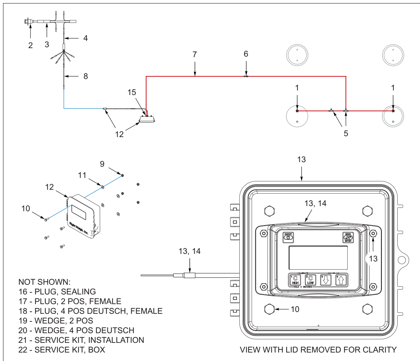
Figure 8-39: Scale, Right Weigh (Options)
