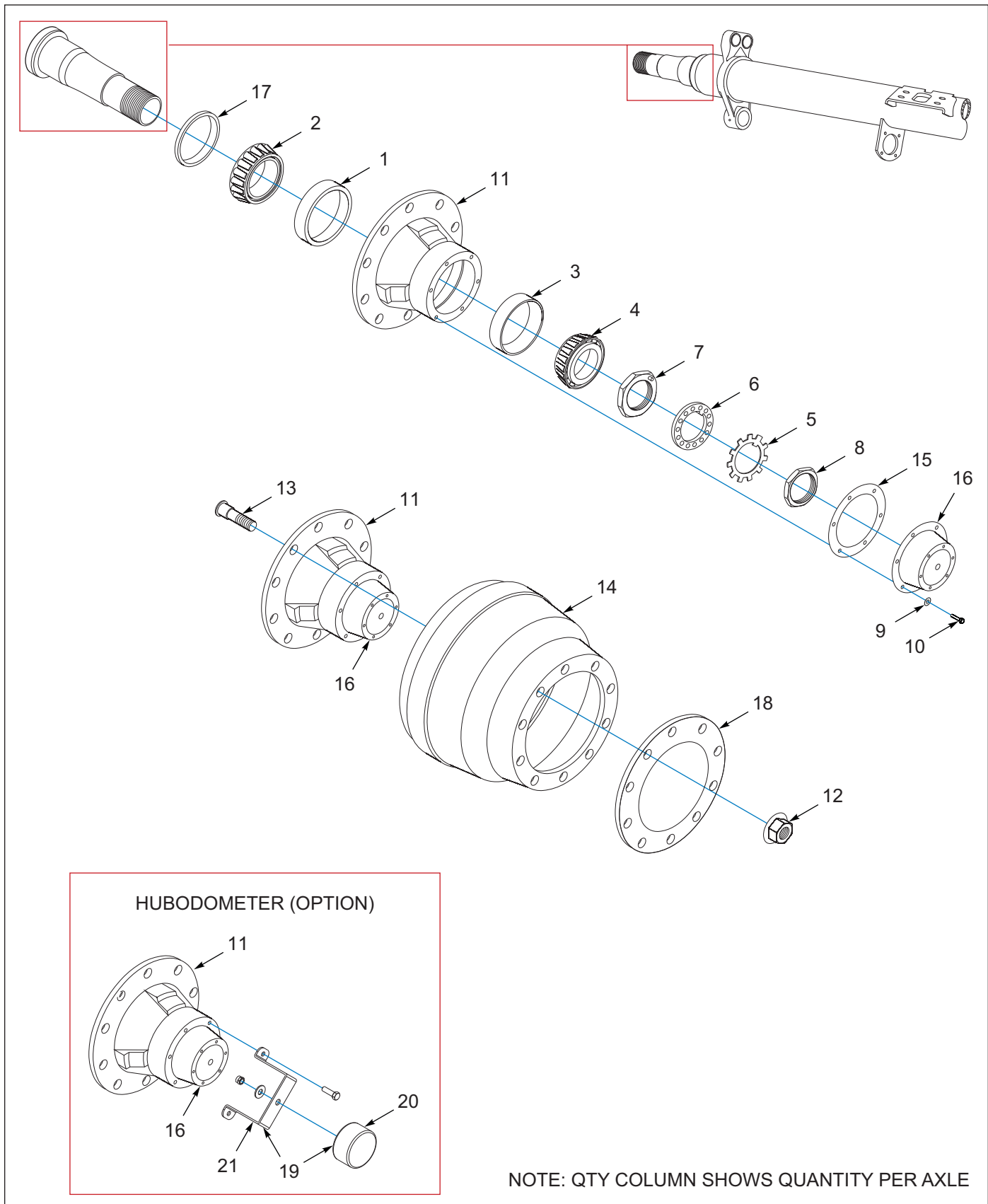
Figure 3-6: Axle Components, 16.50 x 7.00, Drum &amp; Hub
