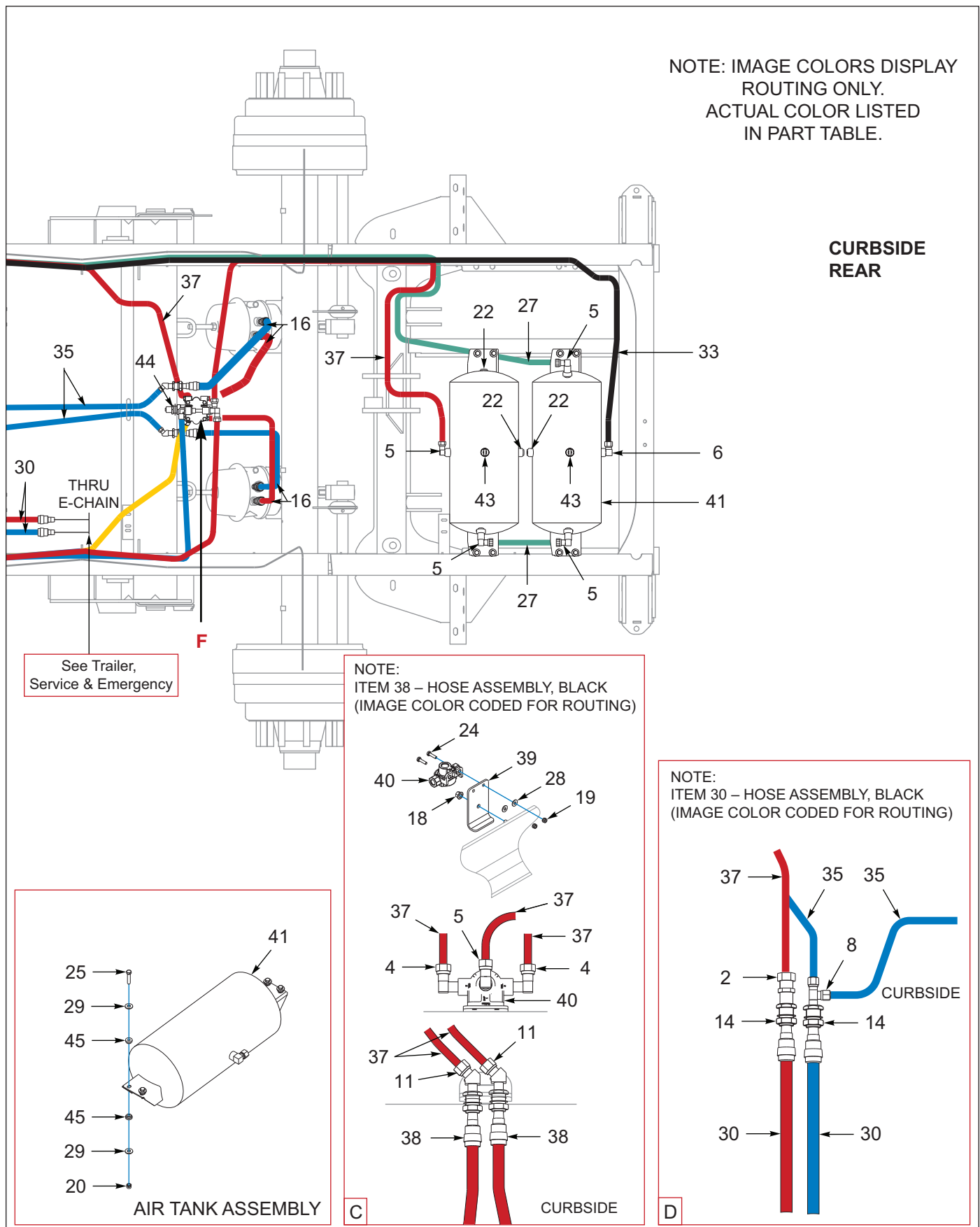
Figure 8-20: ABS, 3 Axle, Drum, Wabco (06/12/2023 To 10/06/2023) (2 of 3)
