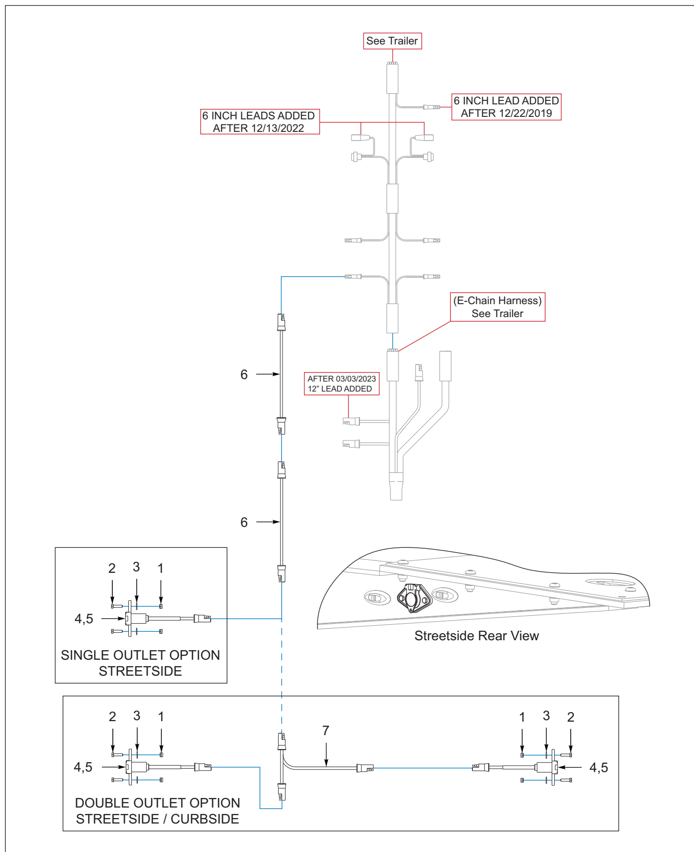
Figure 9-33: Outlet, Electrical, 4-Pole, Rear (Options)
