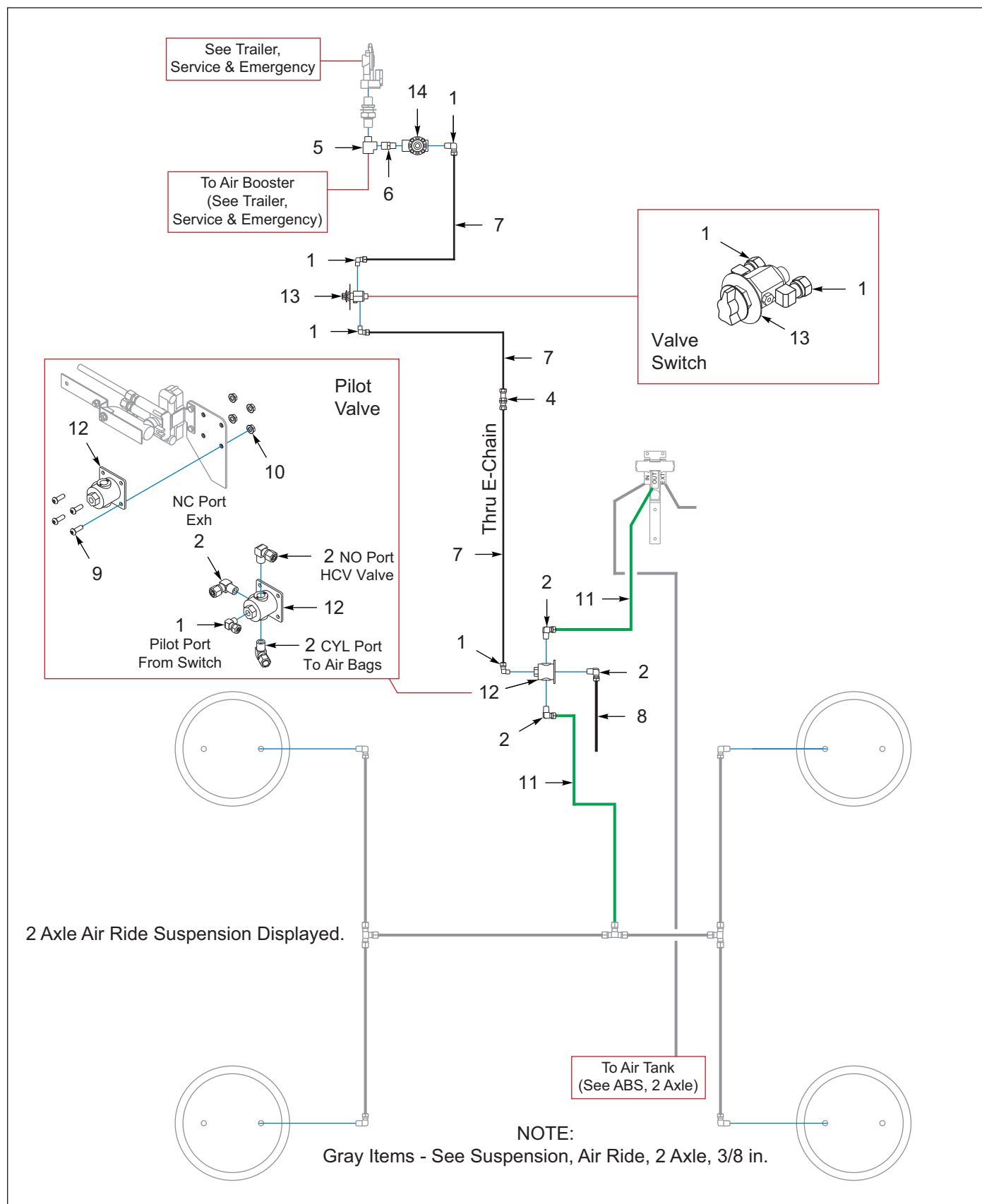
Figure 8-55: Suspension, Air Dump, 2 Axle, 3/8 in (Option) (After 06/14/2023)
