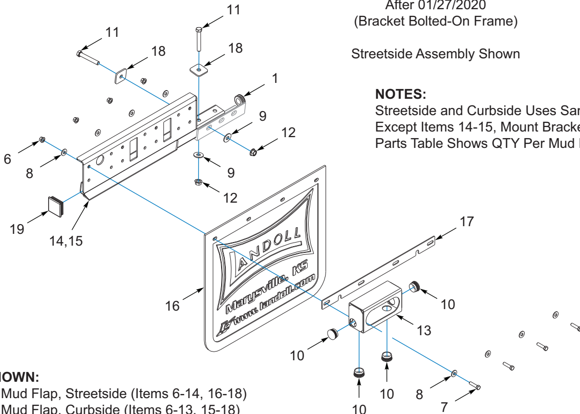
Figure 2-28: Mud Flaps, Rear, 2 Axle Spread, 3 Axle
