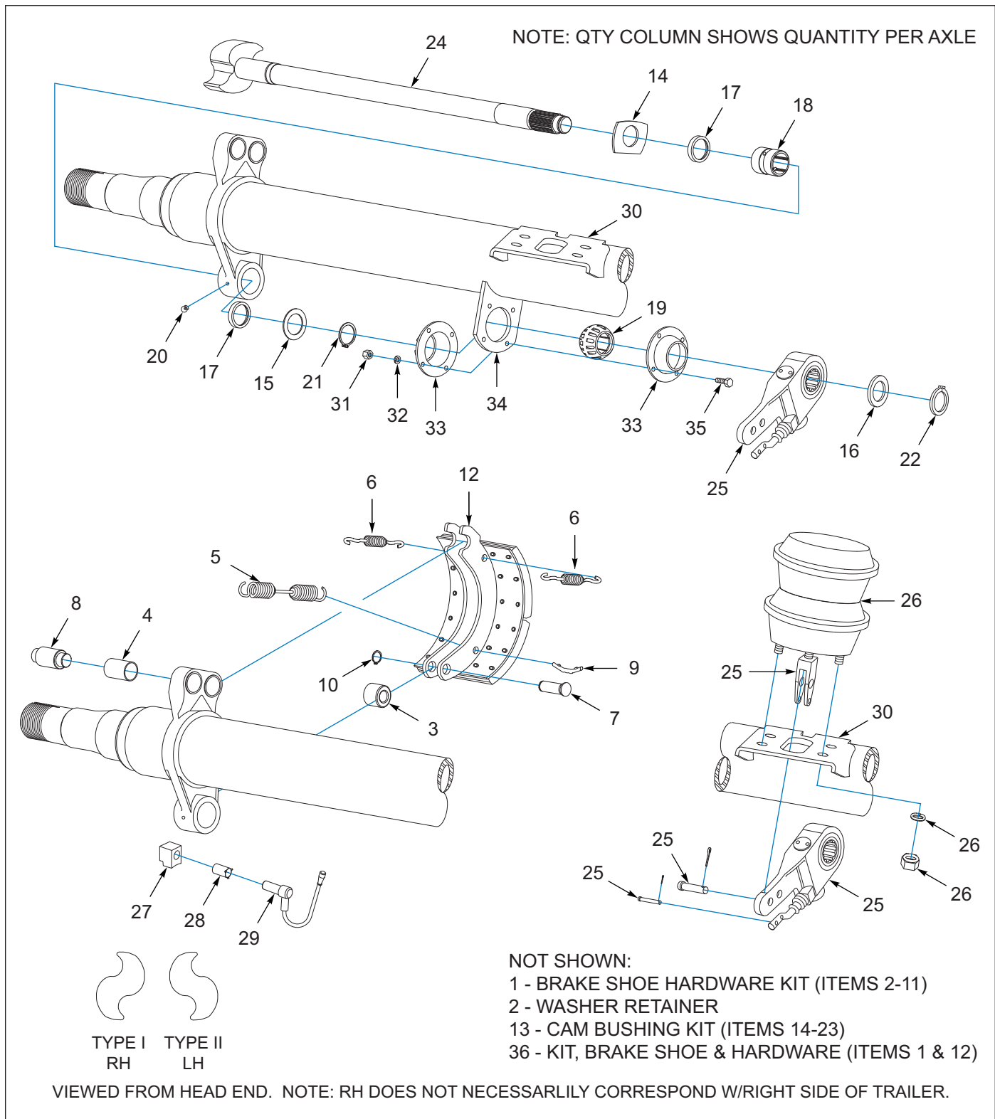
Figure 3-1: Axle 12.25 x 7.50 Drum Brake Components
