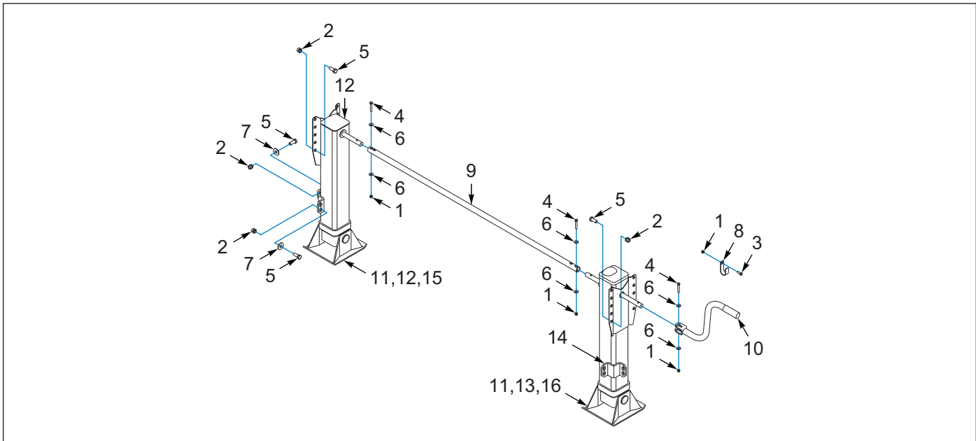
Figure 2-21: Landing Legs, Gear, 2-Speed, Flip Crank, Front Interior Low Mt Bkt
