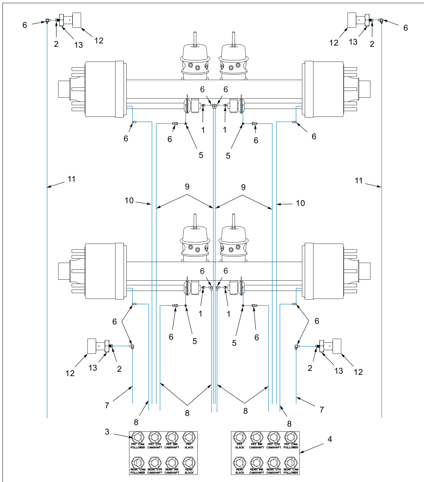
Figure 10-1: 2 Axle, Cam Followers, Drum Brakes (Before 11/07/2018)
