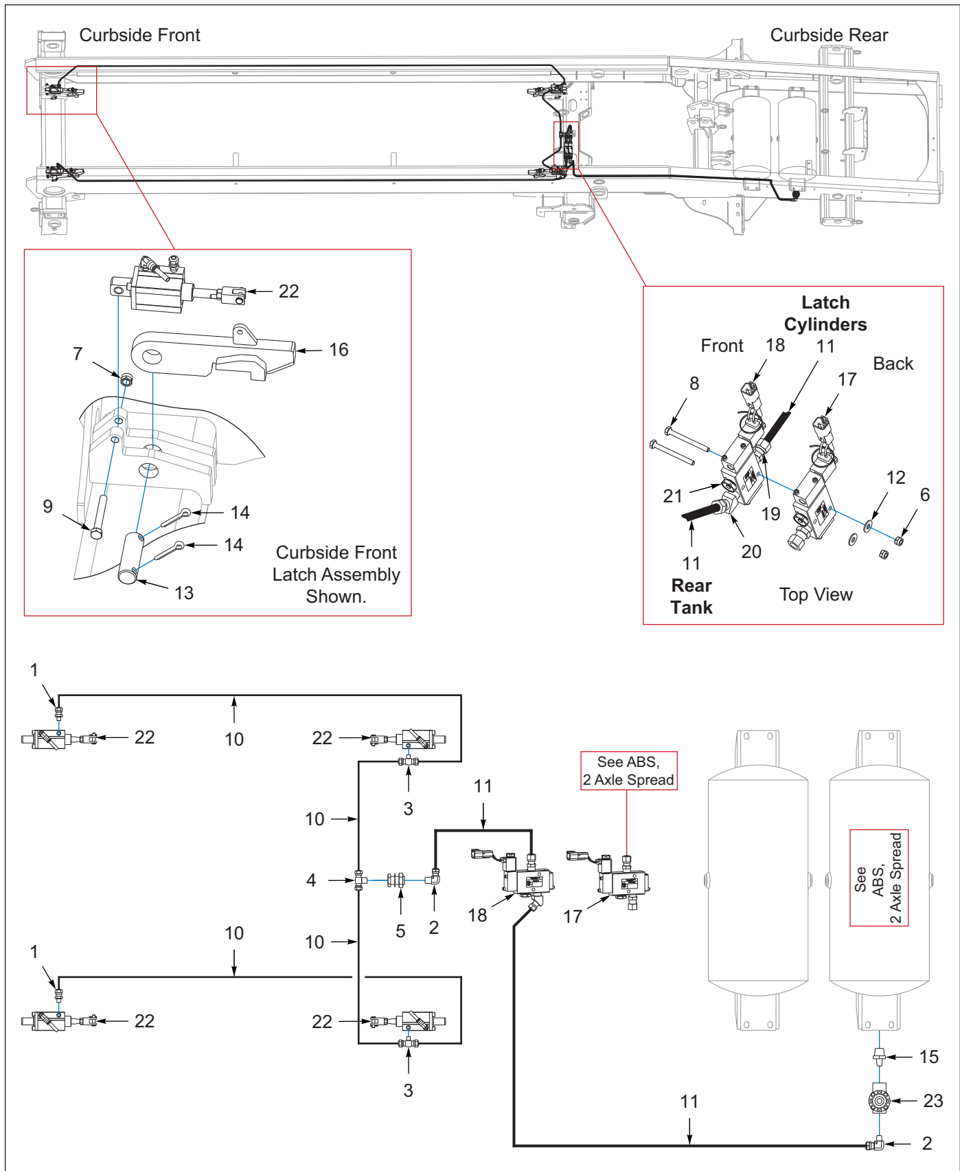
Figure 8-34: Latch Lock, 2 Axle Spread (Option)
