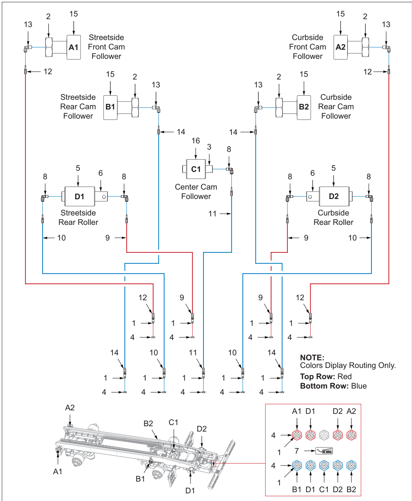
Figure 10-5: 2 Axle Spread, Cam Followers, Rollers (Option)
