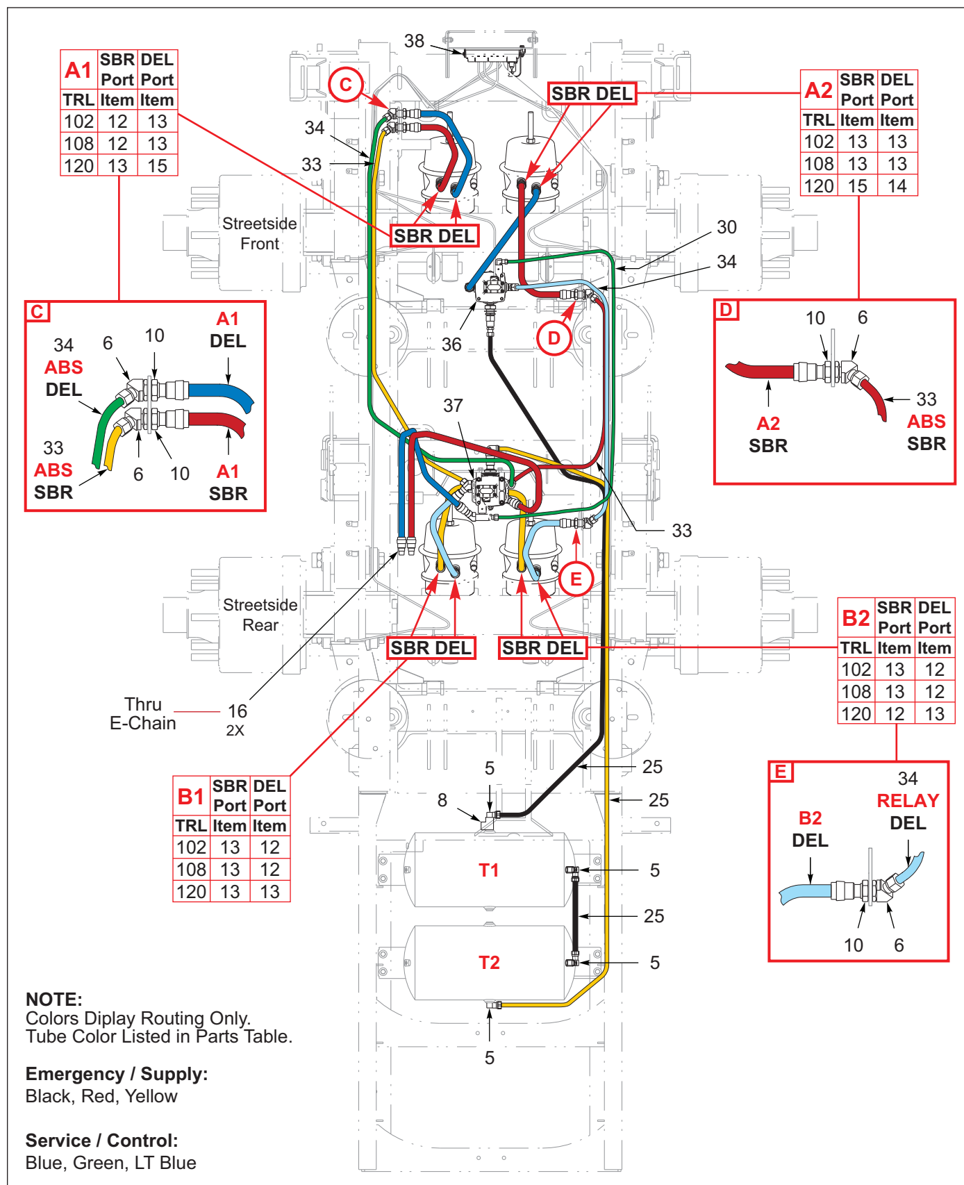
Figure 8-6: ABS, 2 Axle, Drum, Haldex (1 of 2)
