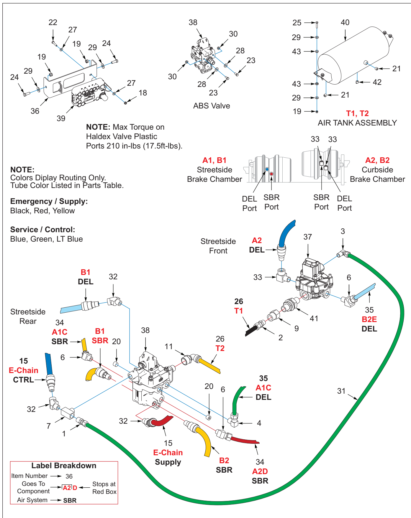
Figure 8-4: ABS, 2 Axle, Disc, Haldex (Option) (2 of 2)
