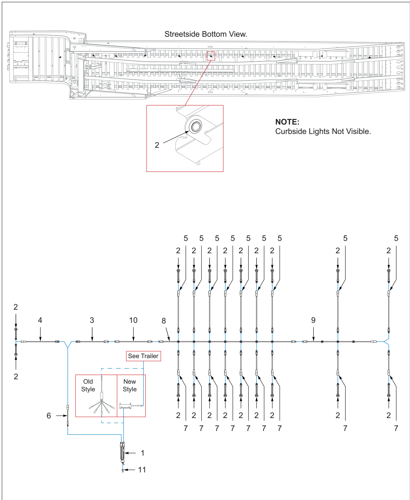
Figure 9-32: Lights, Work Zone, Under Deck (Option) (After 01/19/2024)
