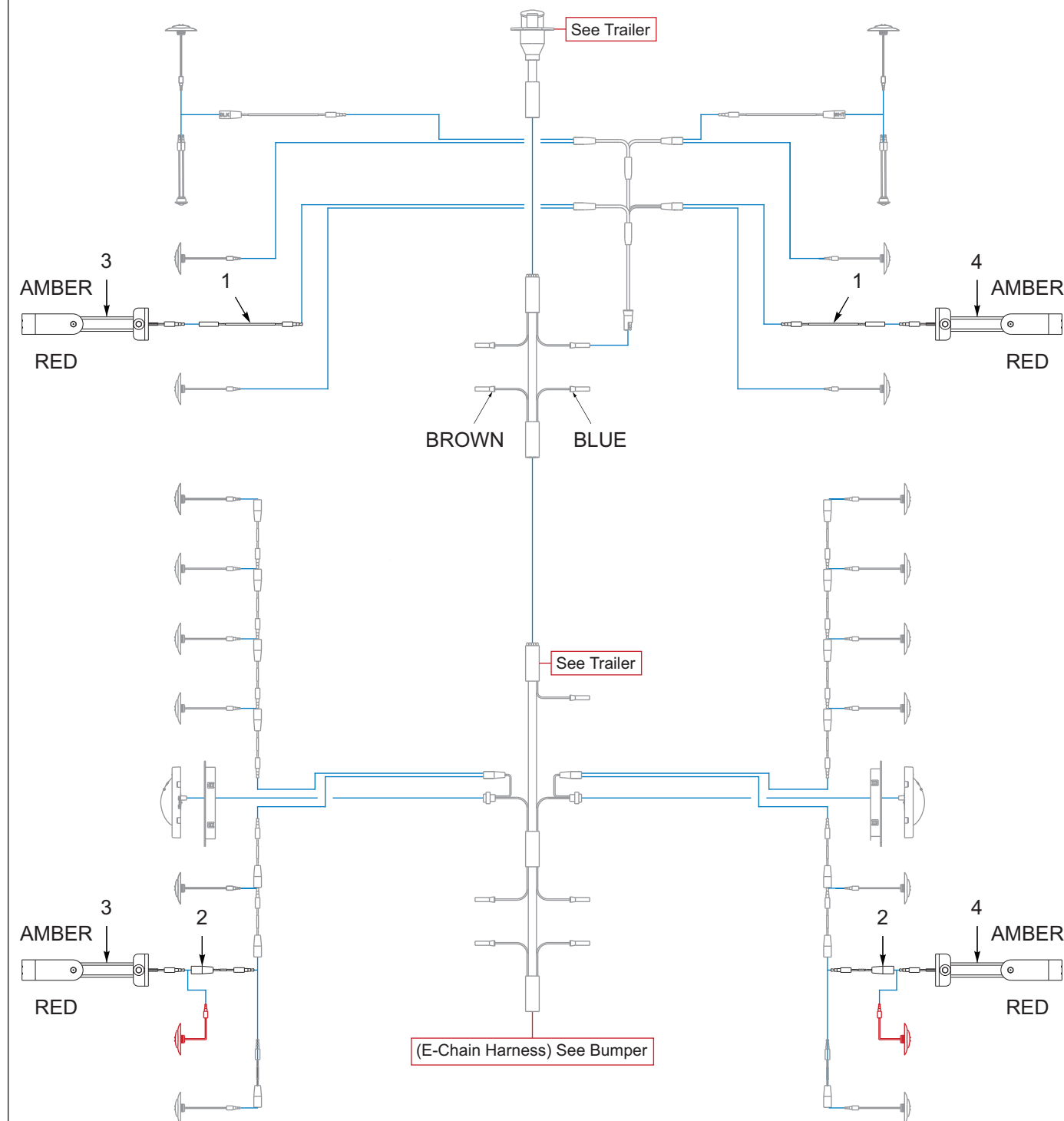
Figure 9-24: Lights, Swing Arm, Marker, Amber & Red (Options) (1 of 2)
