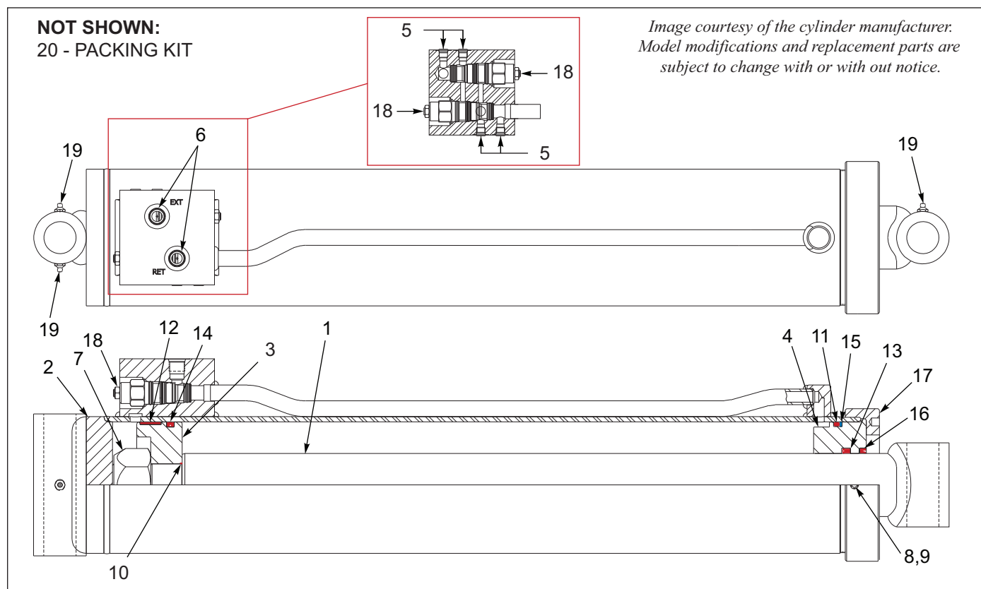
Figure 11-18: Cylinder Components, 6 x 30
