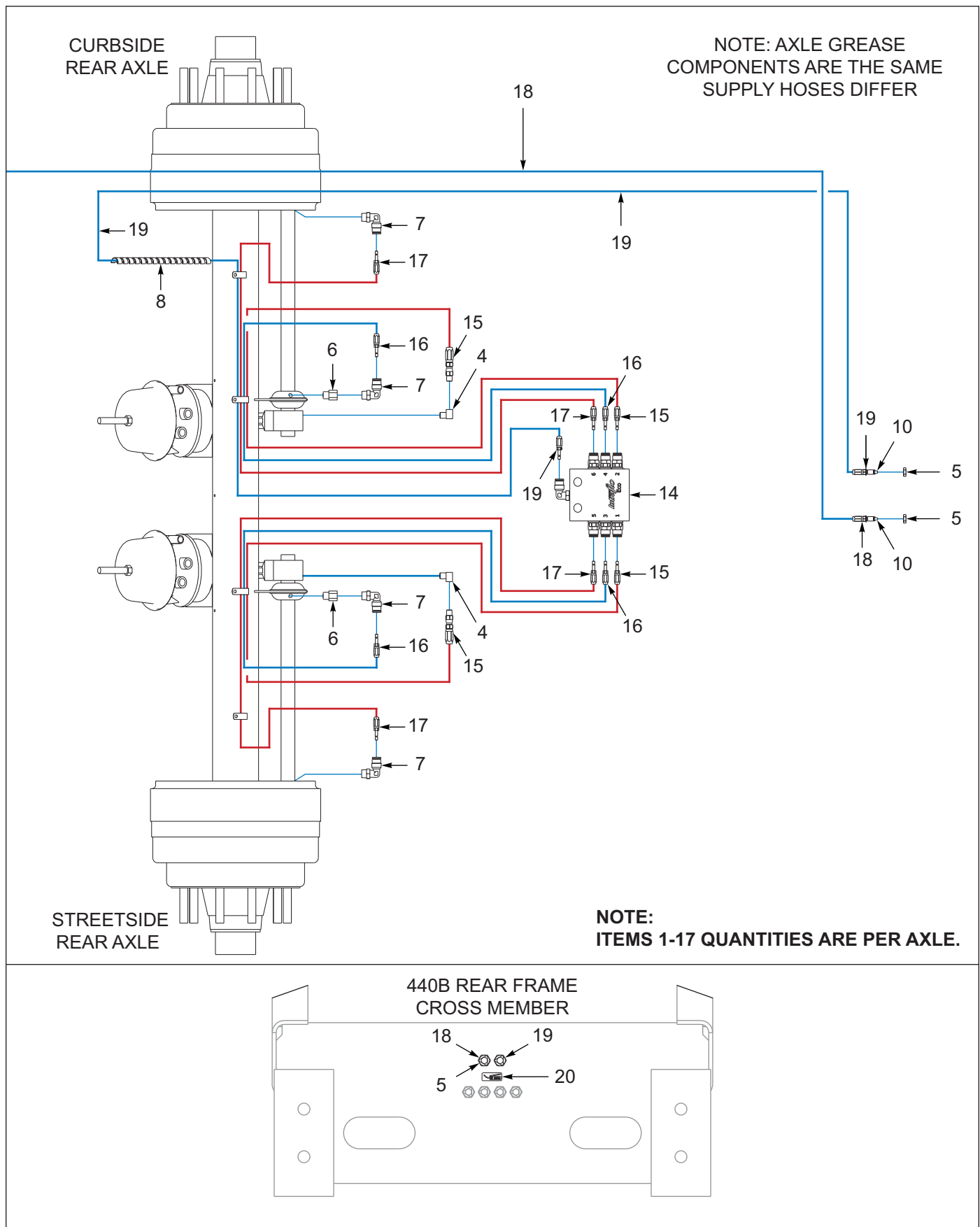
Figure 10-10: 2 Axle, Drum Brakes (After 09/01/2024) (2 of 3)
