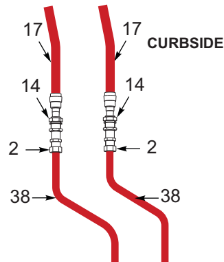
Figure 8-31: ABS, 3 Axle, Drum, Aqua (Option) (After 06/12/2023) (1 of 3)
