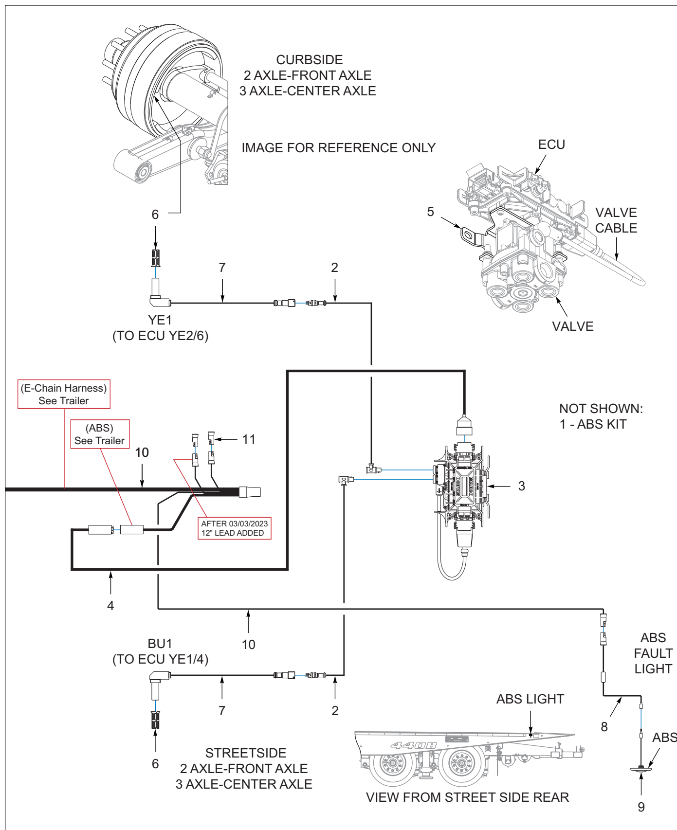
Figure 9-7: ABS, Wabco, Aqua (1 of 2)
