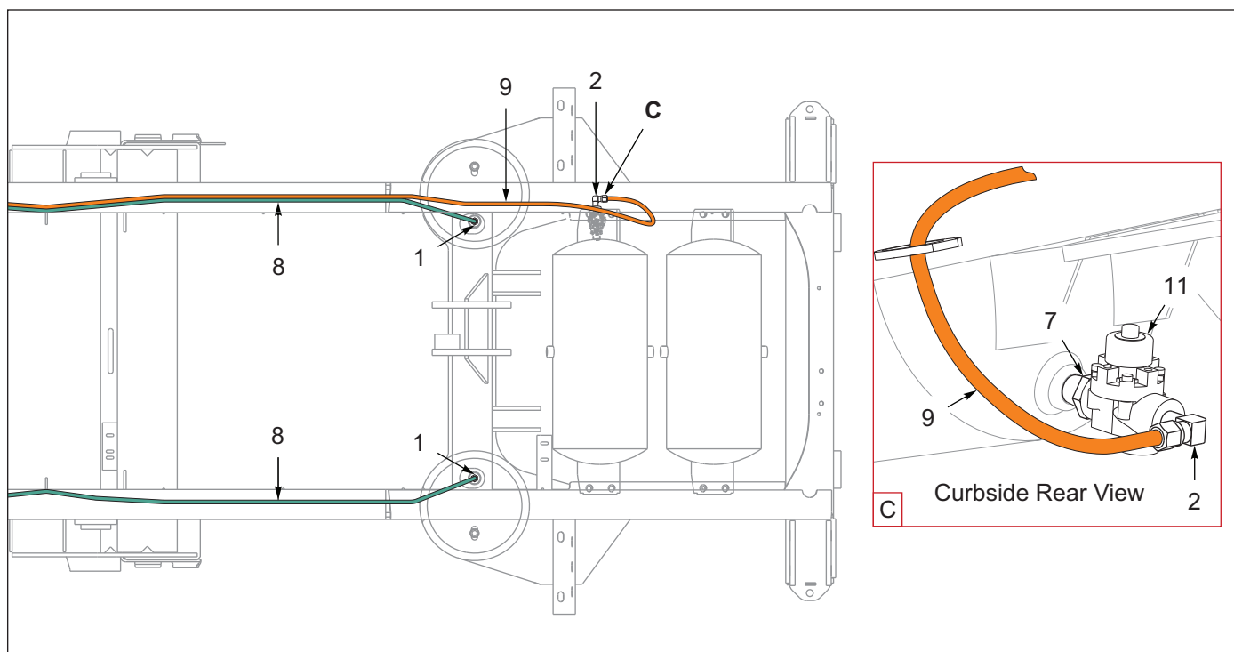
Figure 8-47: Suspension, Air Ride, 3 Ax, 3/8 in (After 03/10/2023) (2 of 2)
