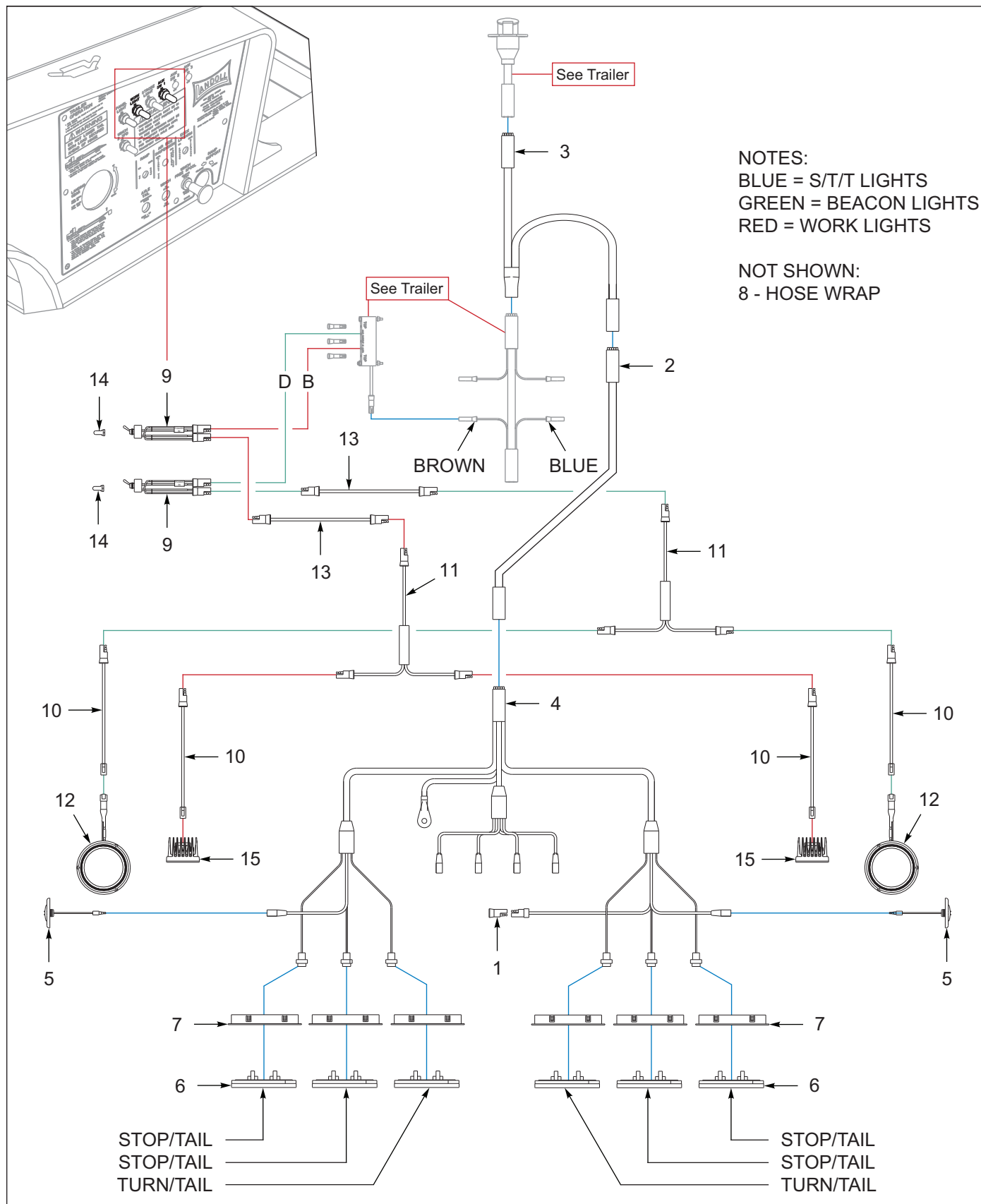
Figure 9-20: Light Bar, Bulkhead (Options)
