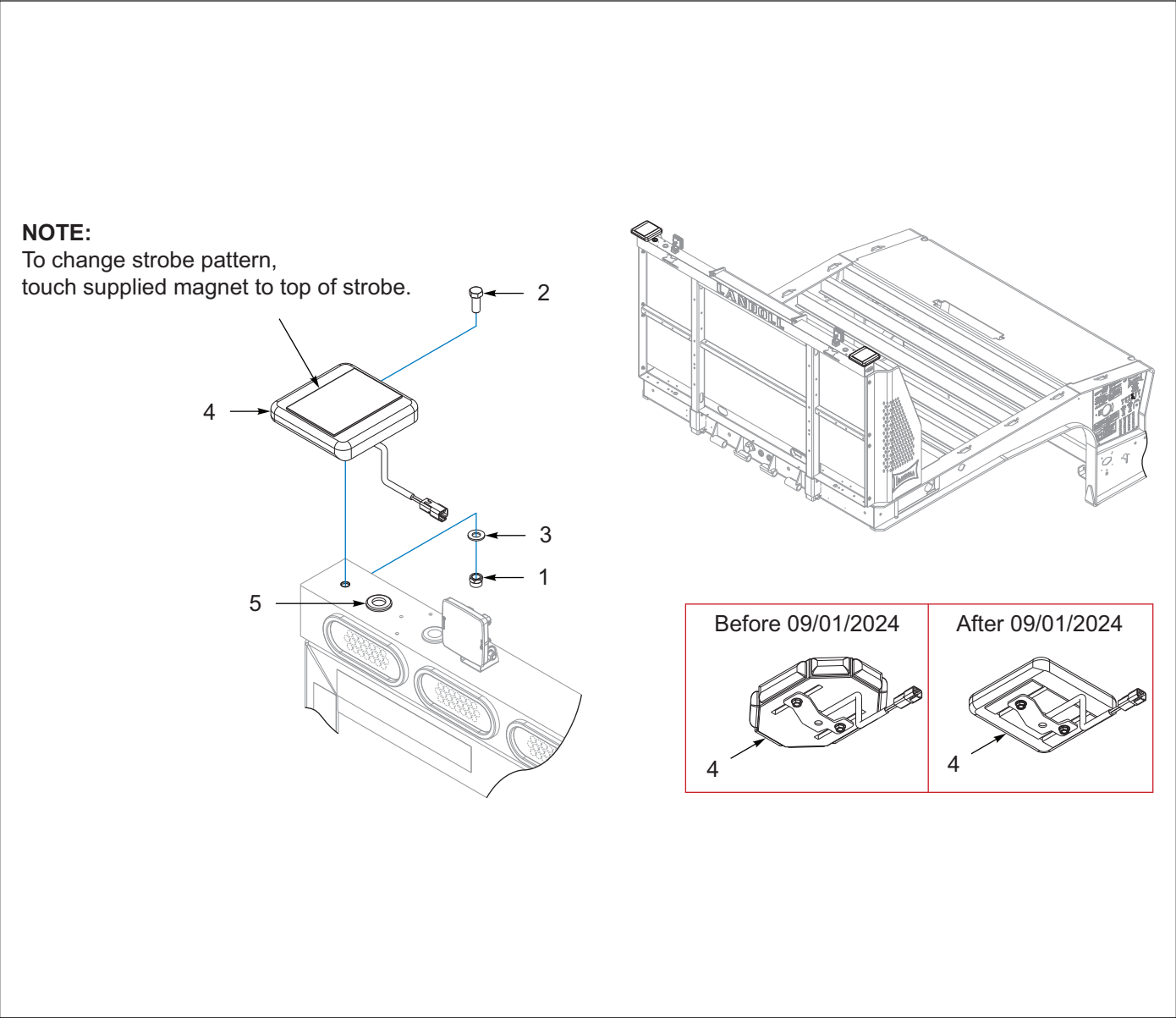
Figure 4-6: Bulkhead, Lights, Strobe, 360 Degree, Amber
