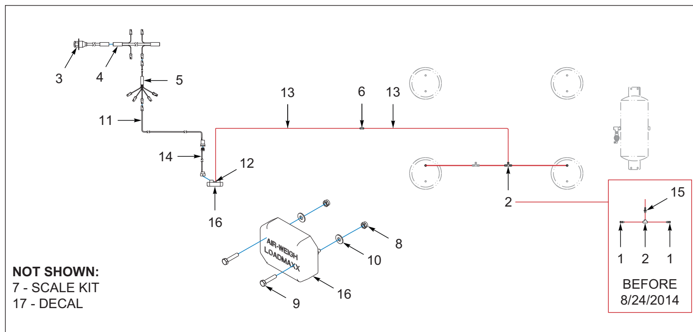
Figure 8-37: Scale, Quickload (Option) (Before 03/31/2020)
