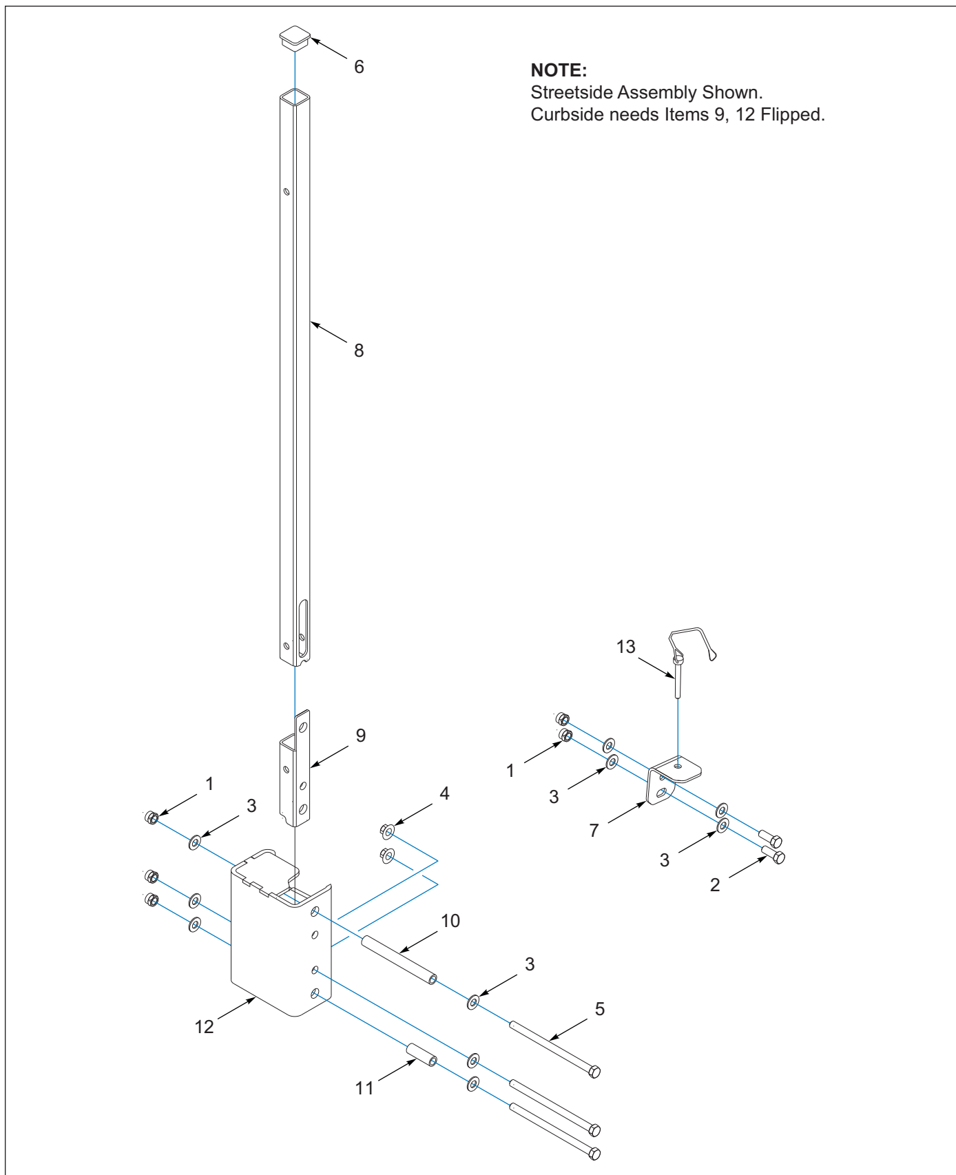
Figure 4-14: Step Handle, Folding
