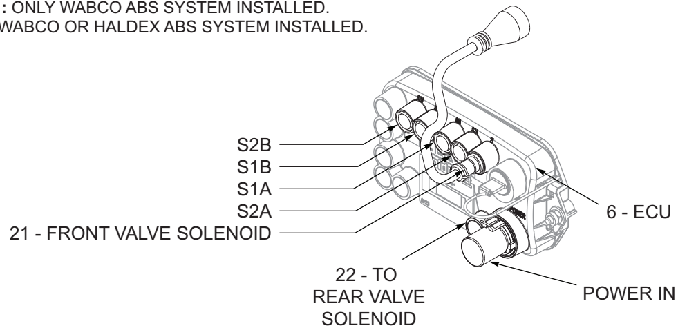
Figure 9-14: ABS, Haldex, 3 Axle (2 of 2)
