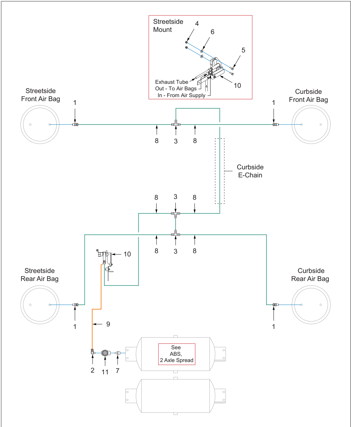
Figure 8-44: Suspension, Air Ride, 2 Ax Spread (Option)
