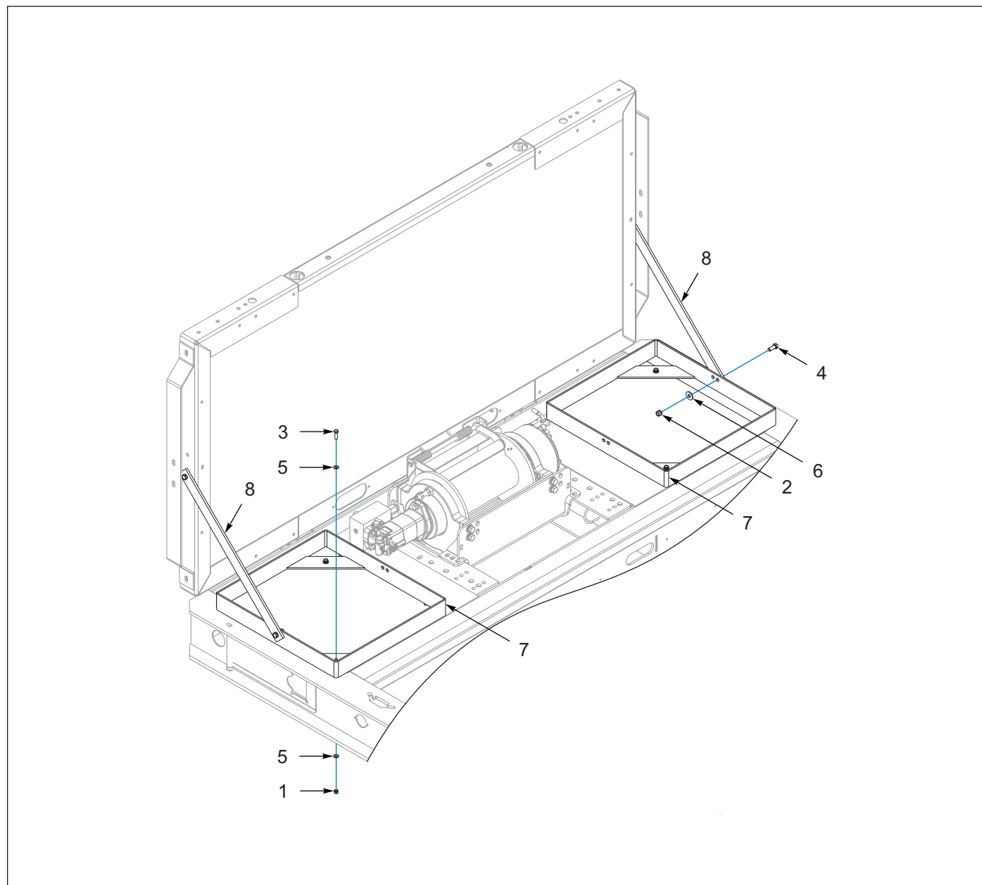
Figure 4-10: Chain Tray, Bulkhead / Upper Deck, Bolt-On
