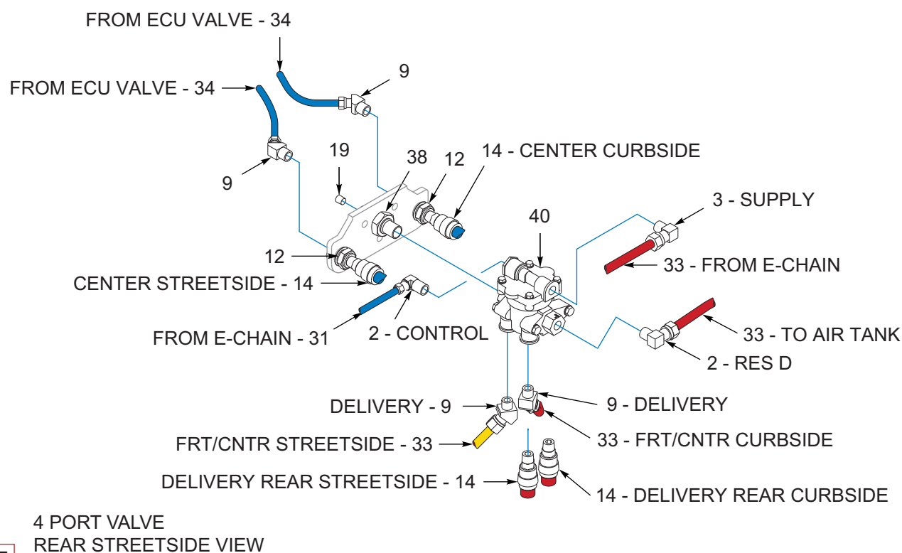
Figure 8-24: ABS, 3 Axle, Drum, Wabco (10/06/2023 To 12/01/2025) (3 of 3)
