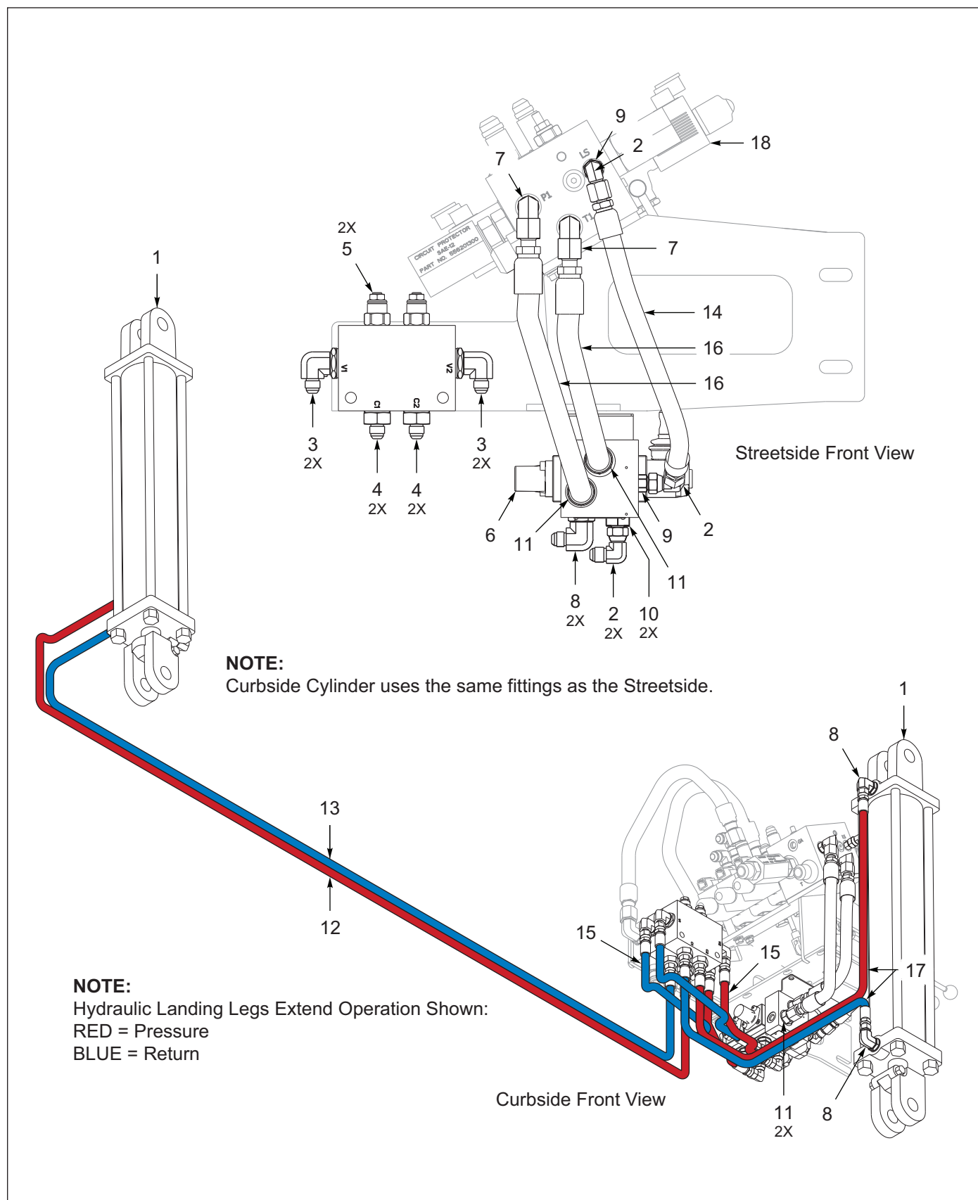
Figure 11-5: Landing Legs, Hydraulic (Option)
