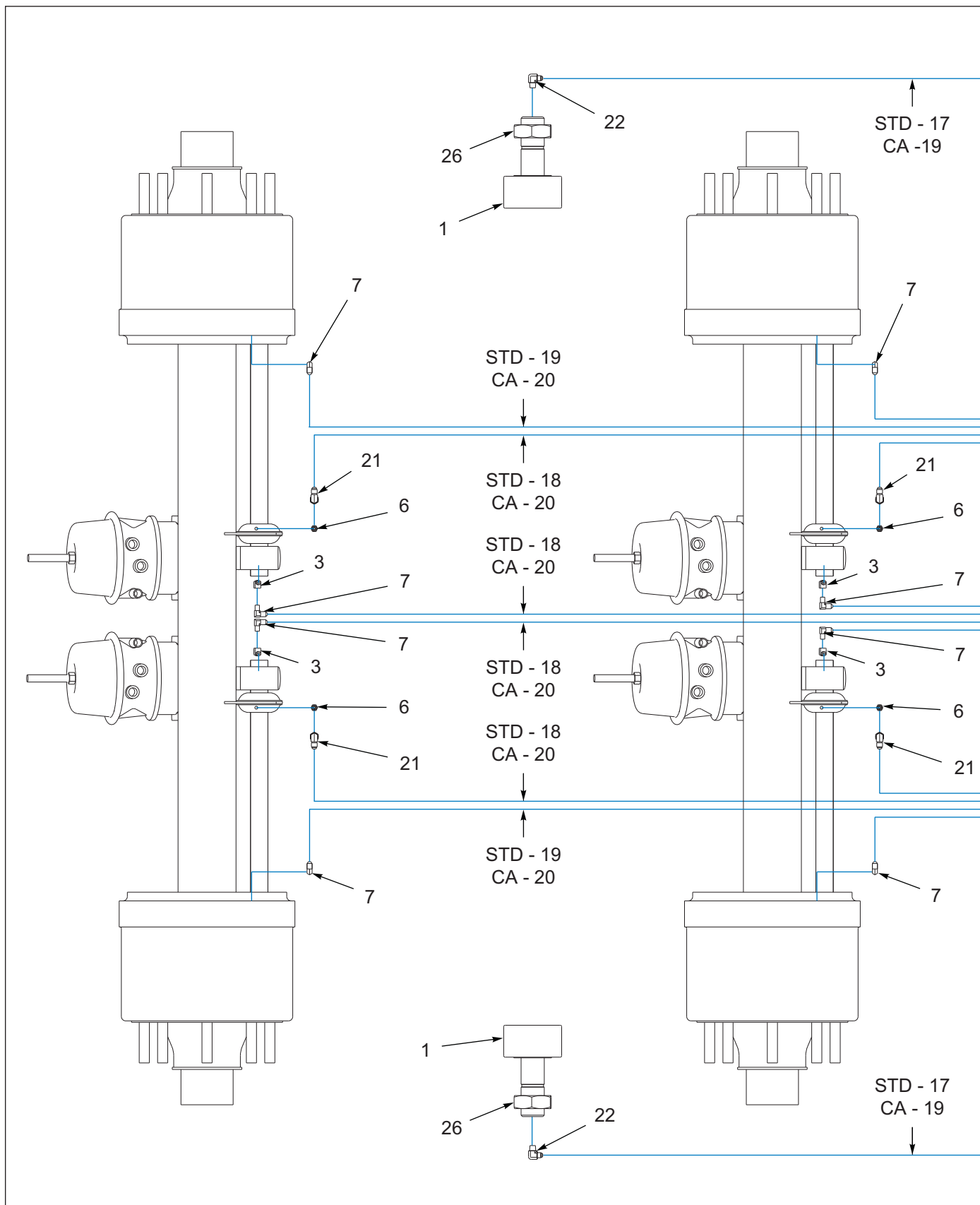
Figure 10-17: 3 Axle, Cam Followers, Drum Brakes (11/07/2018 To 08/31/2020) (1 of 2)
