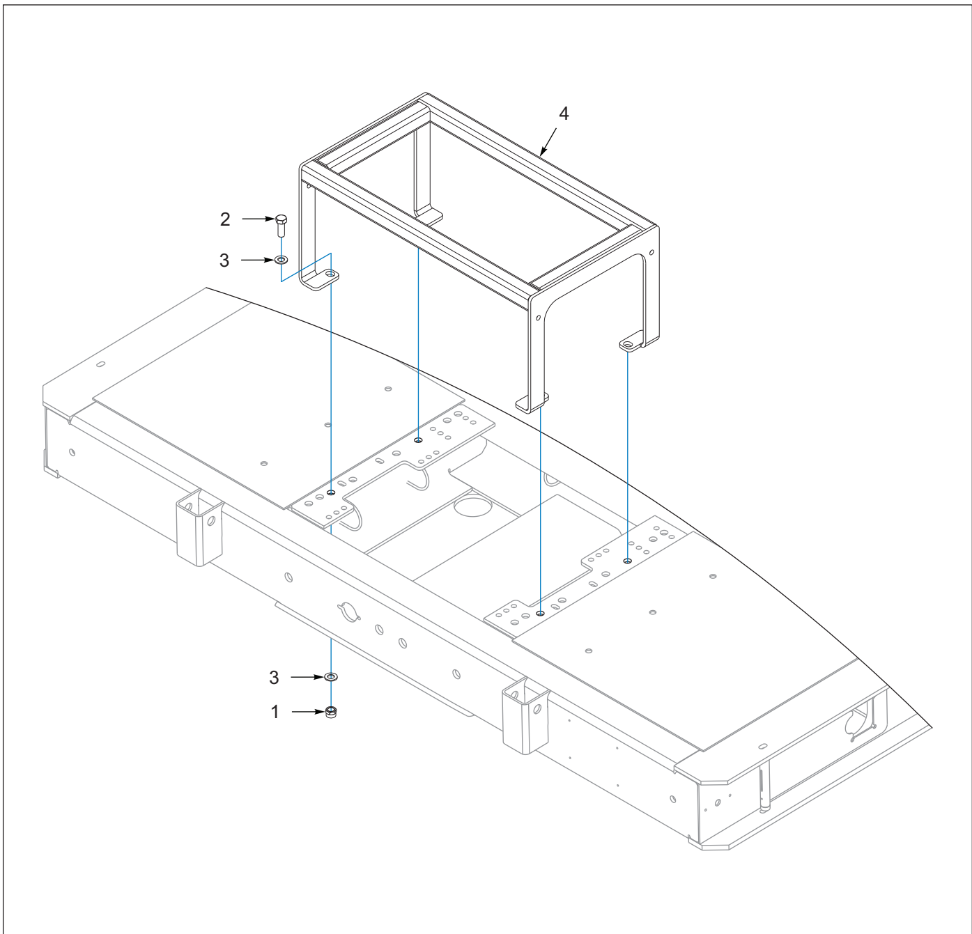
Figure 7-27: Guard, Winch, W/ Cable Pivot Guide
