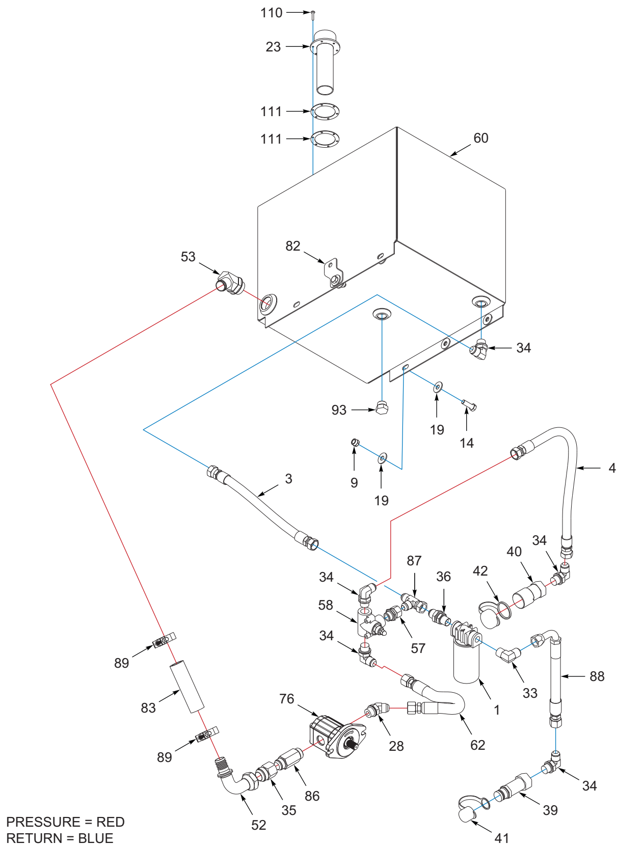
Figure 6-5: Engine, 25HP, Upper Deck Assembly (5 of 5)
