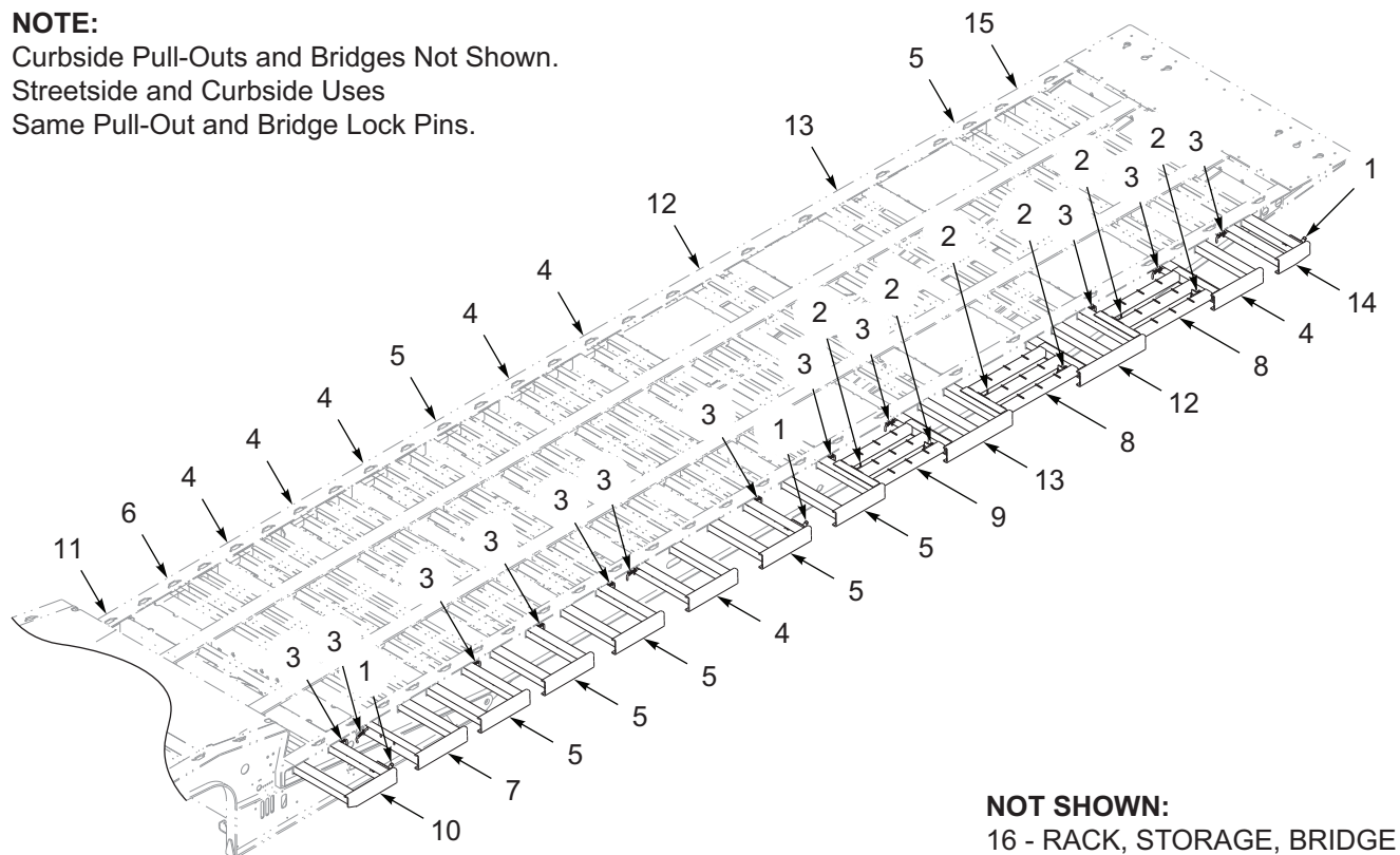
Figure 5-9: Pull-Out / Bridge, 3 Axle, 50 Foot, CA
