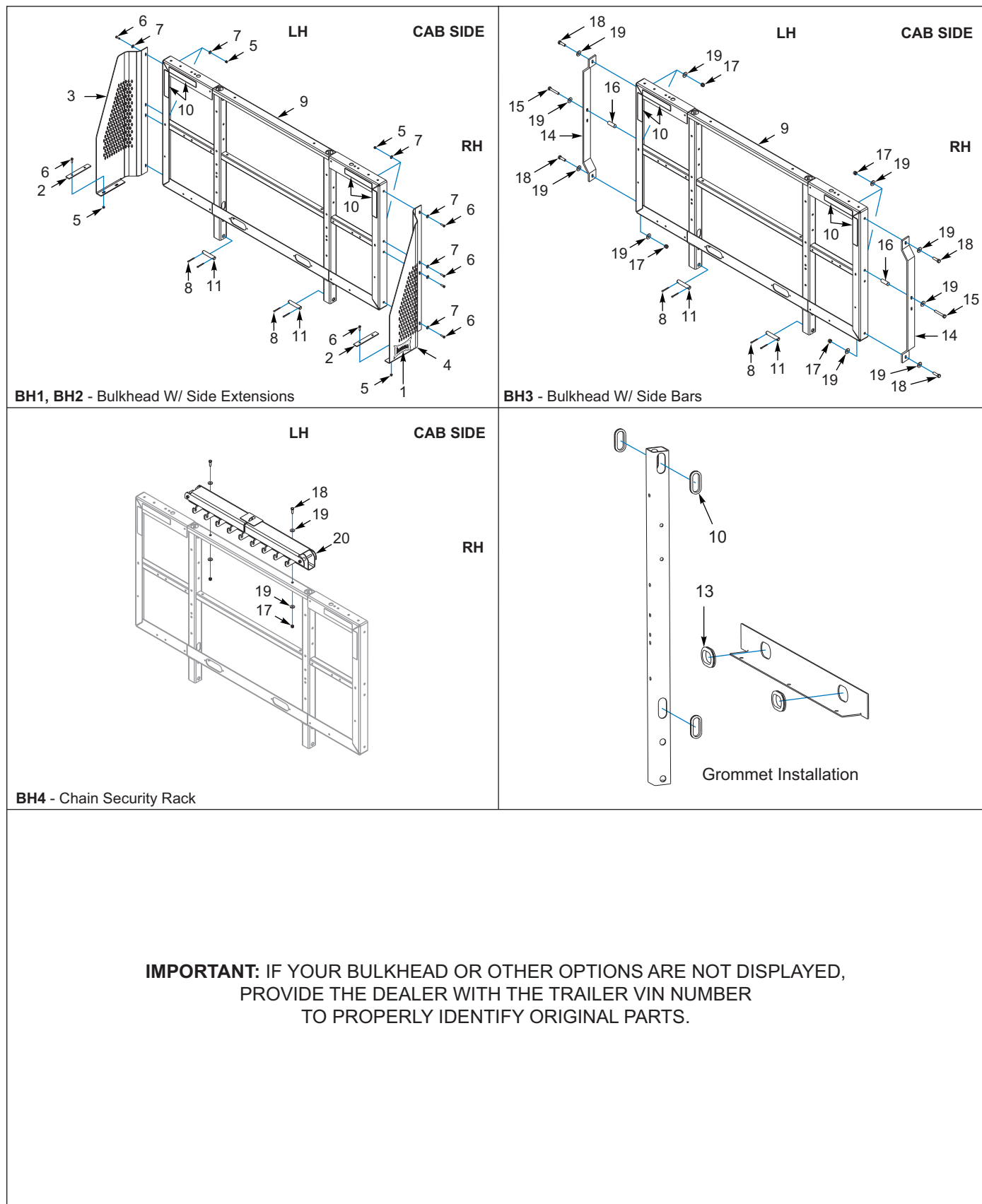
Figure 4-2: Bulkhead Components, 48 x 102
