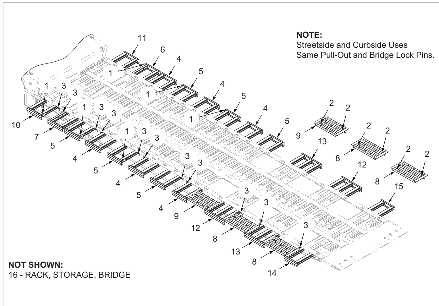
Figure 5-7: Pull-Out / Bridge, 3 Axle, 48 Foot
