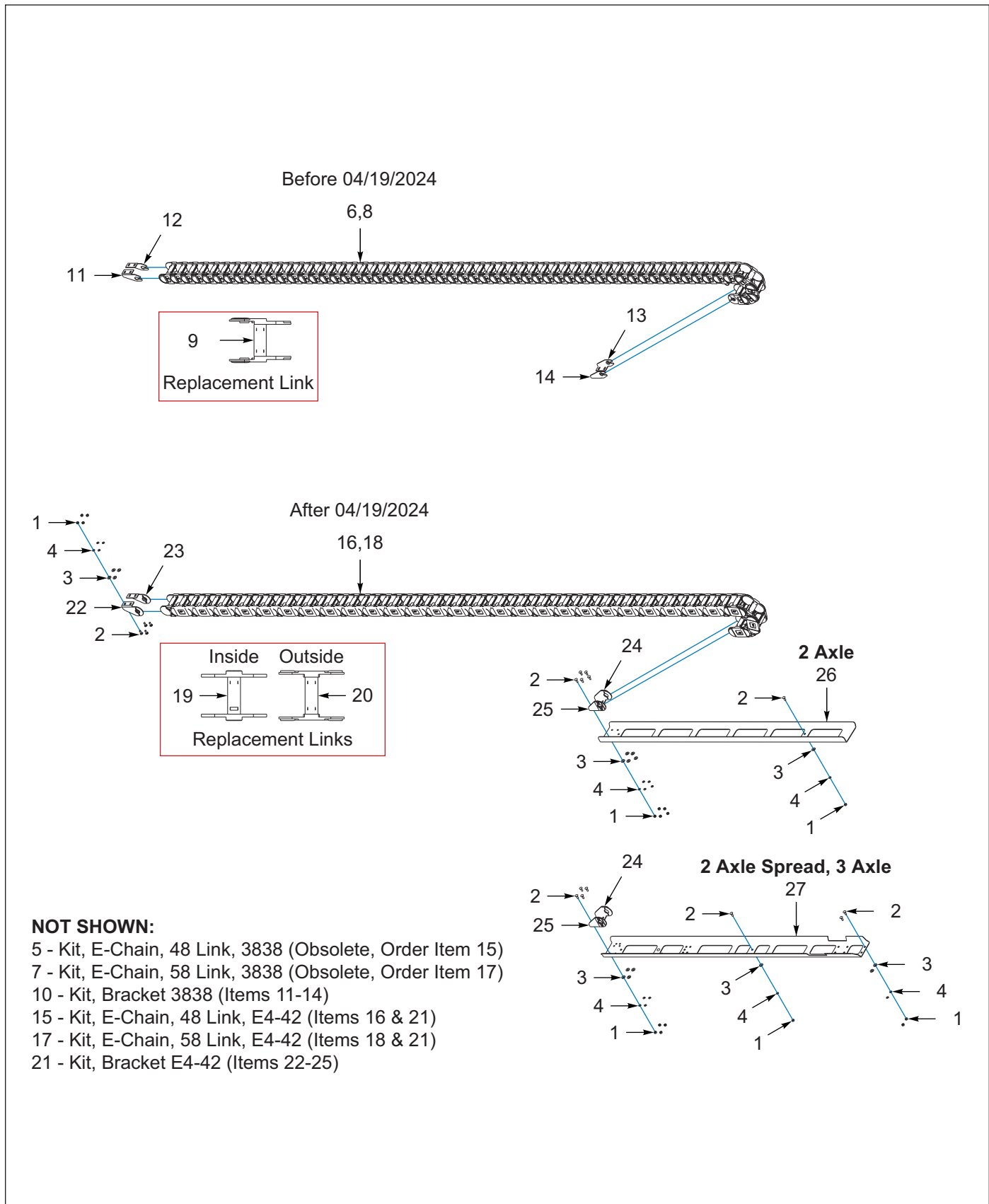
Figure 2-11: E-Chain & E-Chain Tray, Undercarriage
