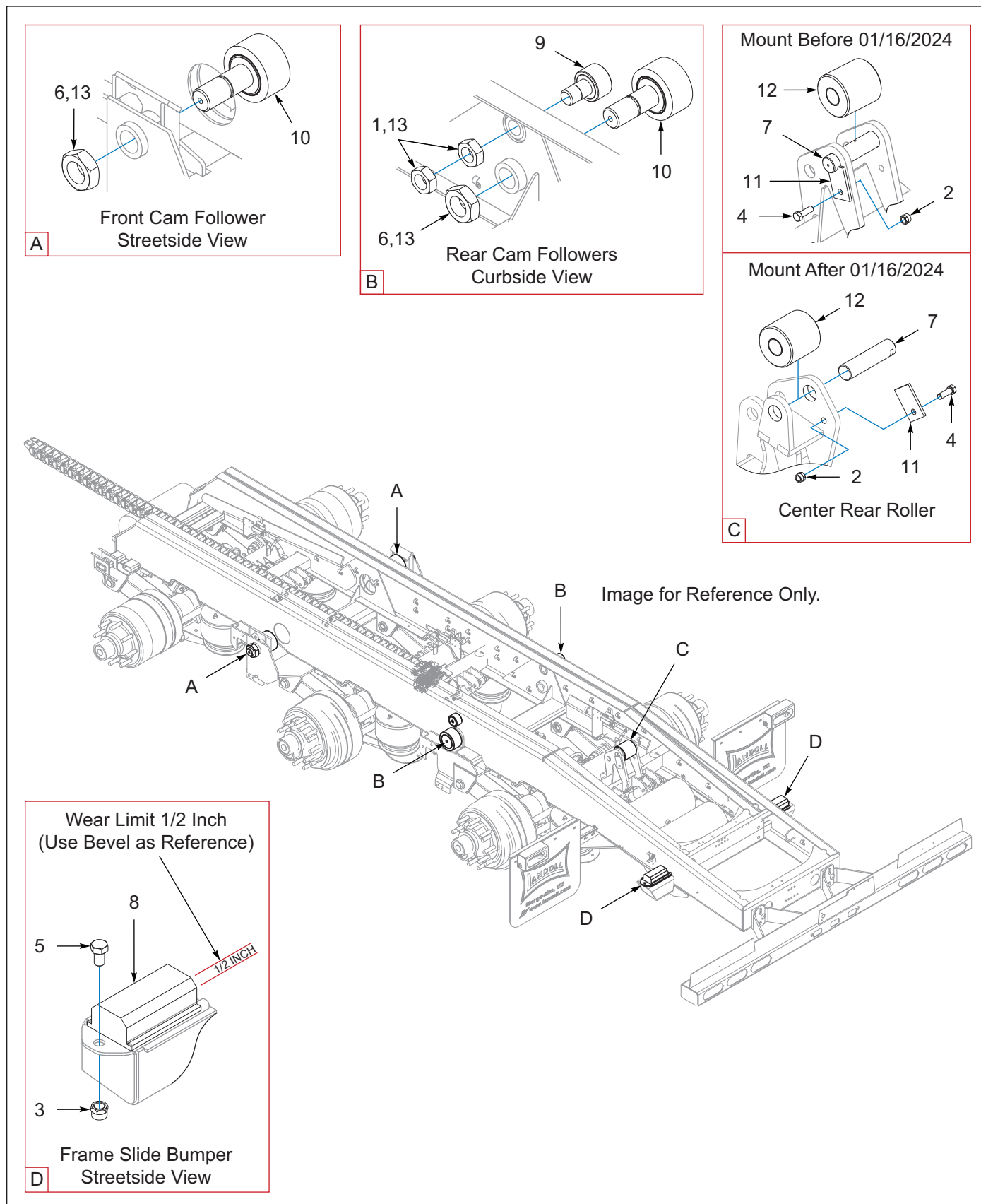
Figure 2-9: Cam Follower, Rear Roller, Slide Bumpers, 3 Axle
