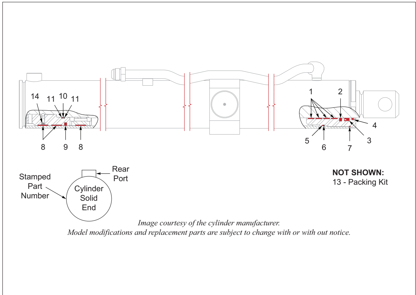
Figure 11-15: Cylinder Components, 4 x 100, 126, 135, Hi-Flow, Dantal
