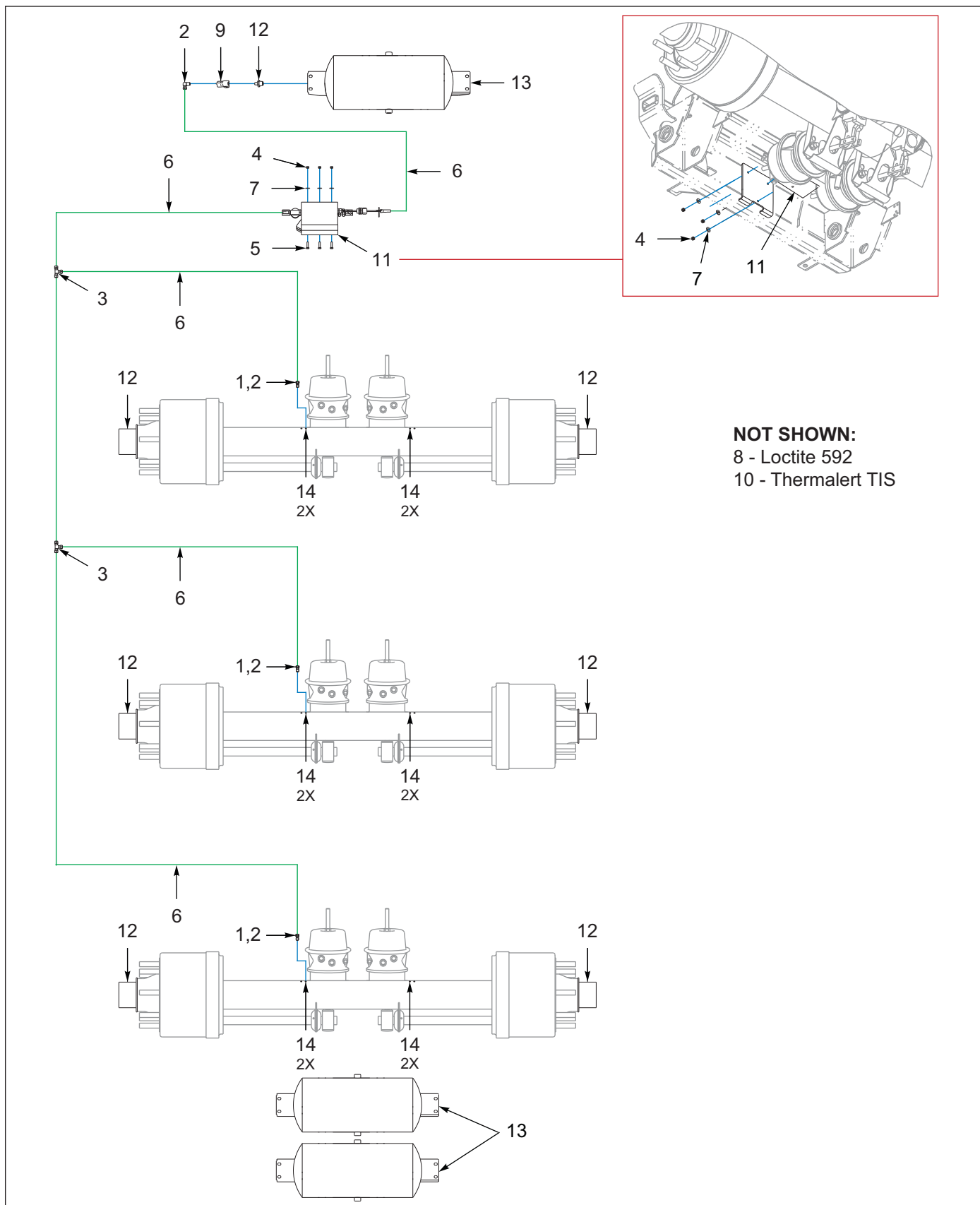
Figure 8-59: Tire Inflation, 3 Axle (Option)
