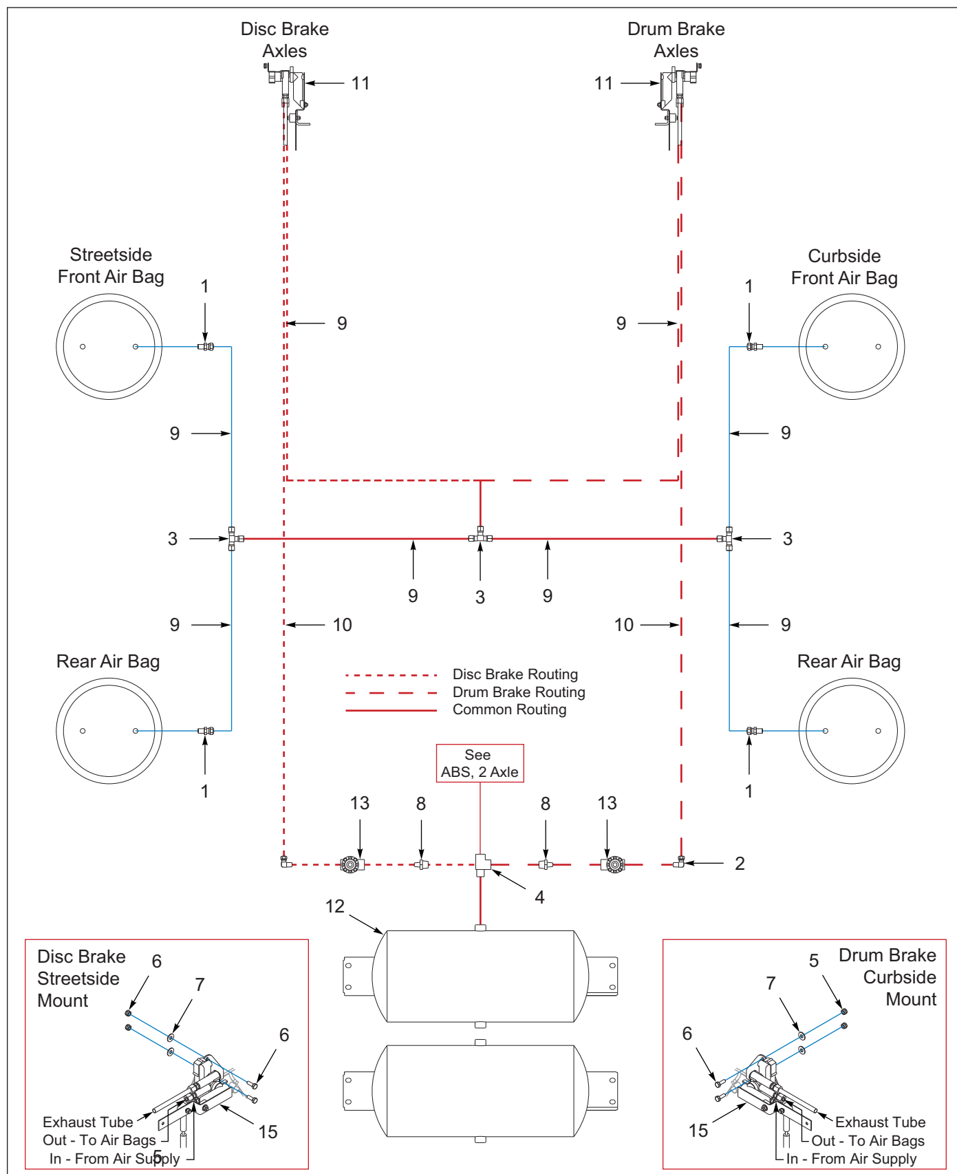
Figure 8-41: Suspension, Air Ride, 2 Ax, 3/8 in (After 06/14/2023 to 09/01/2024)
