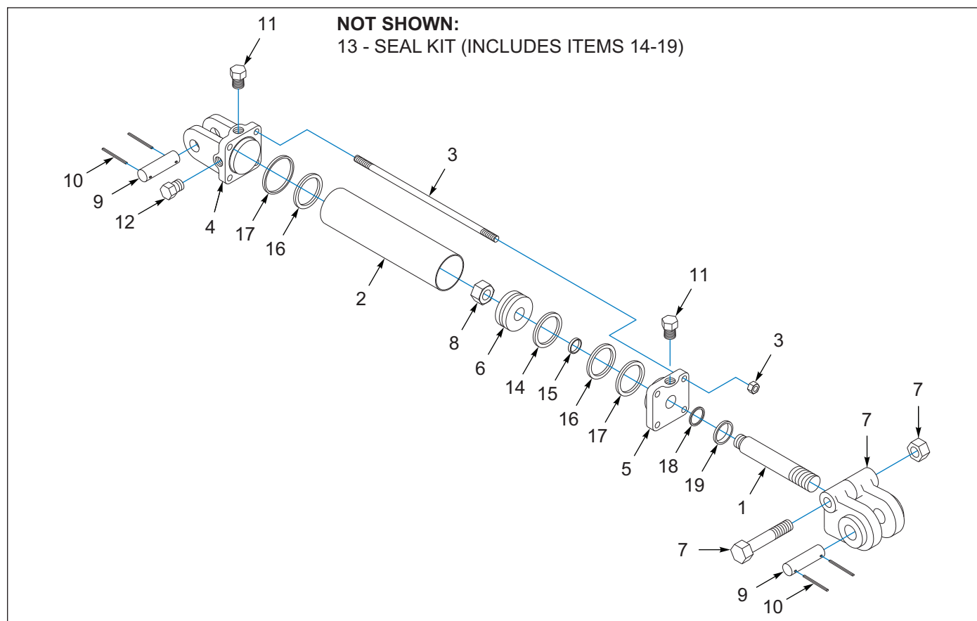
Figure 11-12: Cylinder Components, 3-1/2 x 20 (Option)
