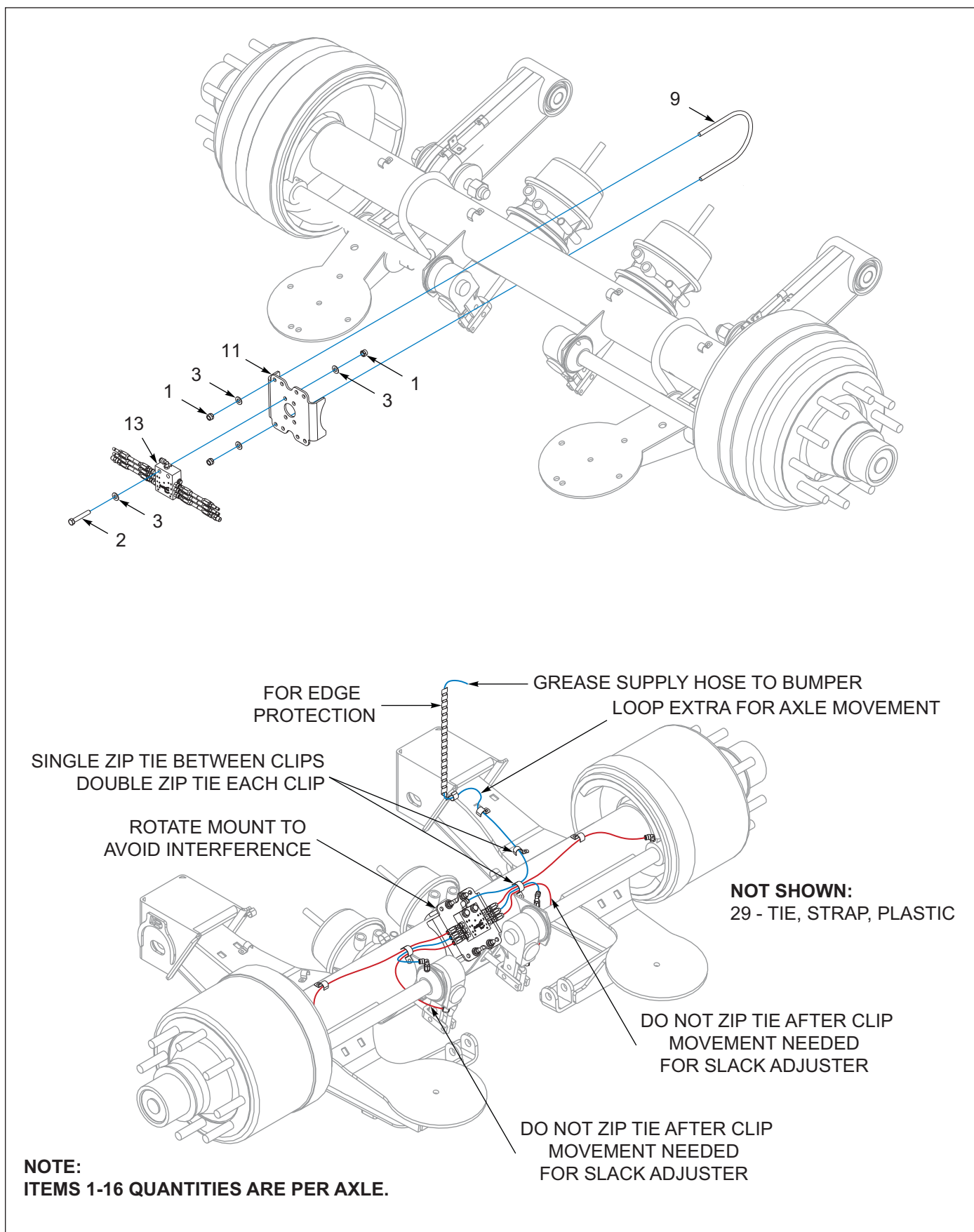
Figure 10-21: 3 Axle, Cam Followers, Drum Brakes (08/31/2020 To 12/01/2025) (3 of 3)
