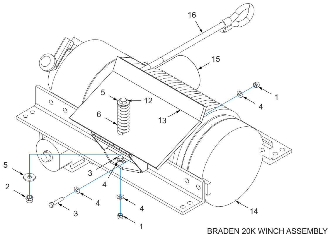
Figure 7-9: Winch Assembly, Braden 12K / 20K, 1-Speed
