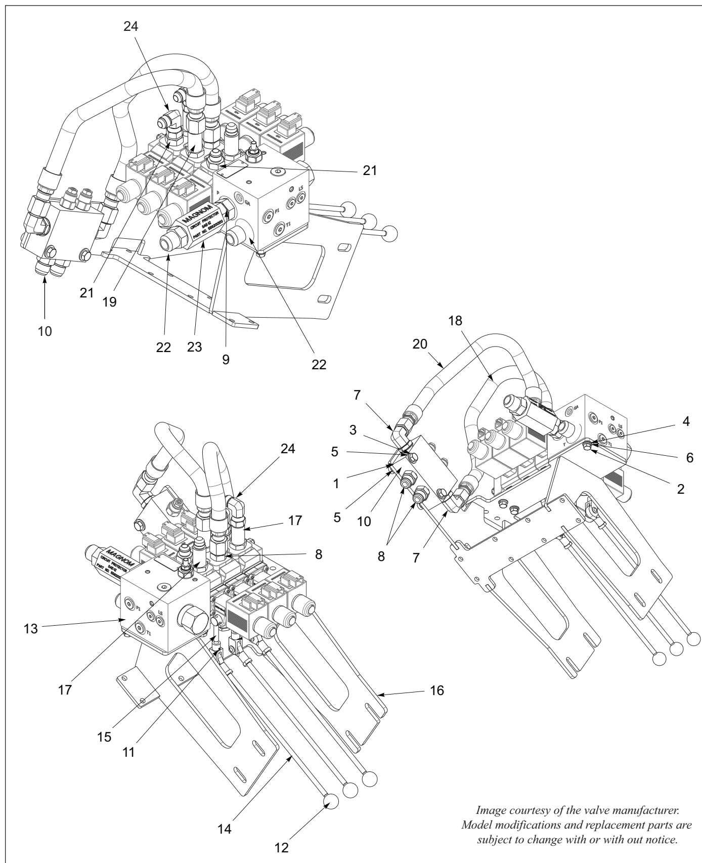
Figure 11-20: Valve Assembly, 3-Spool Solenoid
