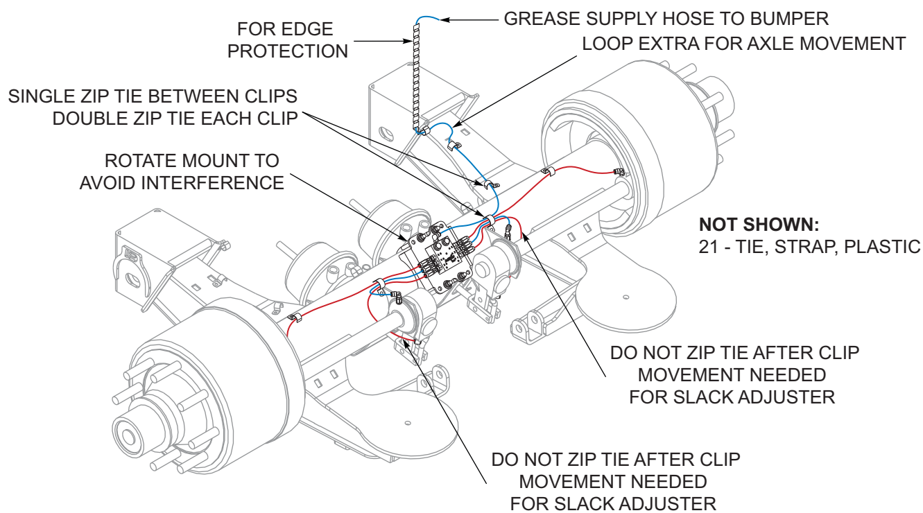
Figure 10-11: 2 Axle, Drum Brakes (After 09/01/2024) (3 of 3)
