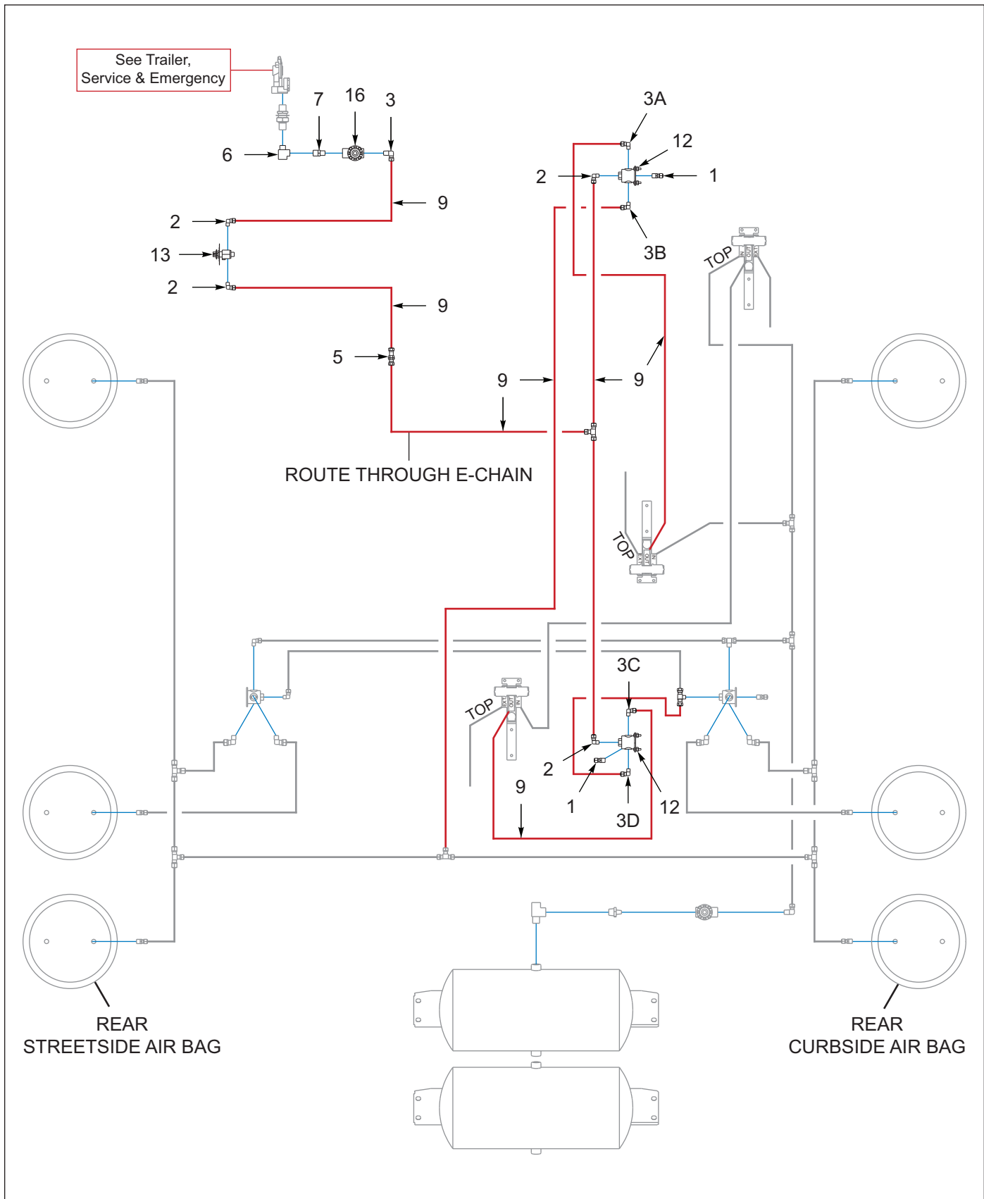
Figure 8-56: Suspension, Air Dump, 3 Axle, Double Pilot (Option) (1 of 2)
