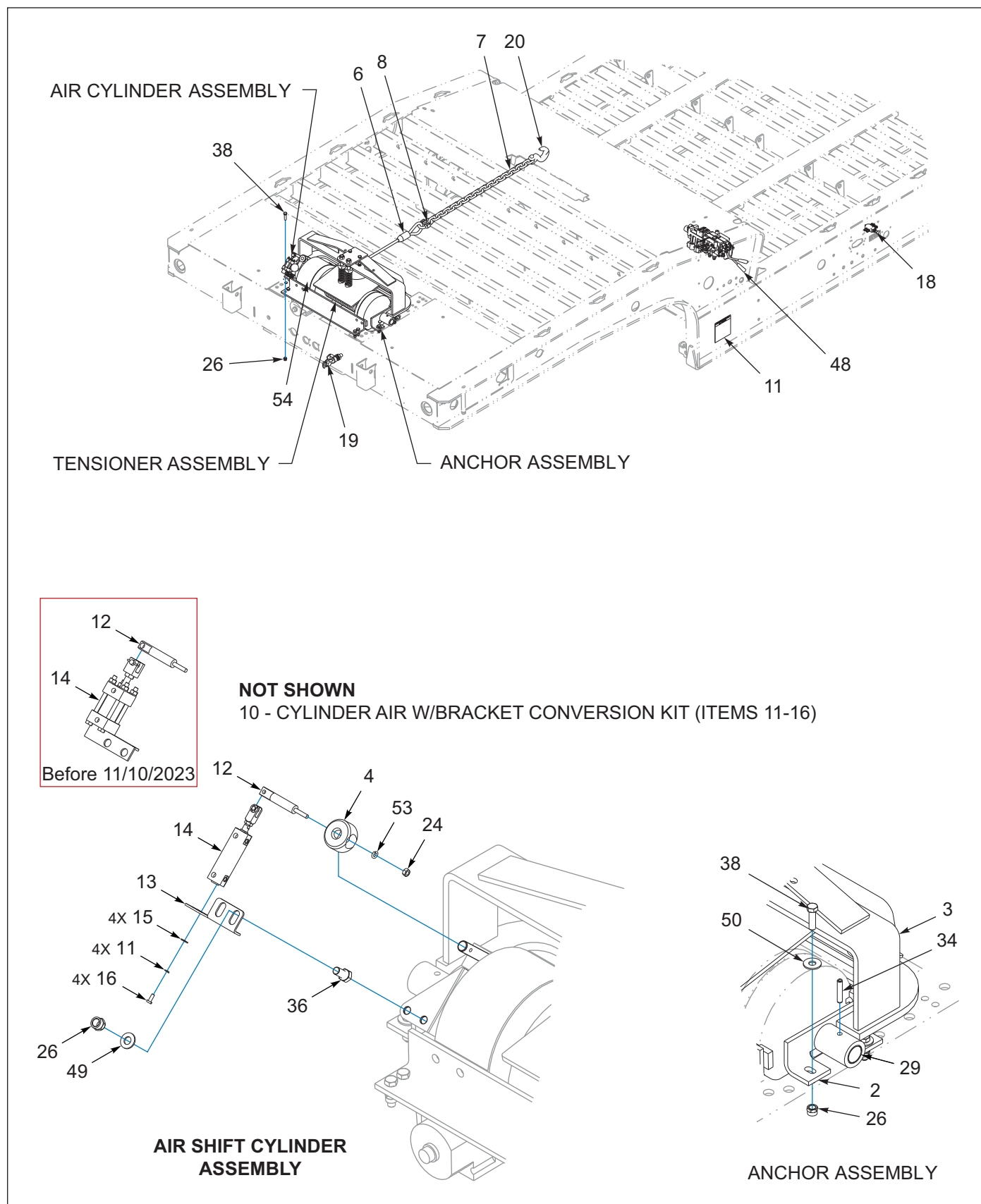
Figure 7-3: Winch Install, Braden 20K, 1-Speed, Air Tension (1 of 3)
