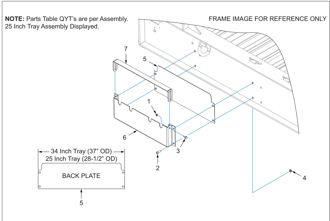
Figure 4-8: Chain Tray, Beam, Bolt-On (After 01/17/2022)
