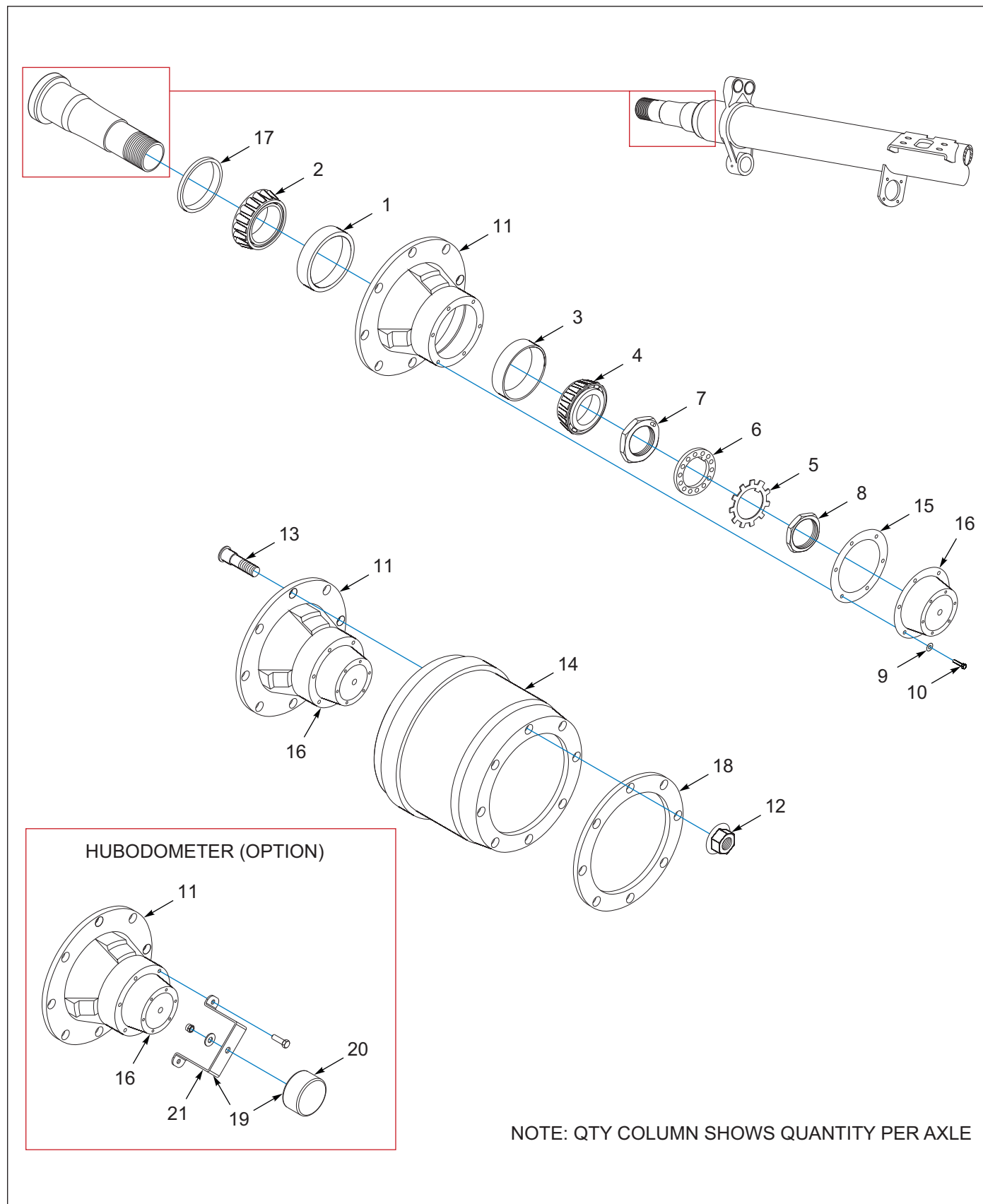
Figure 3-2: Axle 12.25 x 7.50 Drum &amp; Hub Components
