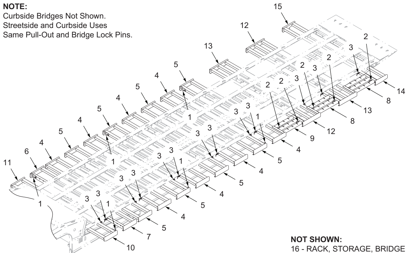
Figure 5-10: Pull-Out / Bridge, 3 Axle, 53 Foot
