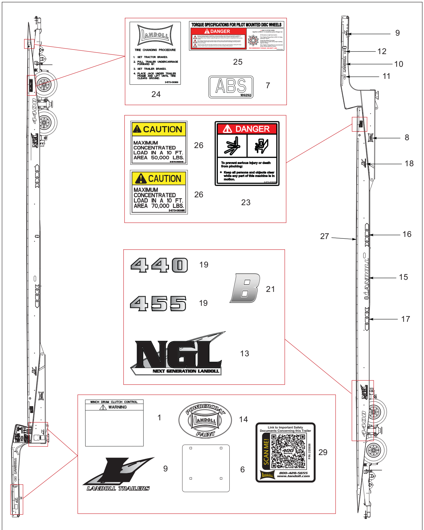
Figure 1-2: Frame Assembly (2 of 2)
