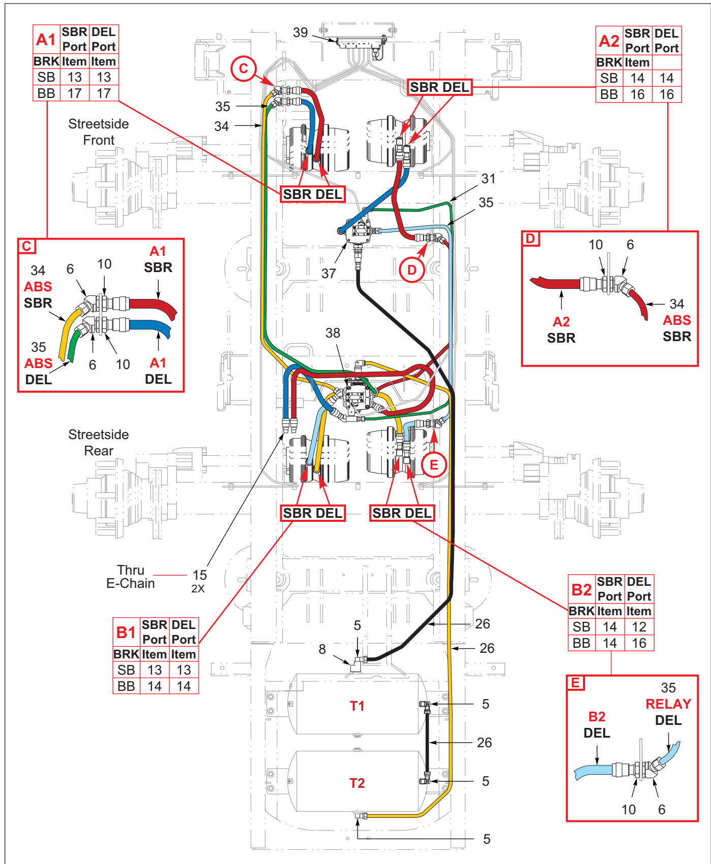
Figure 8-3: ABS, 2 Axle, Disc, Haldex (Option) (1 of 2)
