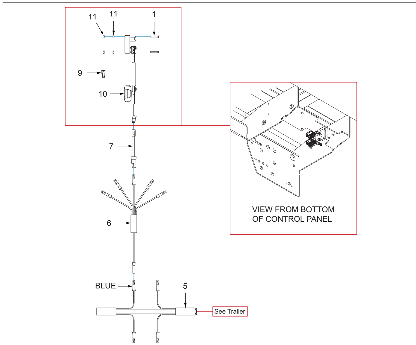
Figure 9-36: Remote Control Assembly, Wireless, Brand (After 08/01/2019)
