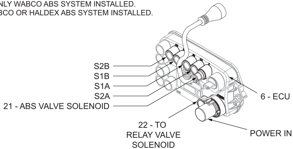
Figure 9-10: ABS, Haldex, 2 Axle (2 of 2)
