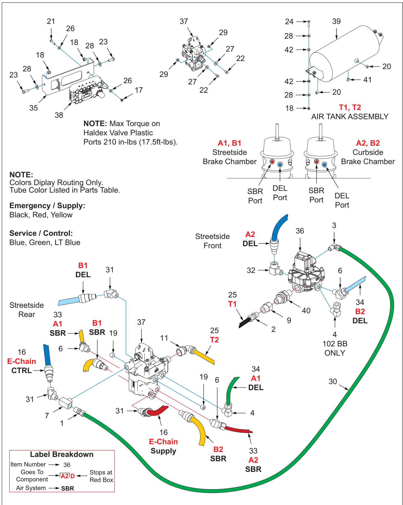
Figure 8-7: ABS, 2 Axle, Drum, Haldex (2 of 2)
