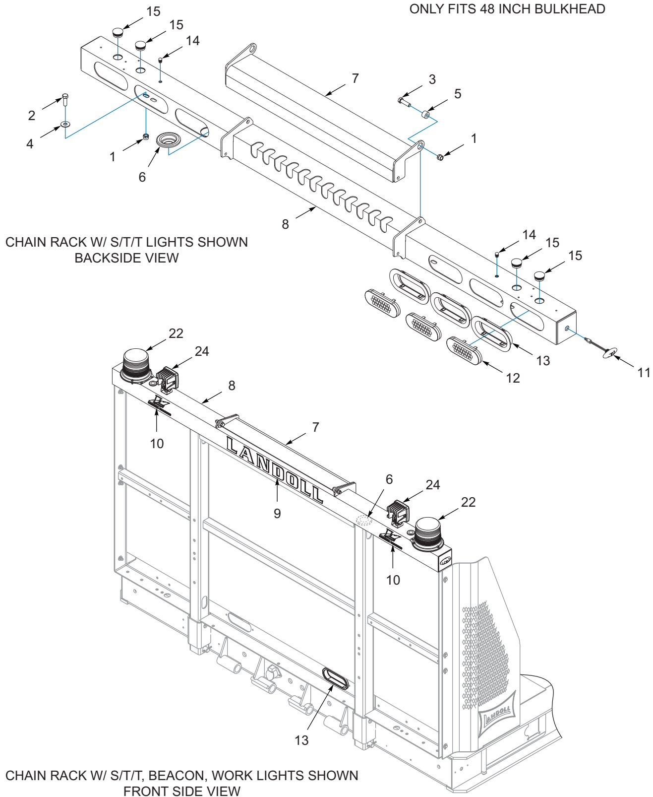
Figure 4-4: Bulkhead, Light Bar, Chain Rack (1 of 2)
