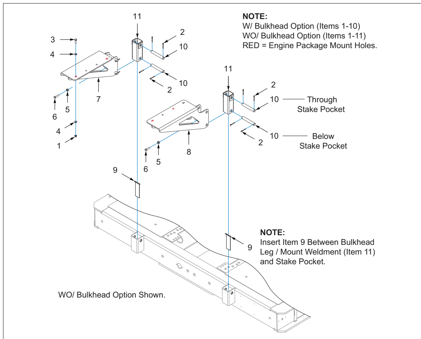
Figure 6-7: Mount, Engine, Front Extension, Pin-On
