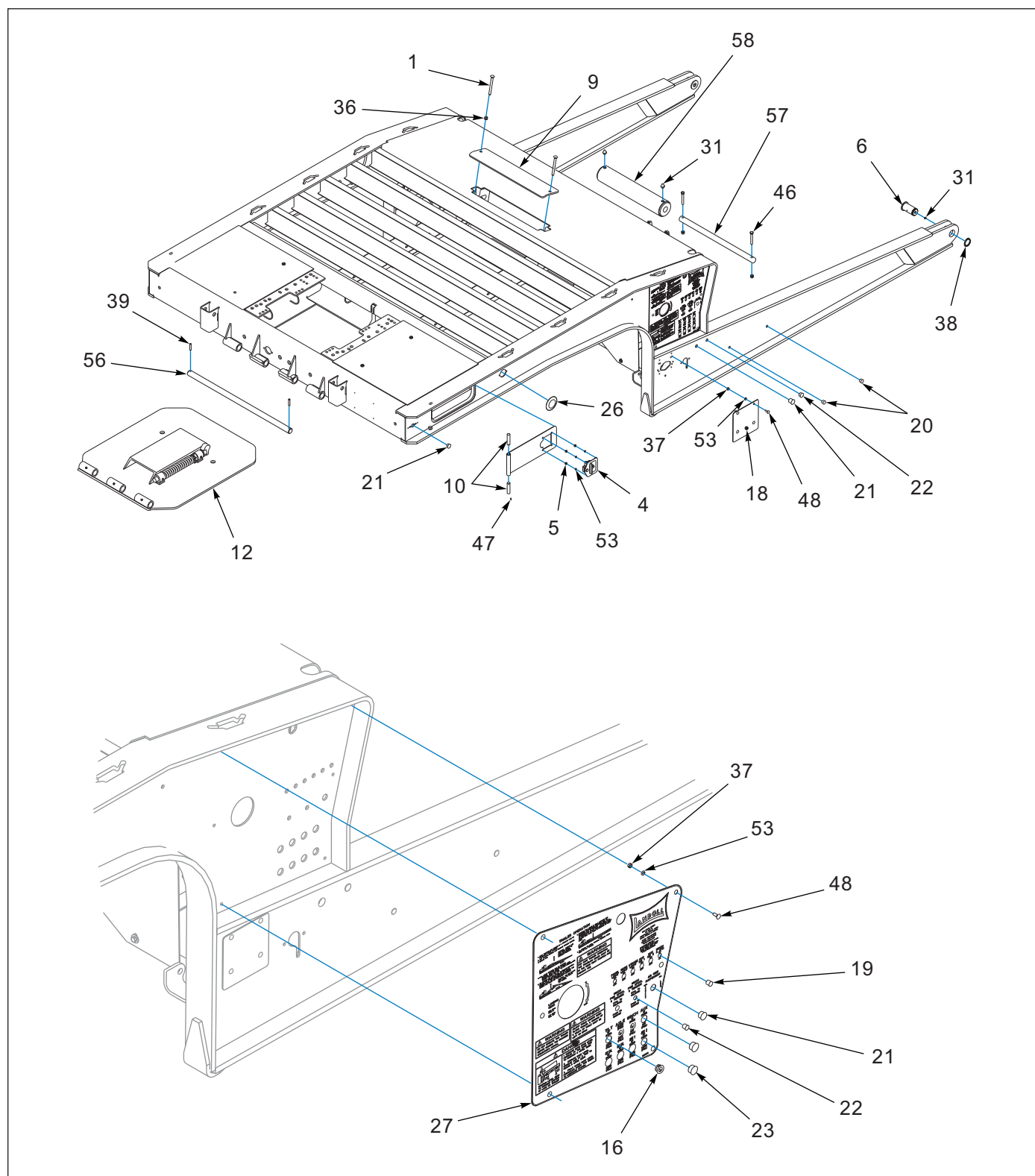
Figure 2-1: Frame Components, Upper Deck (1 of 3)
