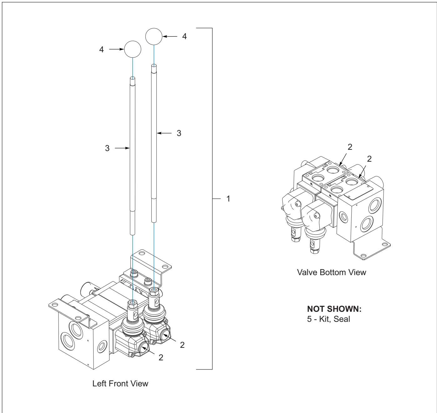
Figure 11-21: Valve Components, 2-Spool, Motor, Manual (Option)
