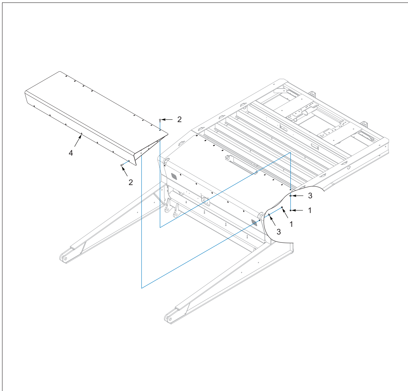
Figure 2-25: Leveler, Upper Deck, Slope Filler (Options)
