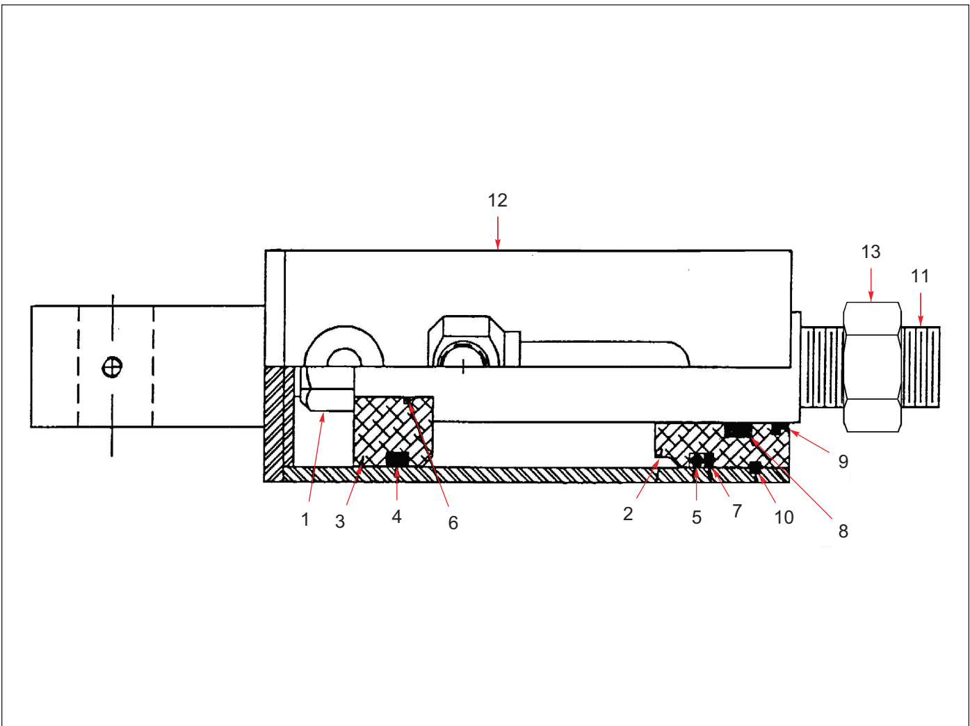
Figure 11-11: Cylinder Components, 2-1/2 x 2-3/4 (Option)
