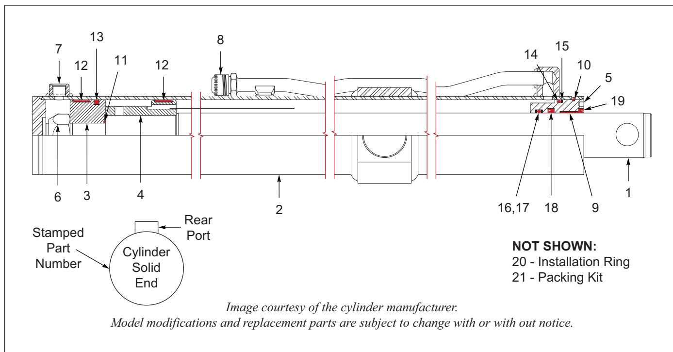
Figure 11-14: Cylinder Components, 4 x 100, 126, 138, Hi-Flow, Prince
