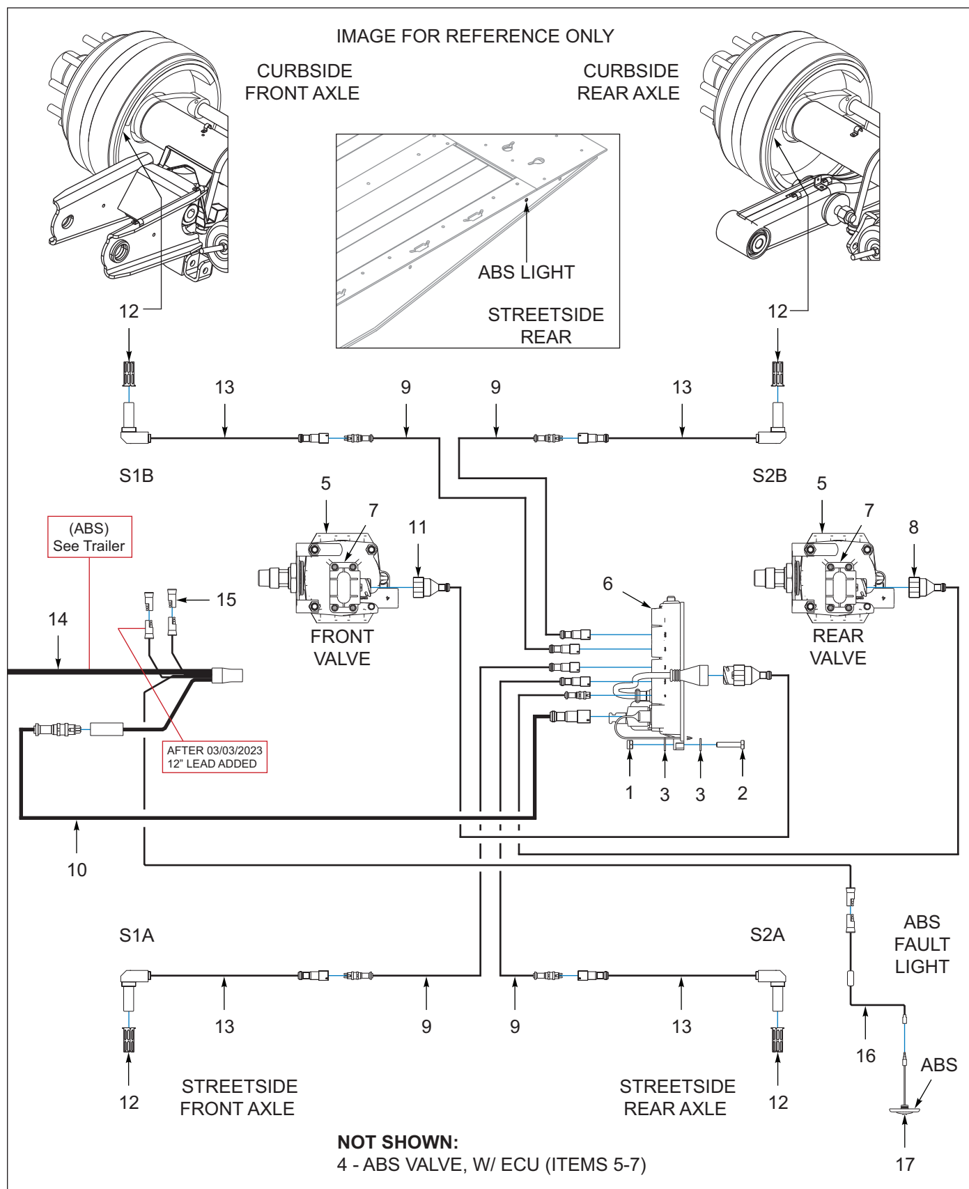
Figure 9-13: ABS, Haldex, 3 Axle (1 of 2)
