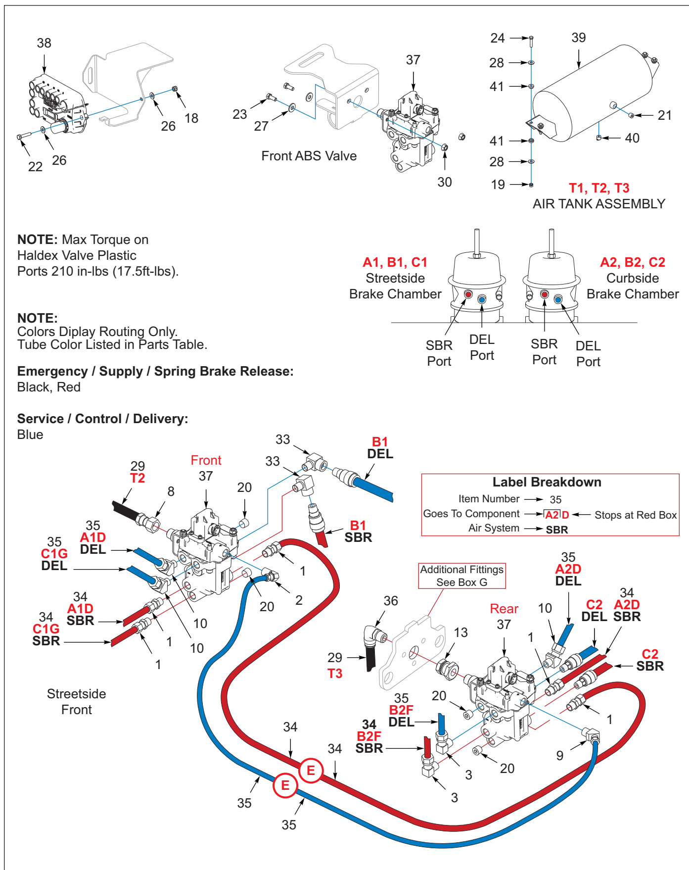
Figure 8-26: ABS, 3 Axle, Drum, Haldex (After 12/01/2025) (2 of 2)
