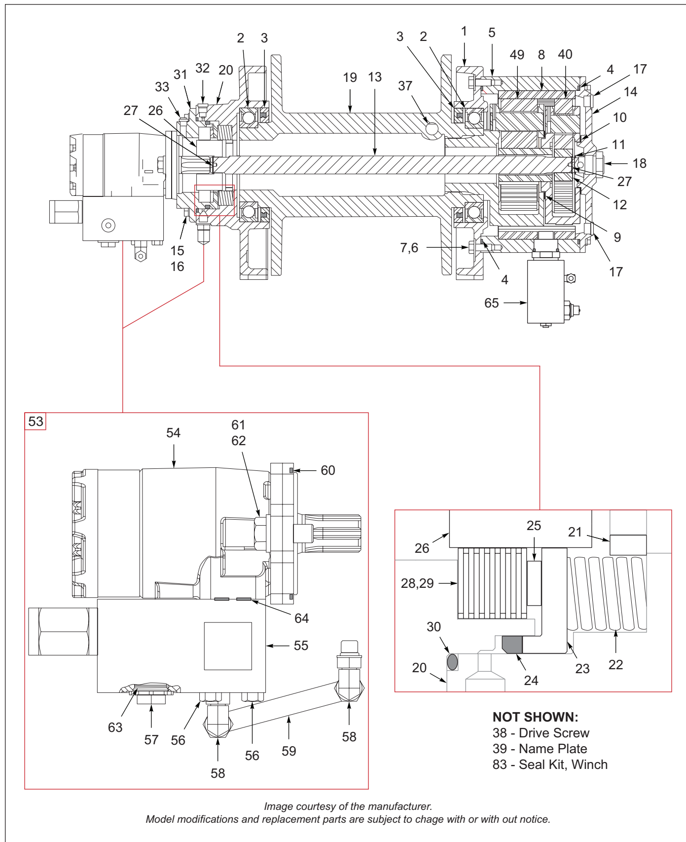
Figure 7-15: Winch Components, Braden 20K, 2-Speed (1 of 2)
