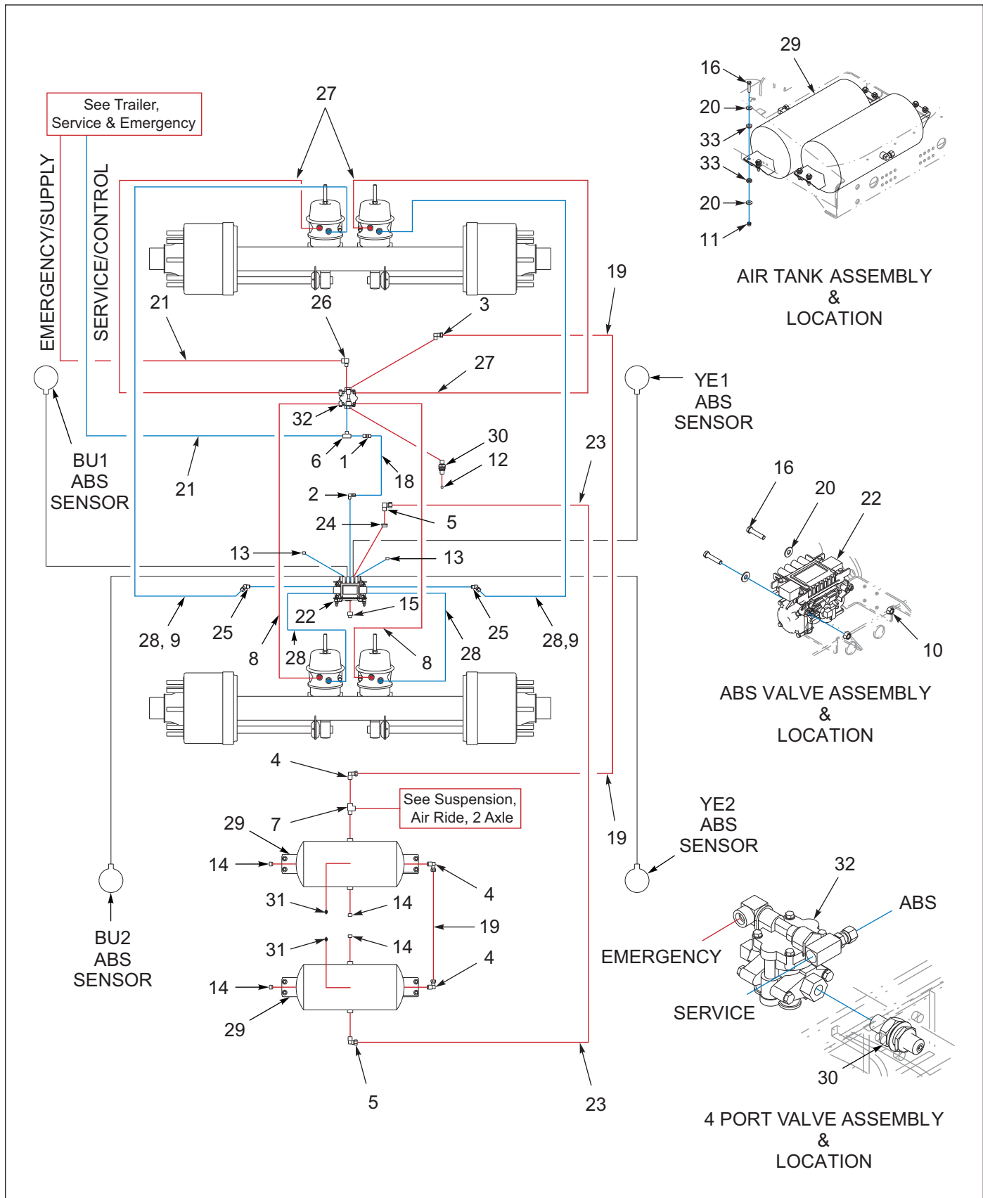
Figure 8-5: ABS, 2 Axle, Drum, Wabco
