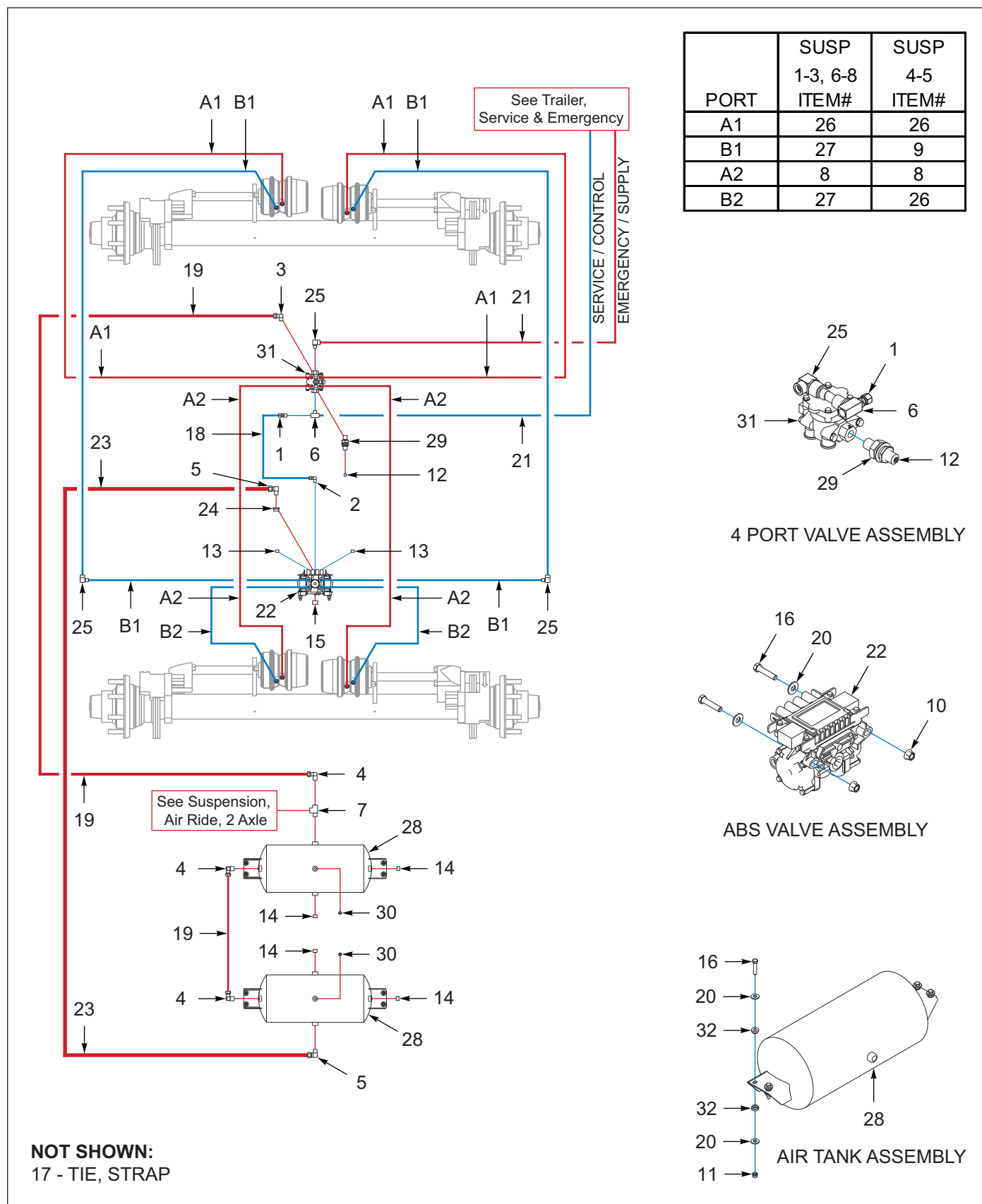
Figure 8-2: ABS, 2 Axle, Disc, Wabco (Option)
