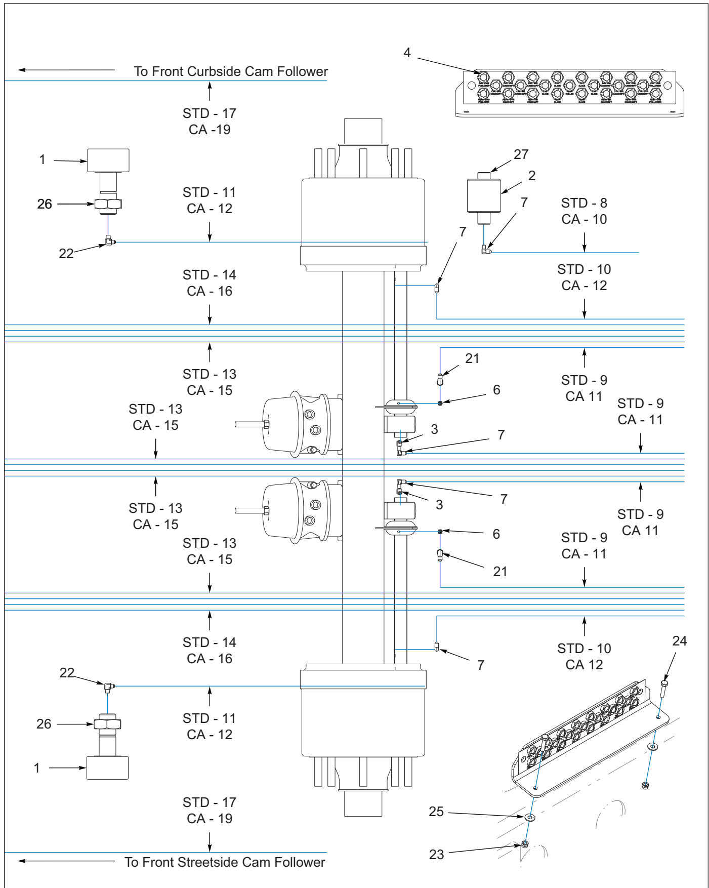
Figure 10-18: 3 Axle, Cam Followers, Drum Brakes (11/07/2018 To 08/31/2020) (2 of 2)
