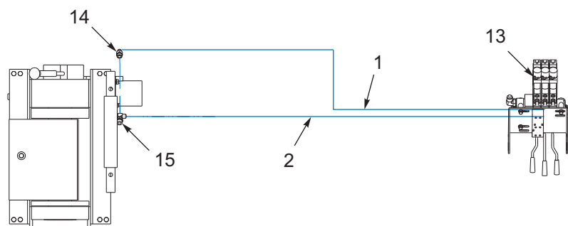
HYDRAULIC SYSTEM
