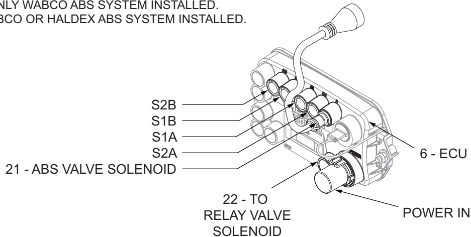
Figure 9-12: ABS, Haldex, 2 Axle, Spread (Option) (2 of 2)
