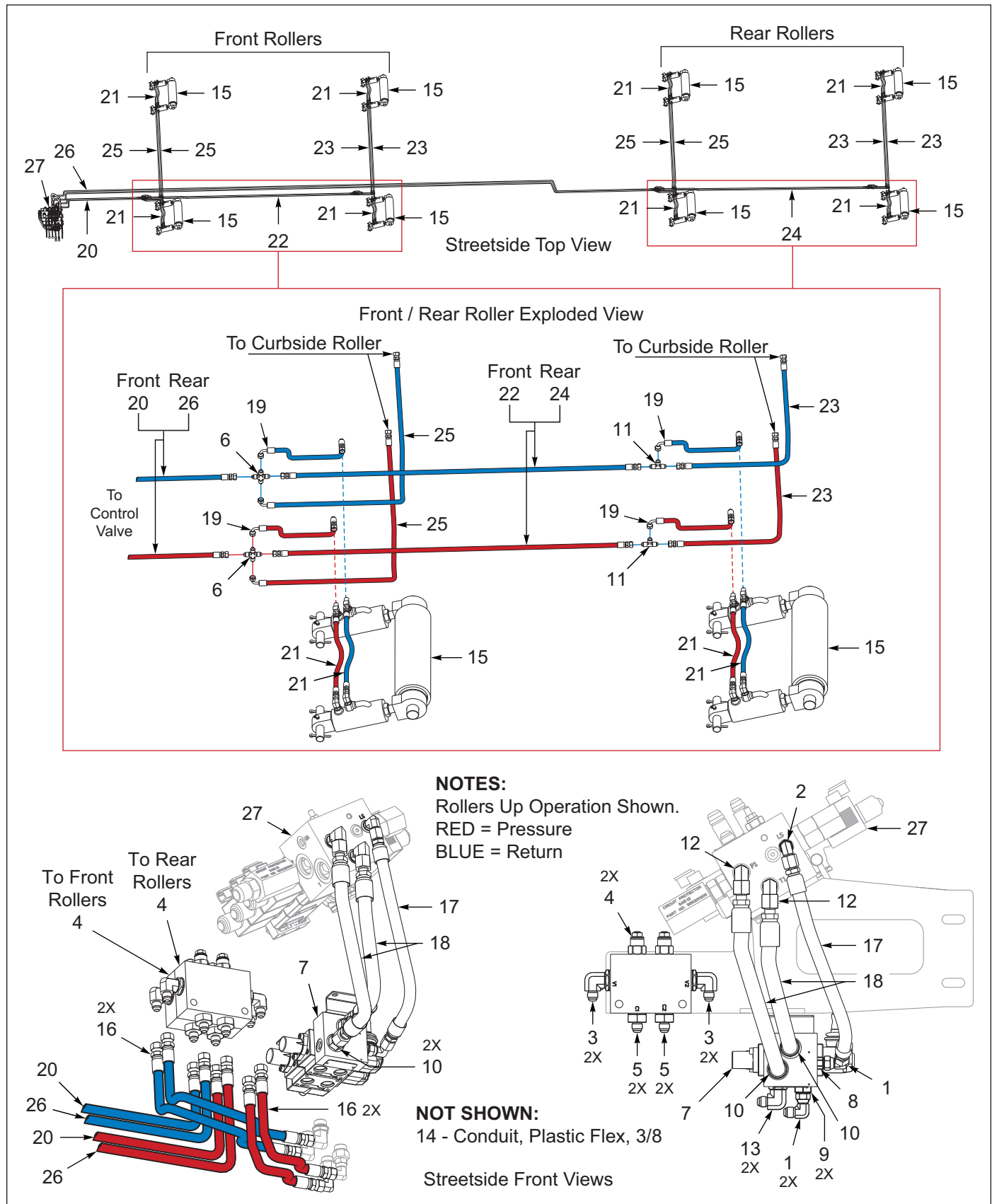
Figure 11-7: Rollers, Deck, 8-Pop-Ups, 57 Foot (Options)
