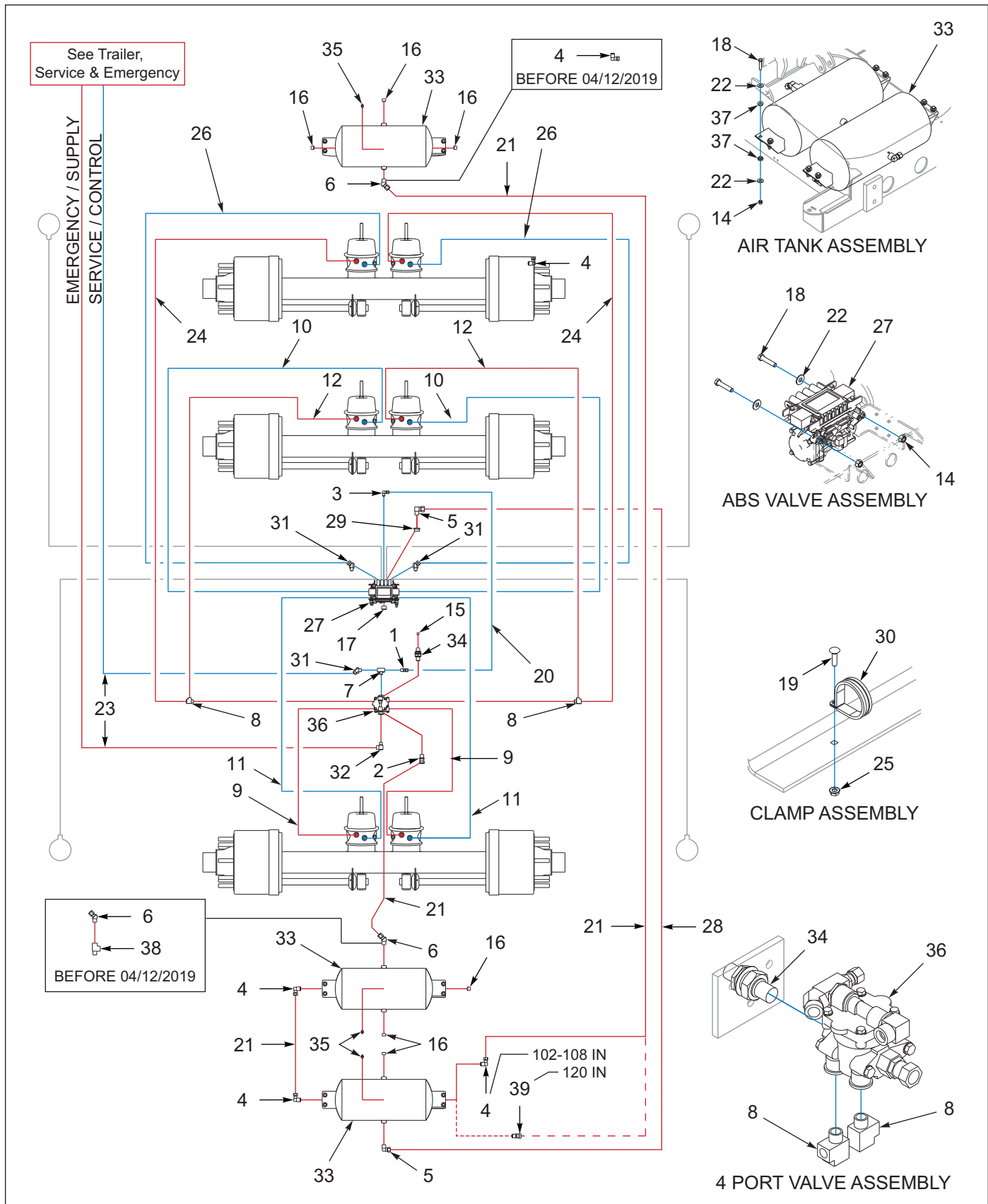
Figure 8-15: ABS, 3 Axle, Drum, Wabco (Before 03/10/2023)
