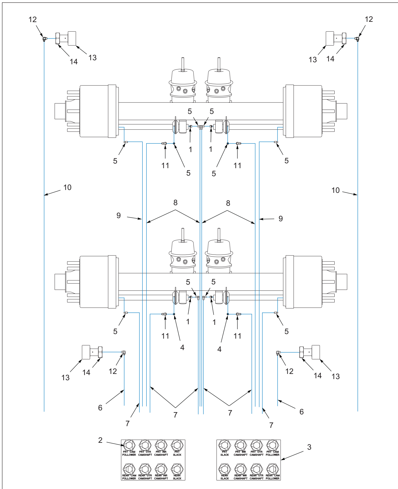
Figure 10-2: 2 Axle, Cam Followers, Drum Brakes (11/07/2018 To 08/31/2020)
