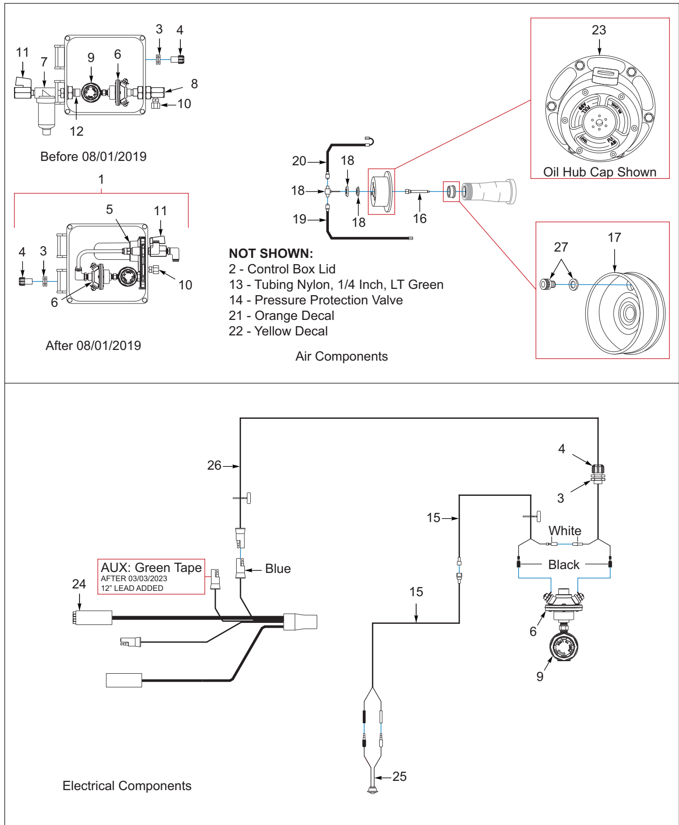
Figure 8-60: Tire Inflation Components &amp; Electrical System (Option)
