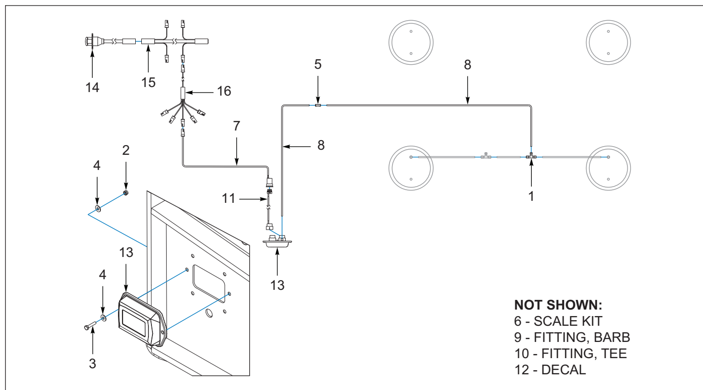
Figure 8-38: Scale, Loadmaxx Plus & Quickload Plus (Options) (AFTER 03/31/2020)
