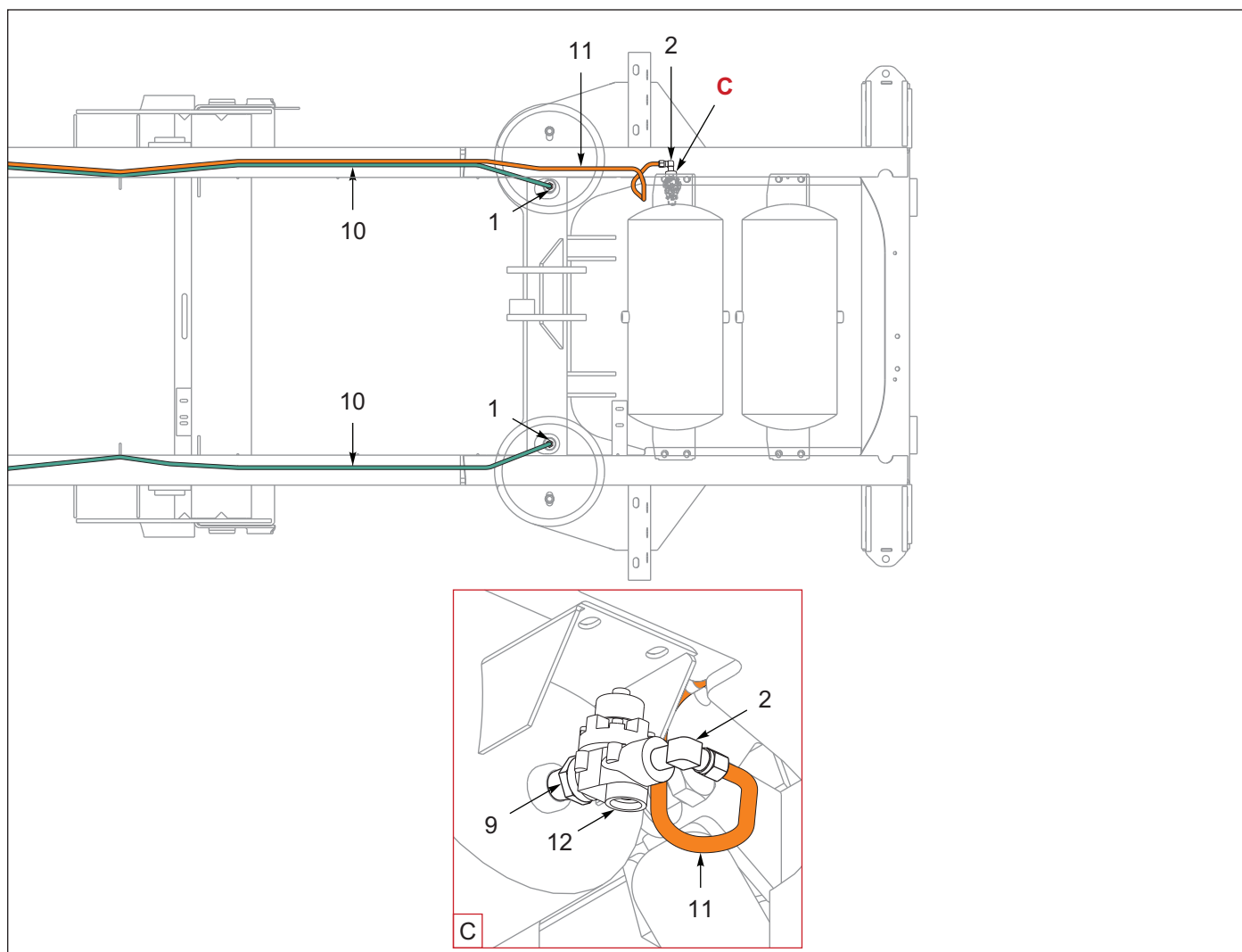
Figure 8-50: Suspension, Air Ride, 3 Ax, Aqua, 3/8 in (Option) (After 03/10/2023) (2 of 2)
