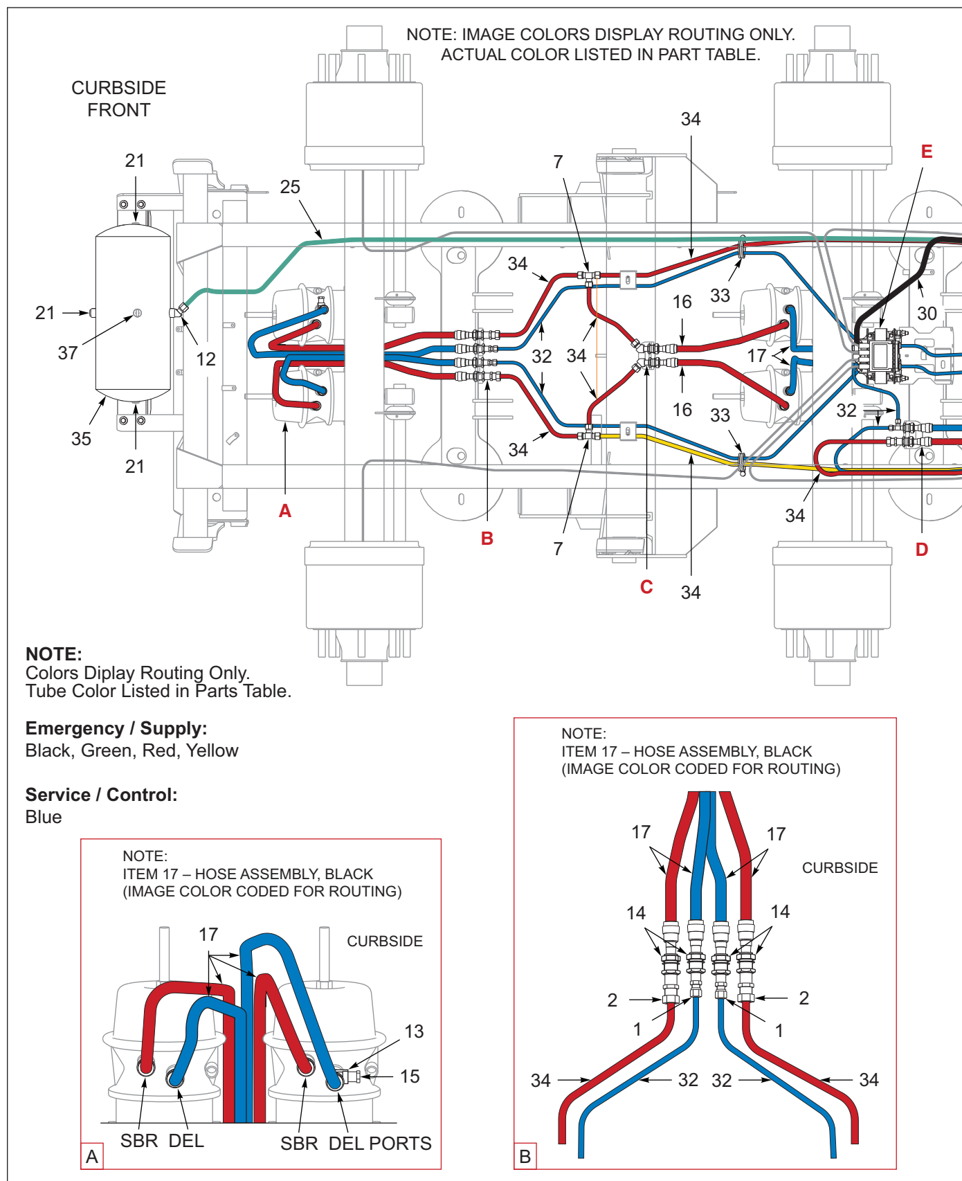
Figure 8-16: ABS, 3 Axle, Drum, Wabco (03/10/2023 To 06/12/2023) (1 of 3)
