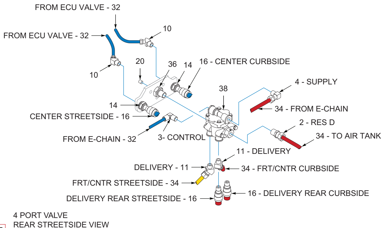
Figure 8-18: ABS, 3 Axle, Drum, Wabco (03/10/2023 To 06/12/2023) (3 of 3)
