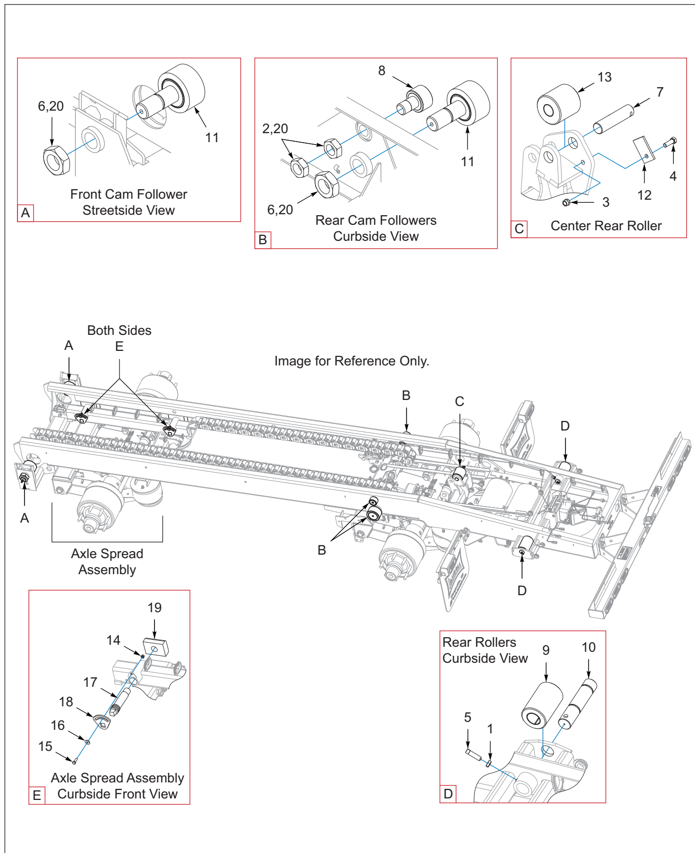
Figure 2-8: Cam Followers, Rear Roller, Slides, 2 Axle Spread (Option)
