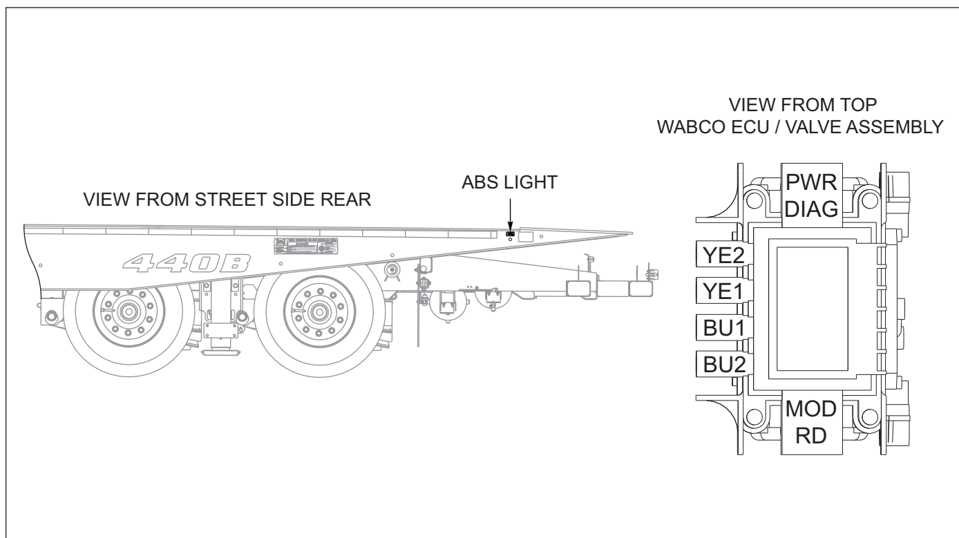
Figure 9-6: ABS, Wabco (2 of 2)
