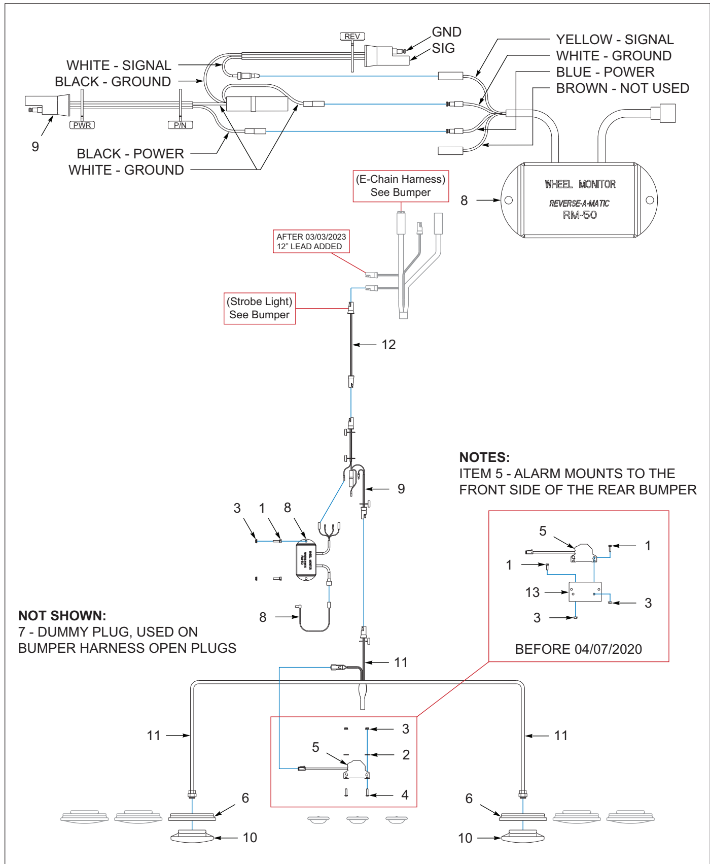
Figure 9-21: Lights, Backup & Alarm, Bumper (Option)
