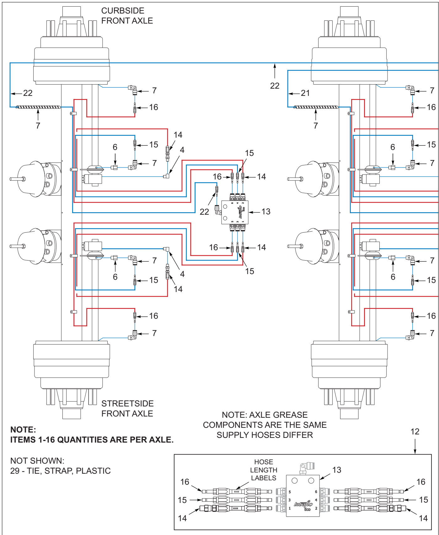
Figure 10-19: 3 Axle, Cam Followers, Drum Brakes (08/31/2020 To 12/01/2025) (1 of 3)
