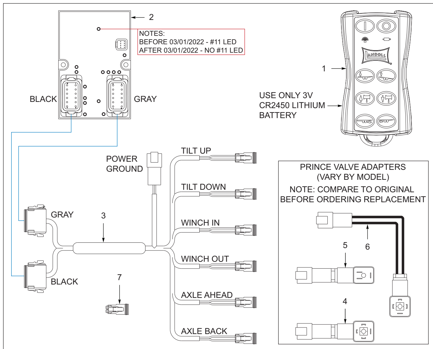
Figure 9-37: Remote Control Kit, Wireless, Brand (After 08/01/2019)
