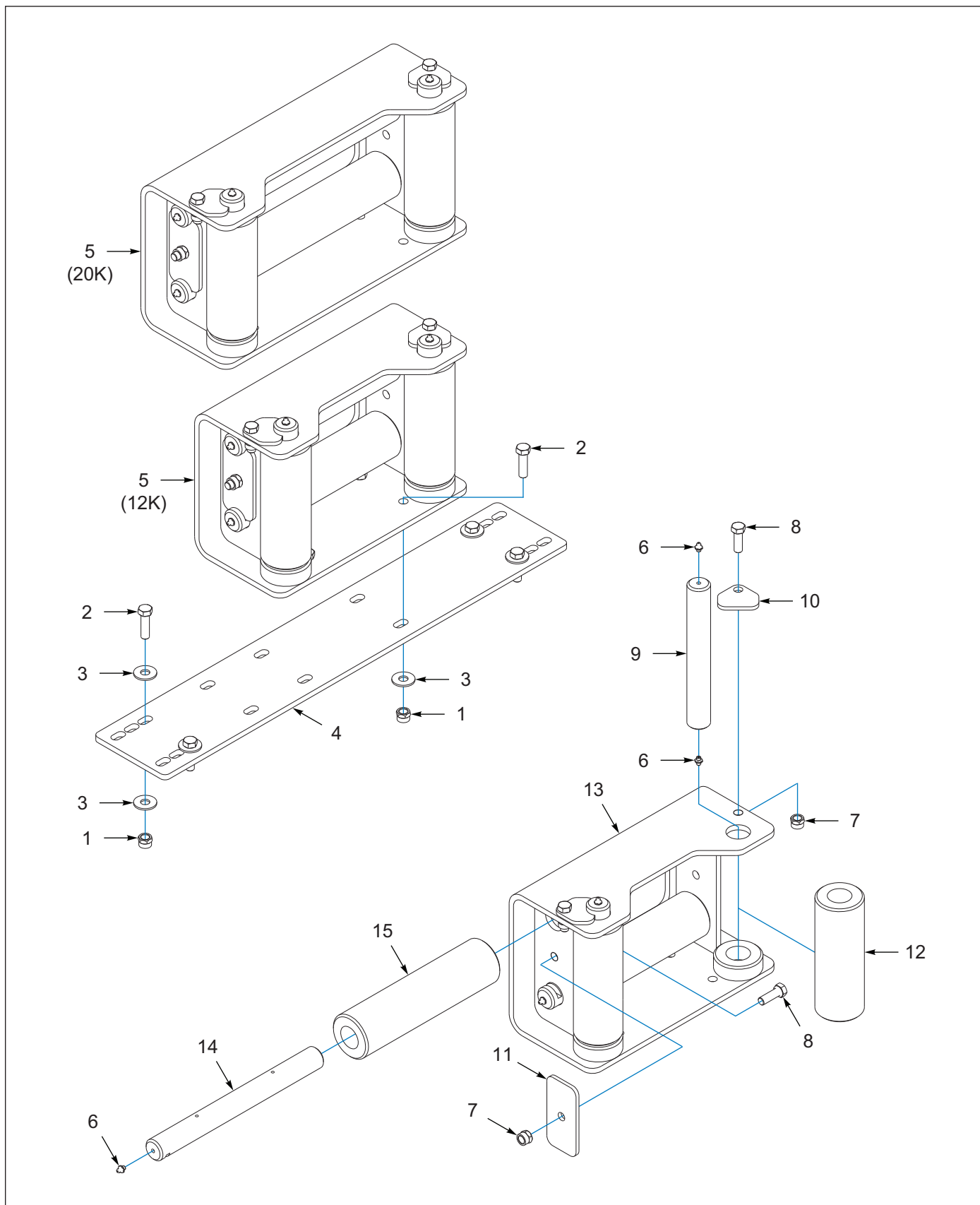
Figure 7-23: Cable Guide, 4-Roller, Braden 12K / 20K
