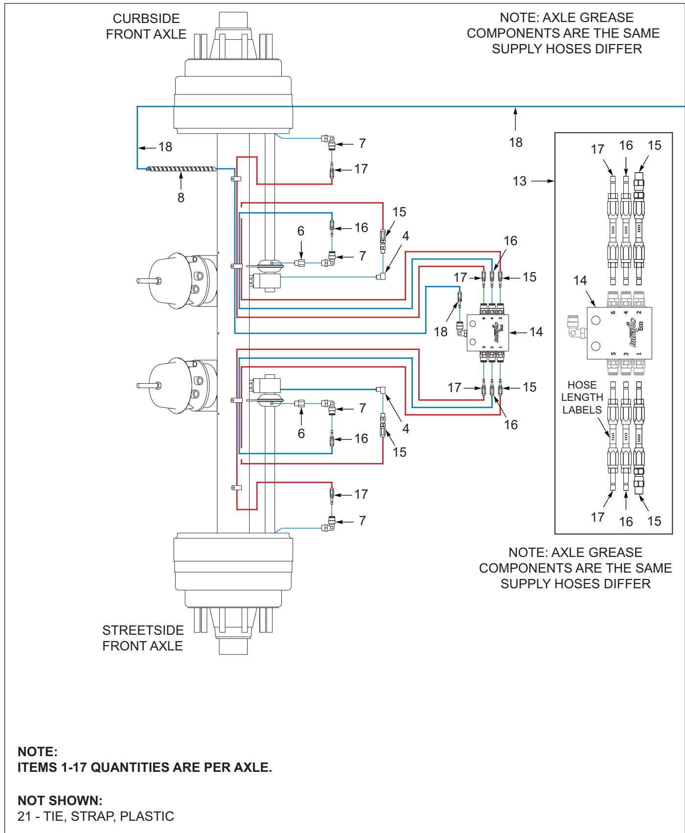
Figure 10-9: 2 Axle, Drum Brakes (After 09/01/2024) (1 of 3)
