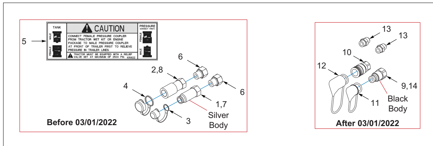
Figure 11-9: Coupler Kit, Hydraulic, Replacement & Repair
