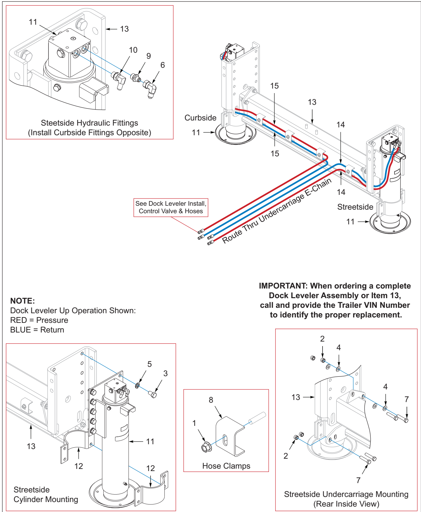
Figure 11-3: Dock Leveler Install, Single Leg Assembly, 62K (Option)
