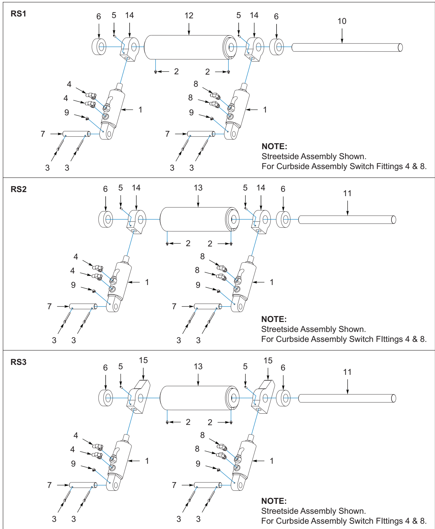
Figure 11-19: Roller Assembly, Deck, Pop-Ups (Options)
