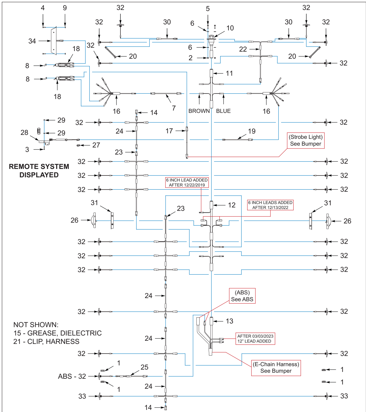
Figure 9-1: Trailer (Before 6/13/2023)
