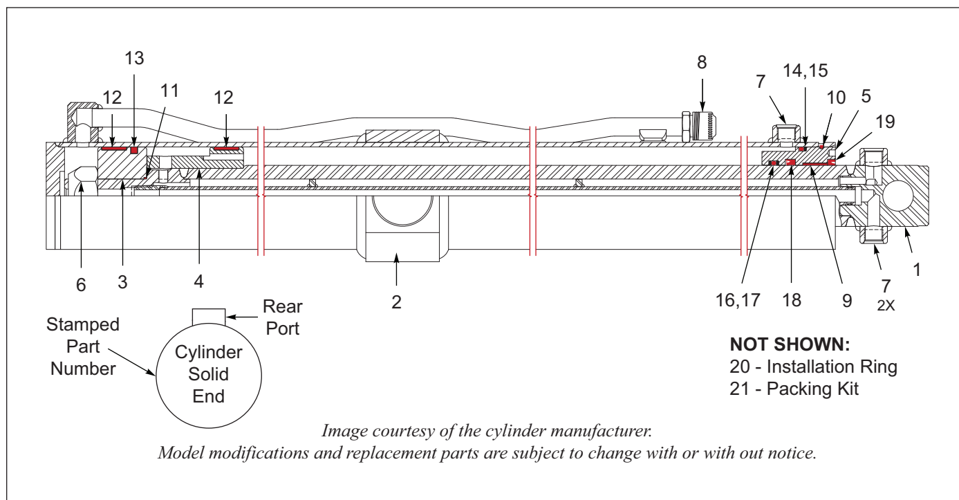
Figure 11-16: Cylinder Components, 4 x 100, 126, 138, Hi-Flow, Ported Rod, Prince
