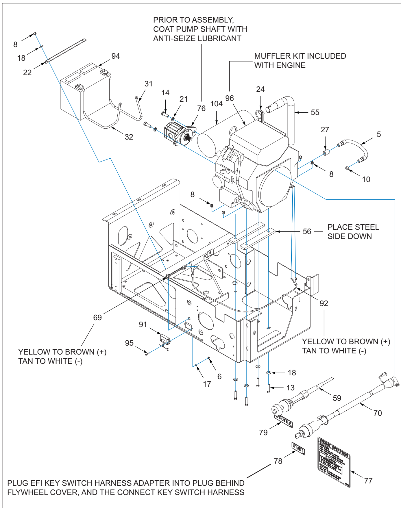
Figure 6-3: Engine, 25HP, Upper Deck Assembly (3 of 5)
