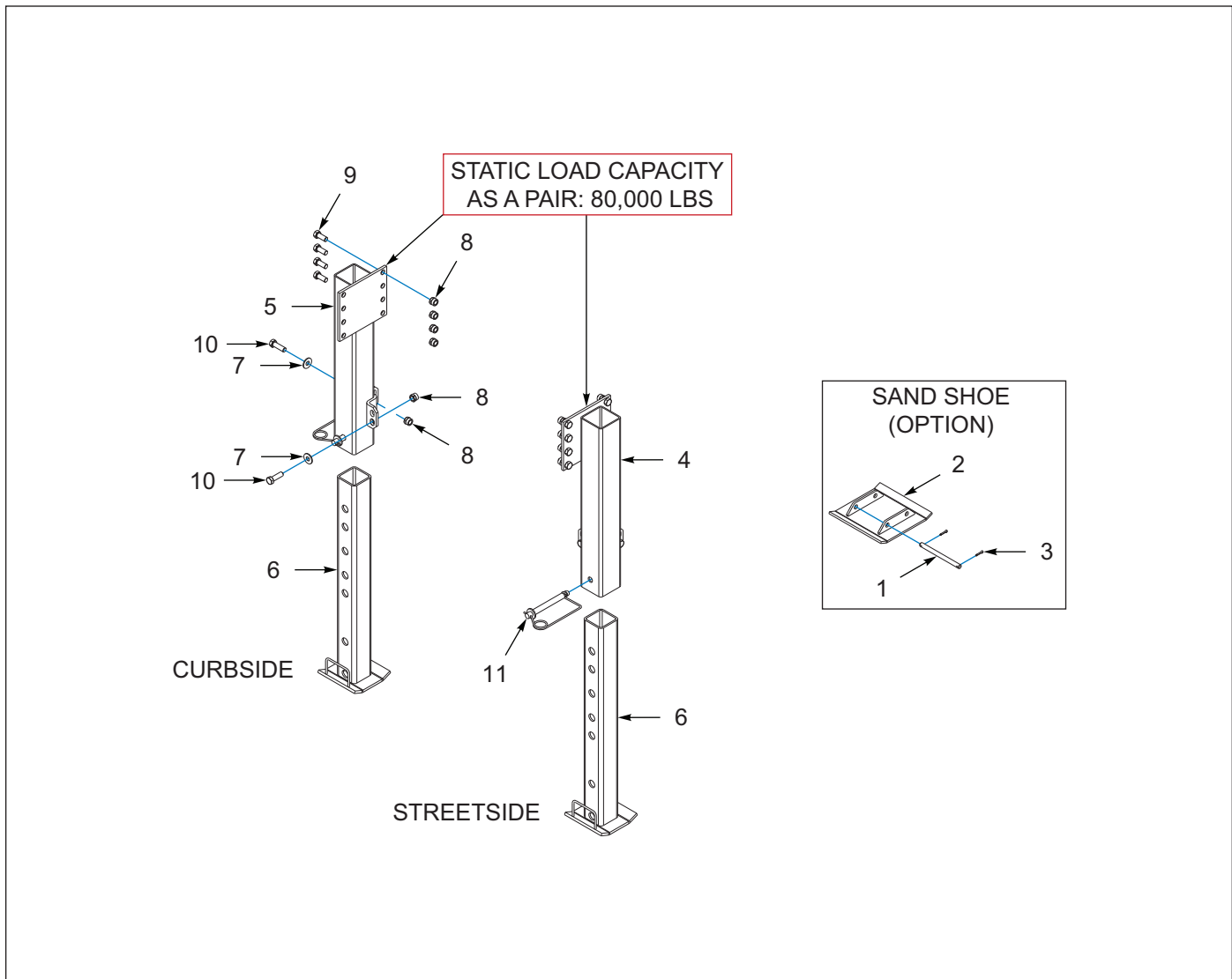
Figure 2-23: Landing Legs, Pinned (Option)
