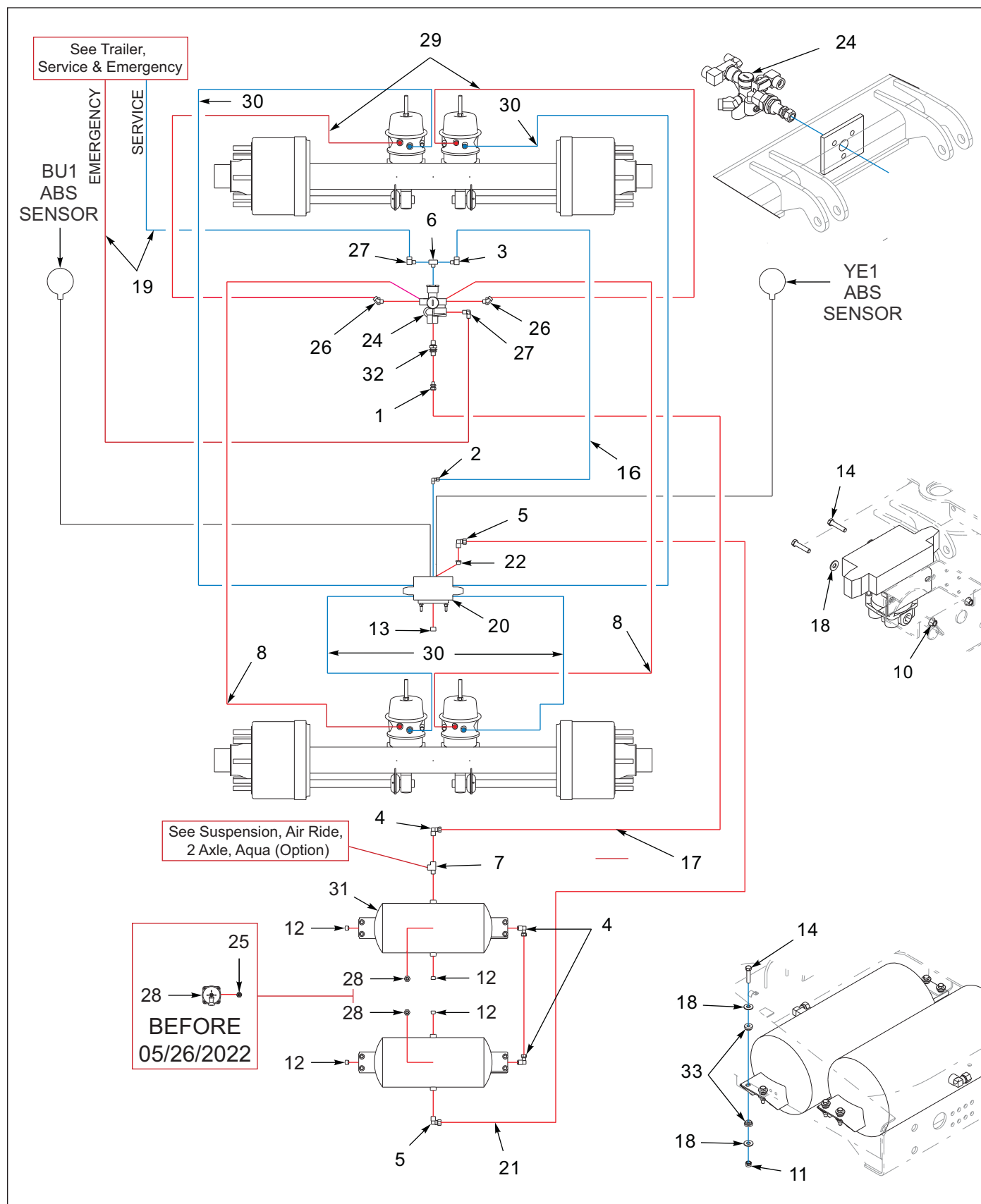
Figure 8-8: ABS, 2 Axle, Drum, Aqua (Option)
