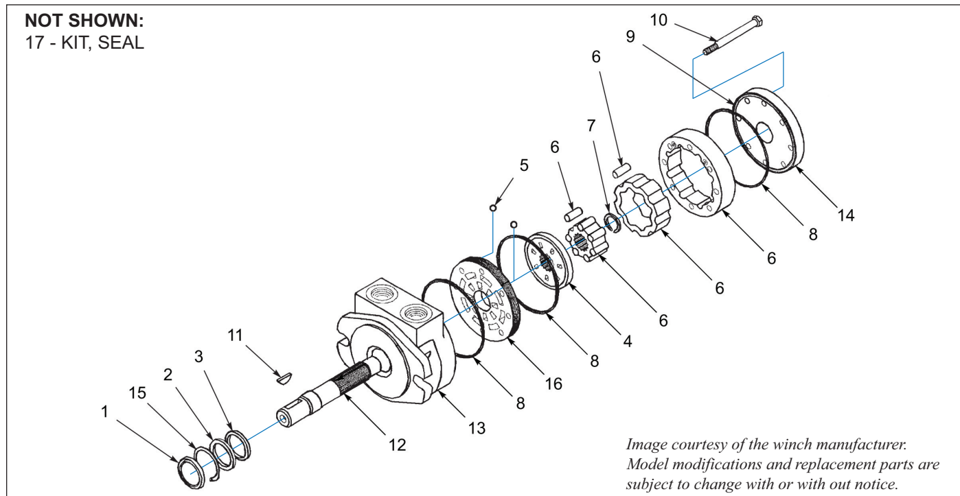
Figure 7-14: Winch Components, Braden 12K / 20K, 1-Speed, Motor
