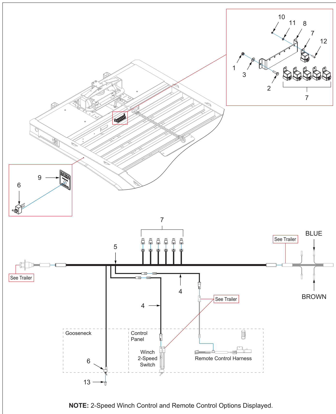
Figure 9-15: Electrical Disconnect, Complete Trailer (Option)
