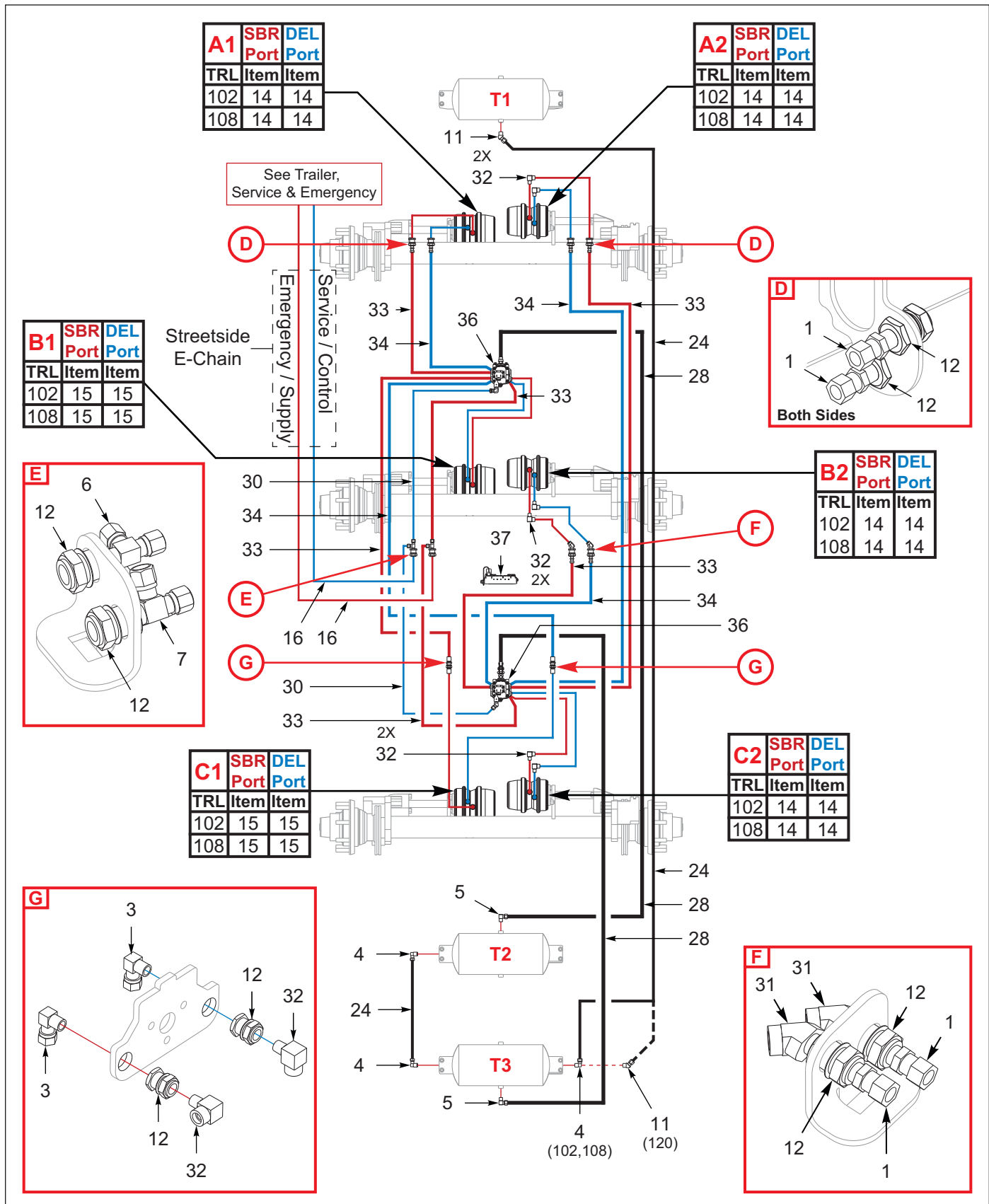
Figure 8-11: ABS, 3 Axle, Disc, Haldex, 102 / 108 (Option) (After 12/01/2025) (1 of 2)
