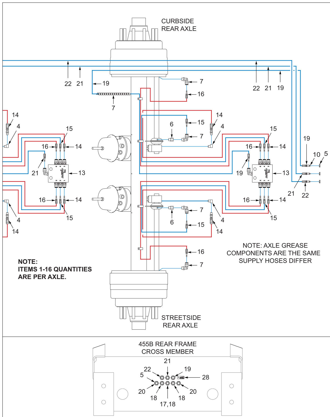
Figure 10-20: 3 Axle, Cam Followers, Drum Brakes (08/31/2020 To 12/01/2025) (2 of 3)
