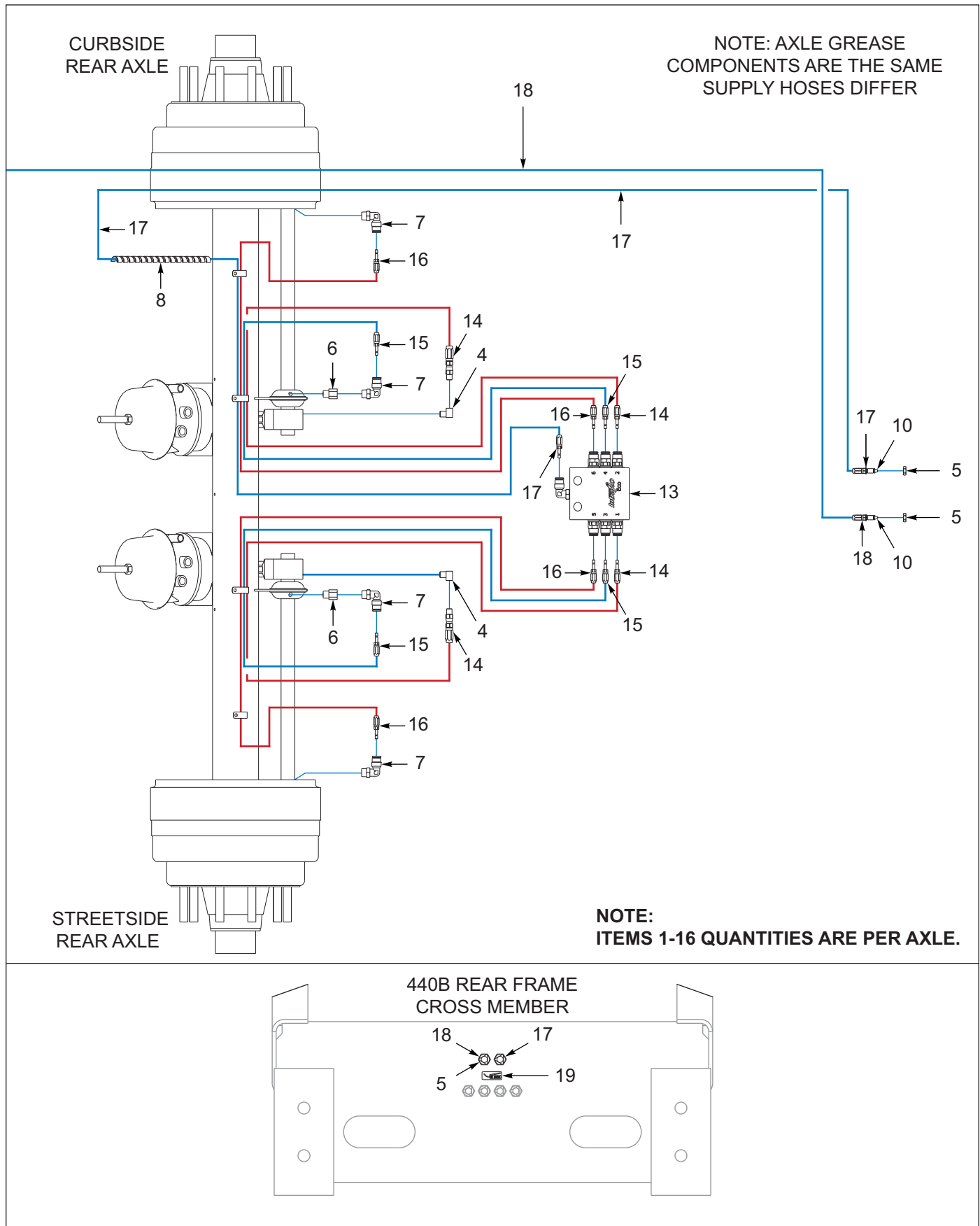
Figure 10-7: Axle, Drum Brakes (After 08/31/2020 To 09/01/2024) (2 of 3)
