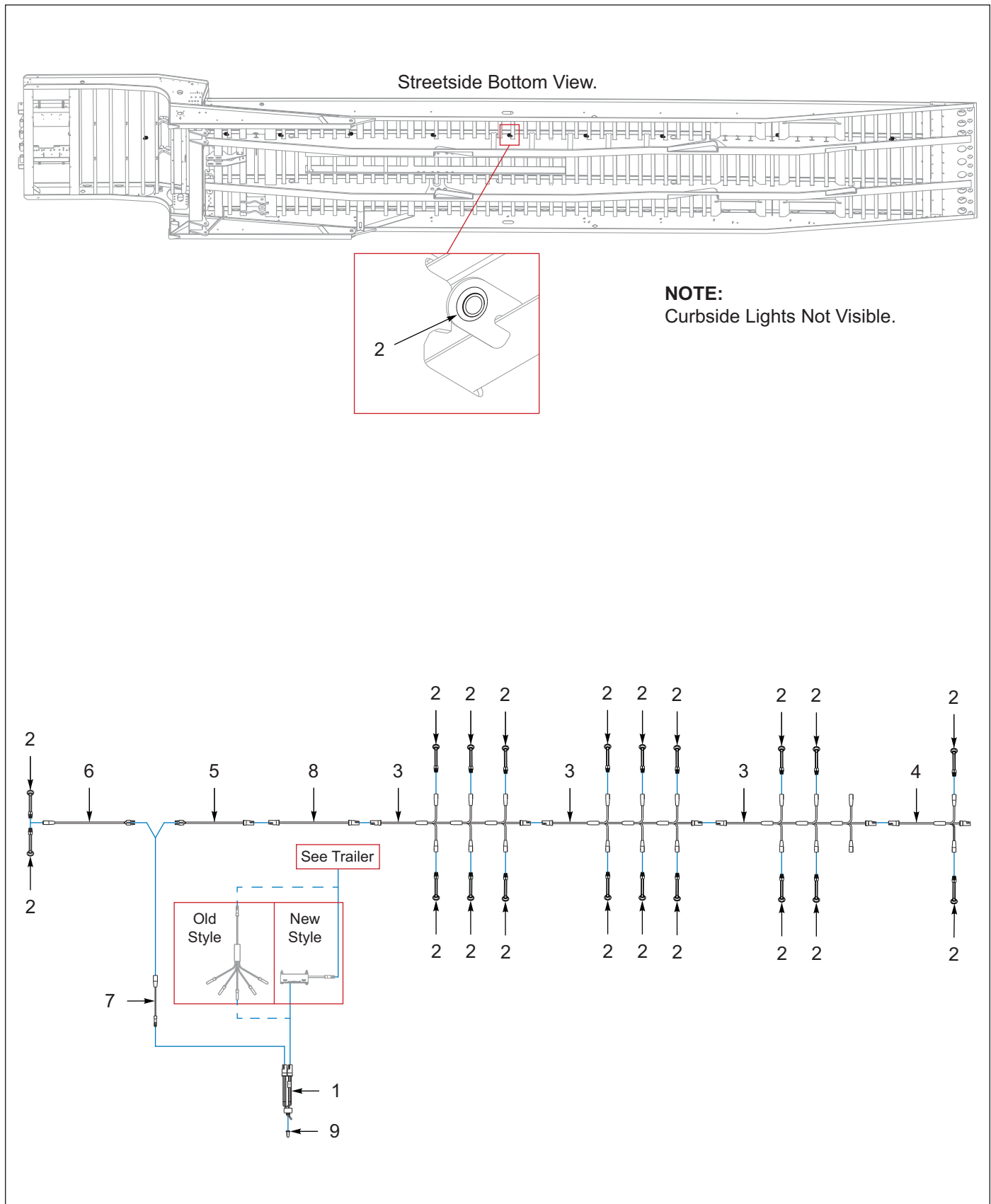
Figure 9-31: Lights, Work Zone, Under Deck (Option) (Before 01/19/2024)
