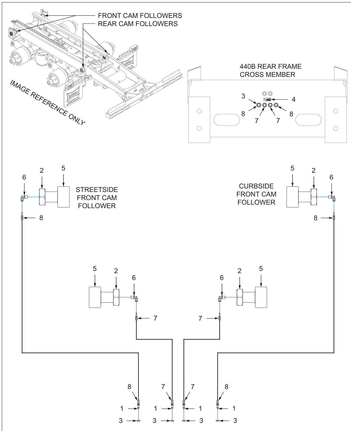
Figure 10-4: 2 Axle, Cam Followers (After 09/01/2024)
