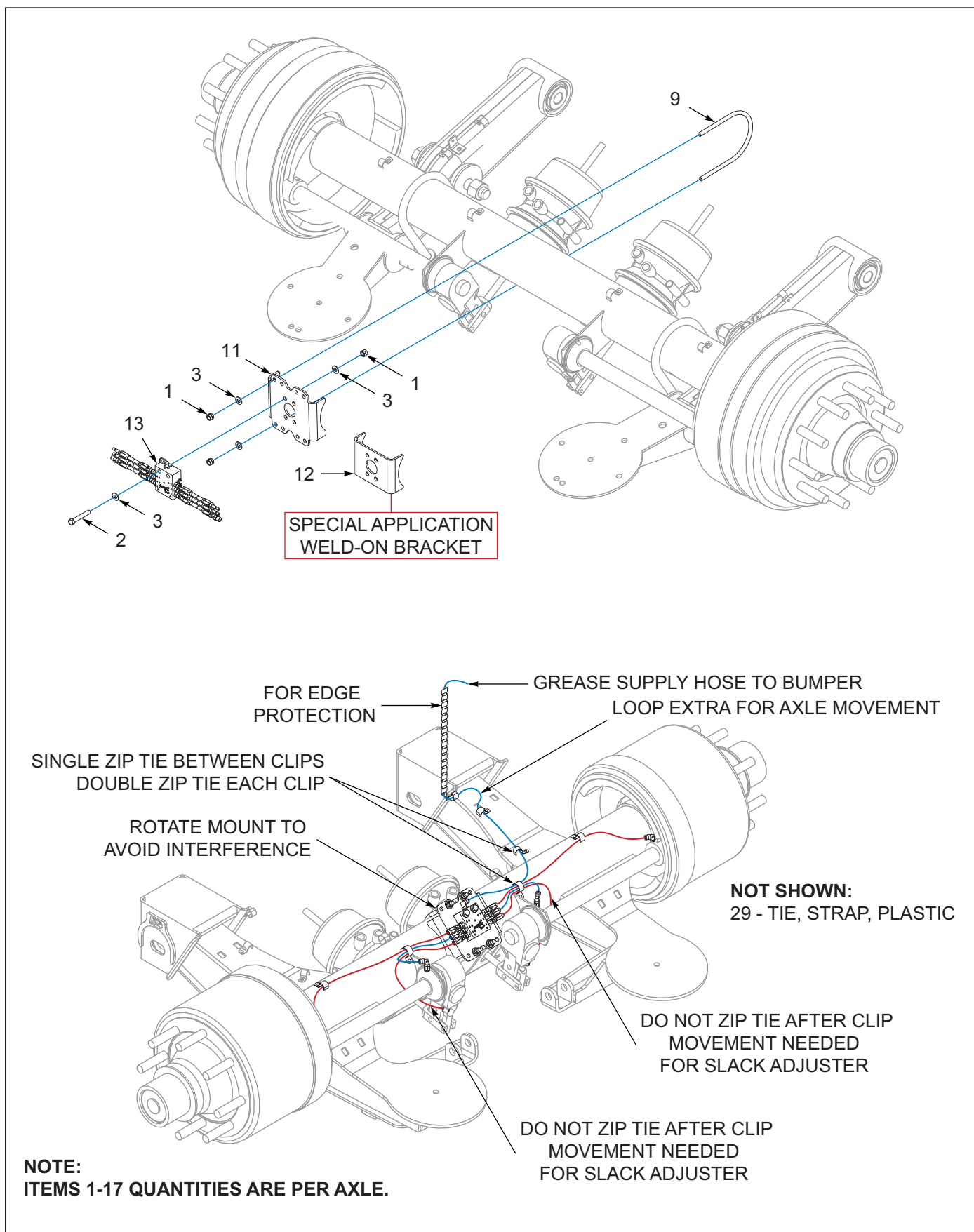
Figure 10-25: 3 Axle, Drum Brakes (After 12/01/2025) (3 of 3)
