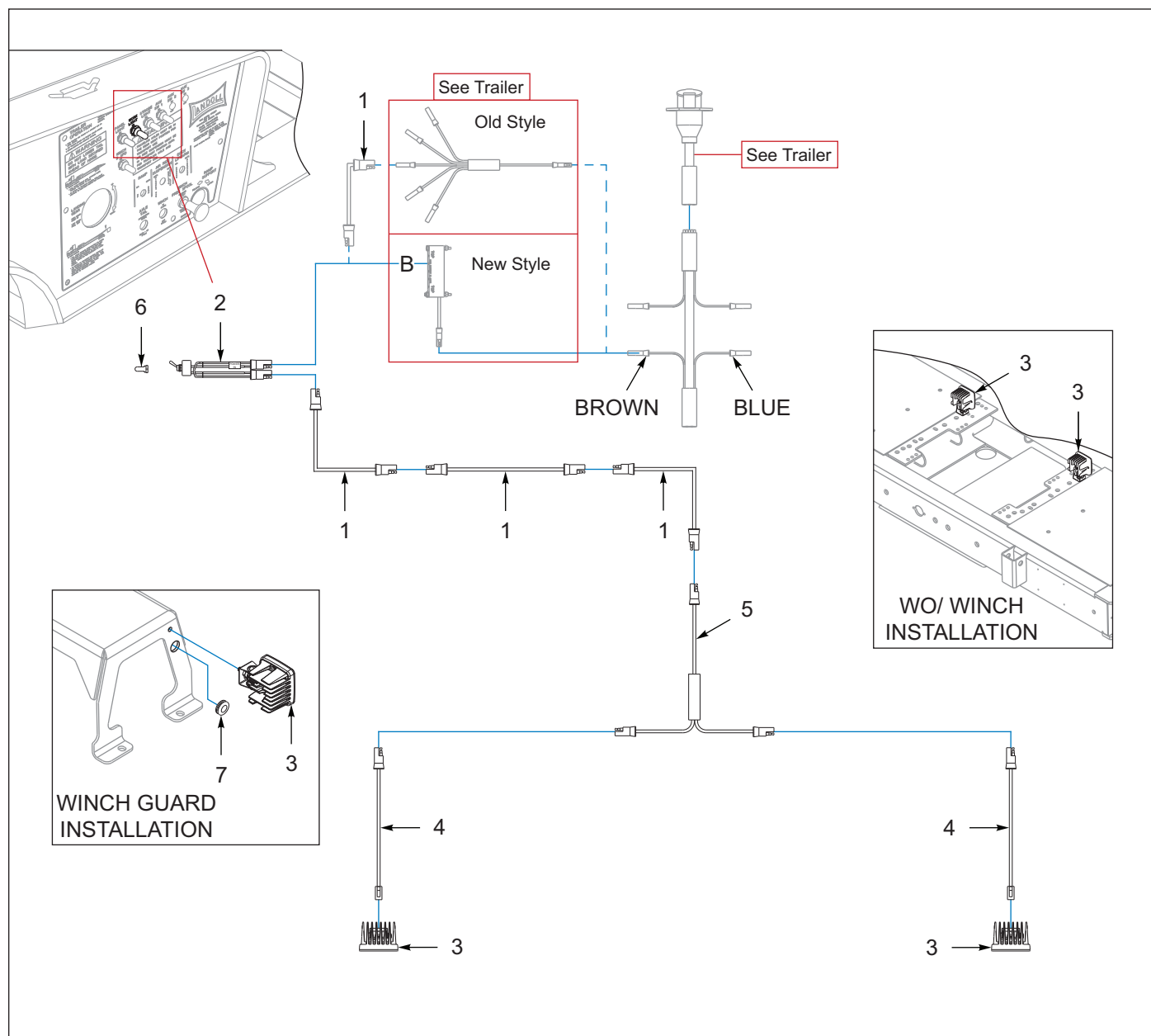
Figure 9-30: Lights, Work, Upper Deck, Winch (Option)
