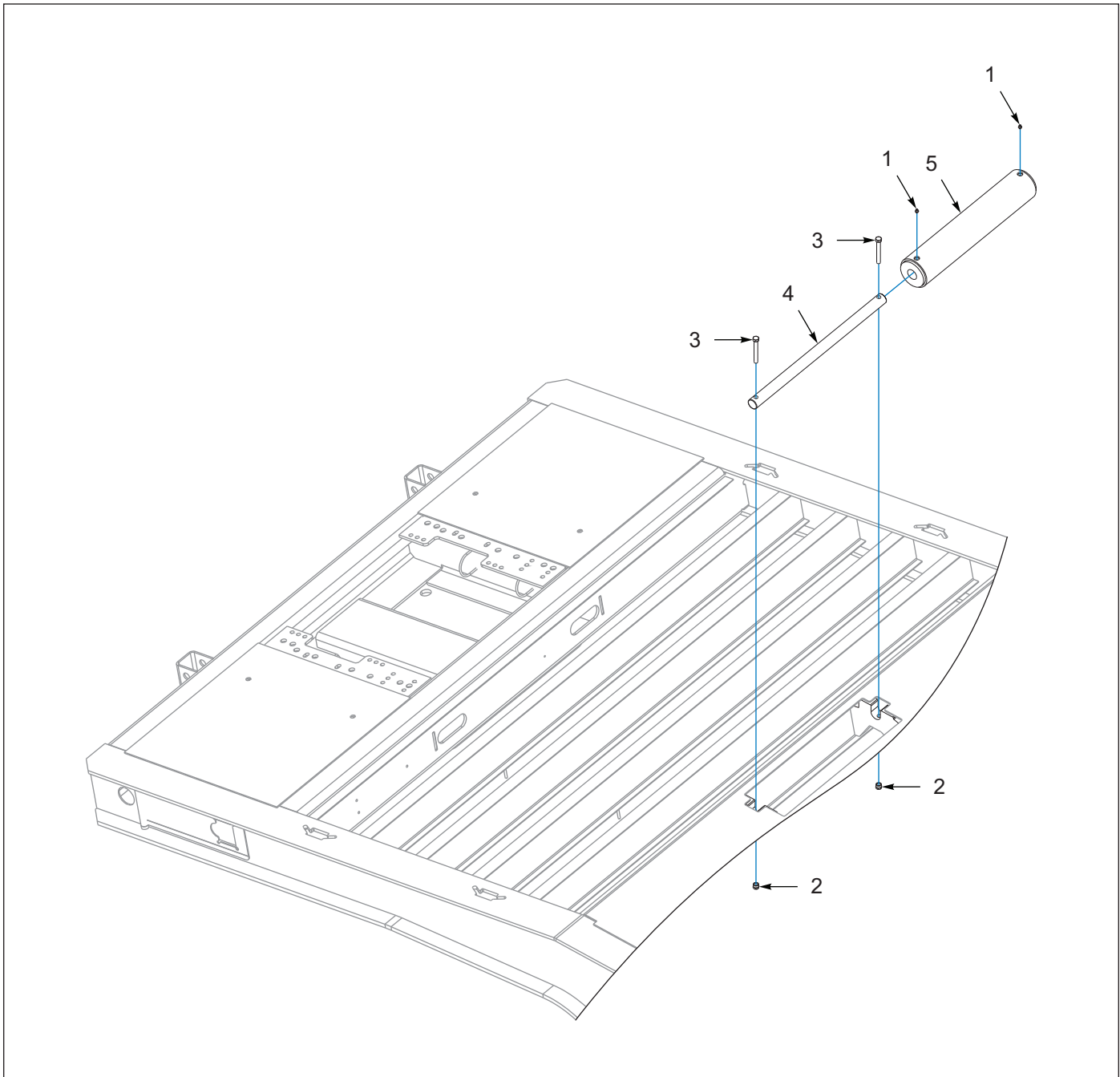
Figure 7-25: Deck Roller, Slope, Upper Deck
