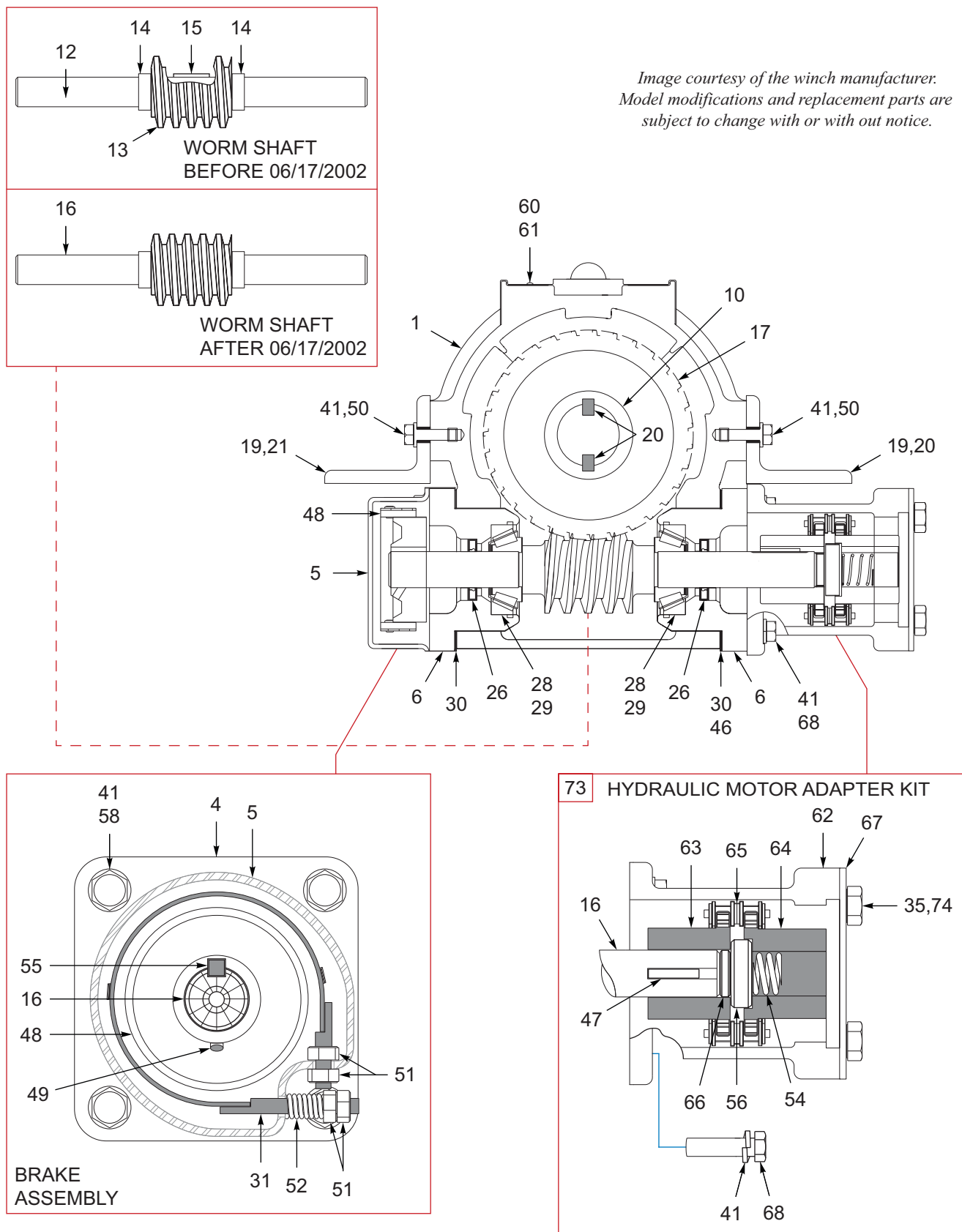
Figure 7-12: Winch Components, Braden 12K, 1-Speed (2 of 2)
