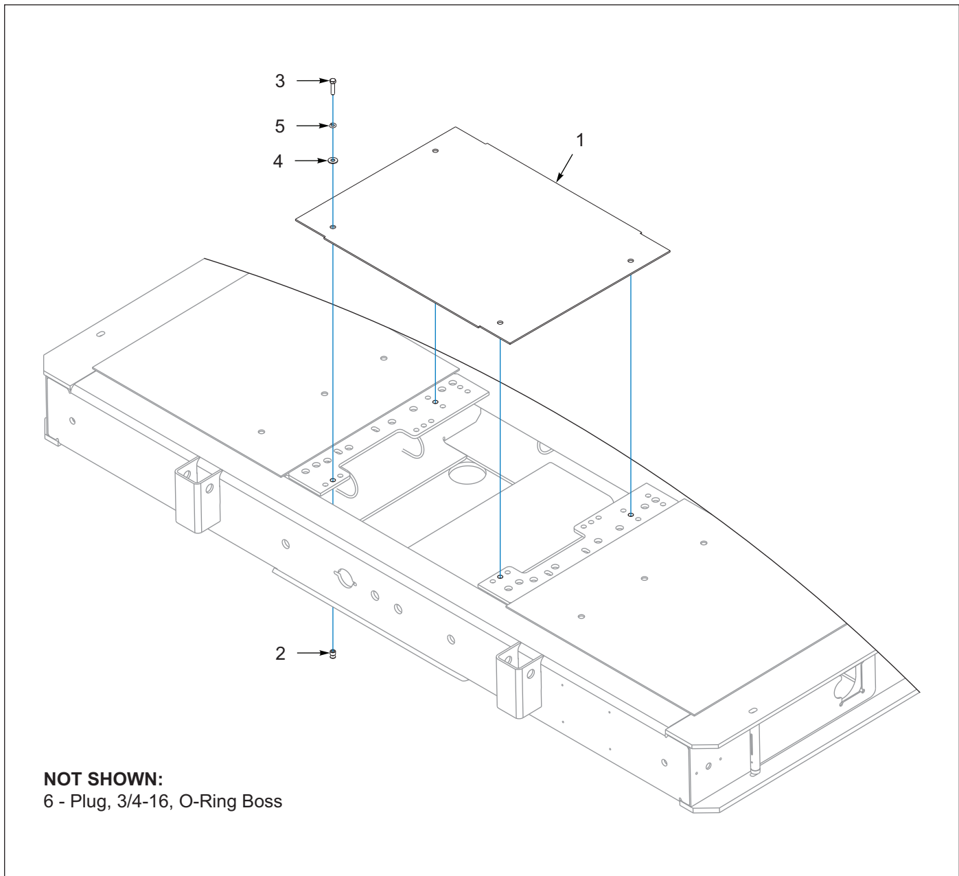
Figure 2-10: Cover, Winch Mount, Upper Deck
