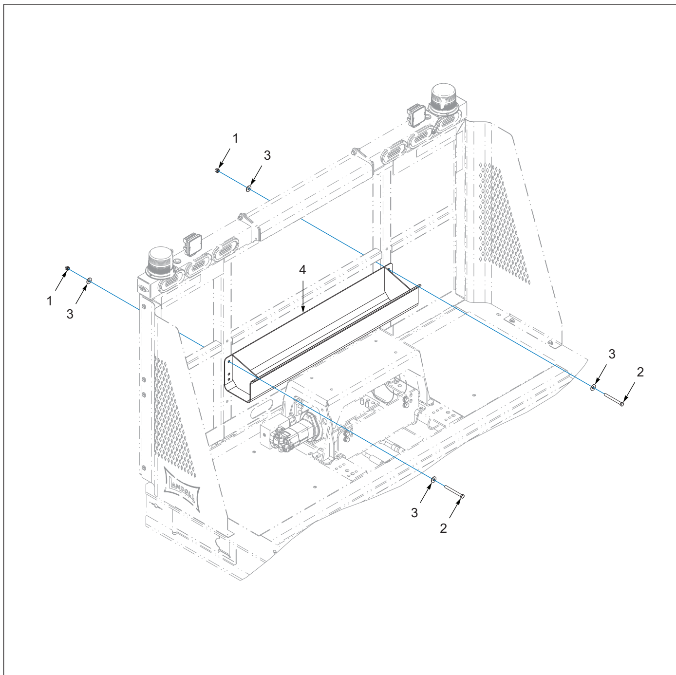
Figure 4-9: Chain Tray, Bulkhead, Bolt-On
