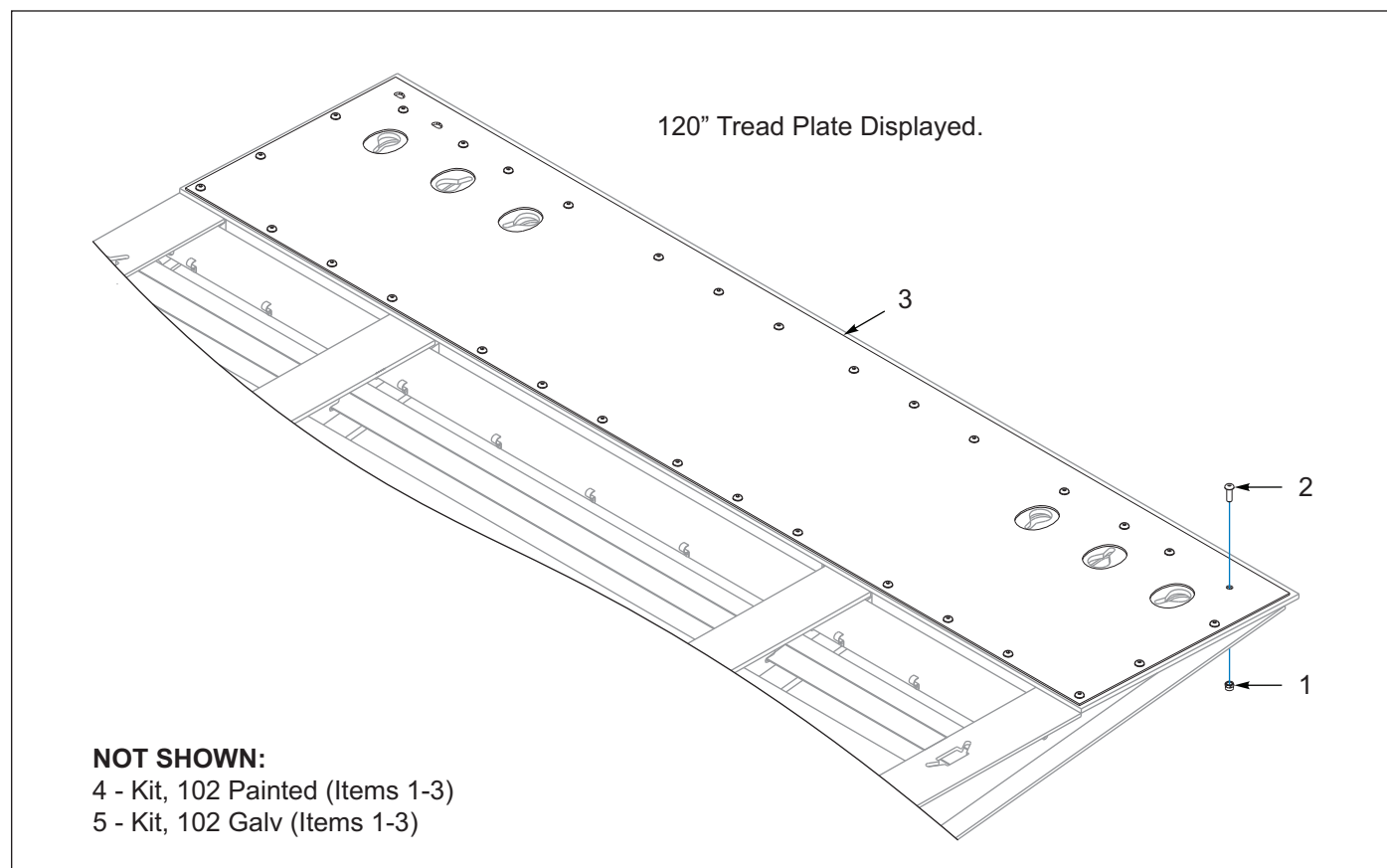
Figure 2-30: Traction Plate, Rear Approach (Options)
