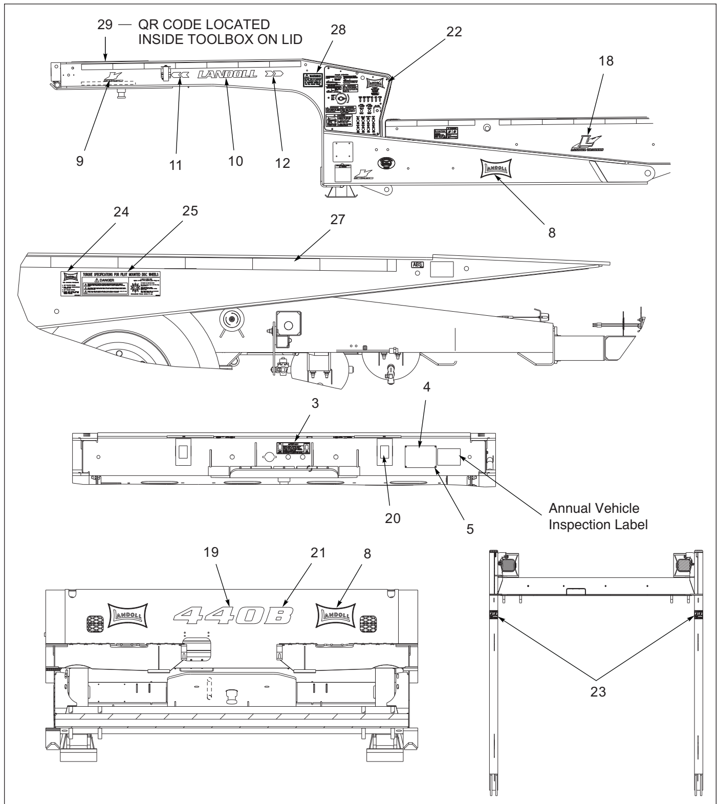
Figure 1-1: Frame Assembly (1 of 2)
