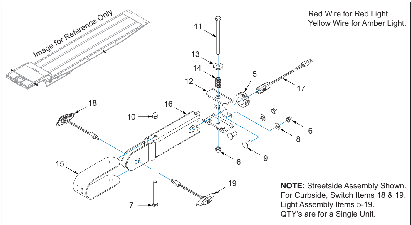
Figure 9-25: Lights, Swing Arm, Marker, Amber &amp; Red (Options) (2 of 2)
