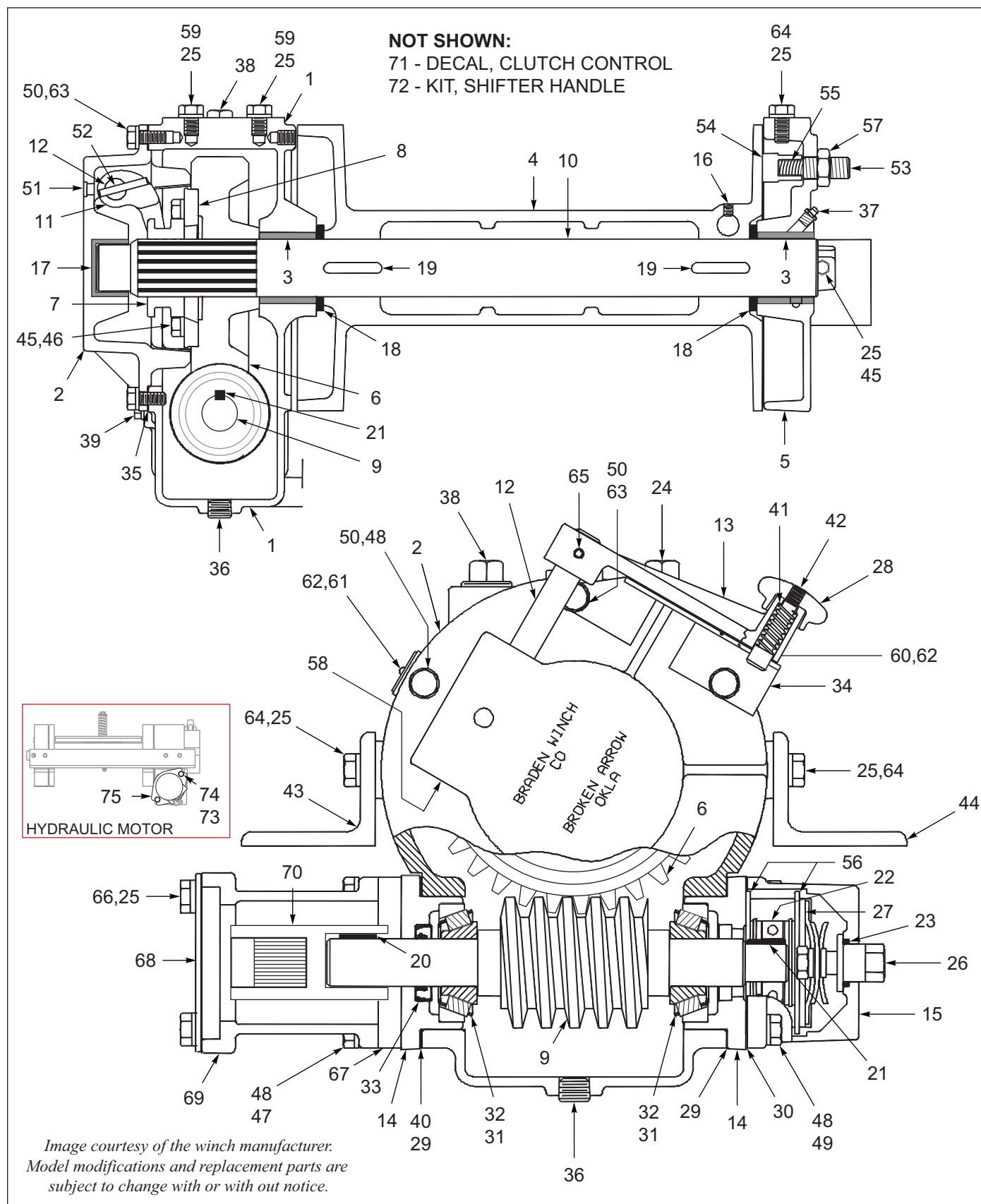
Figure 7-13: Winch Components, Braden 20K, 1-Speed
